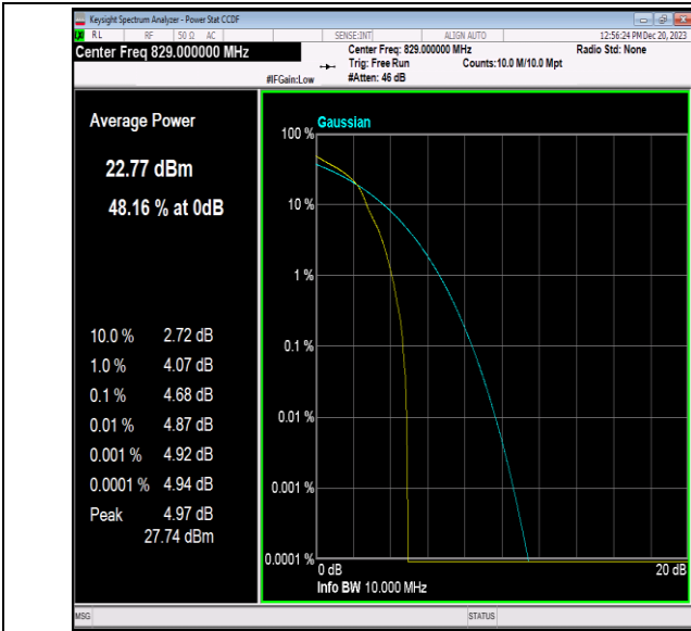
Band5-10MHz-16QAM-20450-1RB#0-PASS
