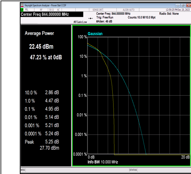
Band5-10MHz-16QAM-20600-1RB#0-PASS
