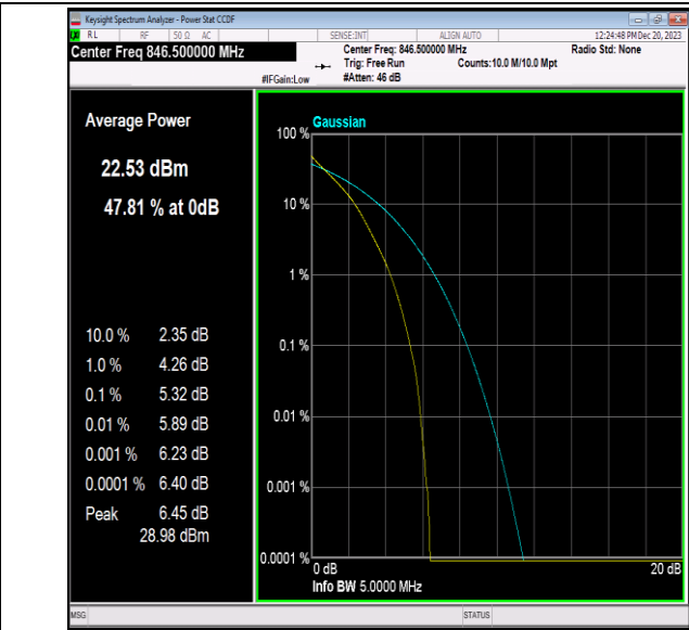
Band5-5MHz-QPSK-20625-25RB#0-PASS
