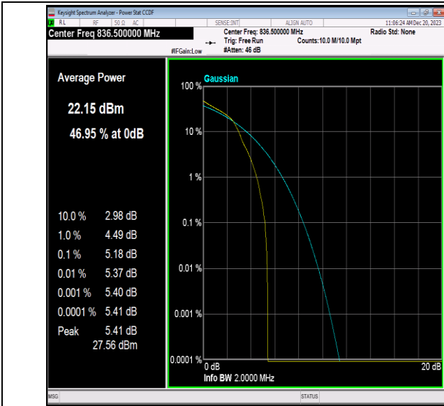
Band5-1.4MHz-16QAM-20525-1RB#0-PASS
