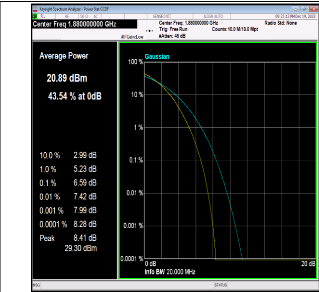
Band2-20MHz-64QAM-18900-100RB#0-PASS
