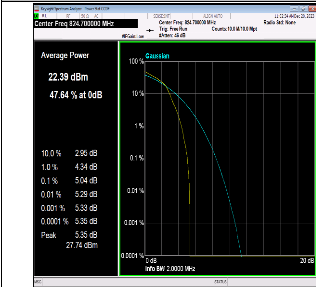
Band5-1.4MHz-16QAM-20407-1RB#0-PASS
