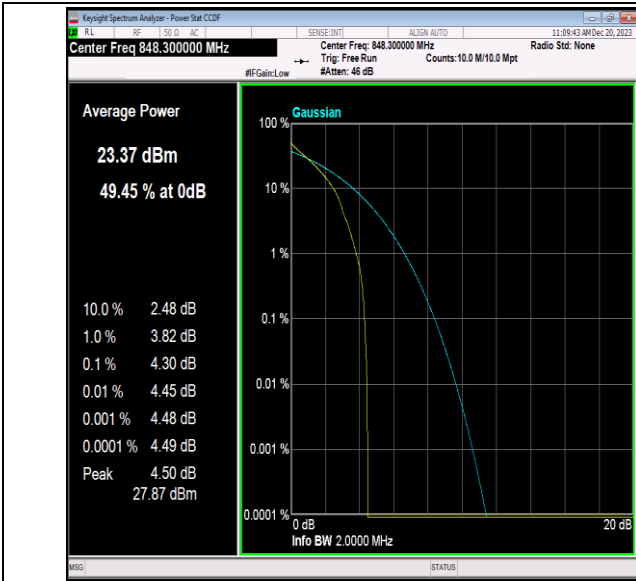
Band5-1.4MHz-QPSK-20643-1RB#0-PASS
