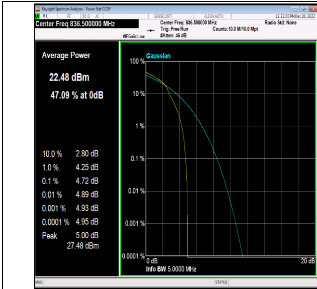
Band5-5MHz-16QAM-20525-1RB#0-PASS
