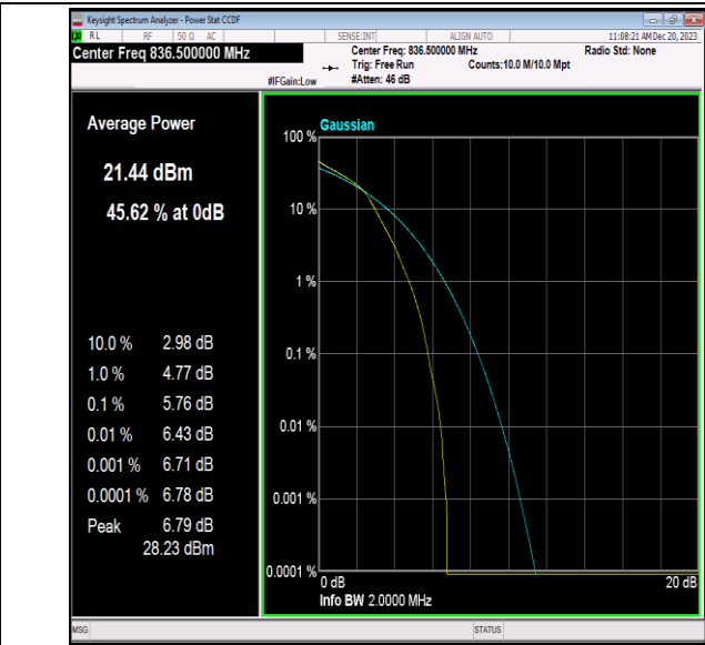
Band5-1.4MHz-16QAM-20525-6RB#0-PASS
