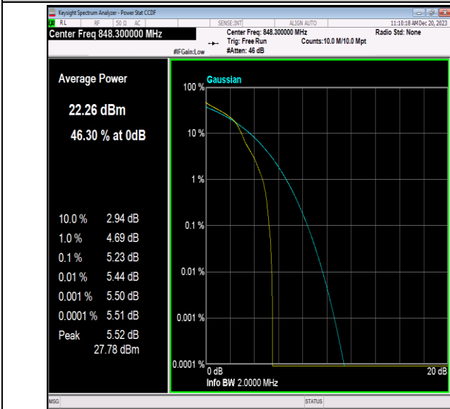
Band5-1.4MHz-16QAM-20643-1RB#0-PASS
