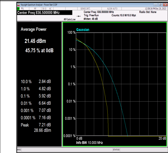
Band5-10MHz-16QAM-20525-50RB#0-PASS
