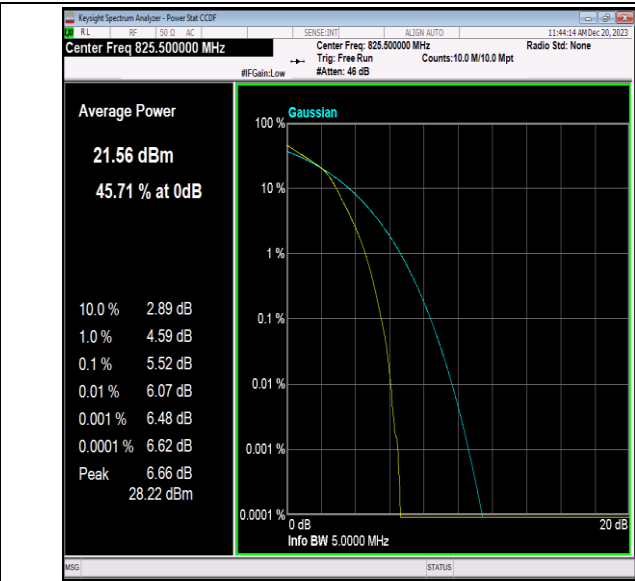
Band5-3MHz-16QAM-20415-15RB#0-PASS
