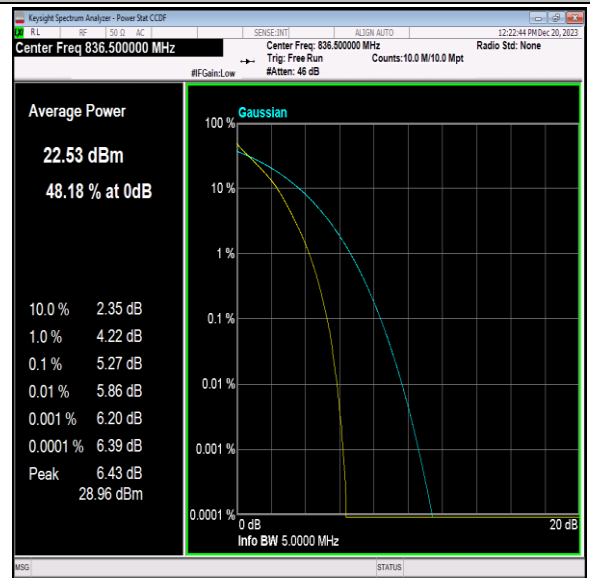
Band5-5MHz-QPSK-20525-25RB#0-PASS
