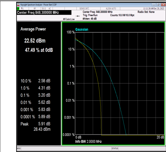
Band5-1.4MHz-QPSK-20643-6RB#0-PASS
