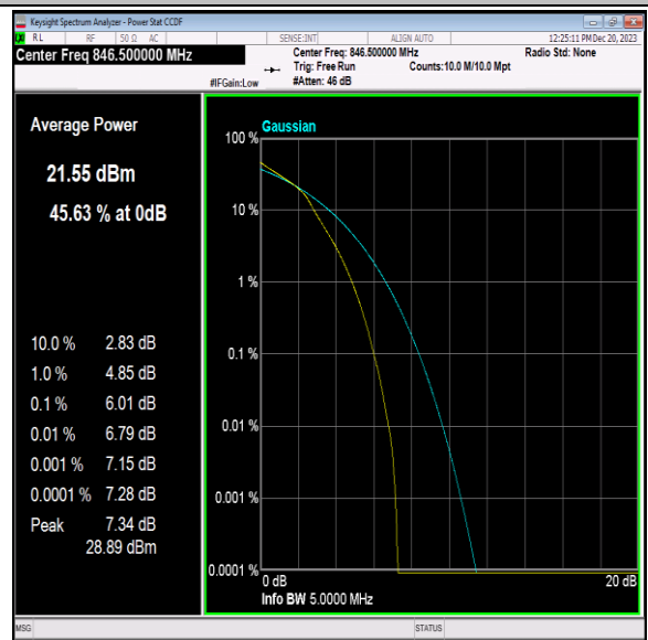
Band5-5MHz-16QAM-20625-25RB#0-PASS
