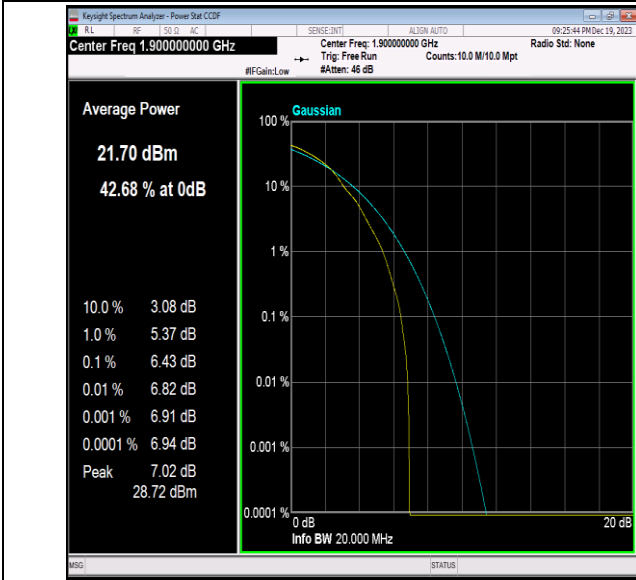
Band2-20MHz-64QAM-19100-1RB#0-PASS
