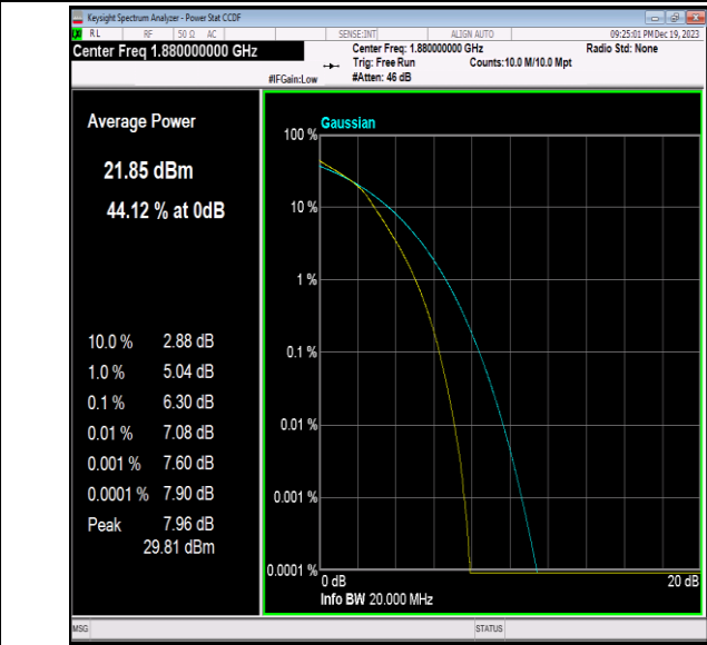
Band2-20MHz-16QAM-18900-100RB#0-PASS
