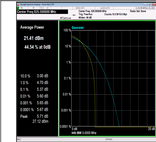
Band5-3MHz-64QAM-20415-1RB#0-PASS
