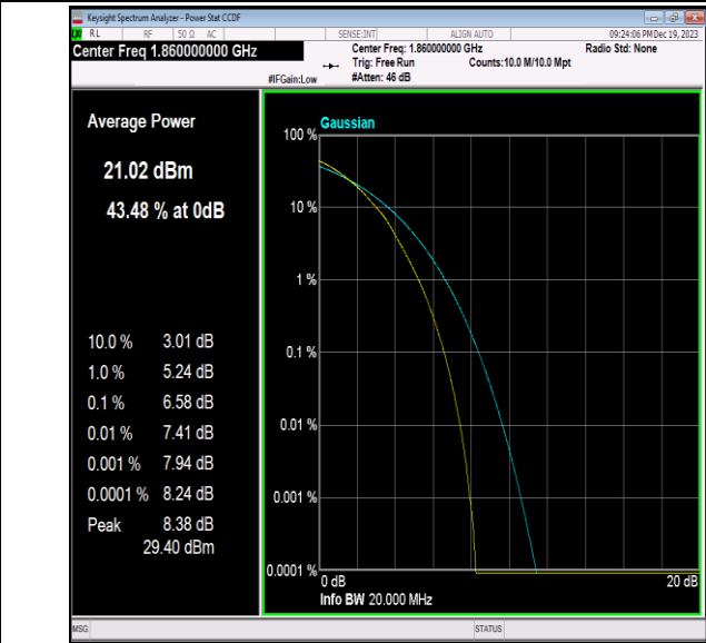
Band2-20MHz-64QAM-18700-100RB#0-PASS
