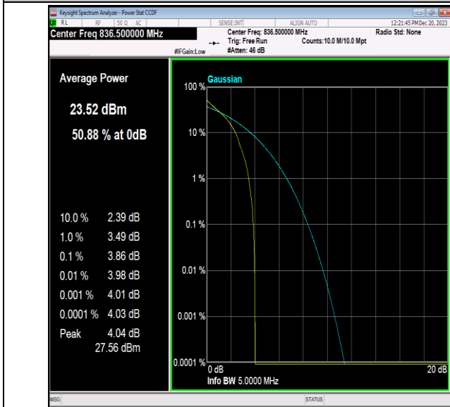
Band5-5MHz-QPSK-20525-1RB#0-PASS
