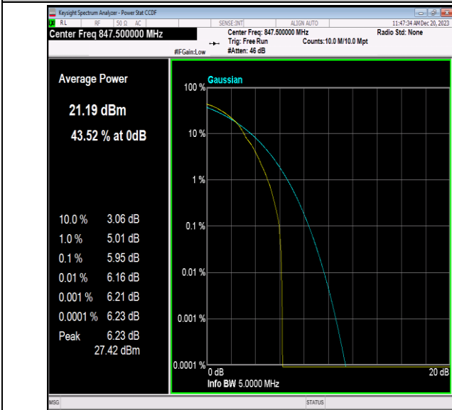
Band5-3MHz-64QAM-20635-1RB#0-PASS
