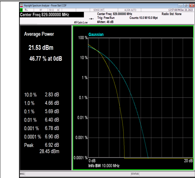
Band5-10MHz-16QAM-20450-50RB#0-PASS
