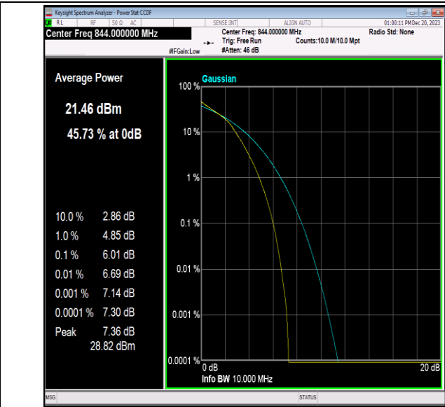
Band5-10MHz-16QAM-20600-50RB#0-PASS
