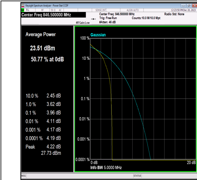
Band5-5MHz-QPSK-20625-1RB#0-PASS
