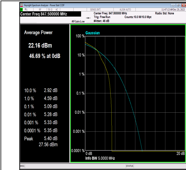
Band5-3MHz-16QAM-20635-1RB#0-PASS
