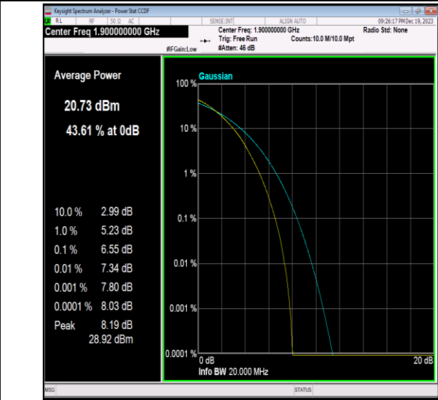
Band2-20MHz-64QAM-19100-100RB#0-PASS
