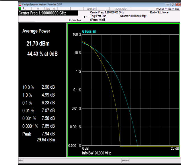
Band2-20MHz-16QAM-19100-100RB#0-PASS
