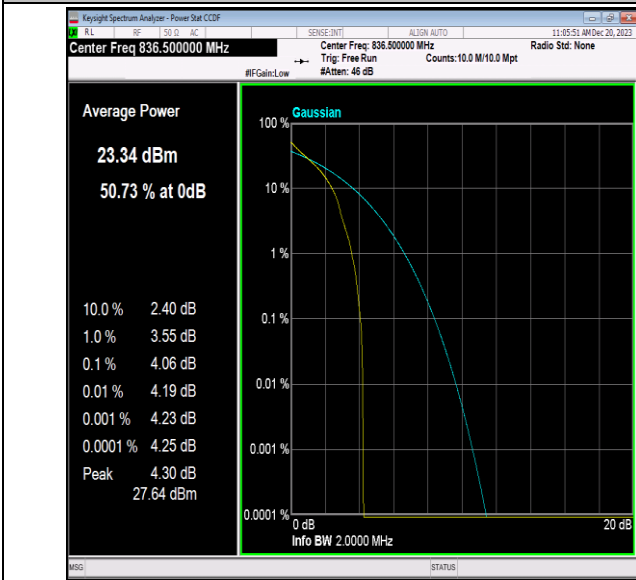
Band5-1.4MHz-QPSK-20525-1RB#0-PASS
