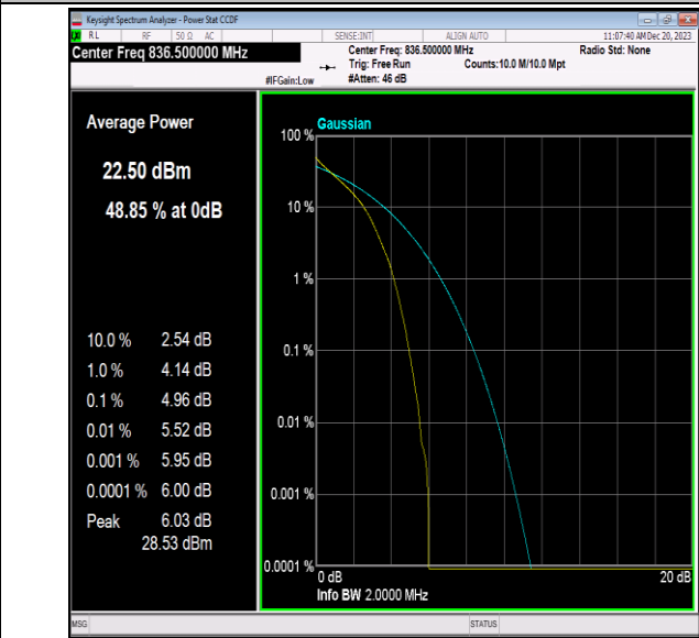
Band5-1.4MHz-QPSK-20525-6RB#0-PASS
