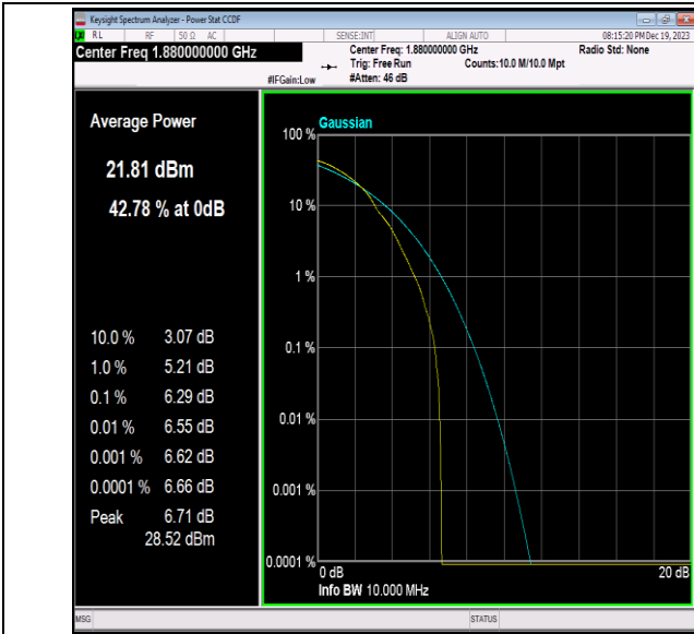
Band2-10MHz-64QAM-18900-1RB#0-PASS
