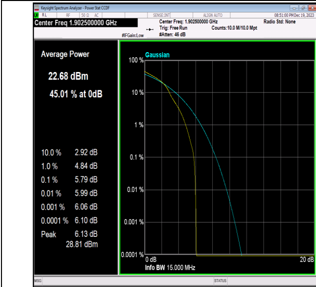
Band2-15MHz-16QAM-19125-1RB#0-PASS
