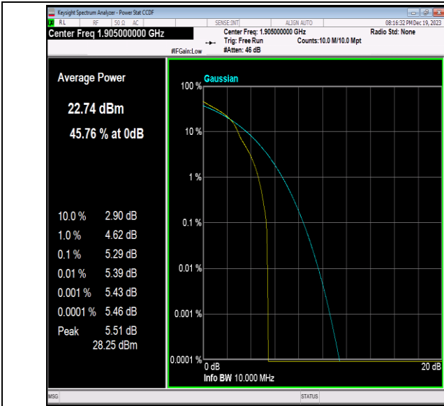
Band2-10MHz-16QAM-19150-1RB#0-PASS
