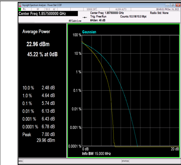
Band2-15MHz-QPSK-18675-75RB#0-PASS
