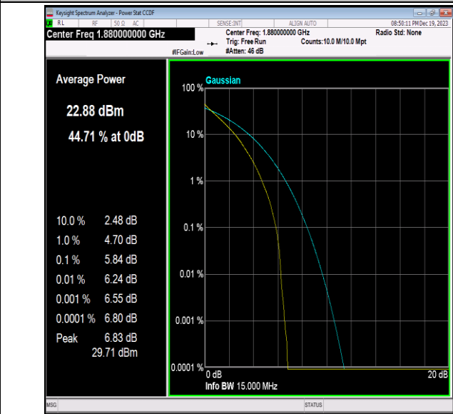
Band2-15MHz-QPSK-18900-75RB#0-PASS
