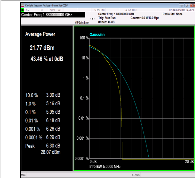
Band2-5MHz-64QAM-18900-1RB#0-PASS
