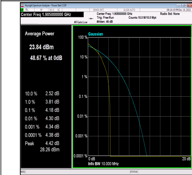
Band2-10MHz-QPSK-19150-1RB#0-PASS
