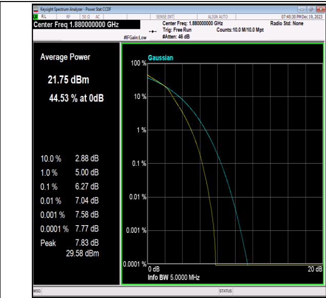
Band2-5MHz-16QAM-18900-25RB#0-PASS
