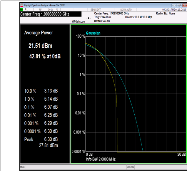
Band2-1.4MHz-64QAM-19193-1RB#0-PASS
