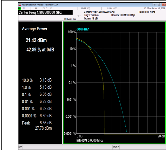
Band2-3MHz-64QAM-19185-1RB#0-PASS
