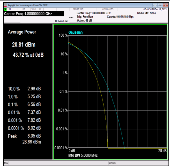
Band2-5MHz-64QAM-18900-25RB#0-PASS
