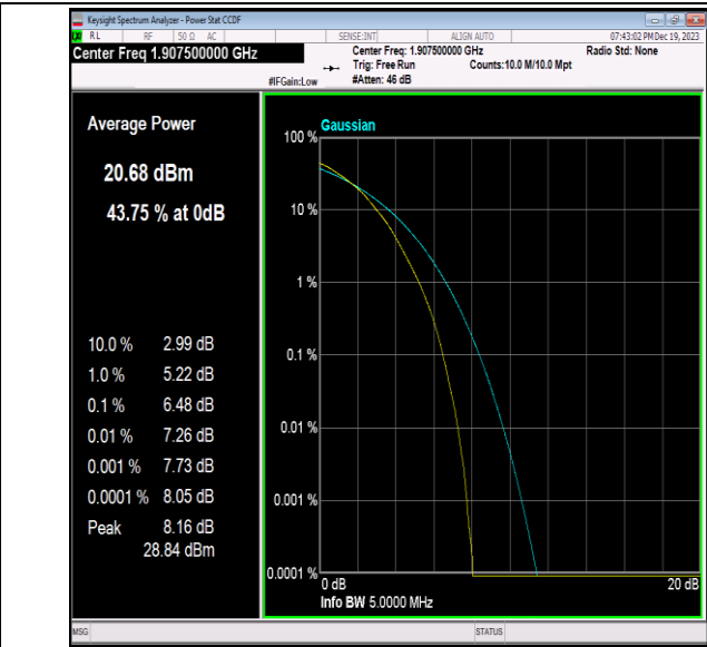
Band2-5MHz-64QAM-19175-25RB#0-PASS
