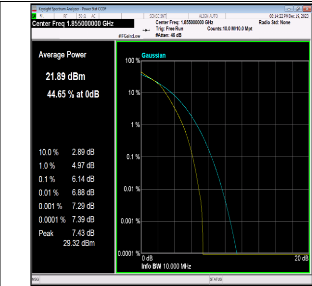
Band2-10MHz-16QAM-18650-50RB#0-PASS
