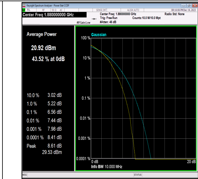
Band2-10MHz-64QAM-18900-50RB#0-PASS
