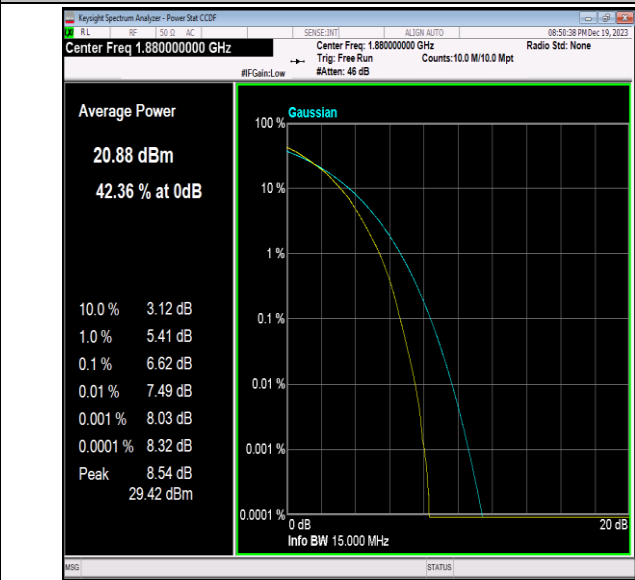
Band2-15MHz-64QAM-18900-75RB#0-PASS
