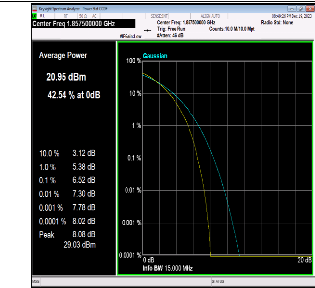
Band2-15MHz-64QAM-18675-75RB#0-PASS
