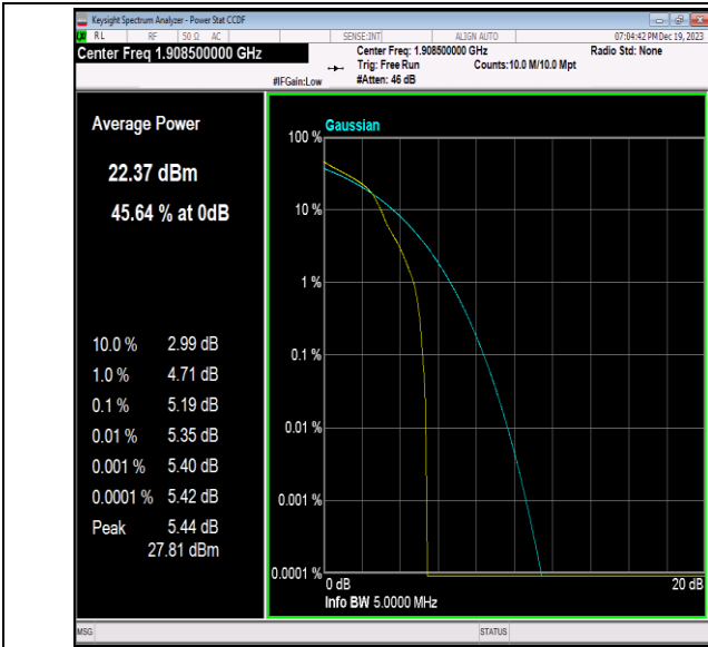
Band2-3MHz-16QAM-19185-1RB#0-PASS
