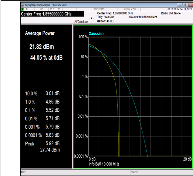
Band2-10MHz-64QAM-18650-1RB#0-PASS
