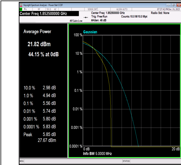
Band2-5MHz-64QAM-18625-1RB#0-PASS
