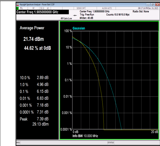
Band2-10MHz-16QAM-19150-50RB#0-PASS
