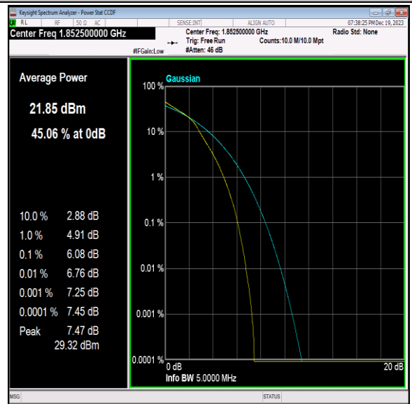
Band2-5MHz-16QAM-18625-25RB#0-PASS
