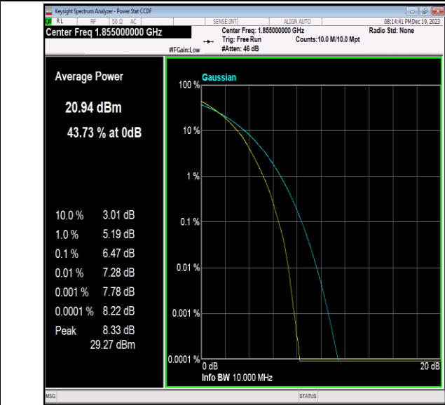
Band2-10MHz-64QAM-18650-50RB#0-PASS
