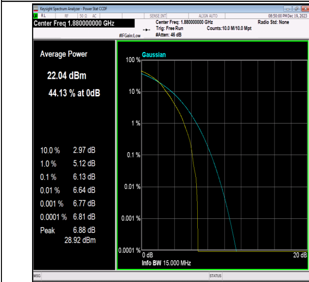
Band2-15MHz-64QAM-18900-1RB#0-PASS
