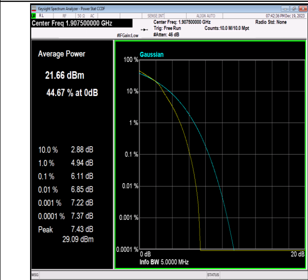
Band2-5MHz-16QAM-19175-25RB#0-PASS
