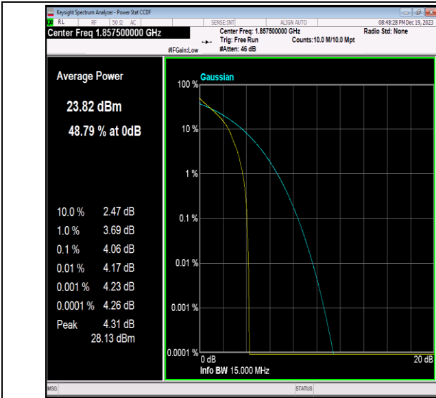
Band2-15MHz-QPSK-18675-1RB#0-PASS
