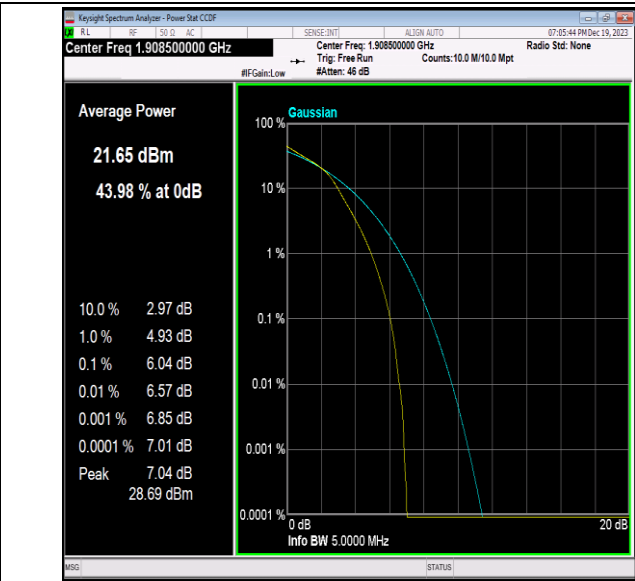
Band2-3MHz-16QAM-19185-15RB#0-PASS
