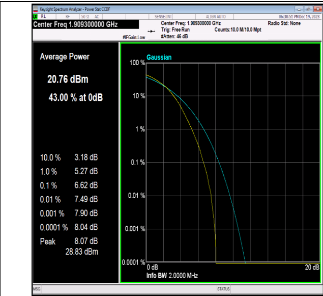
Band2-1.4MHz-64QAM-19193-6RB#0-PASS
