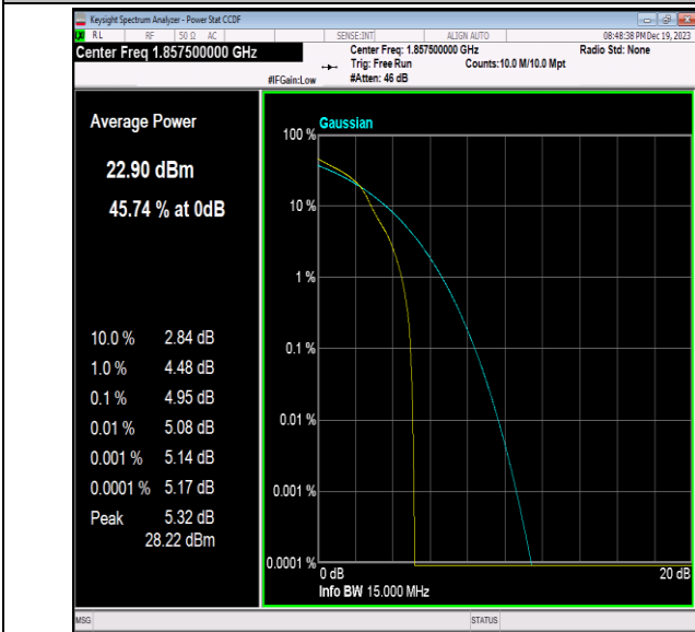
Band2-15MHz-16QAM-18675-1RB#0-PASS
