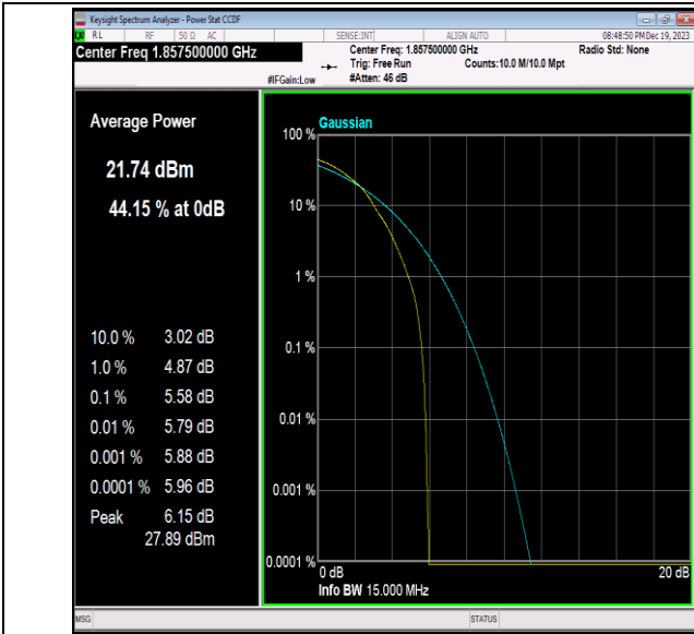
Band2-15MHz-64QAM-18675-1RB#0-PASS
