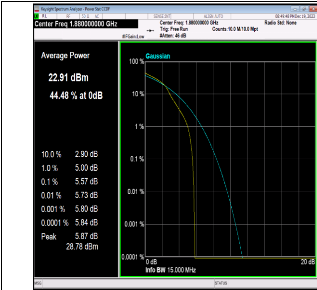
Band2-15MHz-16QAM-18900-1RB#0-PASS
