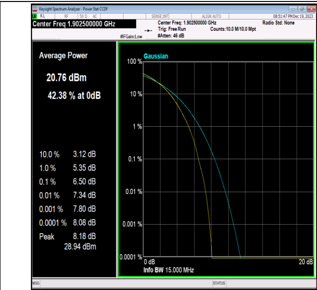
Band2-15MHz-64QAM-19125-75RB#0-PASS
