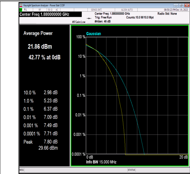
Band2-15MHz-16QAM-18900-75RB#0-PASS
