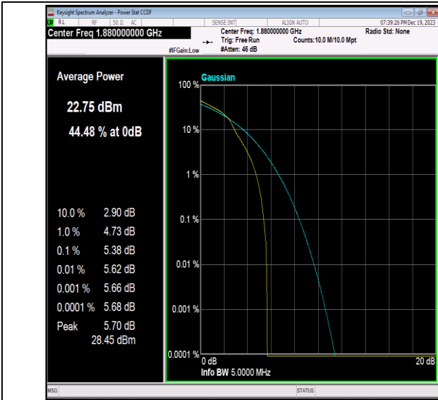
Band2-5MHz-16QAM-18900-1RB#0-PASS
