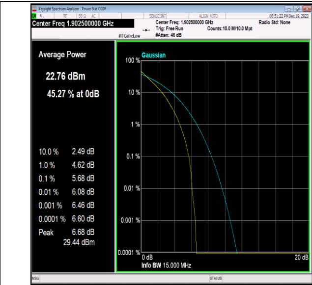
Band2-15MHz-QPSK-19125-75RB#0-PASS
