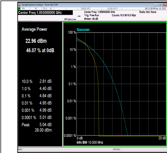
Band2-10MHz-16QAM-18650-1RB#0-PASS
