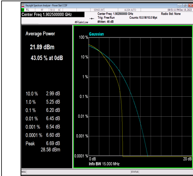
Band2-15MHz-64QAM-19125-1RB#0-PASS
