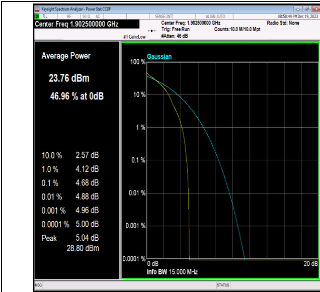
Band2-15MHz-QPSK-19125-1RB#0-PASS
