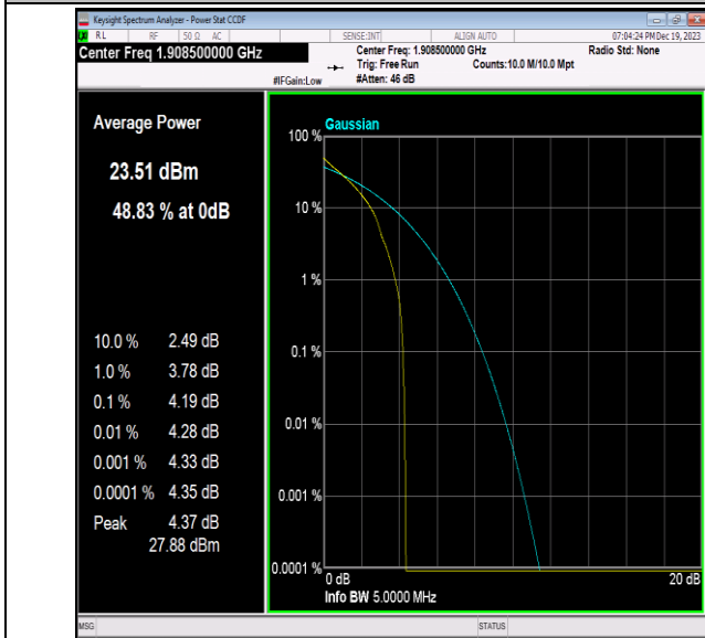
Band2-3MHz-QPSK-19185-1RB#0-PASS
