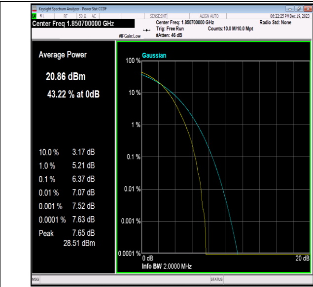
Band2-1.4MHz-64QAM-18607-6RB#0-PASS
