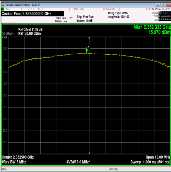
40(2350-2360)-5MHz-QPSK-39175-25RB#0-PASS
