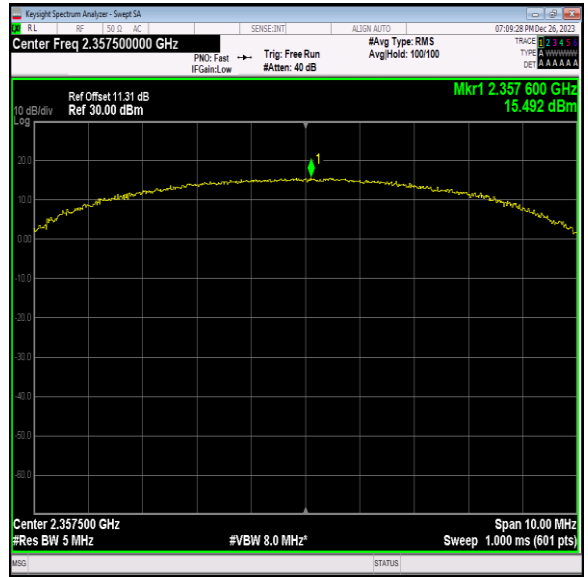
40(2350-2360)-5MHz-16QAM-39225-25RB#0-PASS
