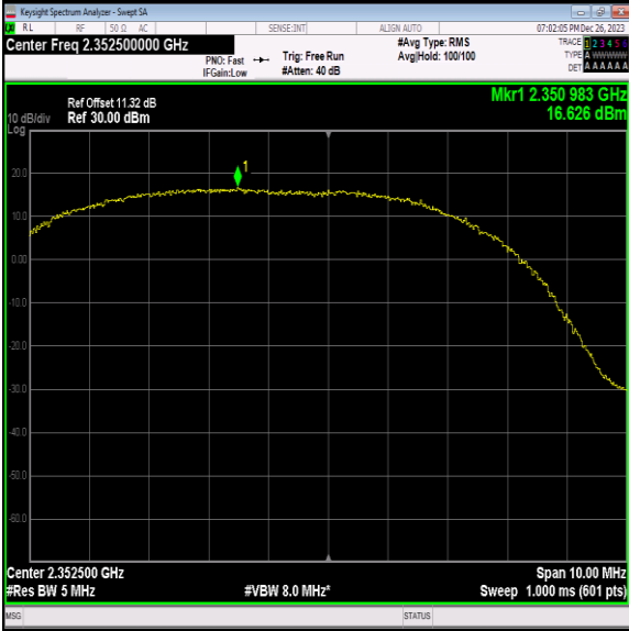
40(2350-2360)-5MHz-16QAM-39175-12RB#0-PASS
