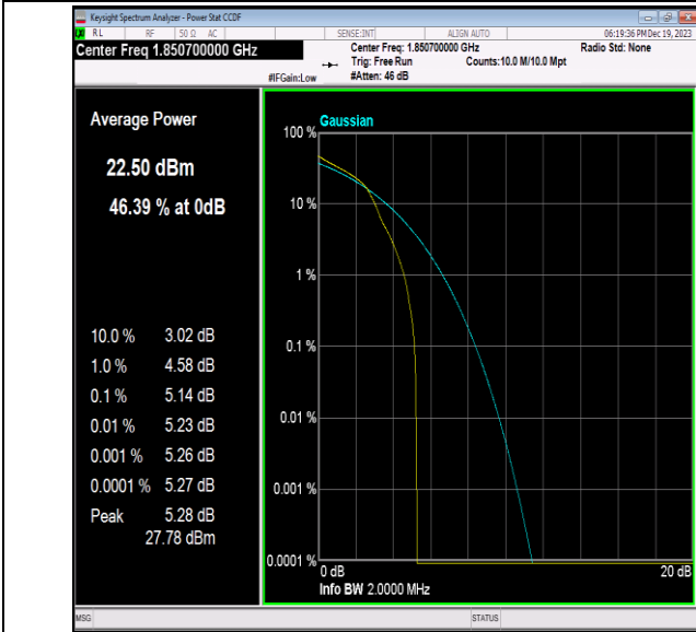
Band2-1.4MHz-16QAM-18607-1RB#0-PASS
