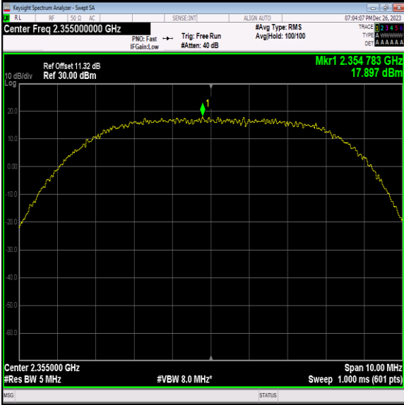
40(2350-2360)-5MHz-QPSK-39200-1RB#12-PASS
