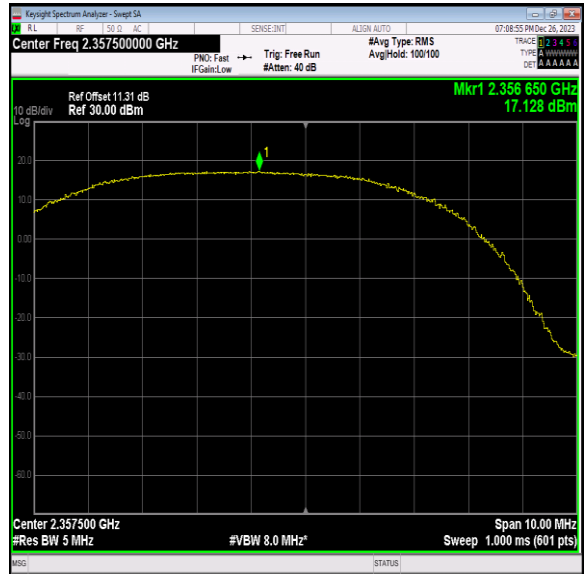
40(2350-2360)-5MHz-QPSK-39225-12RB#11-PASS
