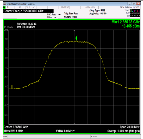
40(2350-2360)-10MHz-16QAM-39200-1RB#24-PASS
