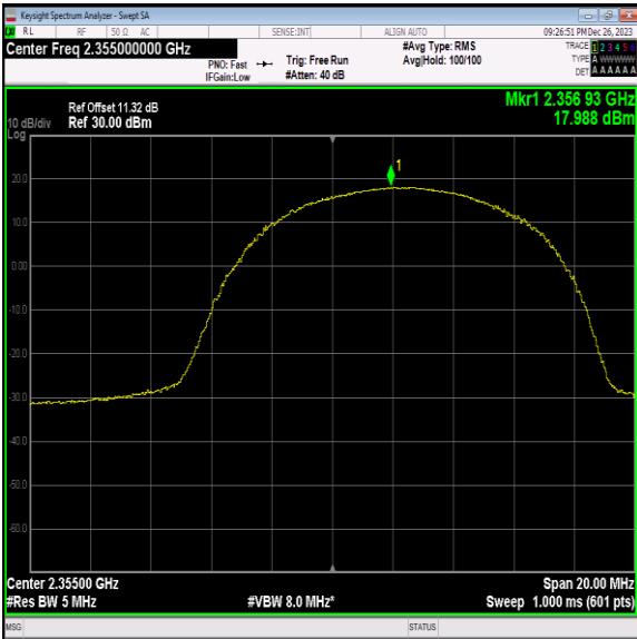
40(2350-2360)-10MHz-64QAM-39200-25RB#25-PASS
