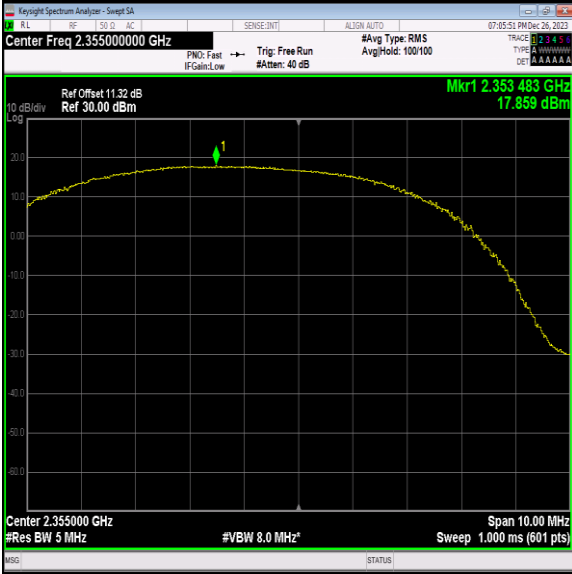
40(2350-2360)-5MHz-QPSK-39200-12RB#11-PASS
