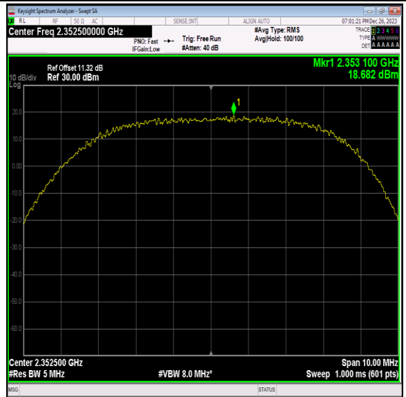
40(2350-2360)-5MHz-64QAM-39175-1RB#12-PASS
