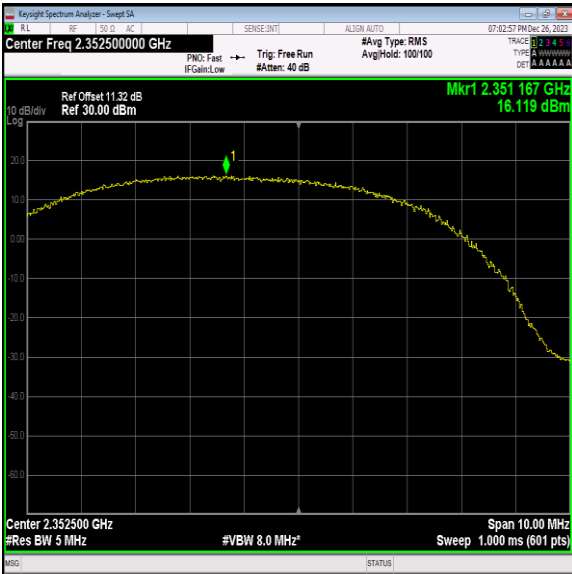
40(2350-2360)-5MHz-16QAM-39175-12RB#11-PASS
