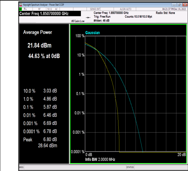
Band2-1.4MHz-16QAM-18607-6RB#0-PASS
