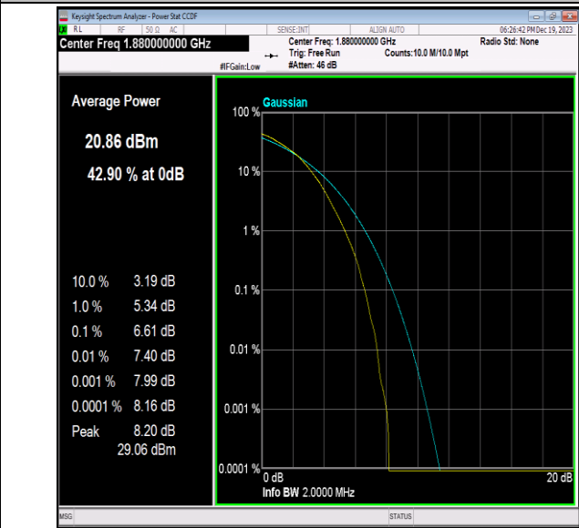
Band2-1.4MHz-64QAM-18900-6RB#0-PASS
