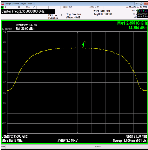
40(2350-2360)-10MHz-16QAM-39200-50RB#0-PASS
