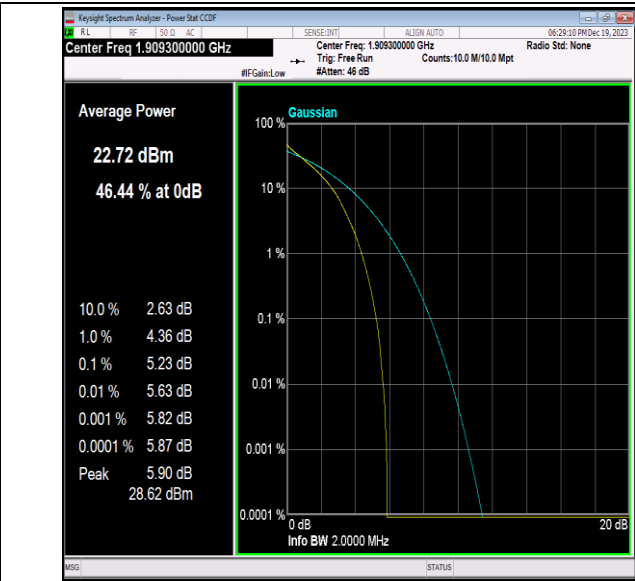
Band2-1.4MHz-QPSK-19193-6RB#0-PASS
