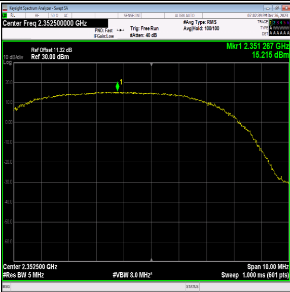
40(2350-2360)-5MHz-64QAM-39175-12RB#6-PASS
