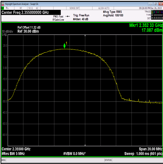
40(2350-2360)-10MHz-64QAM-39200-25RB#0-PASS
