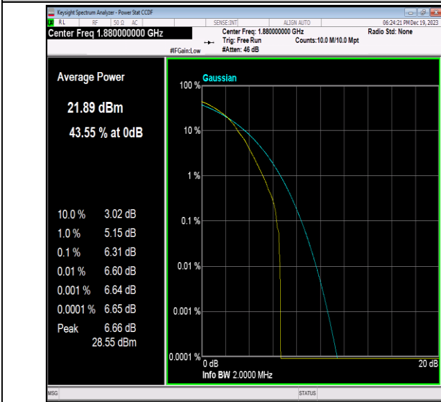
Band2-1.4MHz-64QAM-18900-1RB#0-PASS
