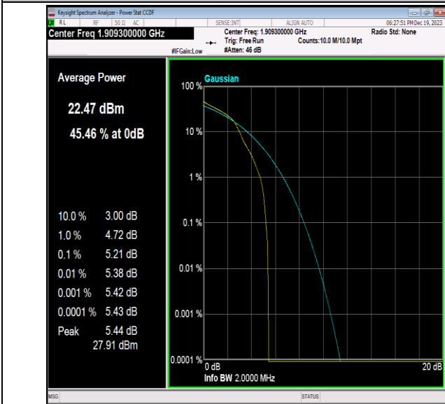
Band2-1.4MHz-16QAM-19193-1RB#0-PASS
