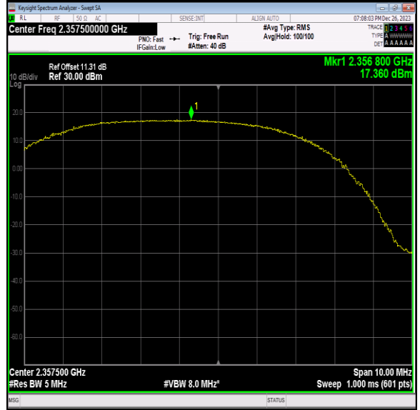
40(2350-2360)-5MHz-QPSK-39225-12RB#0-PASS
