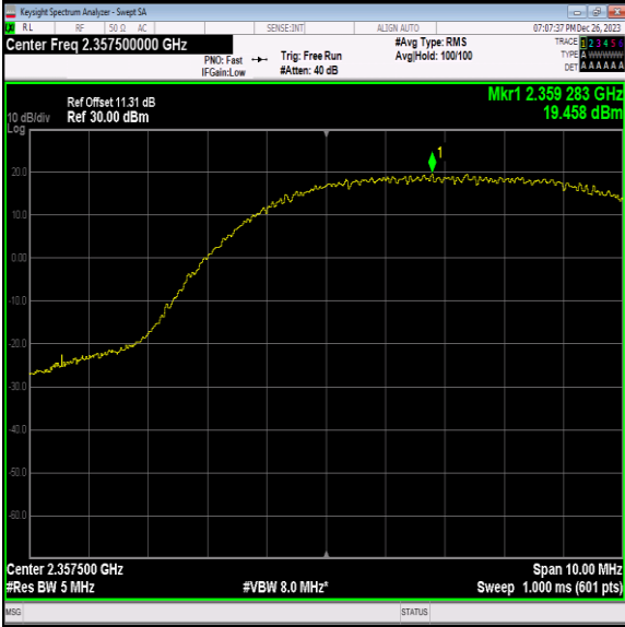
40(2350-2360)-5MHz-QPSK-39225-1RB#24-PASS
