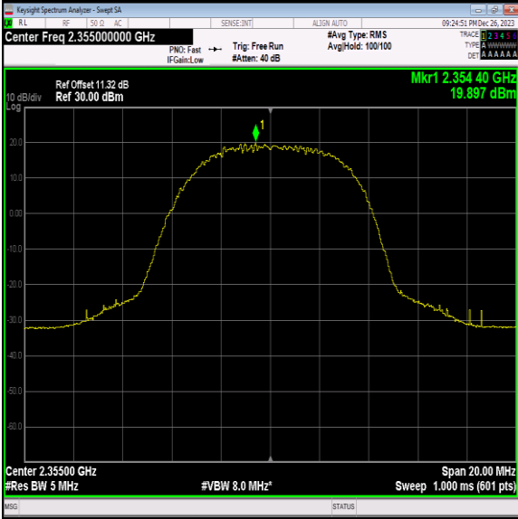
40(2350-2360)-10MHz-QPSK-39200-1RB#24-PASS
