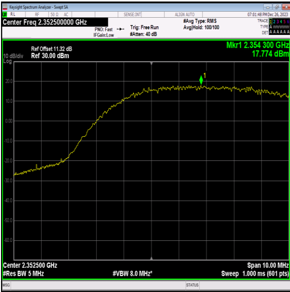
40(2350-2360)-5MHz-64QAM-39175-1RB#24-PASS
