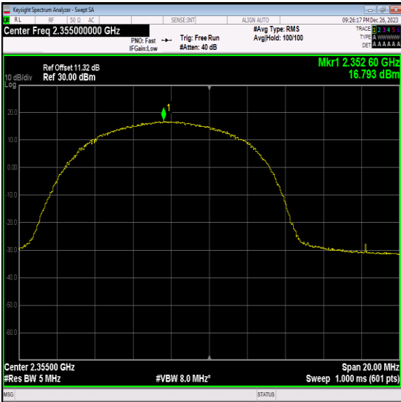
40(2350-2360)-10MHz-16QAM-39200-25RB#12-PASS
