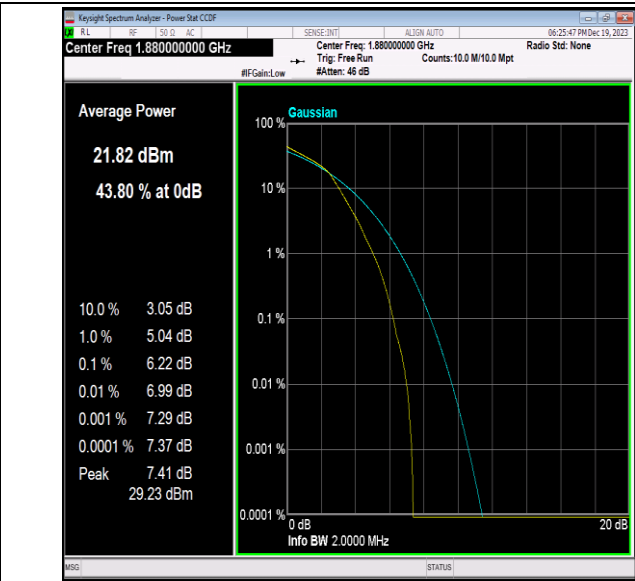
Band2-1.4MHz-16QAM-18900-6RB#0-PASS
