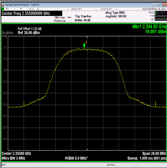
40(2350-2360)-10MHz-64QAM-39200-1RB#24-PASS
