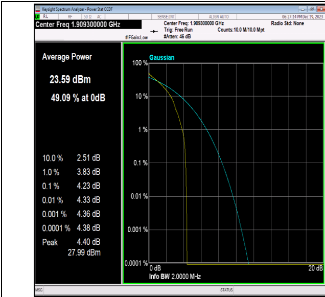
Band2-1.4MHz-QPSK-19193-1RB#0-PASS
