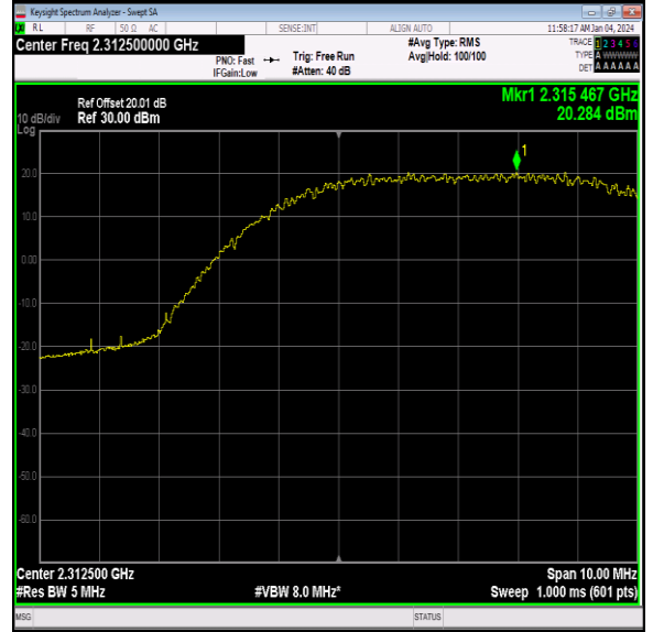
40(2305-2315)-5MHz-16QAM-38775-1RB#24-PASS
