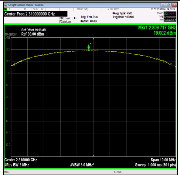
40(2305-2315)-5MHz-64QAM-38750-25RB#0-PASS
