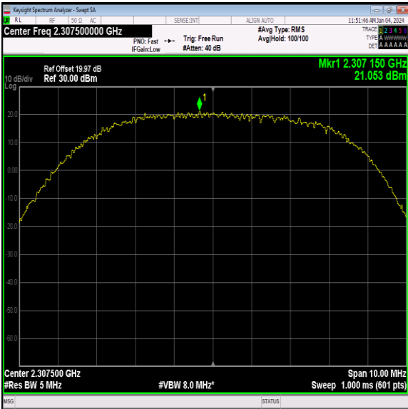
40(2305-2315)-5MHz-16QAM-38725-1RB#12-PASS
