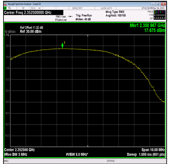
40(2350-2360)-5MHz-QPSK-39175-12RB#0-PASS
