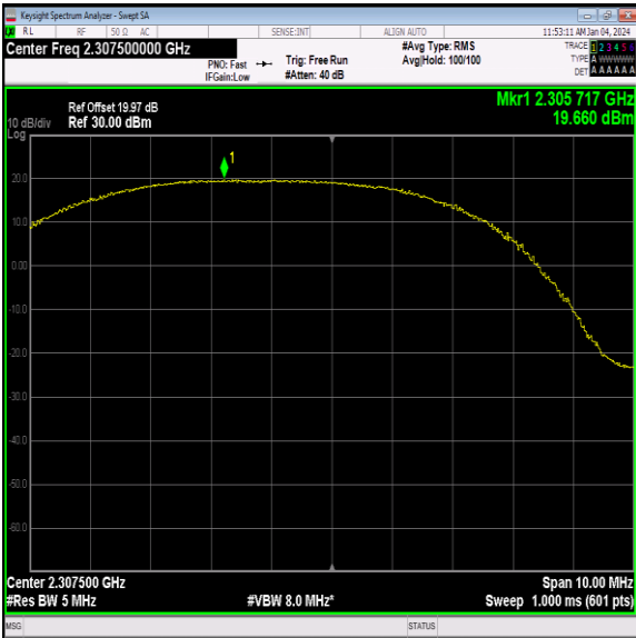
40(2305-2315)-5MHz-64QAM-38725-12RB#6-PASS
