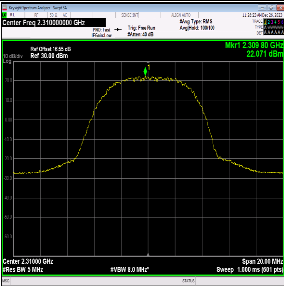
40(2305-2315)-10MHz-64QAM-38750-1RB#24-PASS
