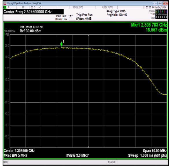
40(2305-2315)-5MHz-16QAM-38725-12RB#6-PASS
