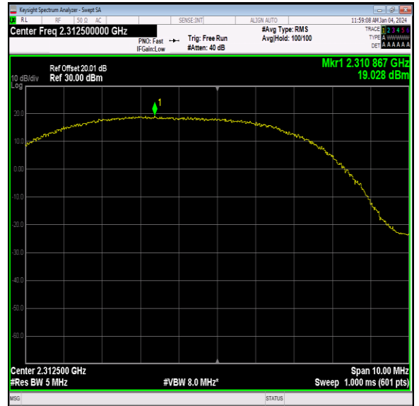
40(2305-2315)-5MHz-16QAM-38775-12RB#6-PASS
