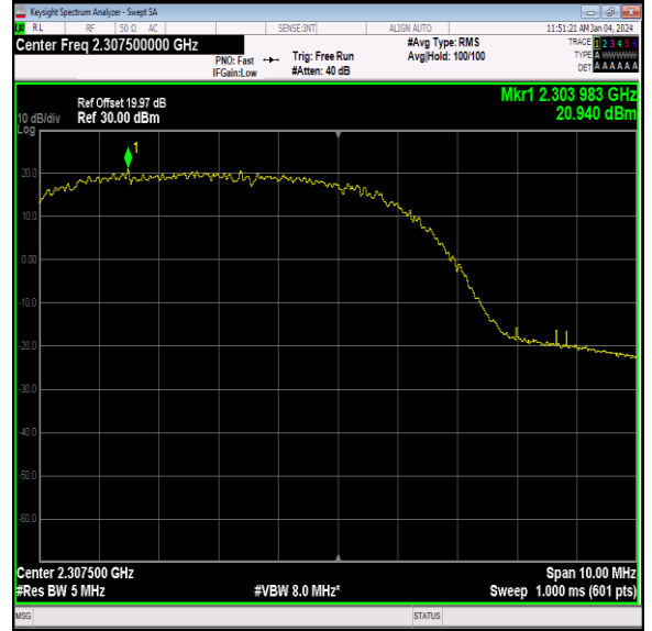
40(2305-2315)-5MHz-16QAM-38725-1RB#0-PASS
