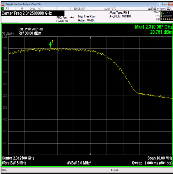
40(2305-2315)-5MHz-64QAM-38775-1RB#0-PASS
