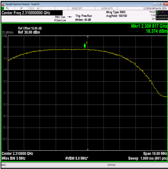
40(2305-2315)-5MHz-16QAM-38750-12RB#6-PASS
