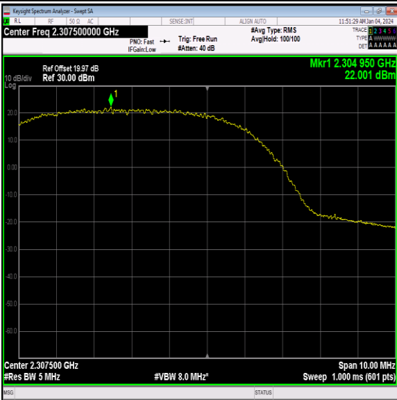
40(2305-2315)-5MHz-64QAM-38725-1RB#0-PASS
