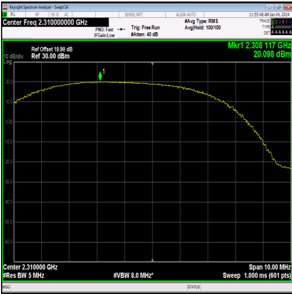
40(2305-2315)-5MHz-64QAM-38750-12RB#0-PASS
