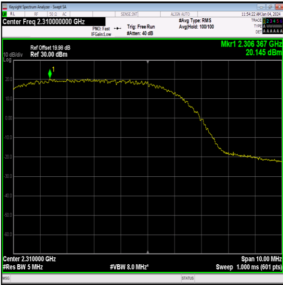
40(2305-2315)-5MHz-16QAM-38750-1RB#0-PASS
