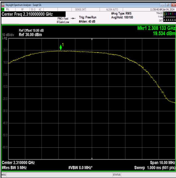
40(2305-2315)-5MHz-64QAM-38750-12RB#11-PASS
