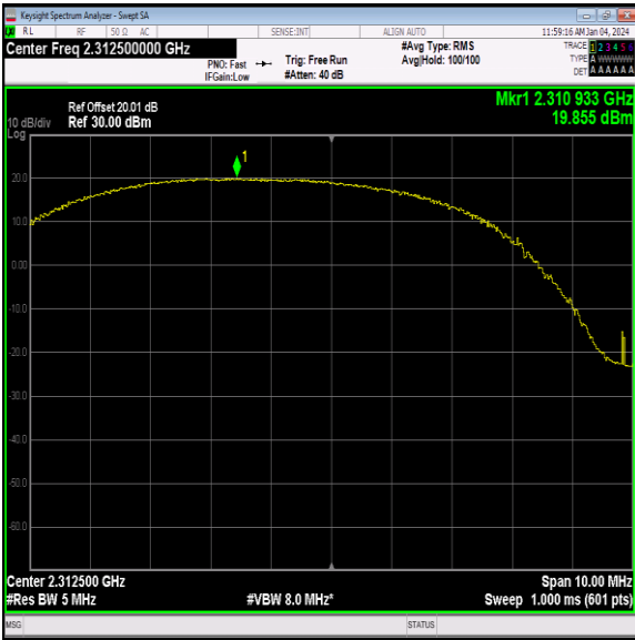
40(2305-2315)-5MHz-64QAM-38775-12RB#6-PASS
