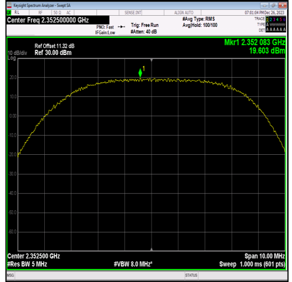
40(2350-2360)-5MHz-QPSK-39175-1RB#12-PASS
