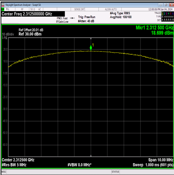
40(2305-2315)-5MHz-64QAM-38775-25RB#0-PASS
