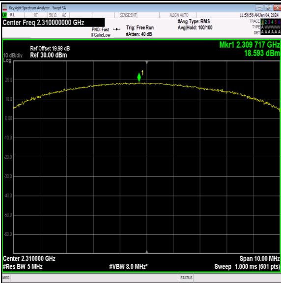
40(2305-2315)-5MHz-16QAM-38750-25RB#0-PASS
