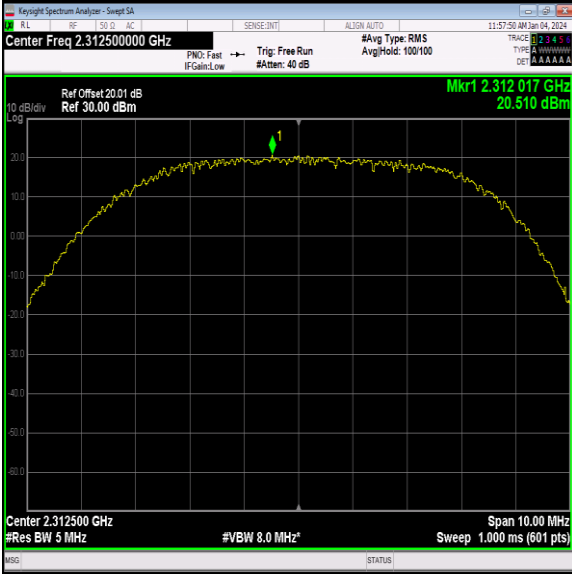
40(2305-2315)-5MHz-16QAM-38775-1RB#12-PASS
