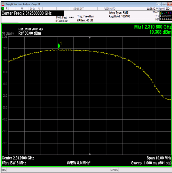
40(2305-2315)-5MHz-16QAM-38775-12RB#0-PASS
