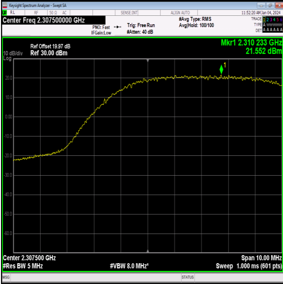
40(2305-2315)-5MHz-64QAM-38725-1RB#24-PASS
