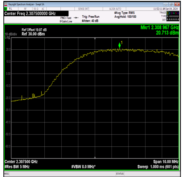
40(2305-2315)-5MHz-16QAM-38725-1RB#24-PASS
