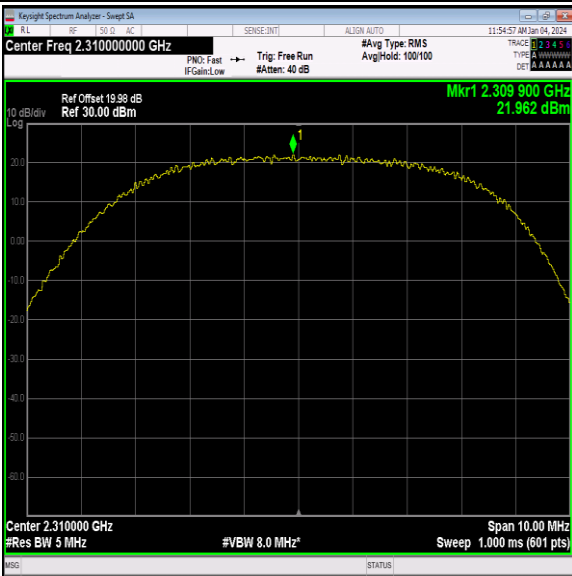
40(2305-2315)-5MHz-64QAM-38750-1RB#12-PASS
