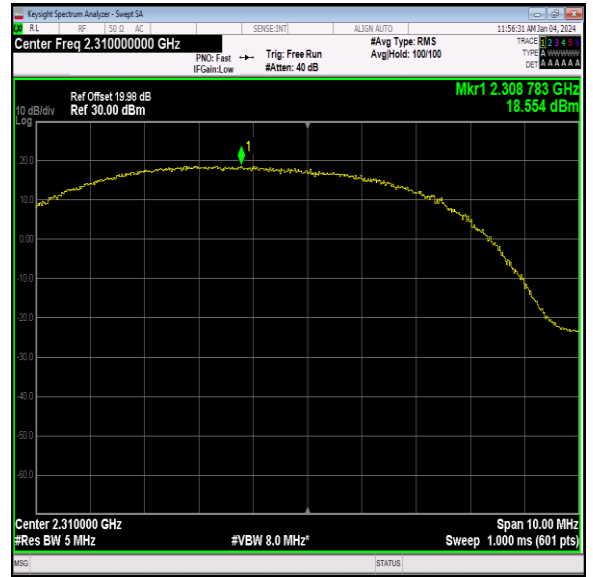
40(2305-2315)-5MHz-16QAM-38750-12RB#11-PASS
