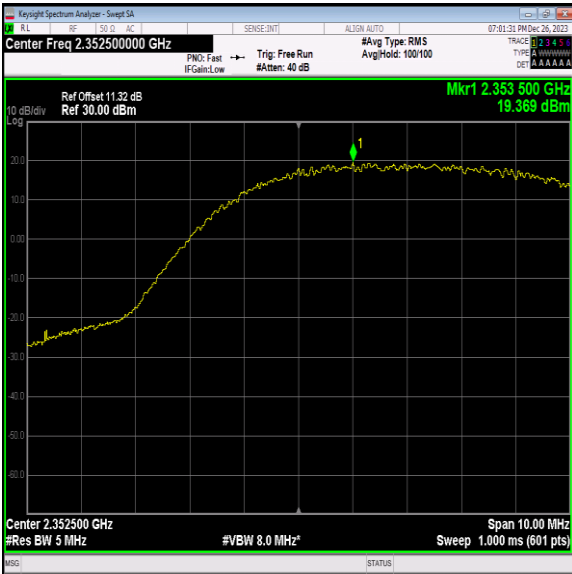
40(2350-2360)-5MHz-QPSK-39175-1RB#24-PASS
