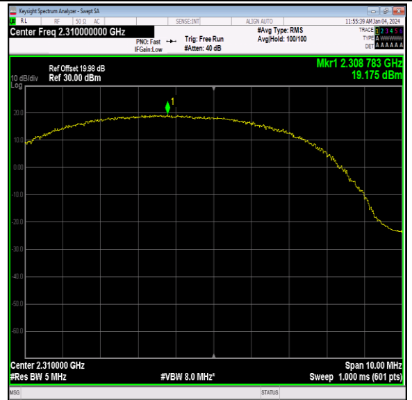
40(2305-2315)-5MHz-16QAM-38750-12RB#0-PASS
