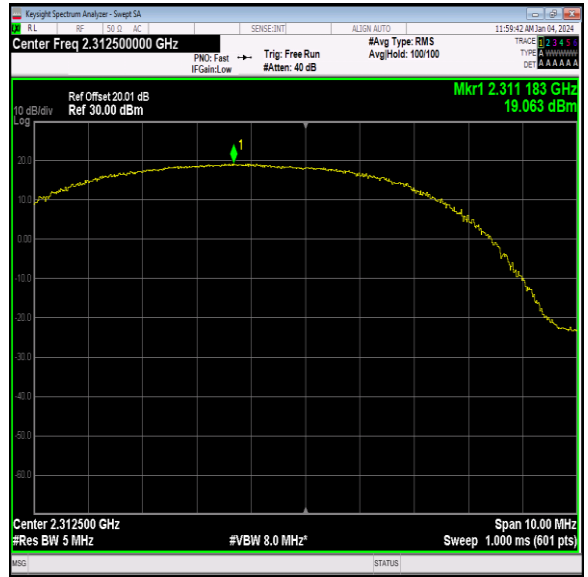
40(2305-2315)-5MHz-64QAM-38775-12RB#11-PASS
