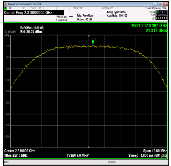
40(2305-2315)-5MHz-16QAM-38750-1RB#12-PASS
