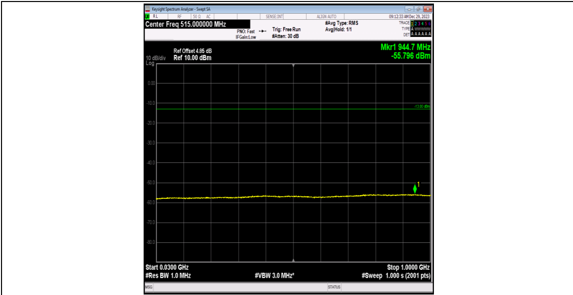
Band4-1413-1-30~1000MHz-PASS
