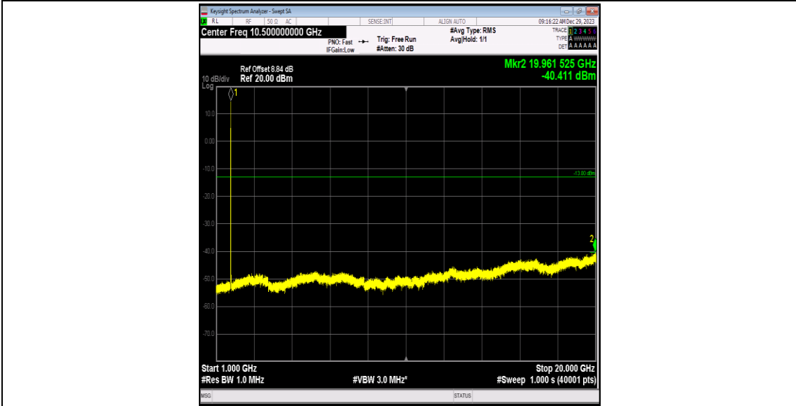
Band4-1413-2-1000~20000MHz-PASS
