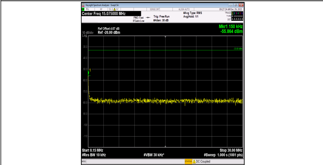
Band4-1513-5-0.15~30MHz-PASS
