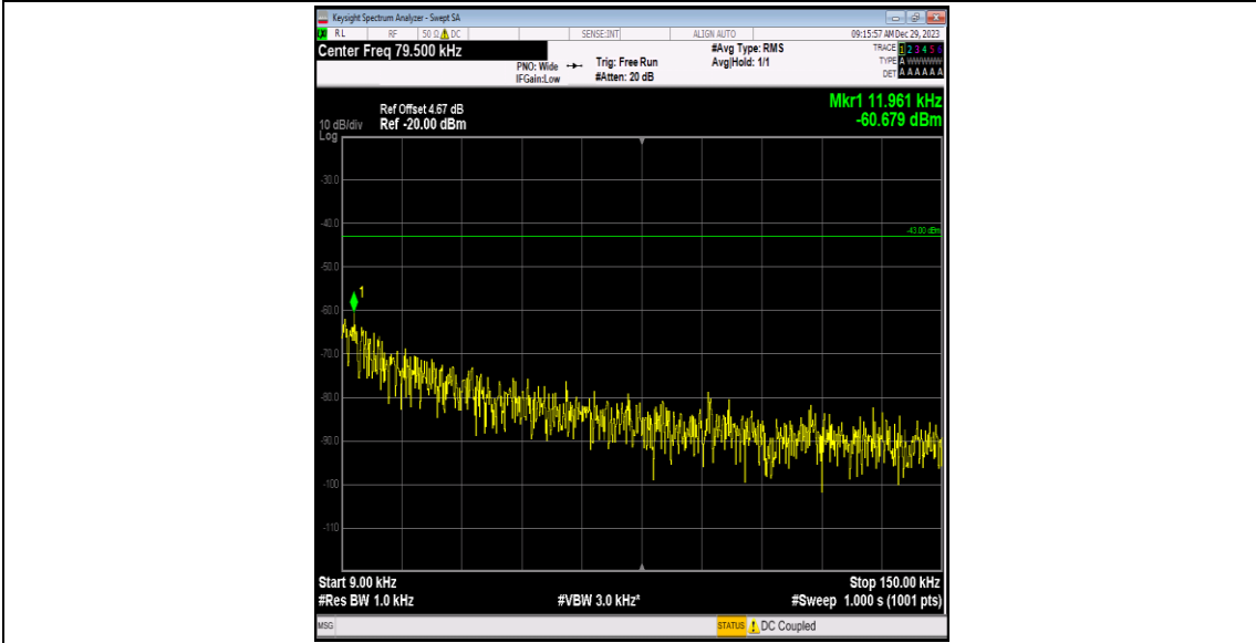
Band4-1413-2-0.009~0.15MHz-PASS
