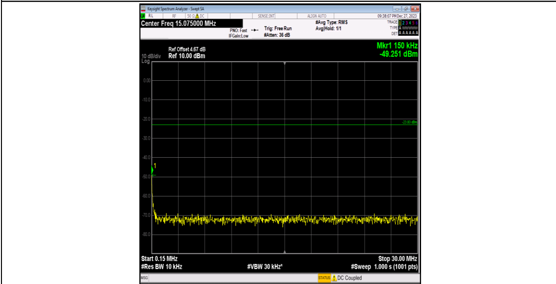
Band5-4132-2-0.15~30MHz-PASS
