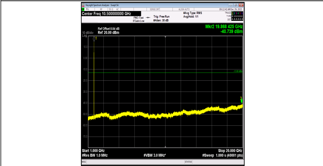
Band4-1413-1-1000~20000MHz-PASS
