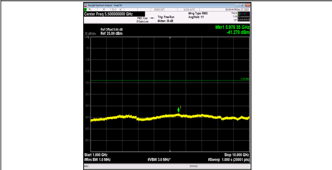
Band5-4132-5-1000~10000MHz-PASS
