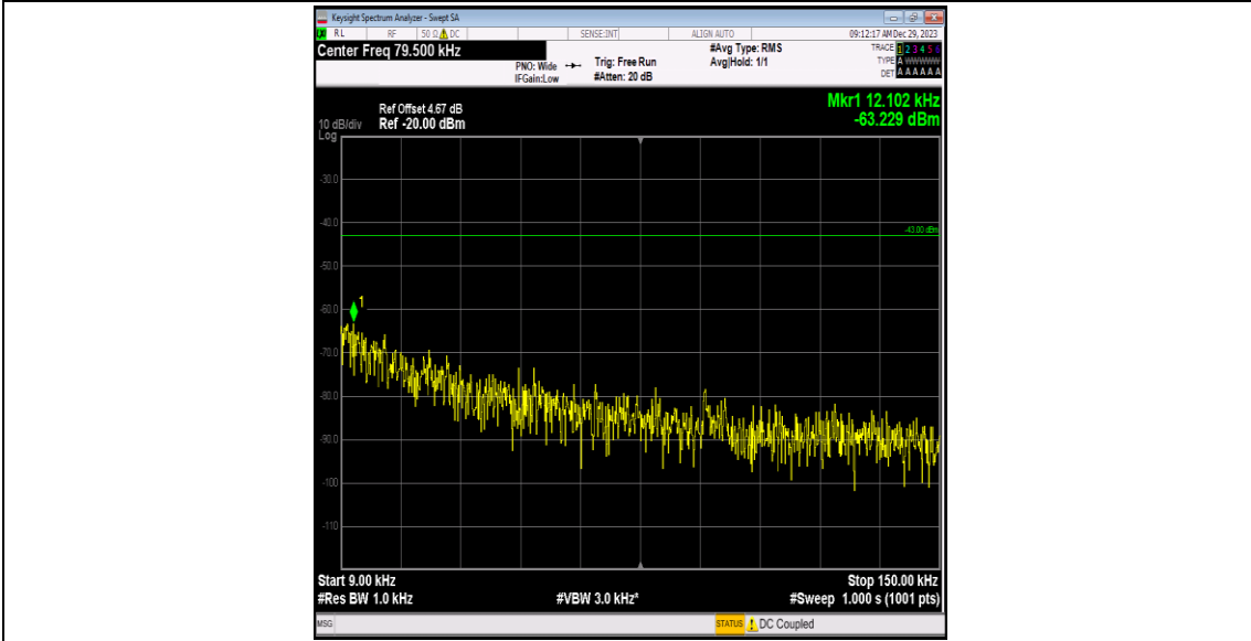
Band4-1413-1-0.009~0.15MHz-PASS
