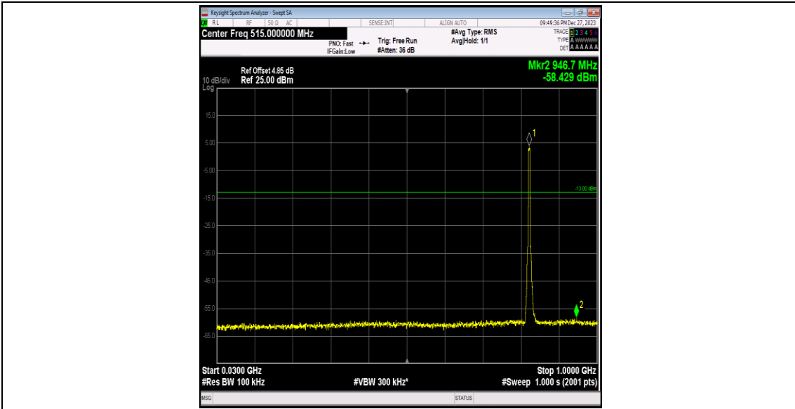
Band5-4132-5-30~1000MHz-PASS
