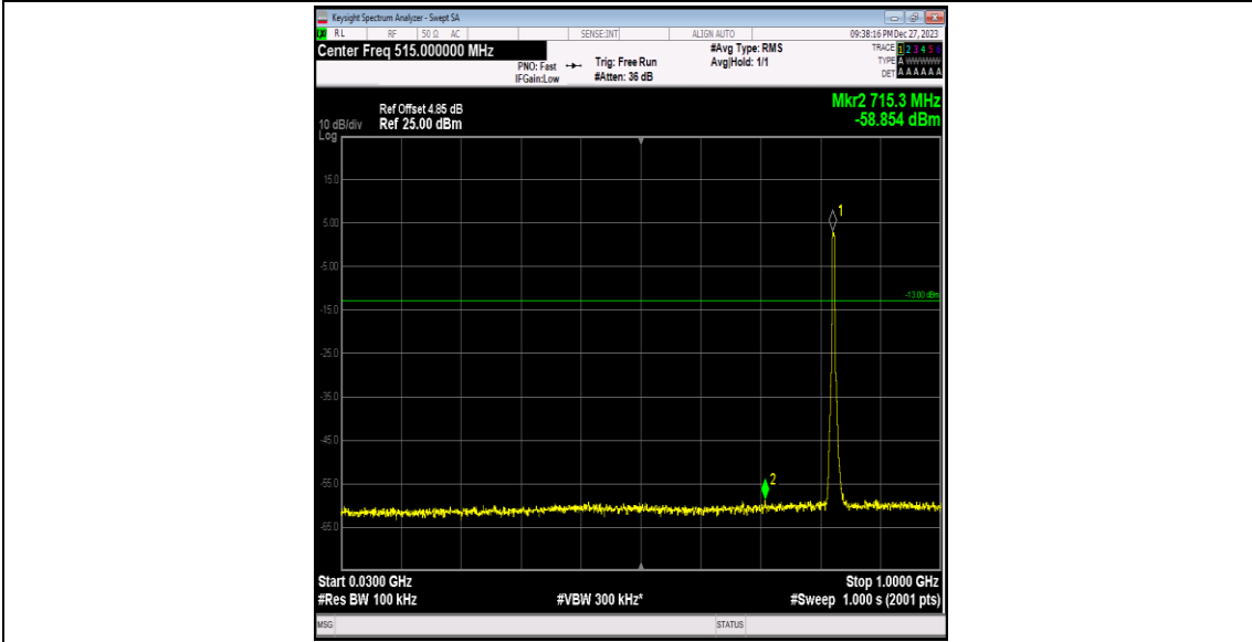
Band5-4132-2-30~1000MHz-PASS
