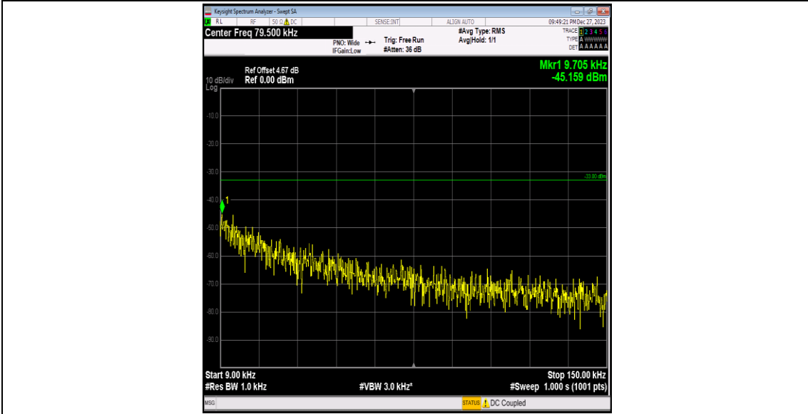
Band5-4132-5-0.009~0.15MHz-PASS
