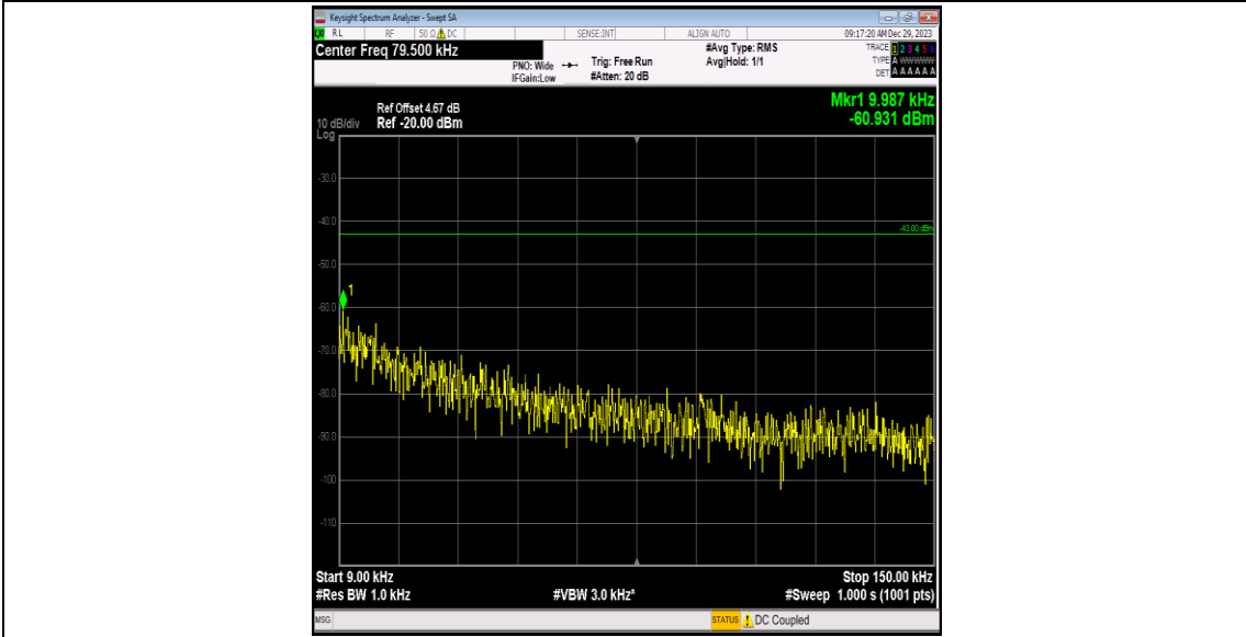
Band4-1513-2-0.009~0.15MHz-PASS
