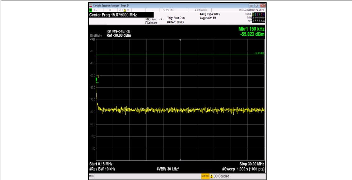
Band4-1413-5-0.15~30MHz-PASS
