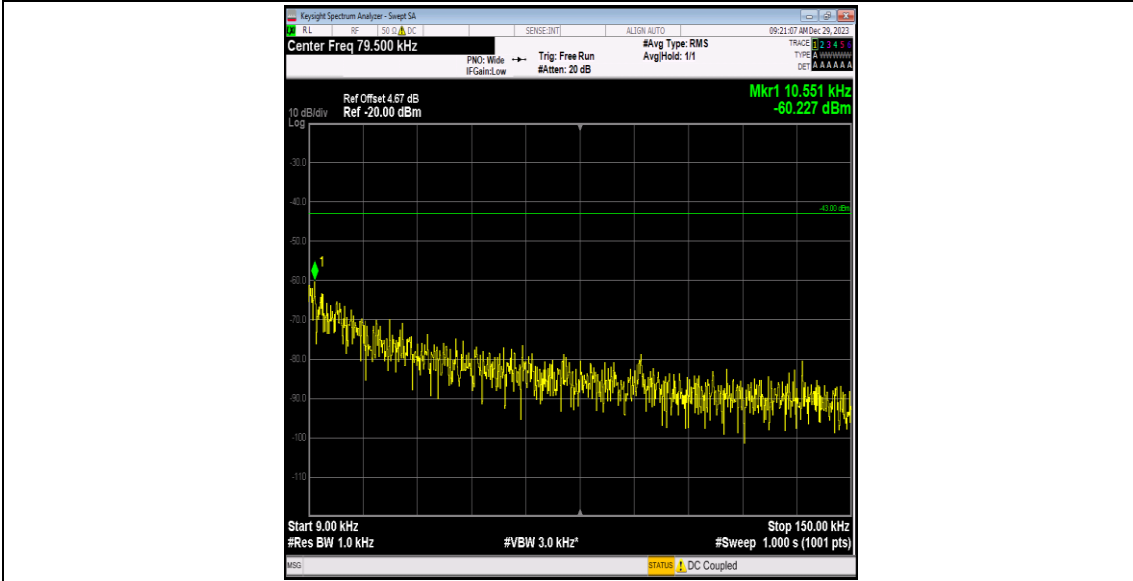
Band4-1513-3-0.009~0.15MHz-PASS
