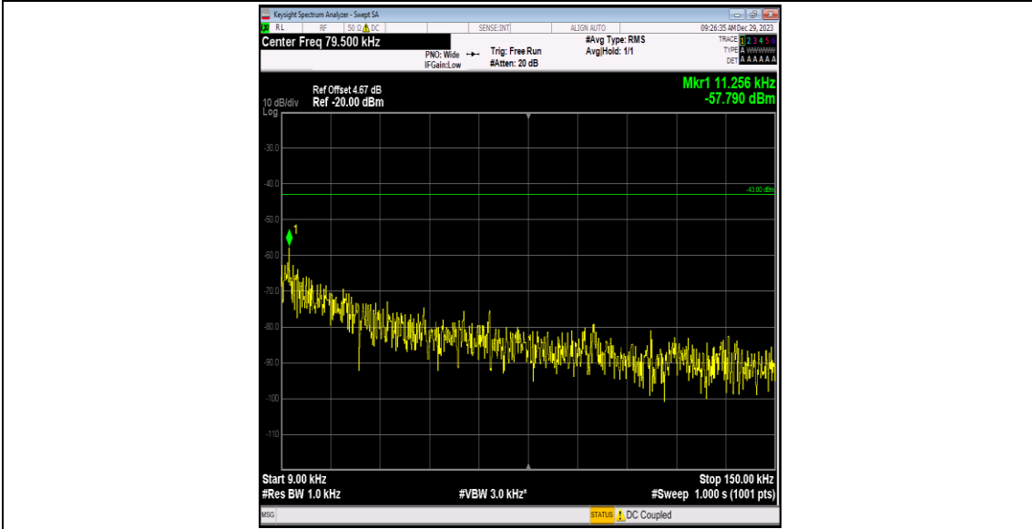
Band4-1413-5-0.009~0.15MHz-PASS
