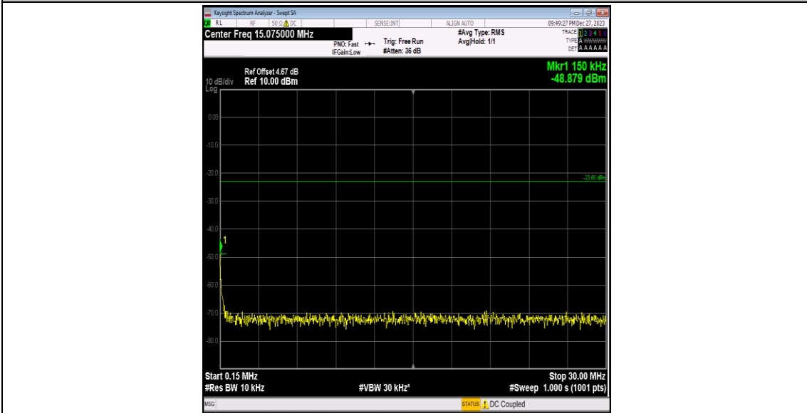
Band5-4132-5-0.15~30MHz-PASS
