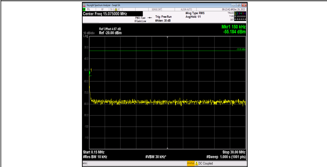
Band4-1513-1-0.15~30MHz-PASS
