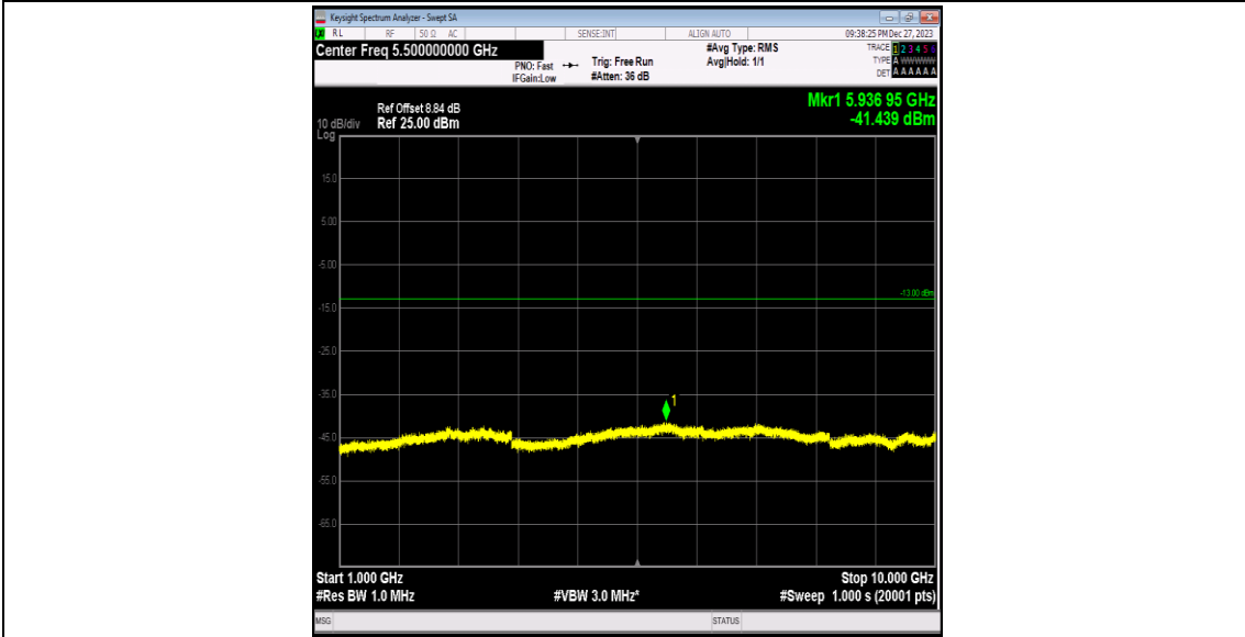
Band5-4132-2-1000~10000MHz-PASS
