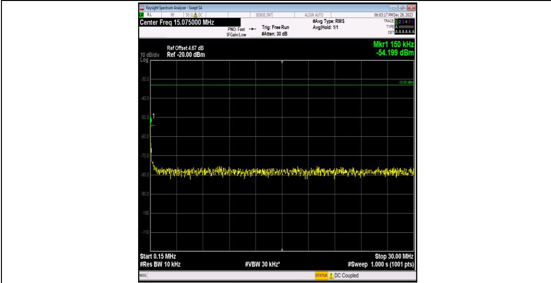
Band2-9400-4-0.15~30MHz-PASS
