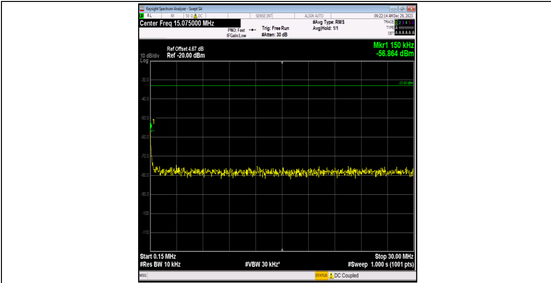
Band4-1312-4-0.15~30MHz-PASS
