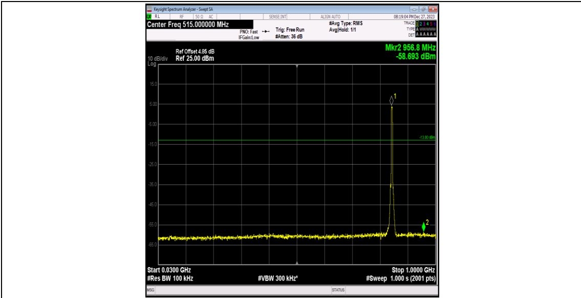
Band5-4233-4-30~1000MHz-PASS
