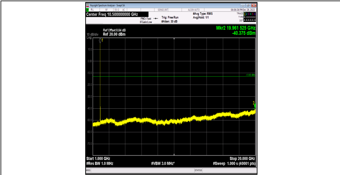
Band2-9400-5-1000~20000MHz-PASS
