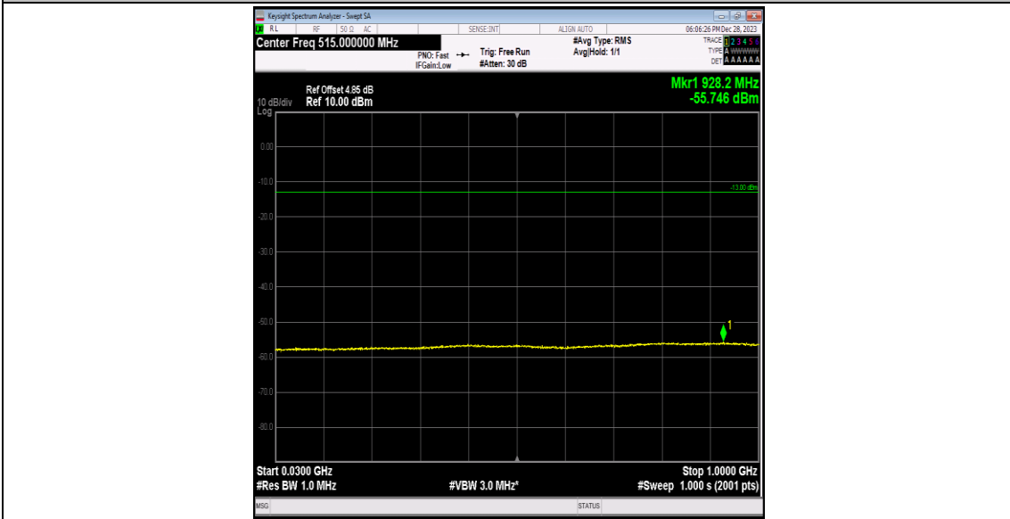
Band2-9400-5-30~1000MHz-PASS
