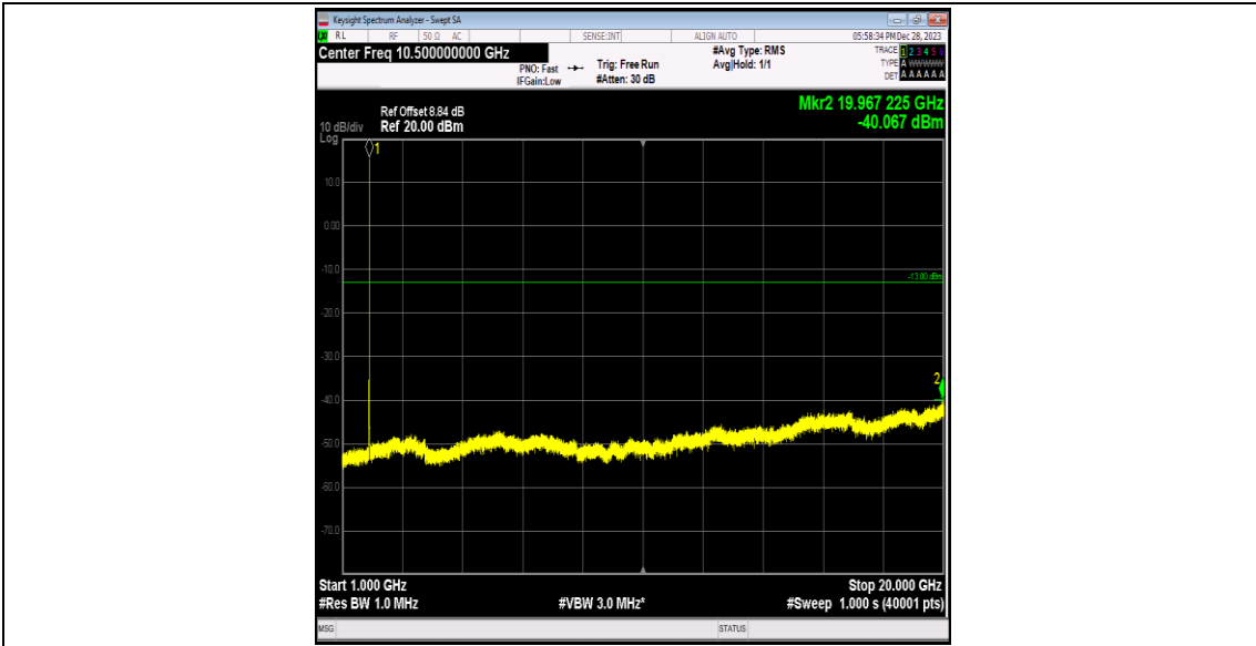
Band2-9262-3-1000~20000MHz-PASS
