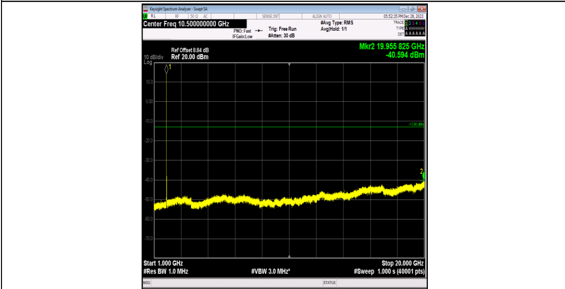
Band2-9400-1-1000~20000MHz-PASS
