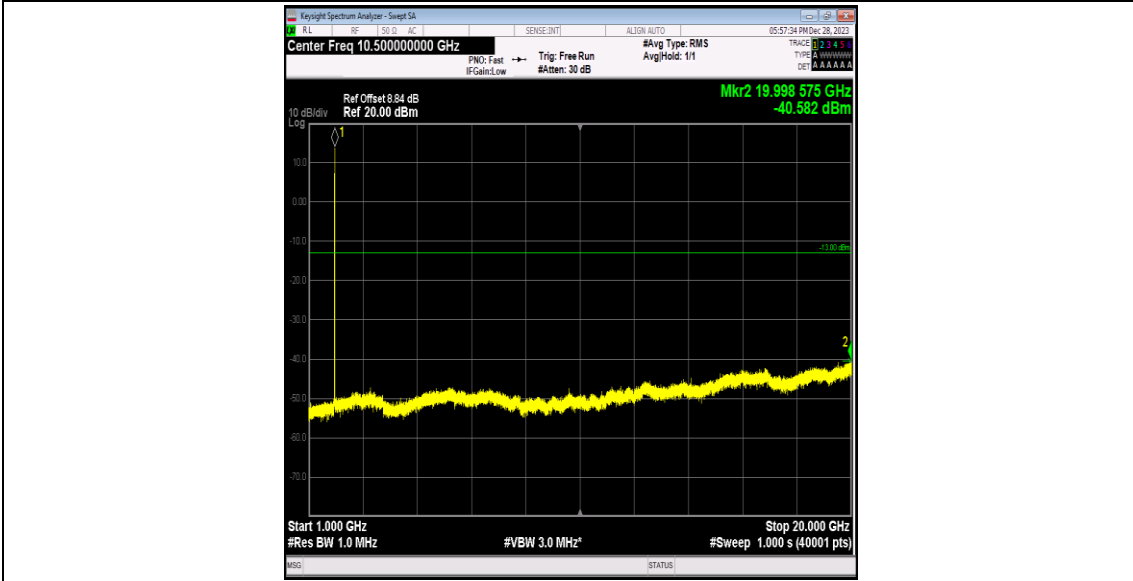
Band2-9538-2-1000~20000MHz-PASS
