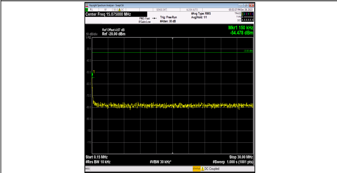
Band2-9538-1-0.15~30MHz-PASS
