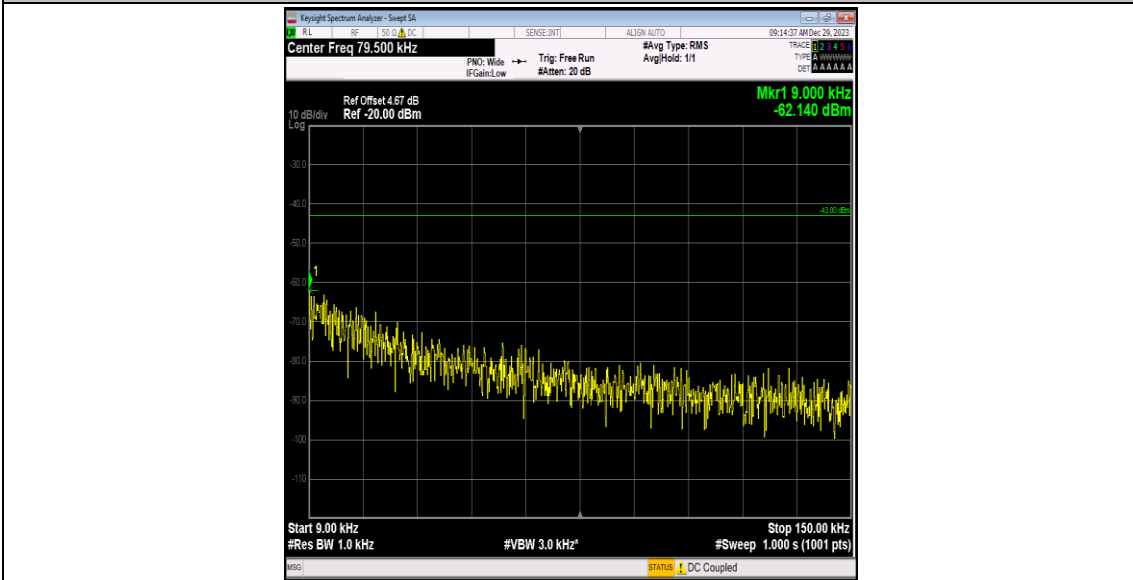
Band4-1312-2-0.009~0.15MHz-PASS
