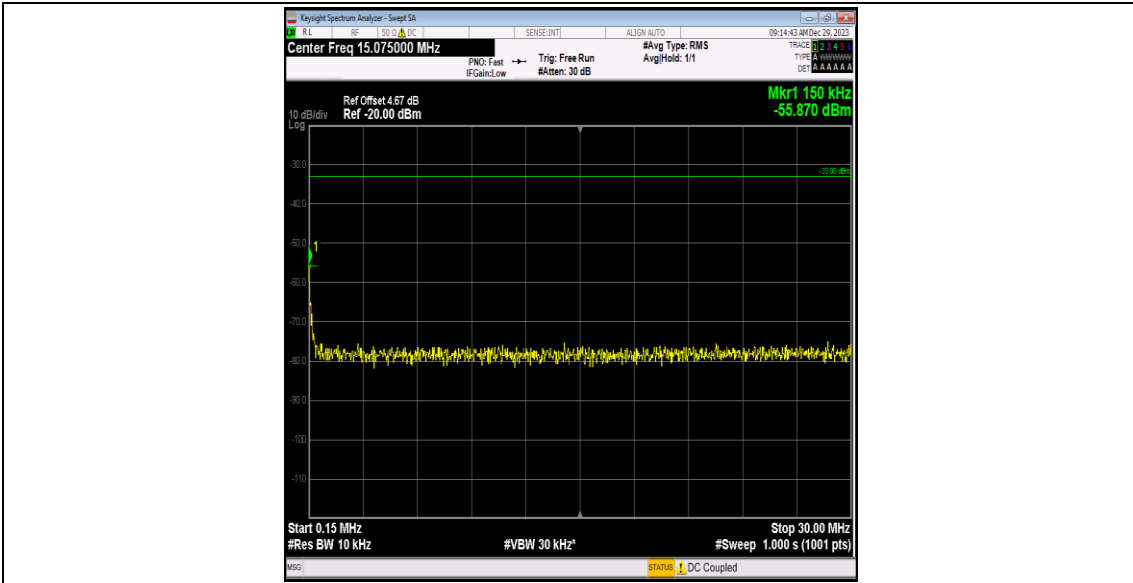
Band4-1312-2-0.15~30MHz-PASS
