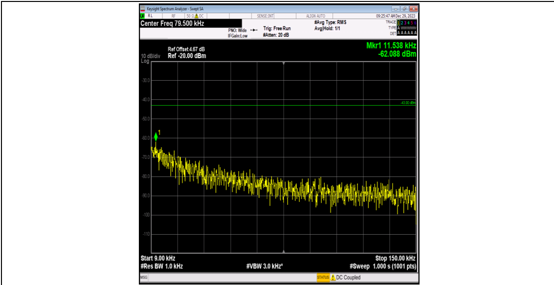
Band4-1312-5-0.009~0.15MHz-PASS
