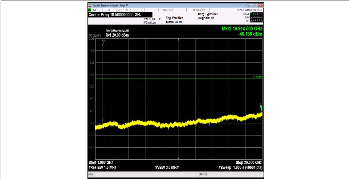
Band2-9400-2-1000~20000MHz-PASS
