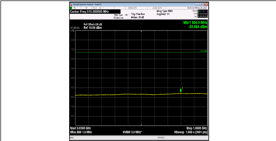
Band2-9262-1-30~1000MHz-PASS
