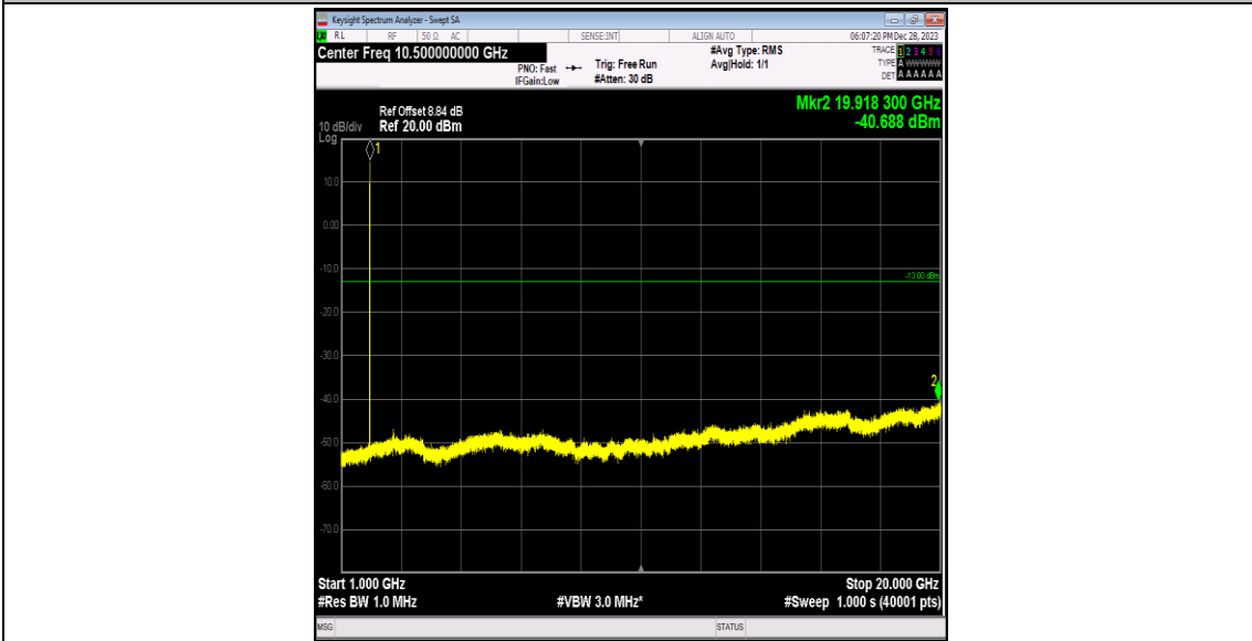
Band2-9538-5-1000~20000MHz-PASS
