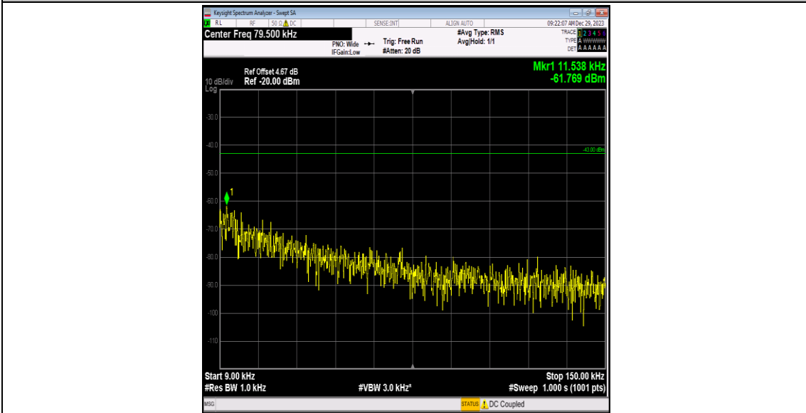
Band4-1312-4-0.009~0.15MHz-PASS
