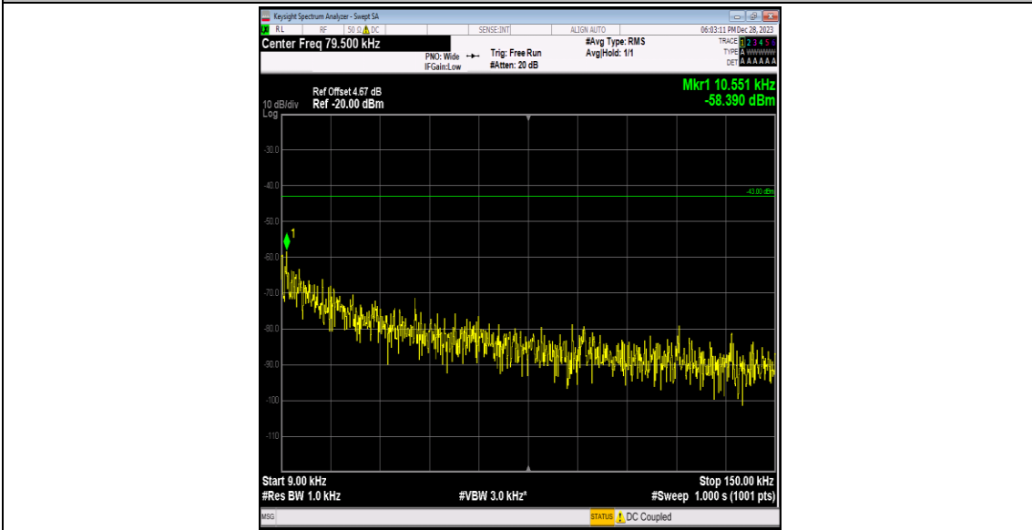
Band2-9400-4-0.009~0.15MHz-PASS
