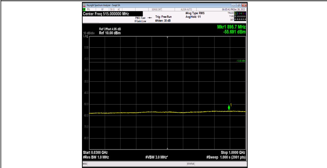
Band2-9262-5-30~1000MHz-PASS
