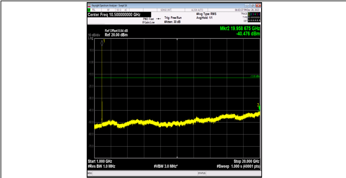
Band2-9400-4-1000~20000MHz-PASS
