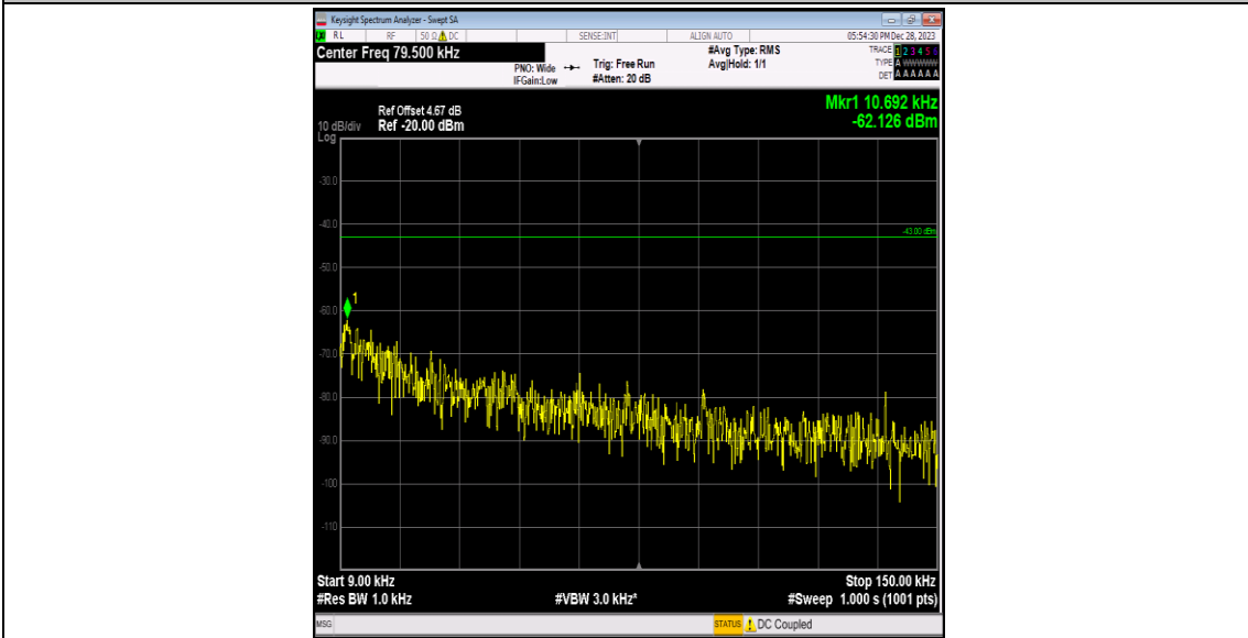
Band2-9262-2-0.009~0.15MHz-PASS
