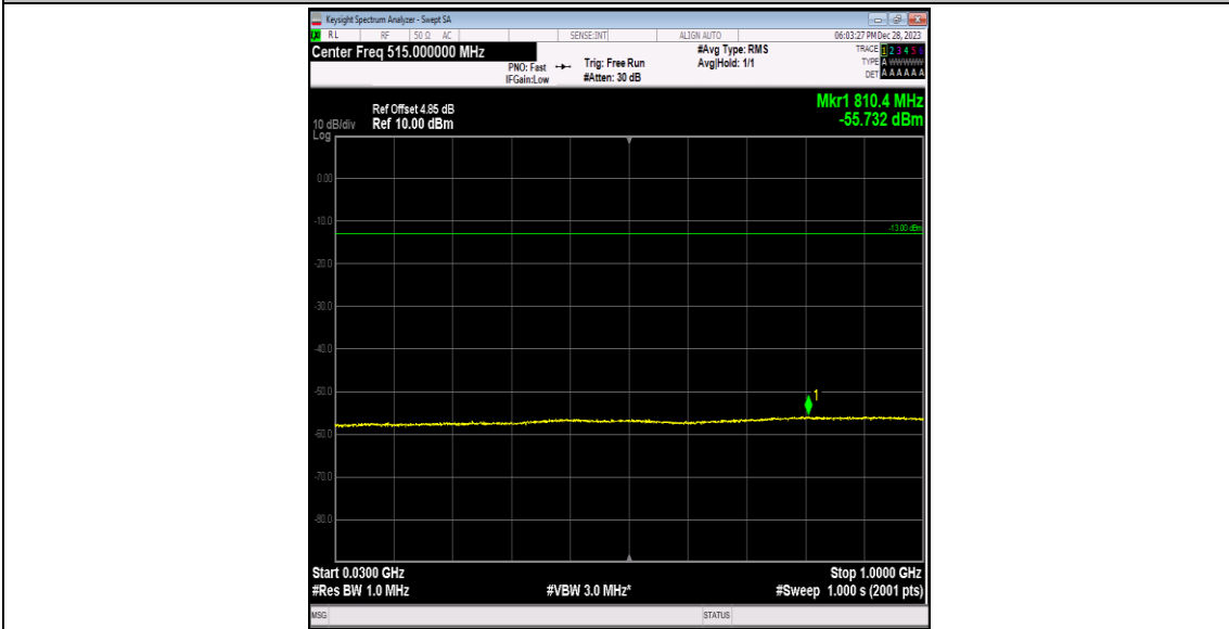
Band2-9400-4-30~1000MHz-PASS
