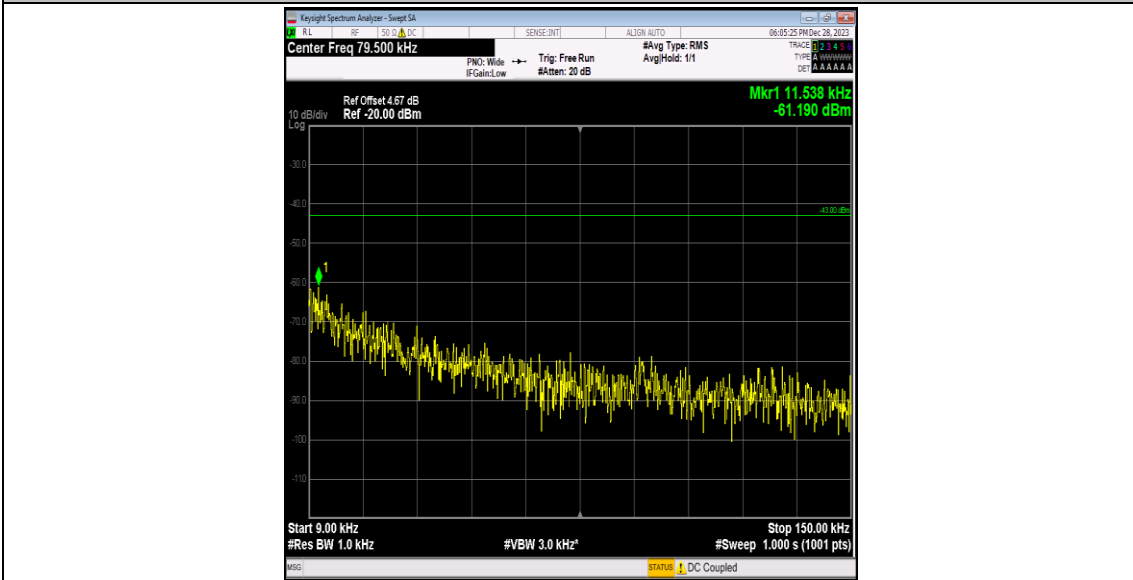
Band2-9262-5-0.009~0.15MHz-PASS
