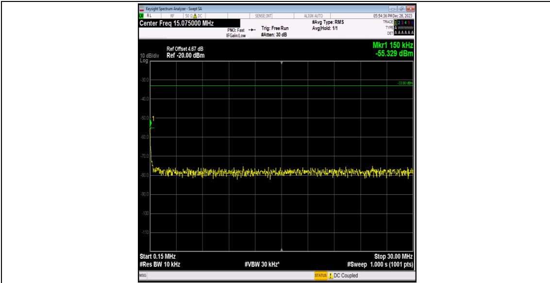
Band2-9262-2-0.15~30MHz-PASS
