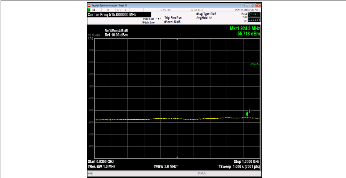
Band2-9262-2-30~1000MHz-PASS
