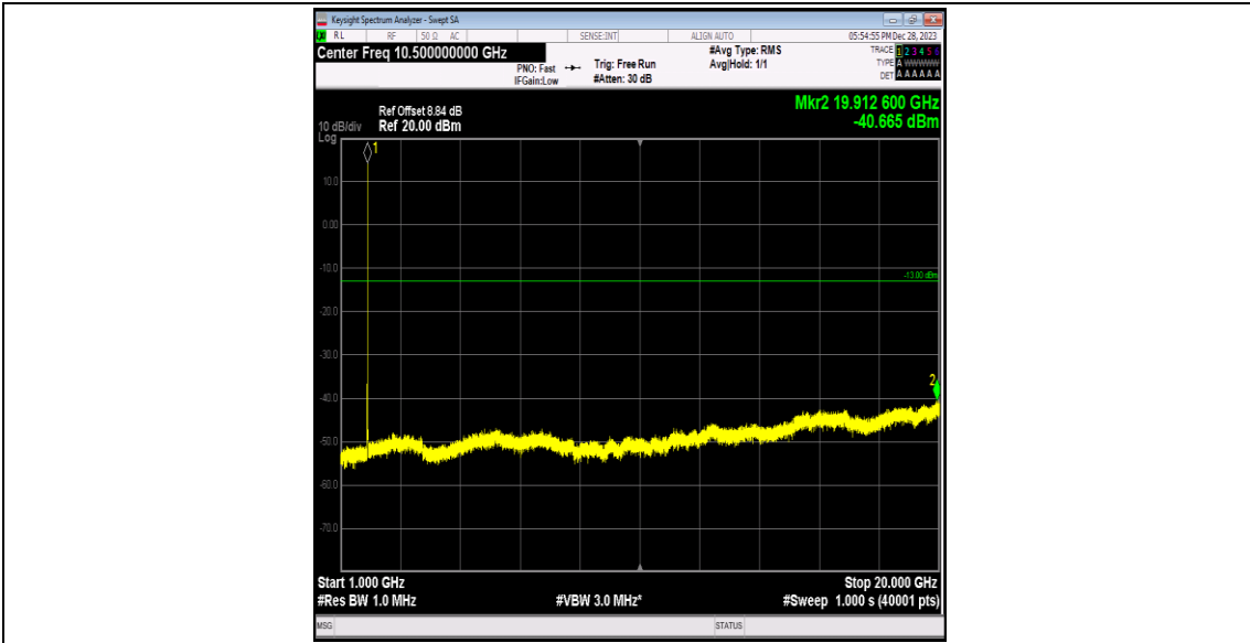
Band2-9262-2-1000~20000MHz-PASS
