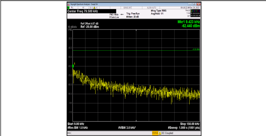
Band4-1312-3-0.009~0.15MHz-PASS
