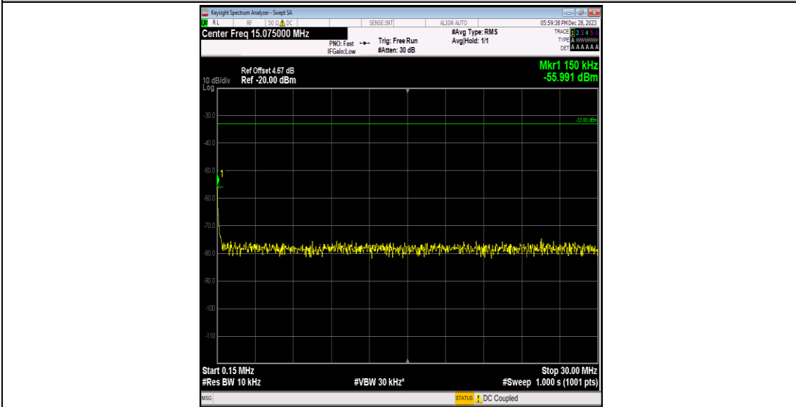
Band2-9400-3-0.15~30MHz-PASS
