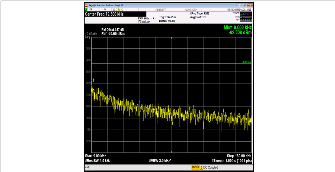
Band2-9538-1-0.009~0.15MHz-PASS
