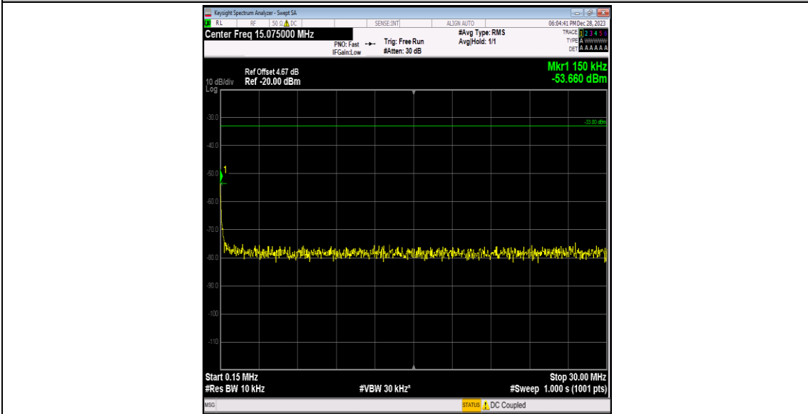
Band2-9538-4-0.15~30MHz-PASS
