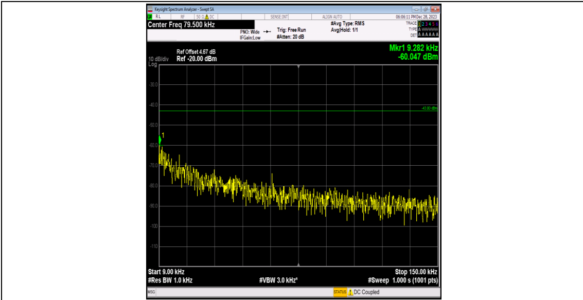
Band2-9400-5-0.009~0.15MHz-PASS
