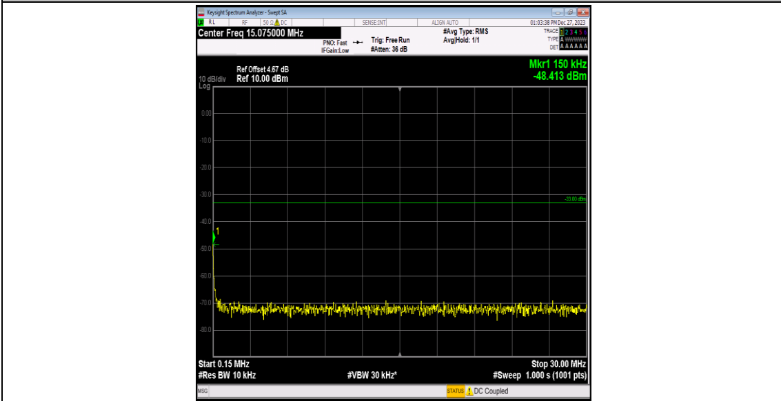
Band4-1513-3-0.15~30MHz-PASS
