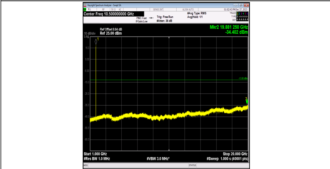
Band4-1312-3-1000~20000MHz-PASS
