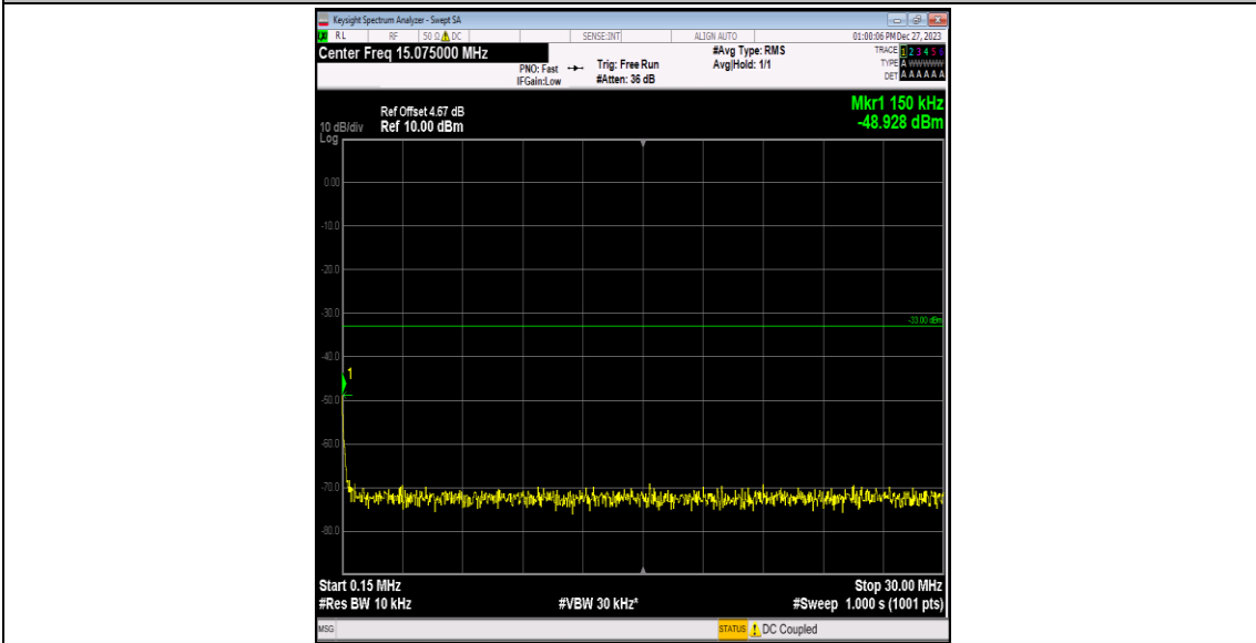
Band4-1312-2-0.15~30MHz-PASS
