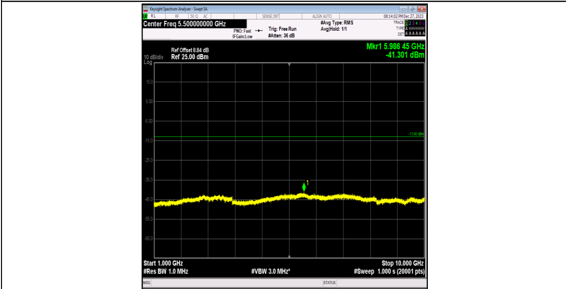
Band5-4132-2-1000~10000MHz-PASS
