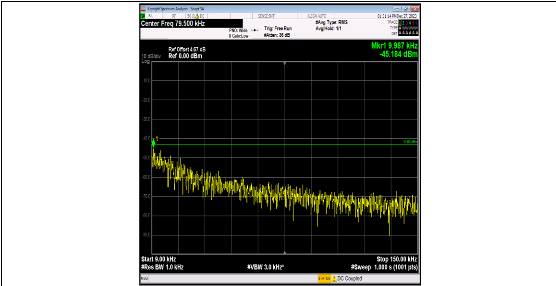
Band4-1513-2-0.009~0.15MHz-PASS
