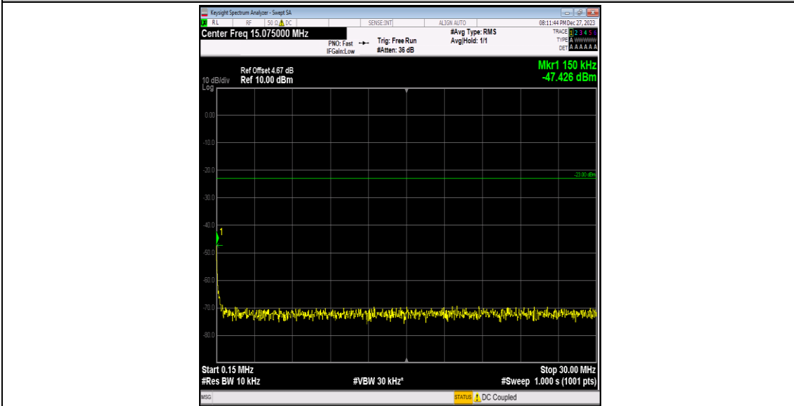
Band5-4132-1-0.15~30MHz-PASS
