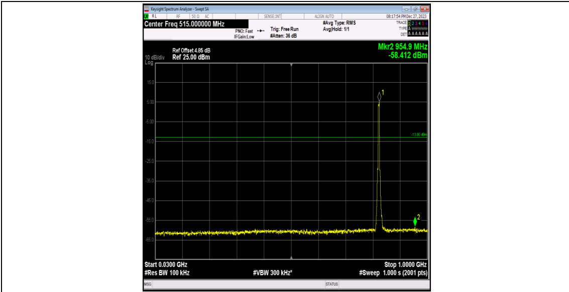
Band5-4132-4-30~1000MHz-PASS
