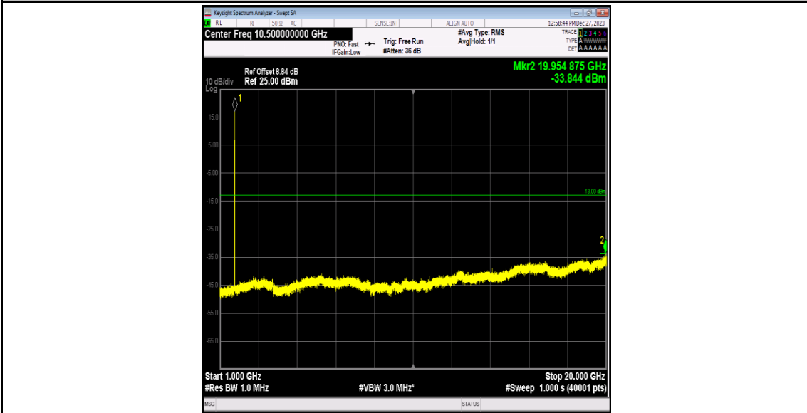
Band4-1413-1-1000~20000MHz-PASS
