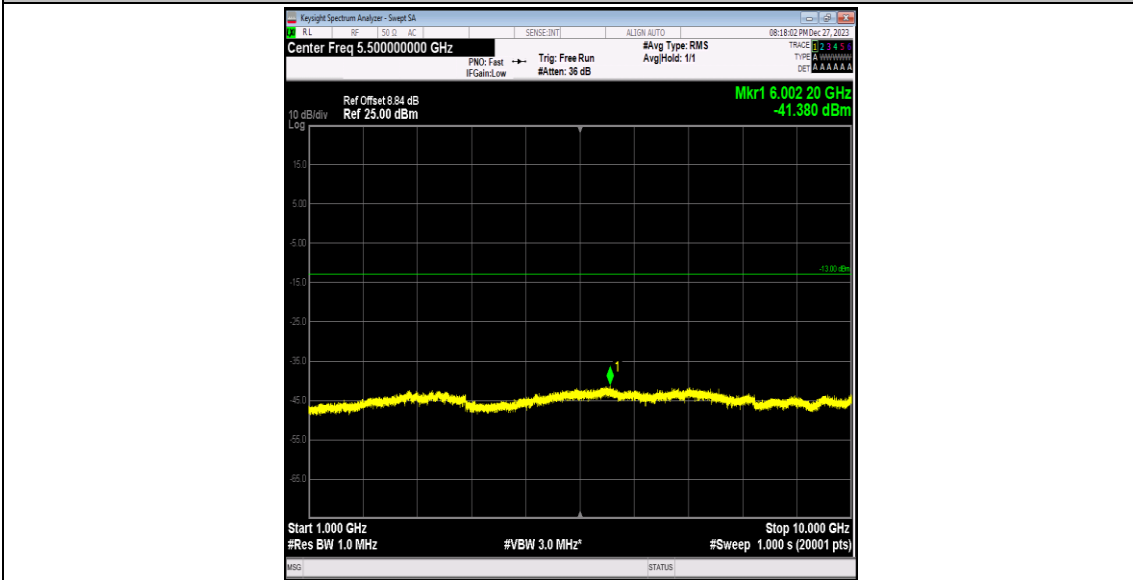
Band5-4132-4-1000~10000MHz-PASS
