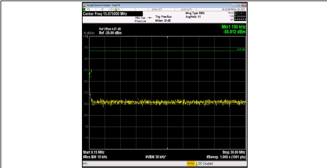
Band2-9538-2-0.15~30MHz-PASS
