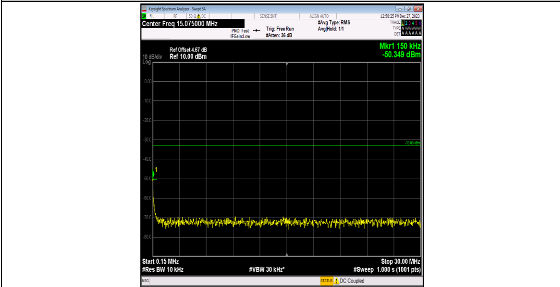
Band4-1413-1-0.15~30MHz-PASS
