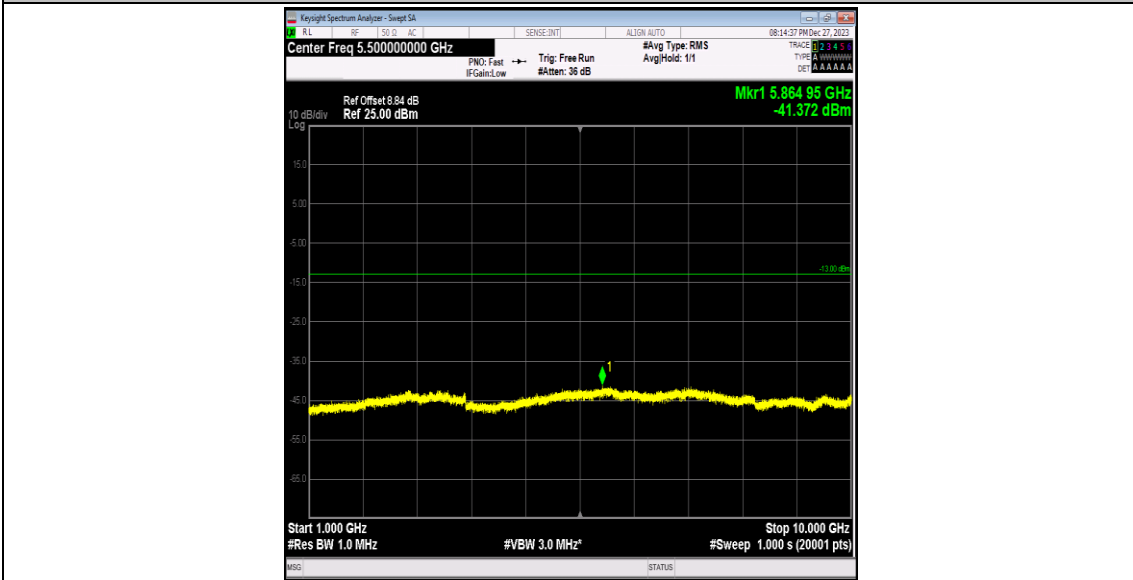
Band5-4182-2-1000~10000MHz-PASS
