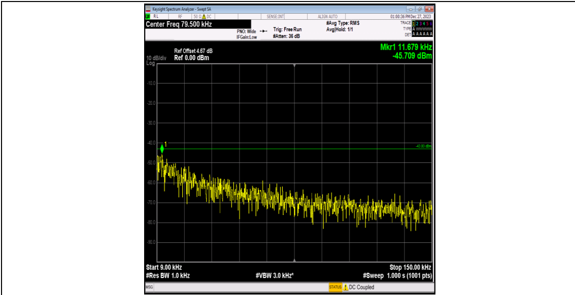
Band4-1413-2-0.009~0.15MHz-PASS
