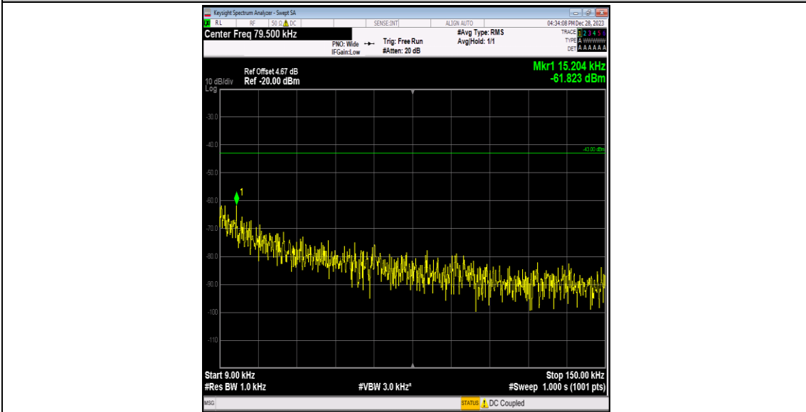
Band2-9538-3-0.009~0.15MHz-PASS
