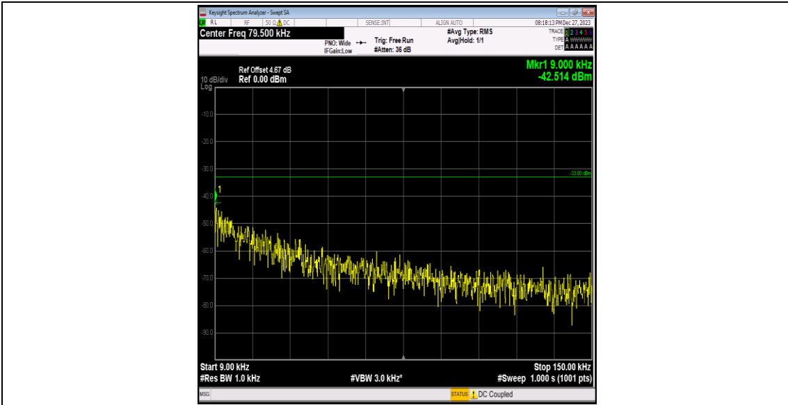
Band5-4182-4-0.009~0.15MHz-PASS
