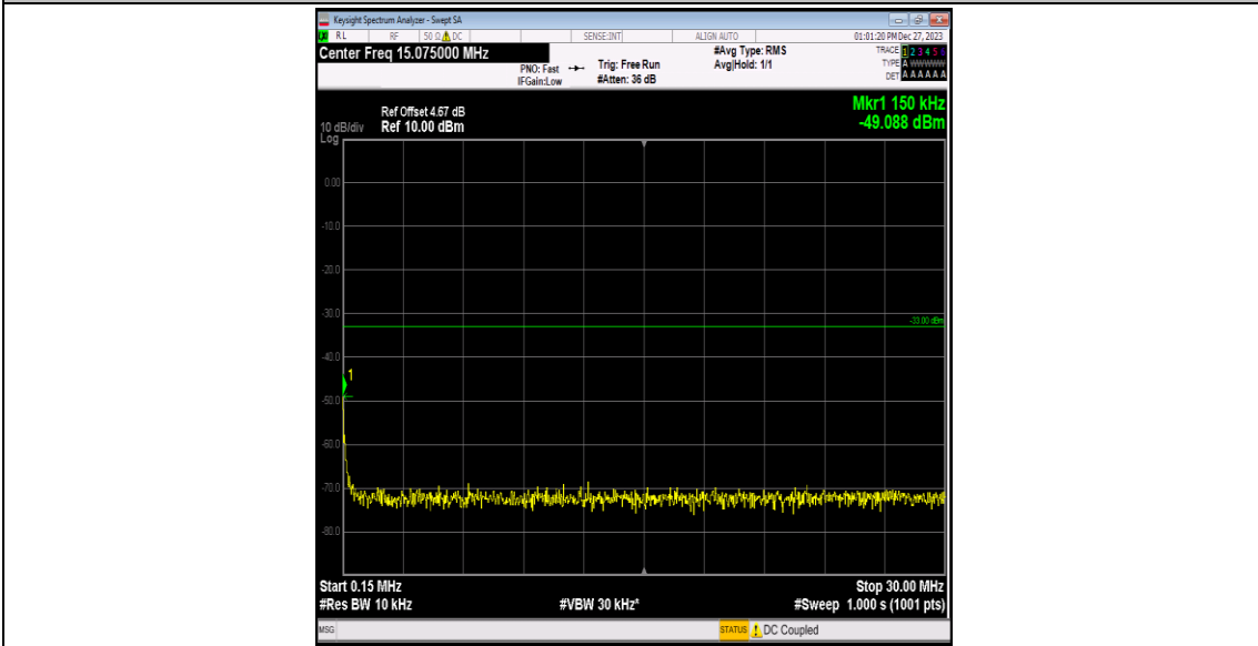
Band4-1513-2-0.15~30MHz-PASS
