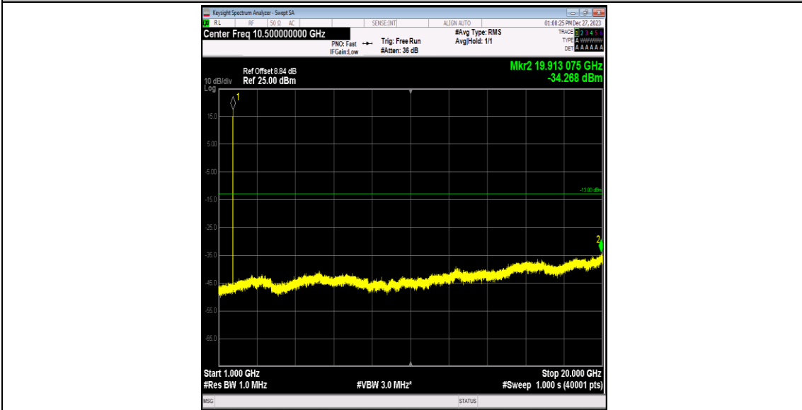
Band4-1312-2-1000~20000MHz-PASS
