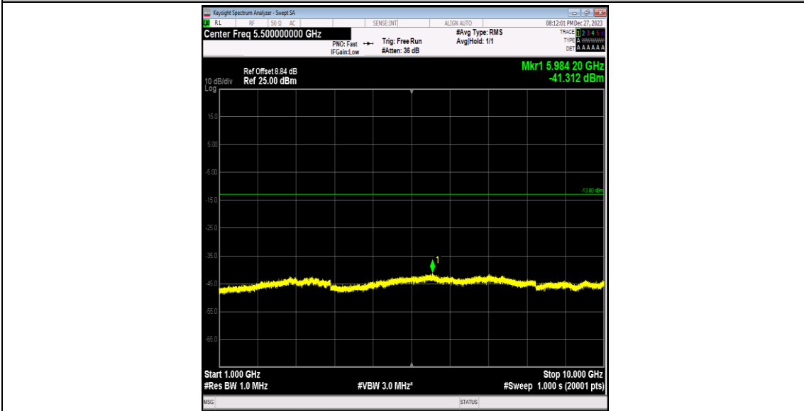
Band5-4132-1-1000~10000MHz-PASS
