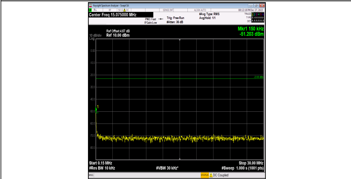
Band5-4182-1-0.15~30MHz-PASS
