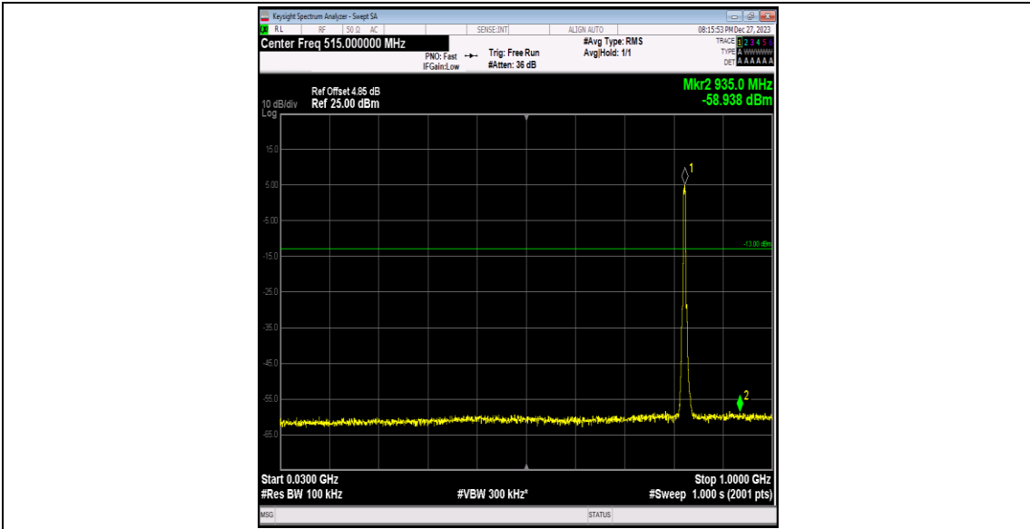
Band5-4132-3-30~1000MHz-PASS
