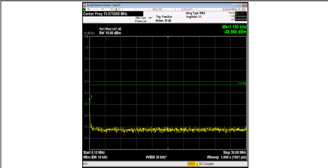
Band4-1312-3-0.15~30MHz-PASS
