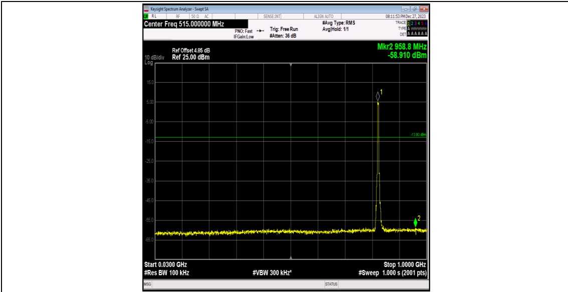
Band5-4132-1-30~1000MHz-PASS
