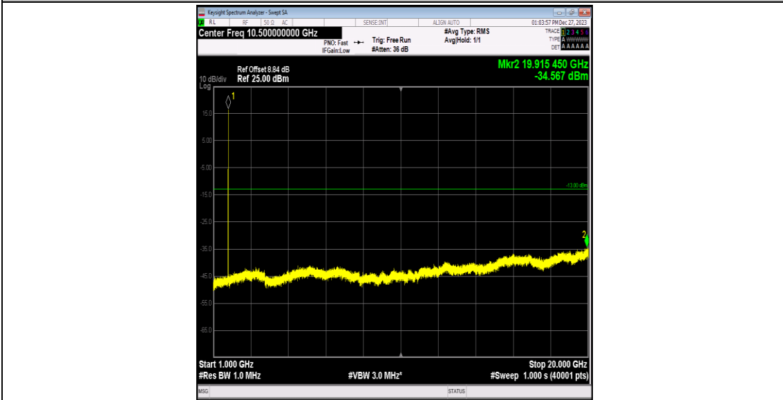
Band4-1513-3-1000~20000MHz-PASS
