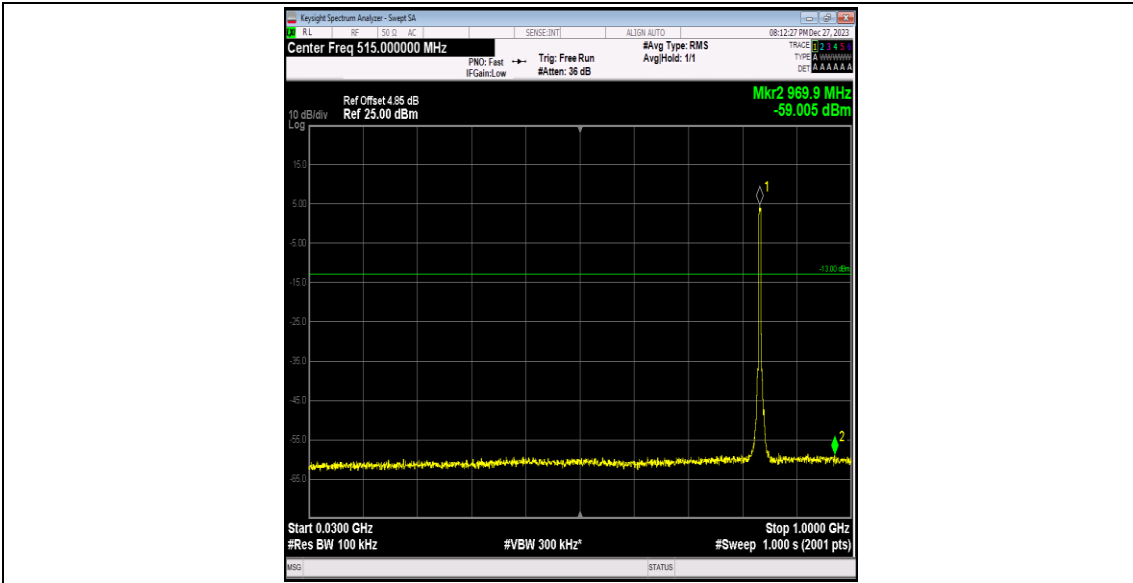
Band5-4182-1-30~1000MHz-PASS
