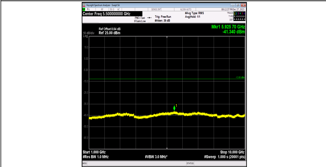
Band5-4182-1-1000~10000MHz-PASS
