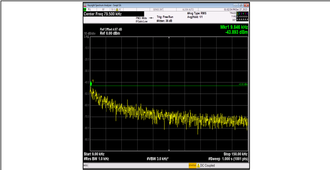
Band4-1413-3-0.009~0.15MHz-PASS
