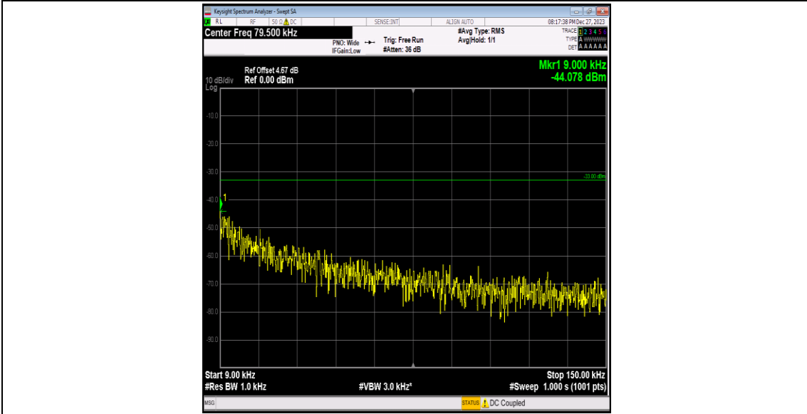
Band5-4132-4-0.009~0.15MHz-PASS
