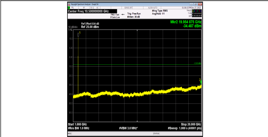
Band4-1513-4-1000~20000MHz-PASS
