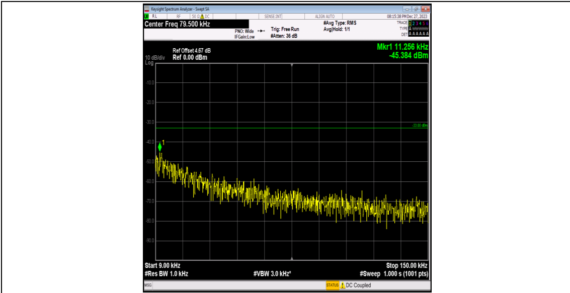
Band5-4132-3-0.009~0.15MHz-PASS
