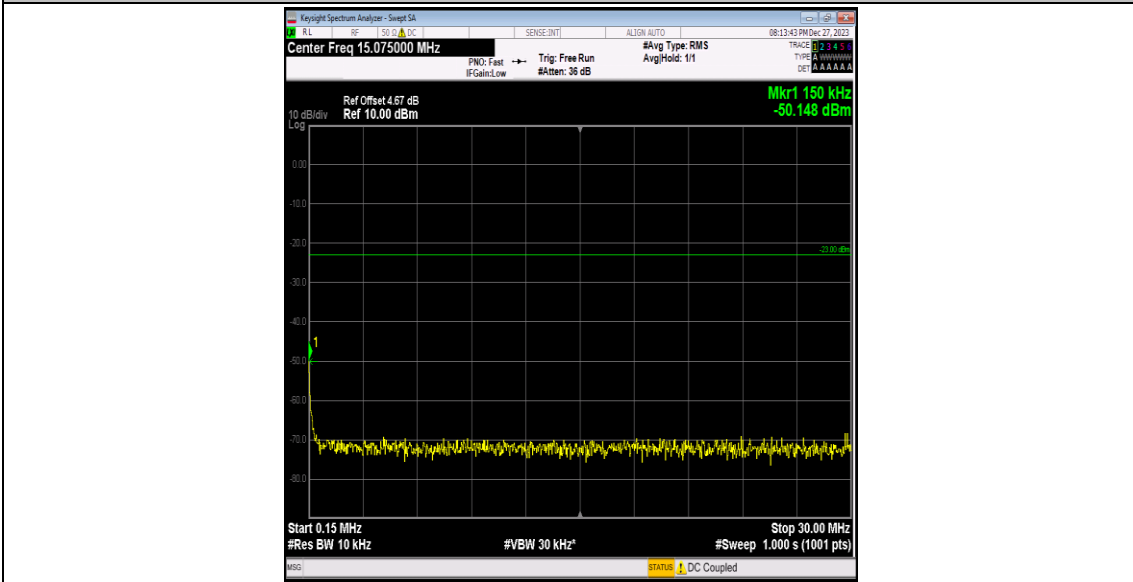
Band5-4132-2-0.15~30MHz-PASS
