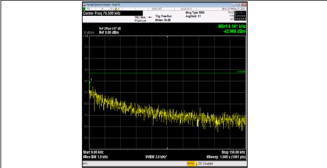
Band5-4132-1-0.009~0.15MHz-PASS
