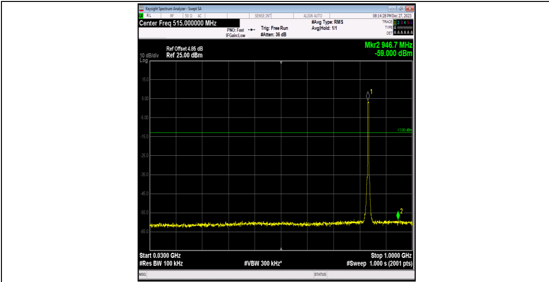
Band5-4182-2-30~1000MHz-PASS
