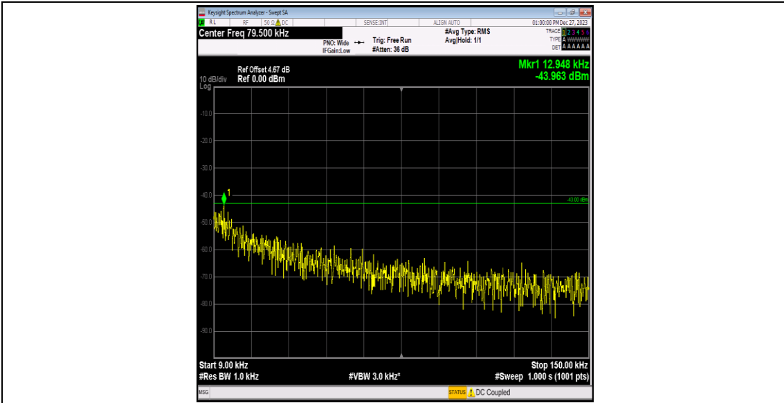
Band4-1312-2-0.009~0.15MHz-PASS
