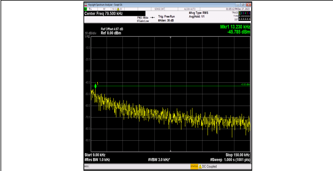
Band4-1413-4-0.009~0.15MHz-PASS
