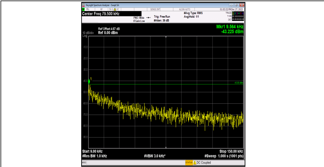
Band4-1513-3-0.009~0.15MHz-PASS
