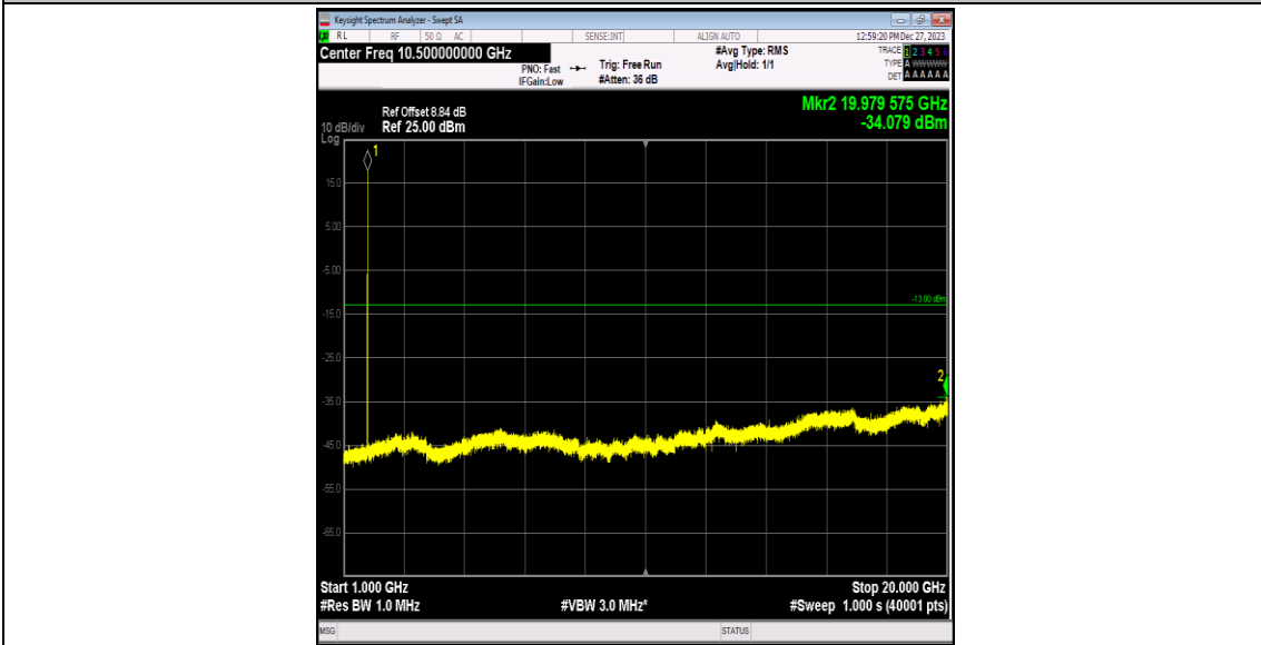
Band4-1513-1-1000~20000MHz-PASS
