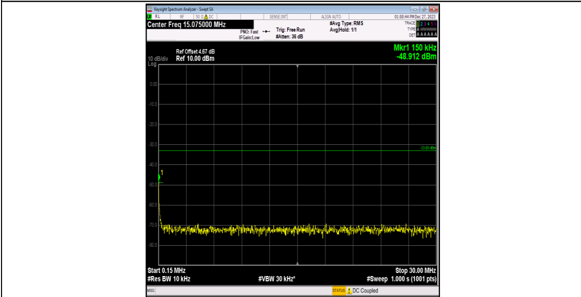
Band4-1413-2-0.15~30MHz-PASS
