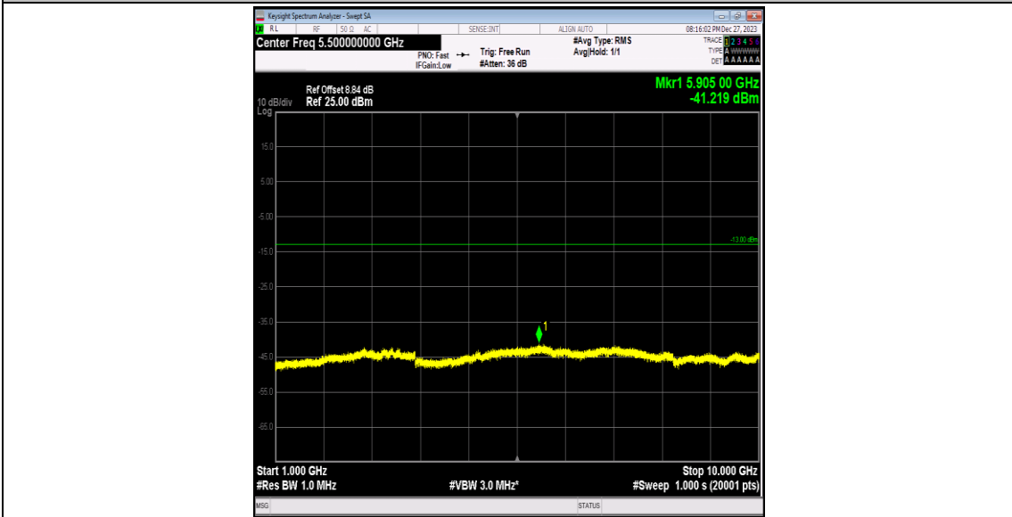
Band5-4132-3-1000~10000MHz-PASS
