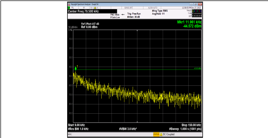
Band4-1513-1-0.009~0.15MHz-PASS
