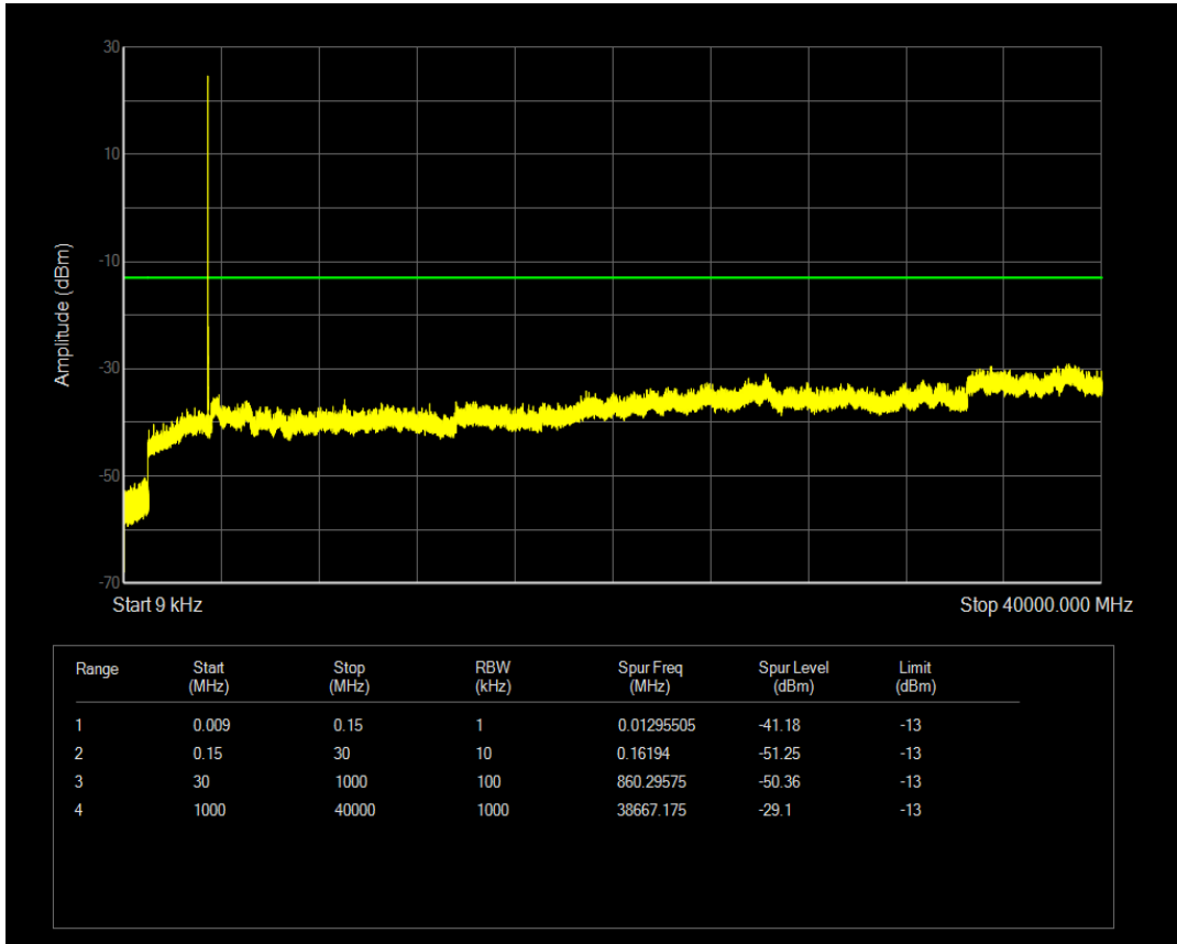
n77(3450-3550) SCS=30kHz DFT_QPSK BW=10MHz Channel=630334 RB=1@23
