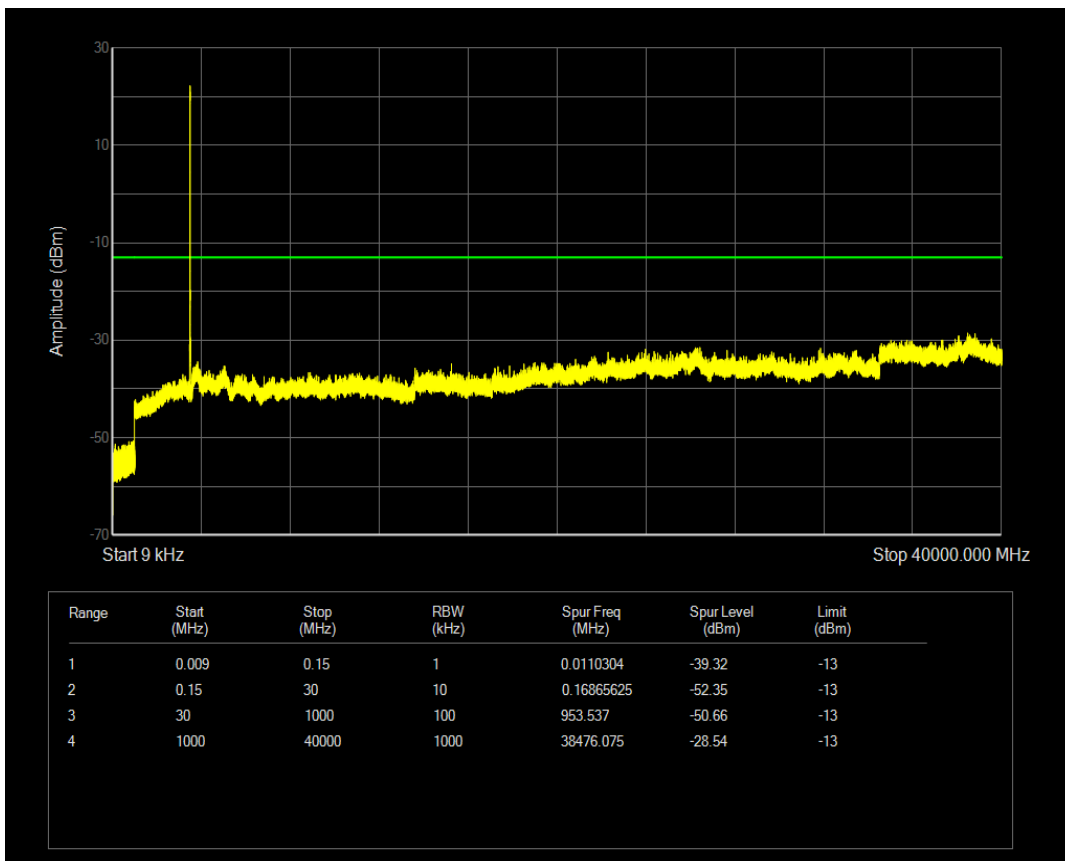
n77(3450-3550) SCS=30kHz DFT_QPSK BW=10MHz Channel=633334 RB=1@0
