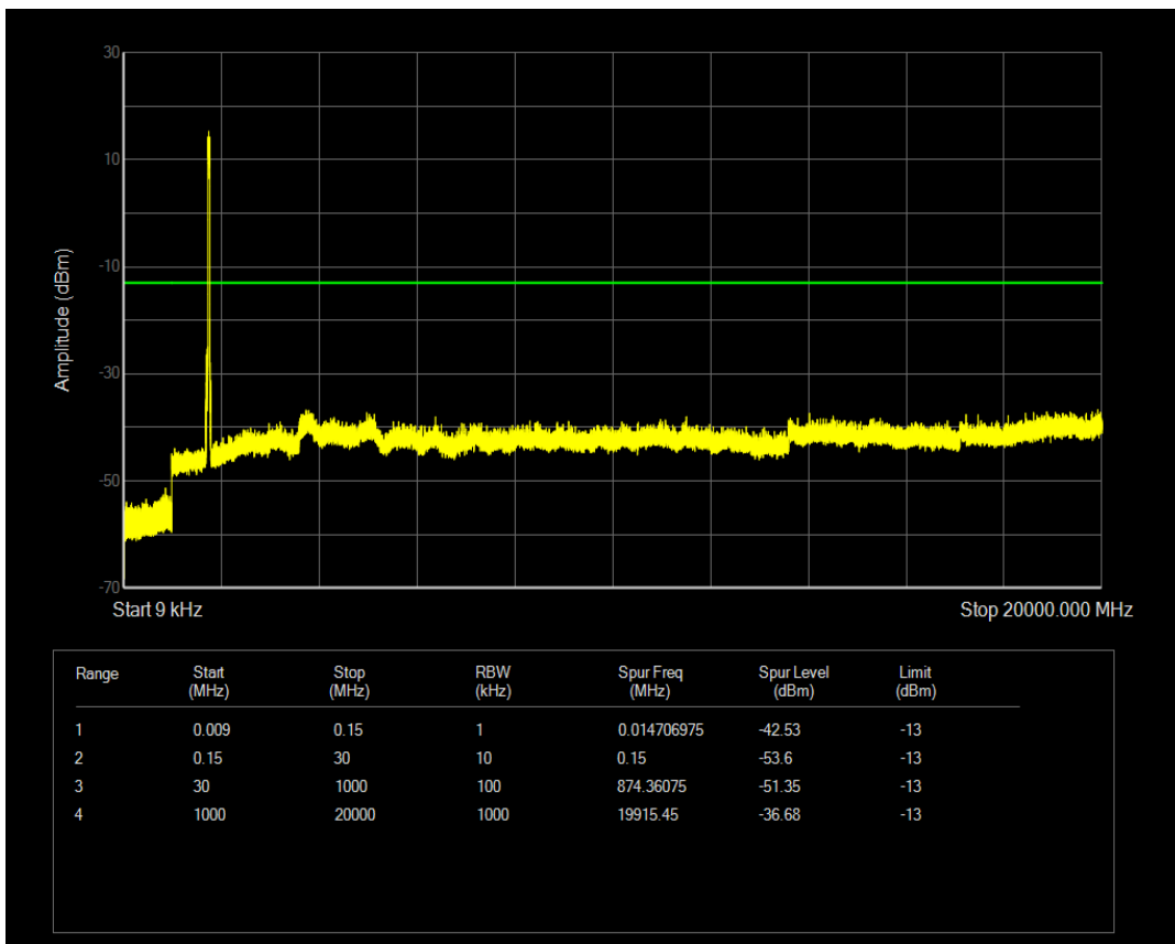
n66 SCS=30kHz DFT_QPSK BW=40MHz Channel=352000 RB=1@105
