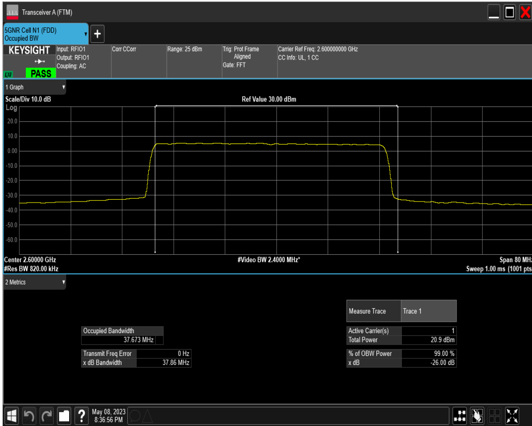
n38 SCS=30kHz DFT_QAM64 BW=40MHz Channel=520000 RB=100@0
