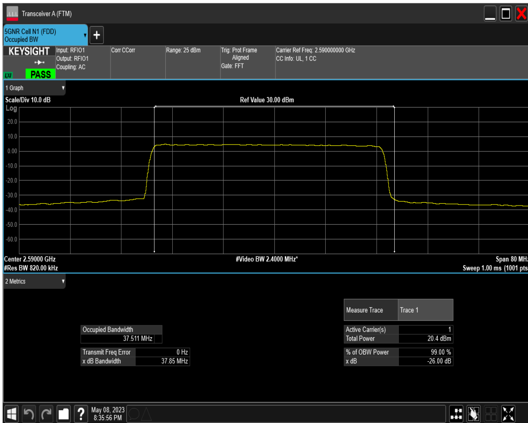
n38 SCS=30kHz DFT_QAM256 BW=40MHz Channel=518000 RB=100@0
