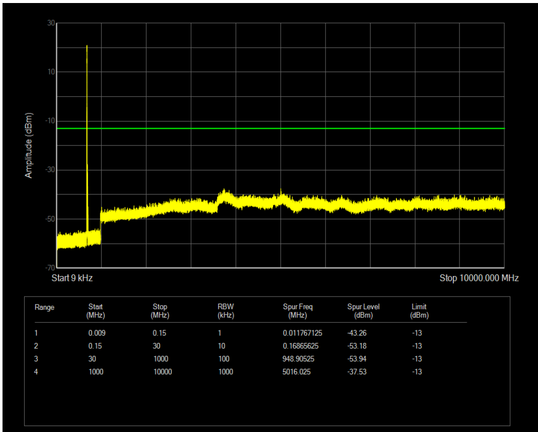
n12 SCS=30kHz DFT_QPSK BW=10MHz Channel=140800 RB=1@23
