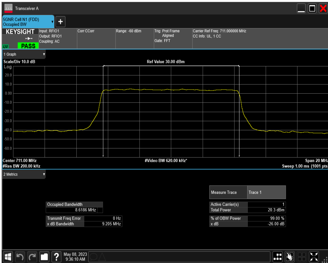
n12 SCS=30kHz DFT_QAM256 BW=10MHz Channel=142200 RB=24@0
