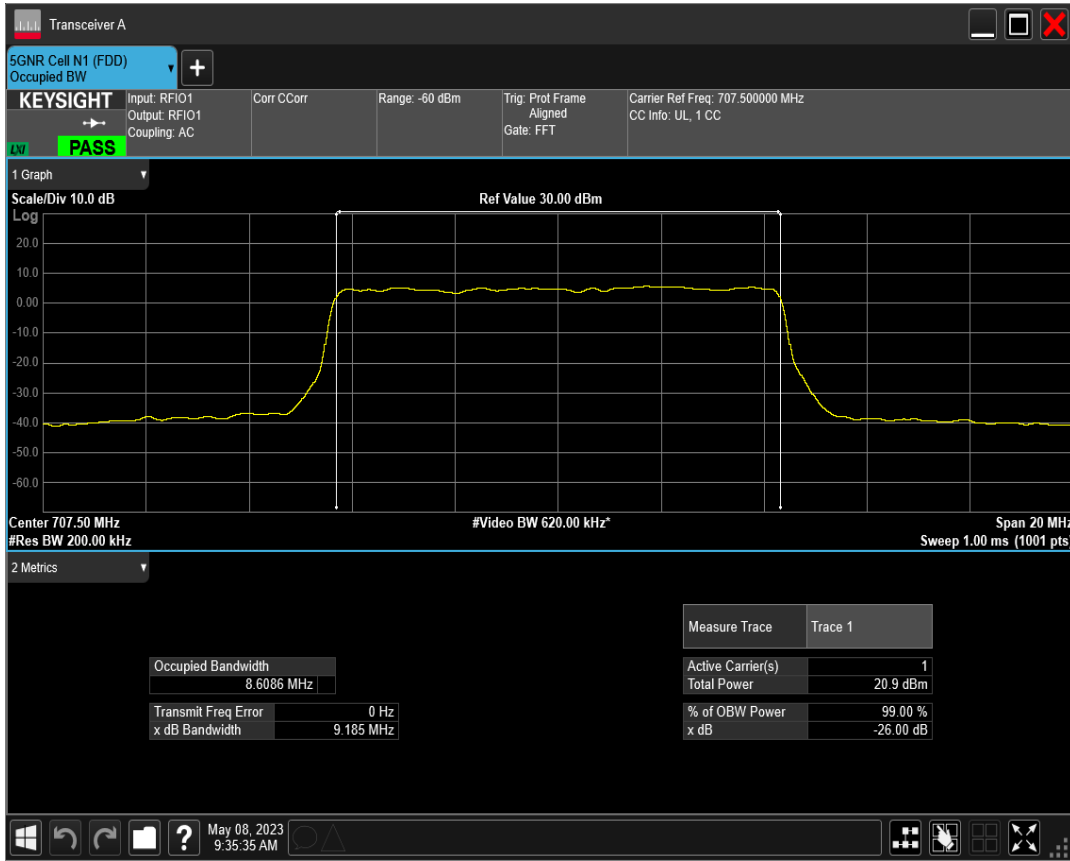
n12 SCS=30kHz DFT_QAM64 BW=10MHz Channel=141500 RB=24@0
