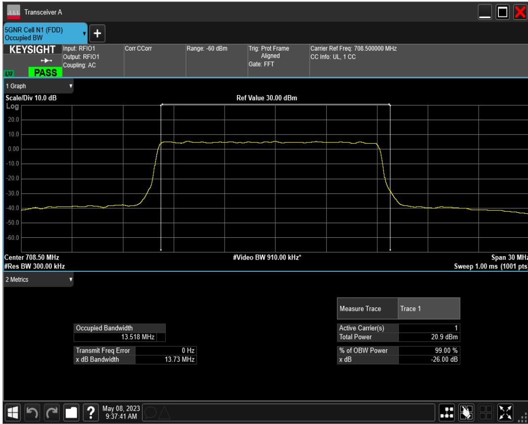
n12 SCS=30kHz DFT_QAM64 BW=15MHz Channel=141700 RB=36@0
