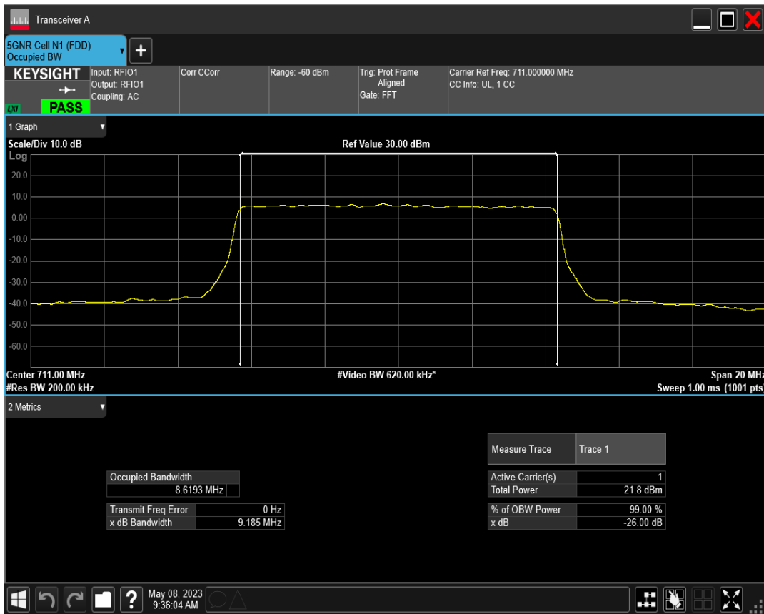
n12 SCS=30kHz DFT_QAM16 BW=10MHz Channel=142200 RB=24@0
