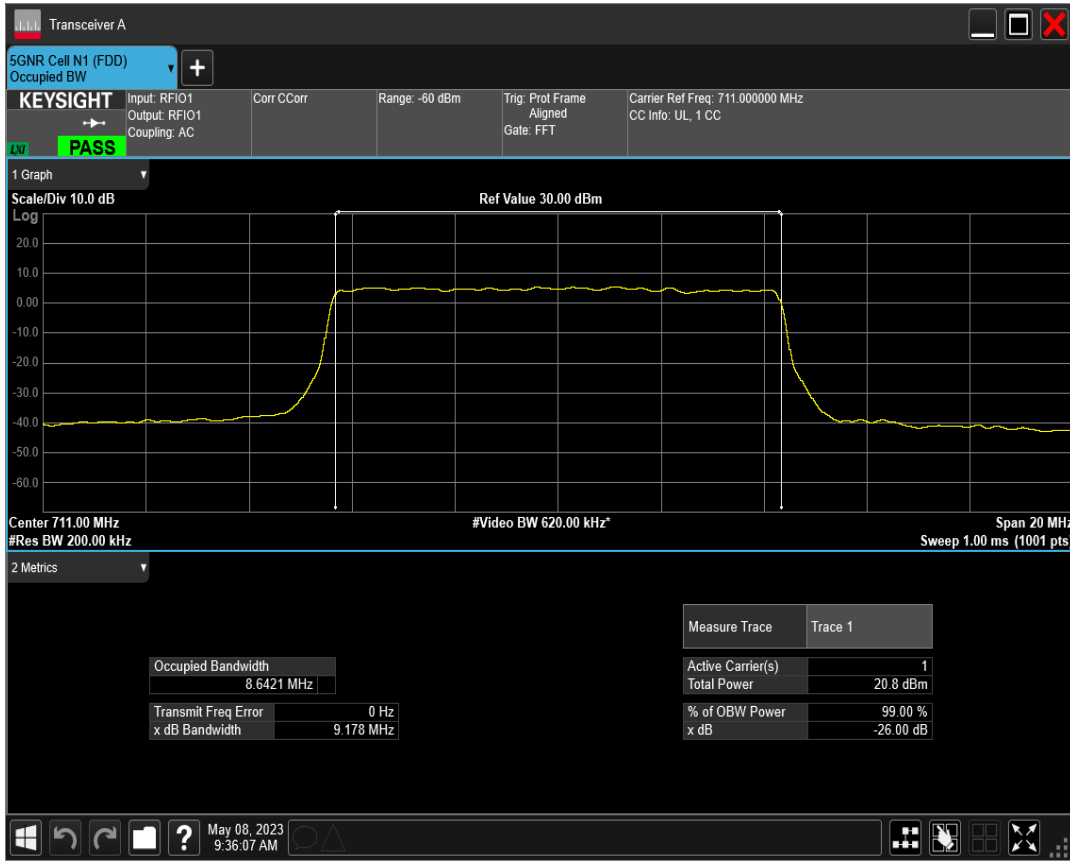
n12 SCS=30kHz DFT_QAM64 BW=10MHz Channel=142200 RB=24@0
