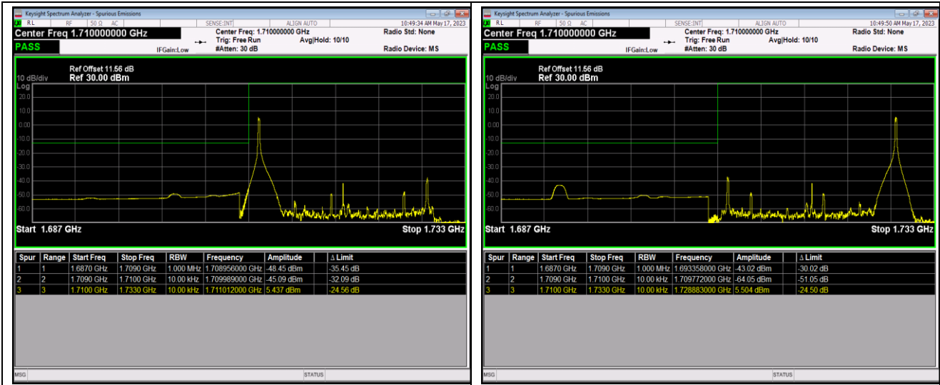
Band66-20MHz-64QAM-132072-100RB#0
