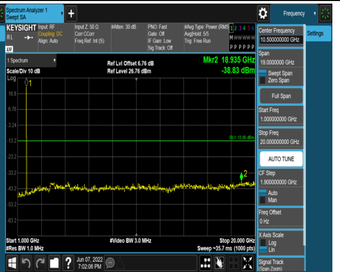
Band66-20MHz-16QAM-132322-1RB#0-Range2:1000 ~20000MHz
