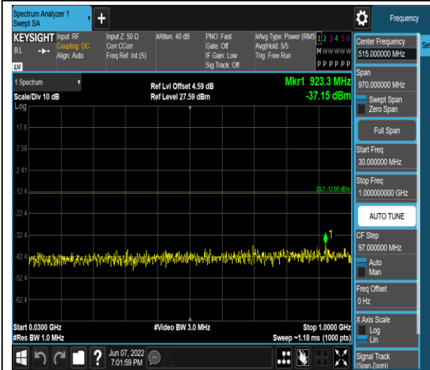
Band66-20MHz-16QAM-132322-1RB#0-Range1:3 0~1000MHz
