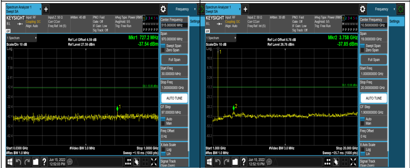
Band66-1.4MHz-QPSK-132665-1RB#0-Range1:30
