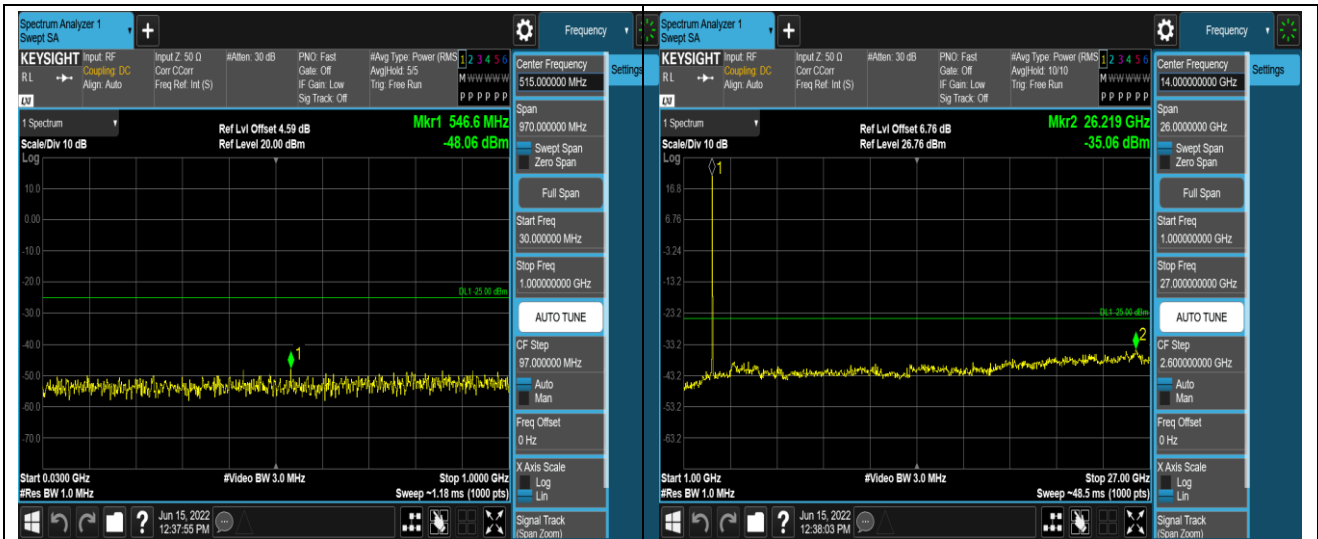
Band41-20MHz-16QAM-41140-1RB#0-Range1:30 ~1000MHz
