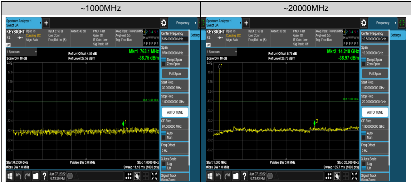
Band66-1.4MHz-16QAM-131979-1RB#0-Range1:3 0~1000MHz
