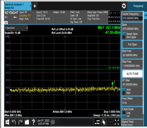
Band7-5MHz-QPSK-21425-1RB#0-Range1:30~1000MHz
