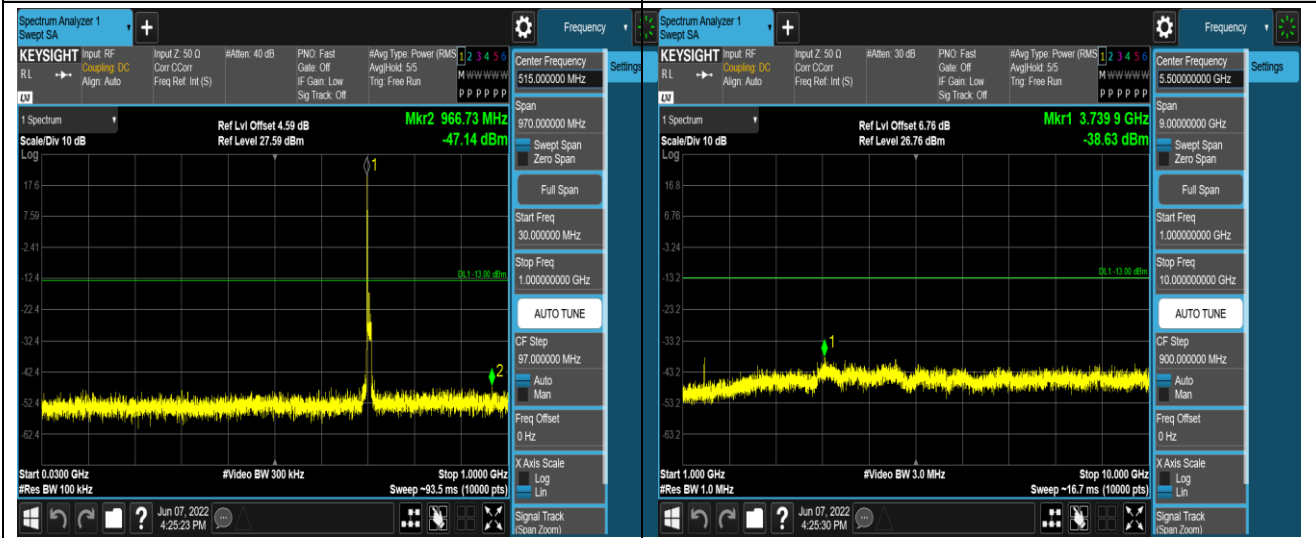
Band12-10MHz-16QAM-23060-1RB#0-Range1:30
