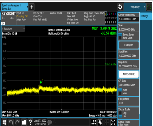
Band5-1.4MHz-16QAM-20643-1RB#0-Range2:1000~10000MHz
