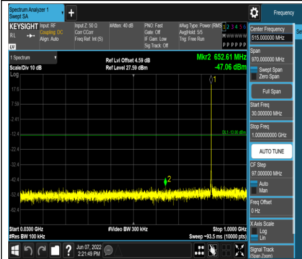
Band5-1.4MHz-16QAM-20407-1RB#0-Range1:30~1000MHz
