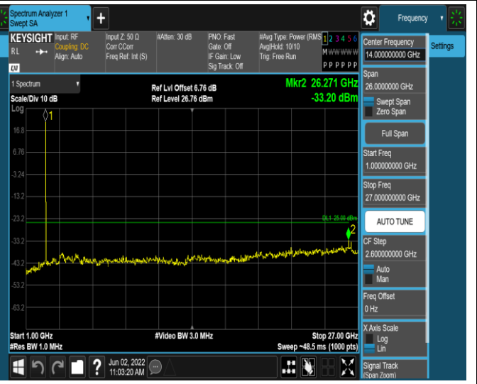
Band41-20MHz-16QAM-40140-1RB#0-Range2:1000~27000MHz
