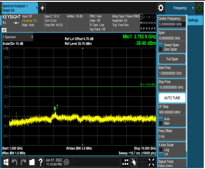
Band12-1.4MHz-16QAM-23017-1RB#0-Range2:1000~10000MHz
