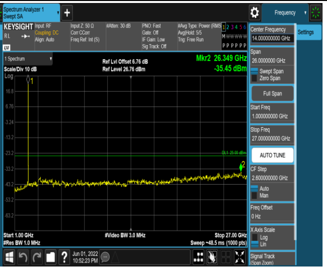
Band7-20MHz-16QAM-21100-1RB#0-Range2:1000~27000MHz
