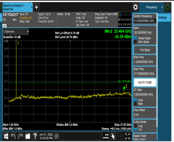
Band7-5MHz-16QAM-21425-1RB#0-Range2:1000~27000MHz
