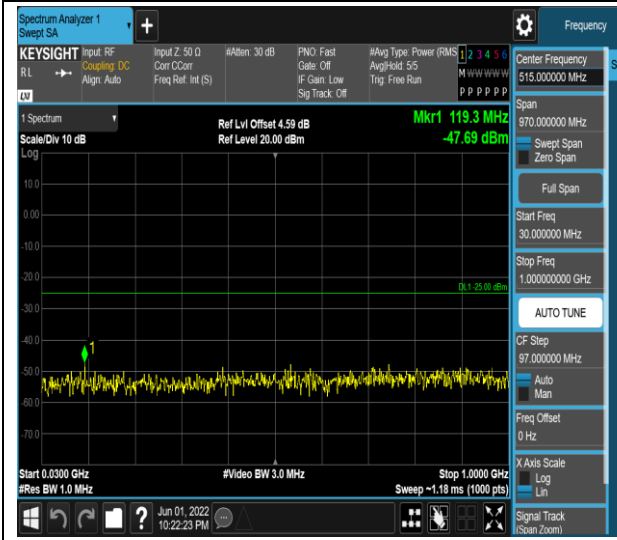
Band7-5MHz-16QAM-21425-1RB#0-Range1:30~1000MHz
