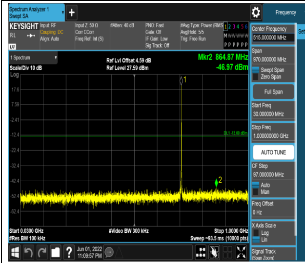
Band12-1.4MHz-16QAM-23017-1RB#0-Range1:30~1000MHz
