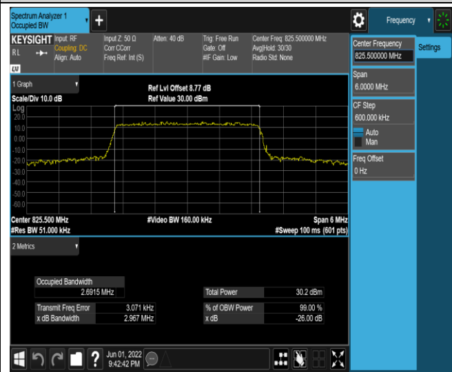
Band5-3MHz-16QAM-20635-15RB#0
