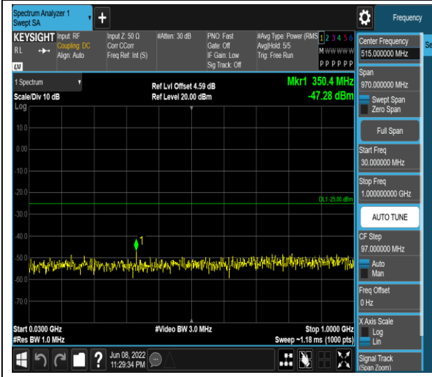
Band41-20MHz-16QAM-41140-1RB#0-Range1:30 ~1000MHz
