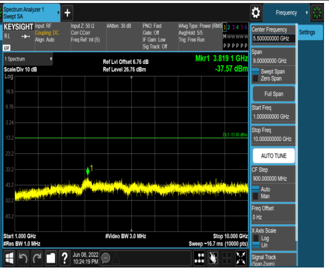
Band17-10MHz-16QAM-23800-1RB#0-Range2:1000~ 10000MHz
