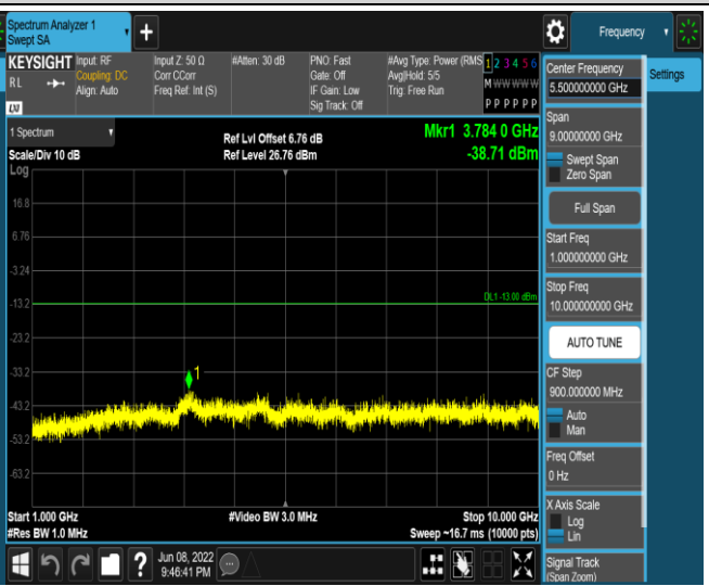
Band12-10MHz-QPSK-23060-1RB#0-Range2:1000~1 0000MHz
