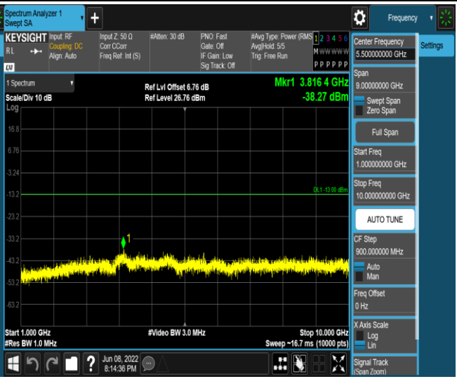
Band5-10MHz-16QAM-20600-1RB#0-Range2:1000~10000MHz
