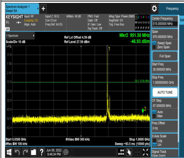
Band12-10MHz-QPSK-23060-1RB#0-Range1:30~ 1000MHz
