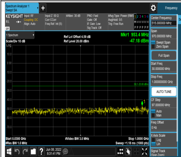
Band7-20MHz-QPSK-20850-1RB#0-Range1:30~1000MHz
