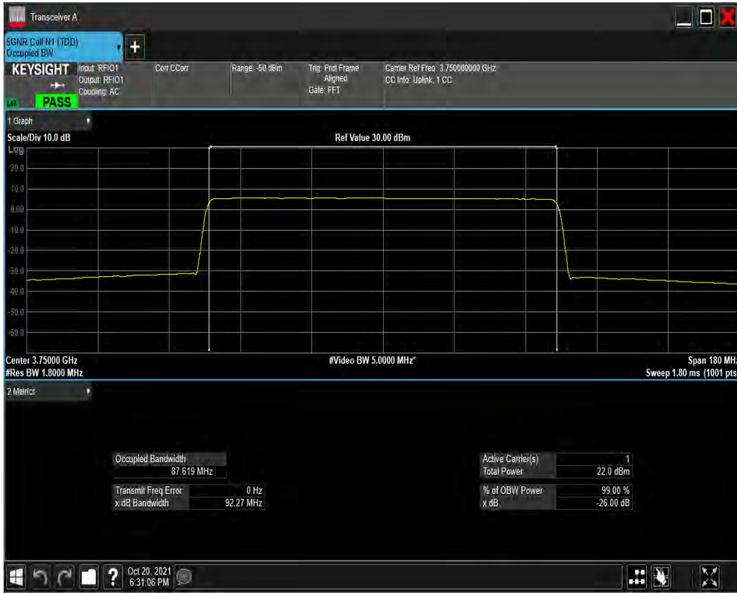
n78(3700-3800) SCS=30kHz CP_QAM256 BW=90MHz Channel=650000 RB=245@0
