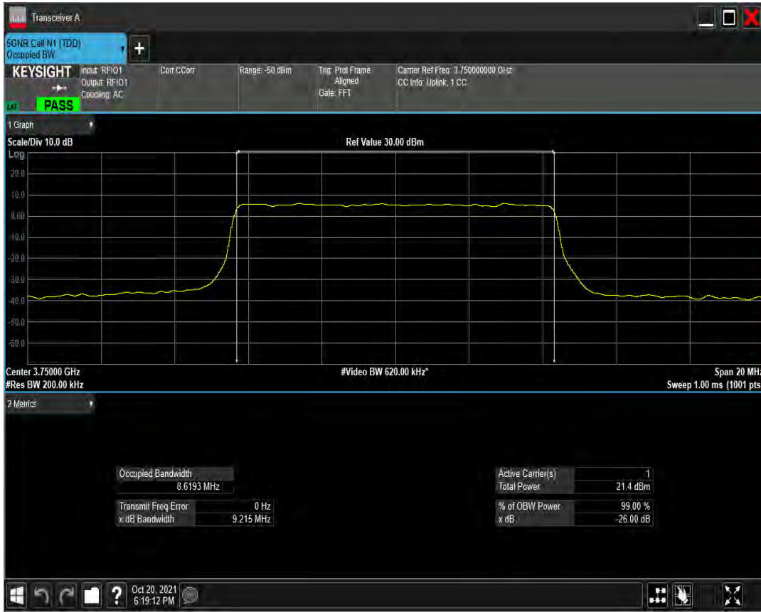
n78(3700-3800) SCS=30kHz CP_QPSK BW=10MHz Channel=650000 RB=24@0
