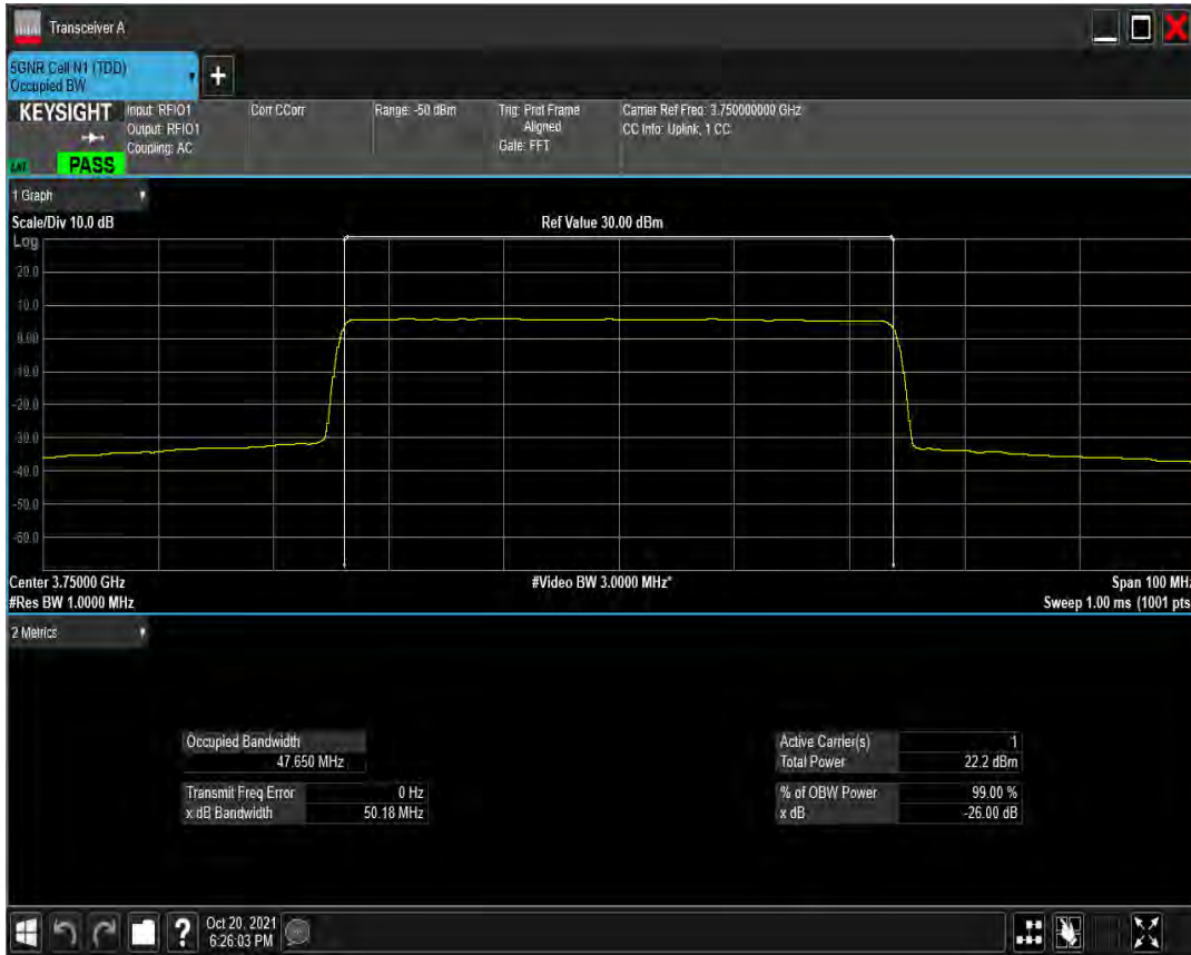
n78(3700-3800) SCS=30kHz CP_QAM256 BW=50MHz Channel=650000 RB=133@0
