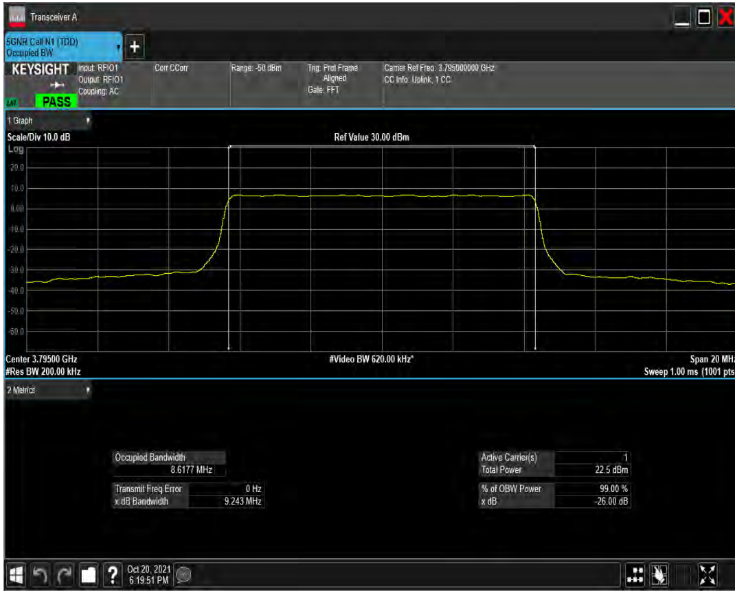
n78(3700-3800) SCS=30kHz CP_QAM64 BW=10MHz Channel=653000 RB=24@0
