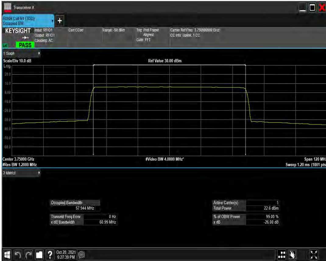
n78(3700-3800) SCS=30kHz CP_QAM16 BW=60MHz Channel=650000 RB=162@0
