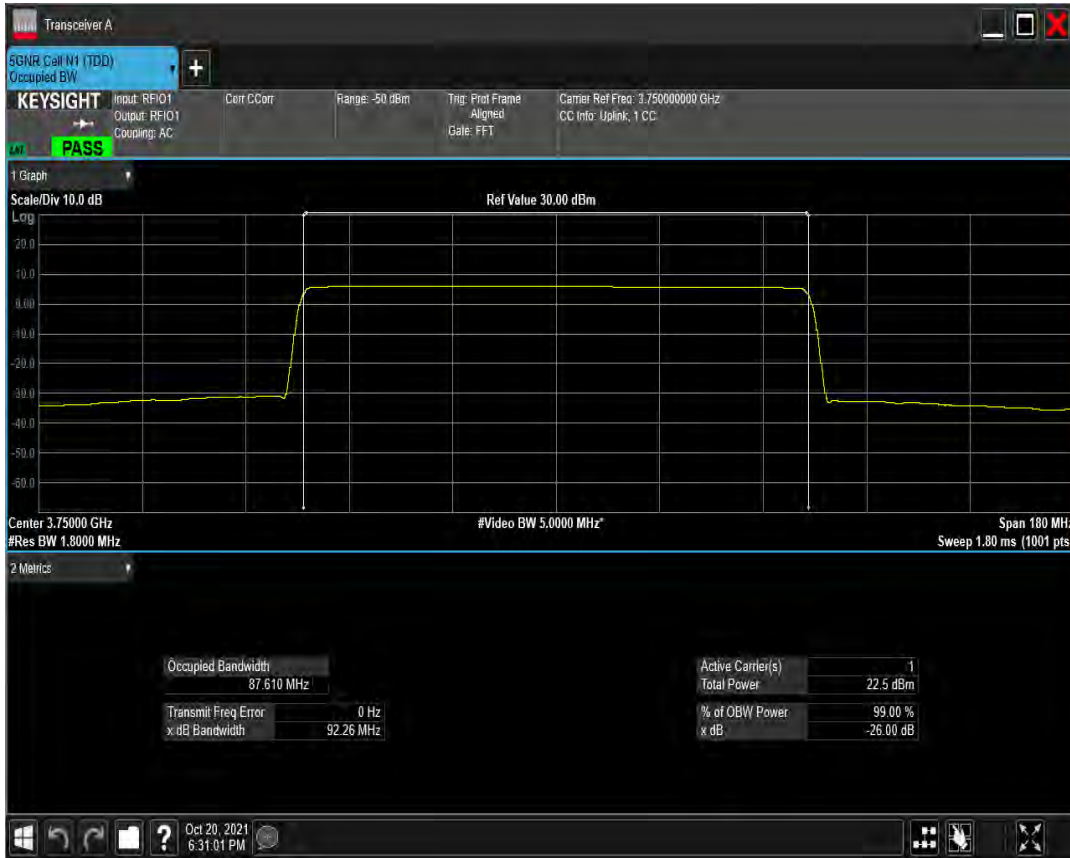
n78(3700-3800) SCS=30kHz CP_QAM16 BW=90MHz Channel=650000 RB=245@0
