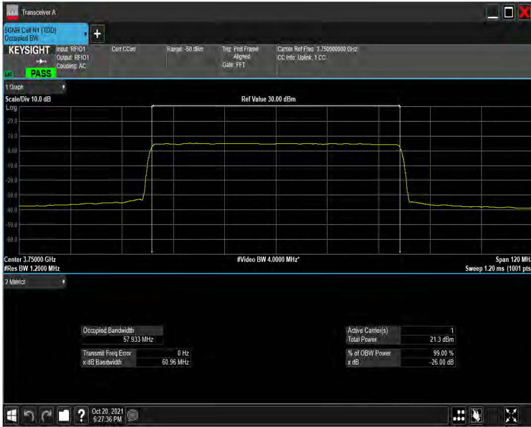
n78(3700-3800) SCS=30kHz CP_QPSK BW=60MHz Channel=650000 RB=162@0
