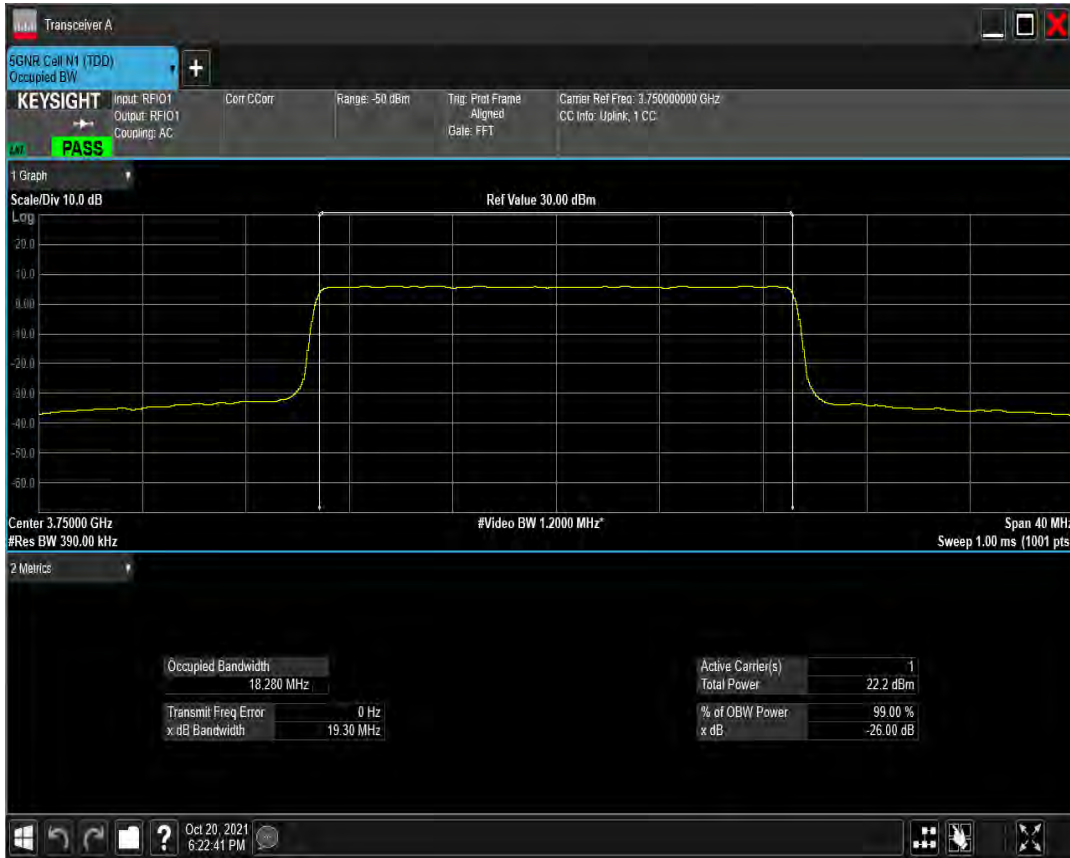
n78(3700-3800) SCS=30kHz CP_QAM256 BW=20MHz Channel=650000 RB=51 @0
