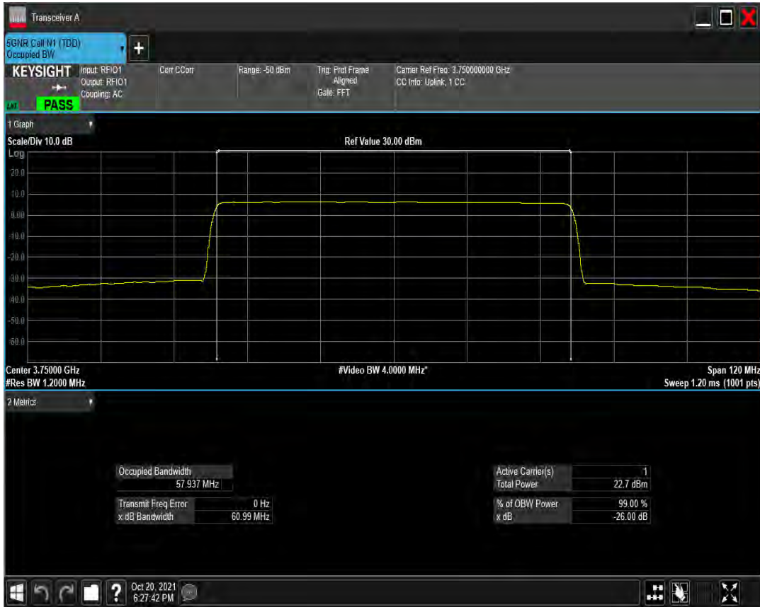
n78(3700-3800) SCS=30kHz CP_QAM64 BW=60MHz Channel=650000 RB=162@0
