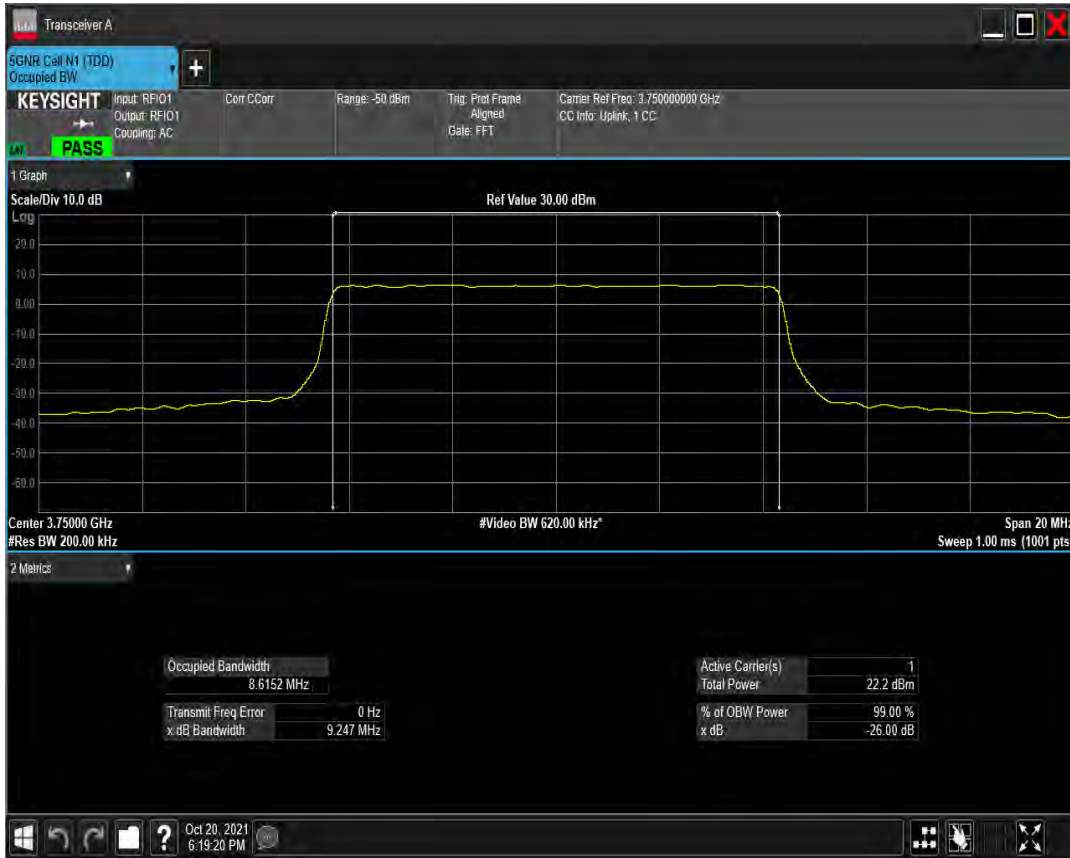
n78(3700-3800) SCS=30kHz CP_QAM256 BW=10MHz Channel=650000 RB=24@0
