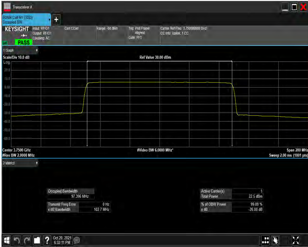
n78(3700-3800) SCS=30kHz CP_QAM64 BW=100MHz Channel=650000 RB=273@0
