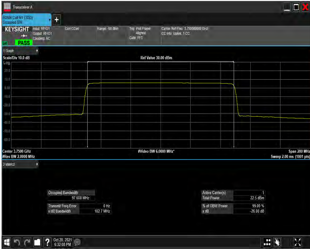
n78(3700-3800) SCS=30kHz CP_QAM16 BW=100MHz Channel=650000 RB=273@0
