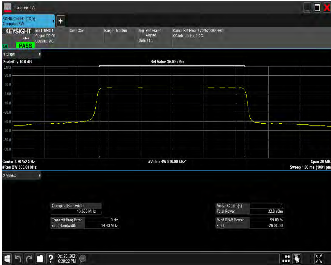
n78(3700-3800) SCS=30kHz CP_QAM16 BW=15MHz Channel=647168 RB=38@0
