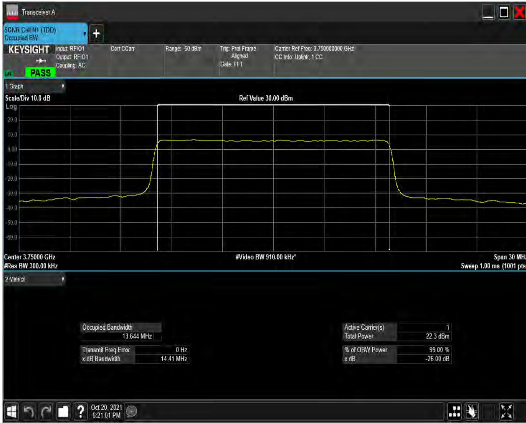
n78(3700-3800) SCS=30kHz CP_QAM256 BW=15MHz Channel=650000 RB=38@0
