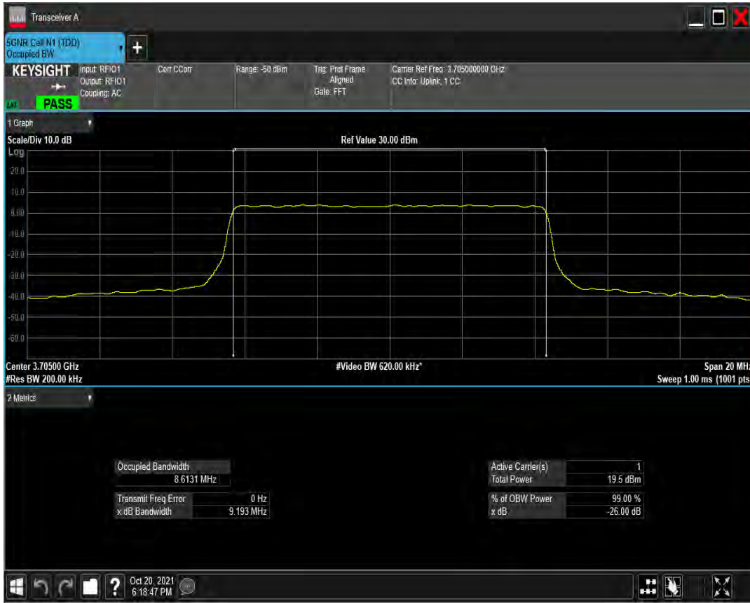
n78(3700-3800) SCS=30kHz CP_QAM256 BW=10MHz Channel=647000 RB=24@0
