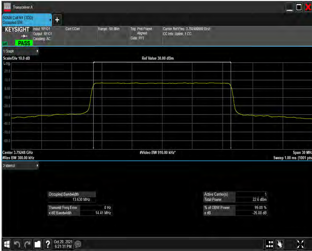
n78(3700-3800) SCS=30kHz CP_QAM64 BW=15MHz Channel=652832 RB=38@0
