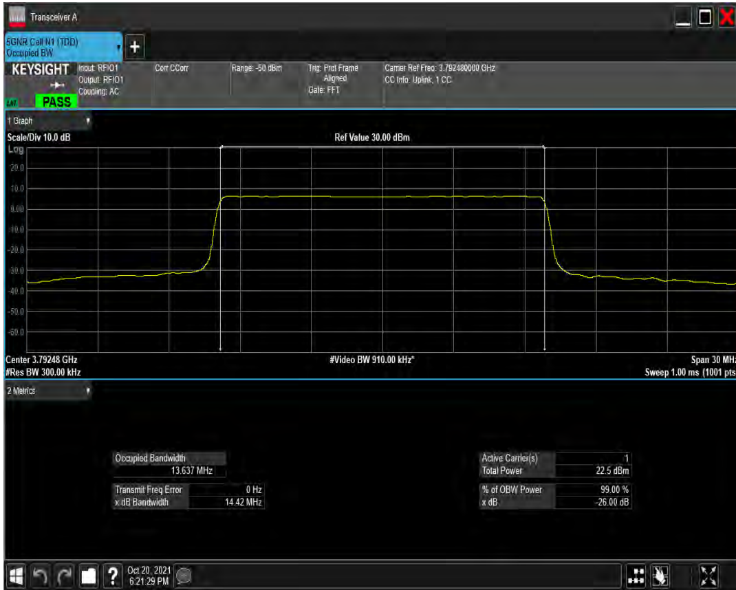
n78(3700-3800) SCS=30kHz CP_QAM16 BW=15MHz Channel=652832 RB=38@0
