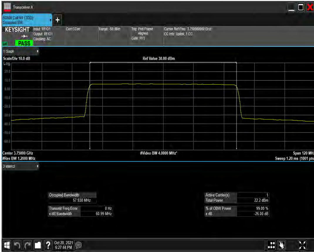
n78(3700-3800) SCS=30kHz CP_QAM256 BW=60MHz Channel=650000 RB=162@0
