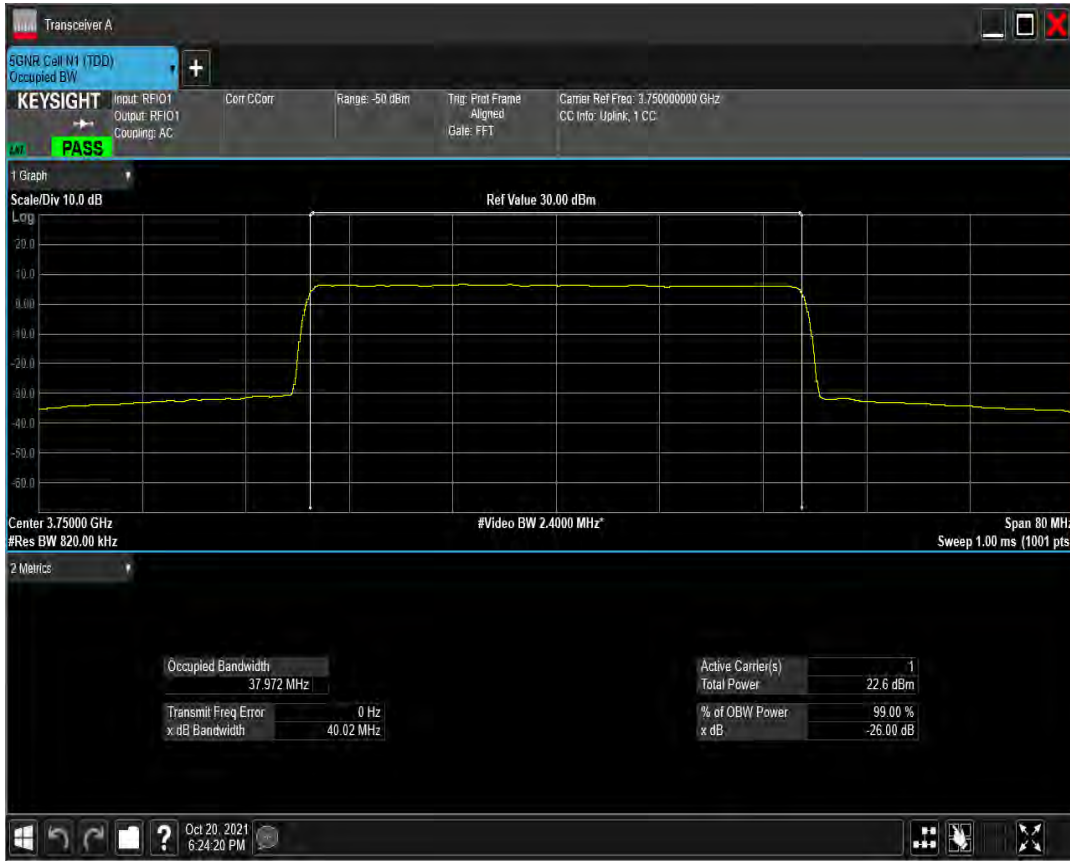
n78(3700-3800) SCS=30kHz CP_QAM64 BW=40MHz Channel=650000 RB=106@0
