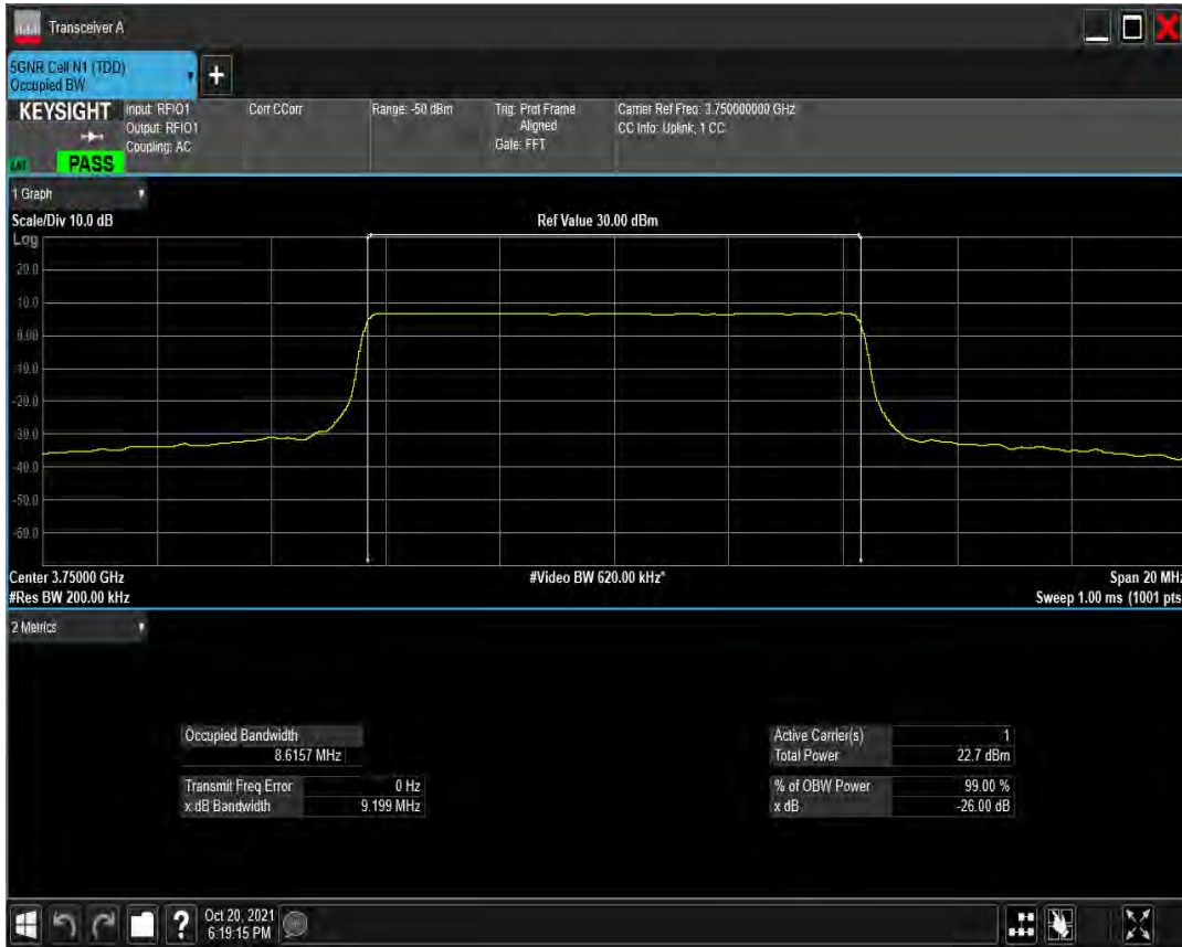
n78(3700-3800) SCS=30kHz CP_QAM16 BW=10MHz Channel=650000 RB=24@0
