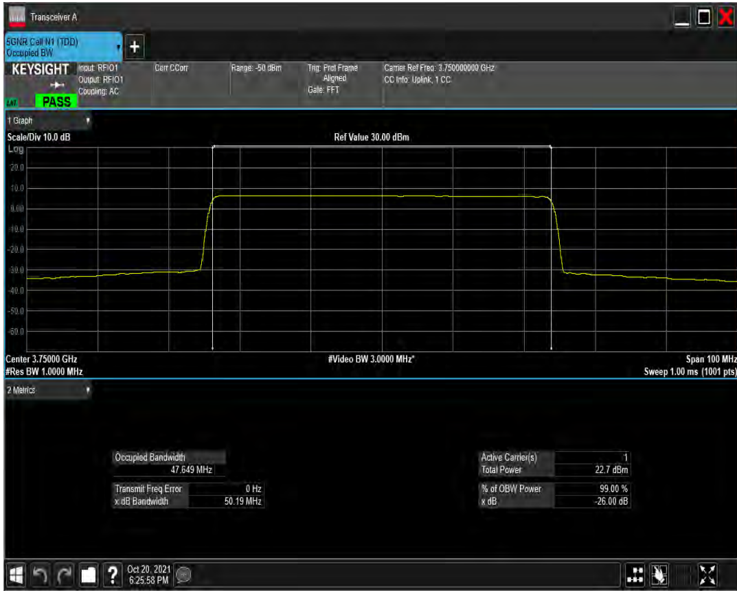
n78(3700-3800) SCS=30kHz CP_QAM16 BW=50MHz Channel=650000 RB=133@0
