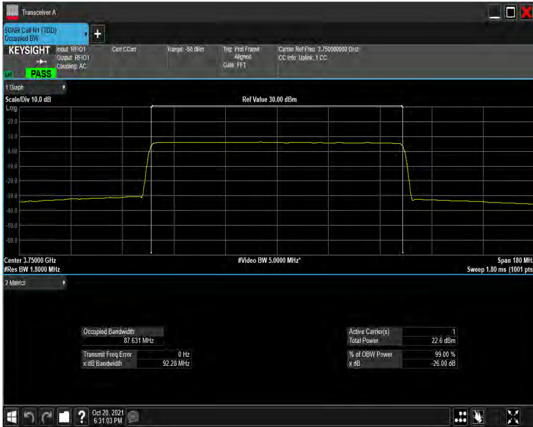
n78(3700-3800) SCS=30kHz CP_QAM64 BW=90MHz Channel=650000 RB=245@0
