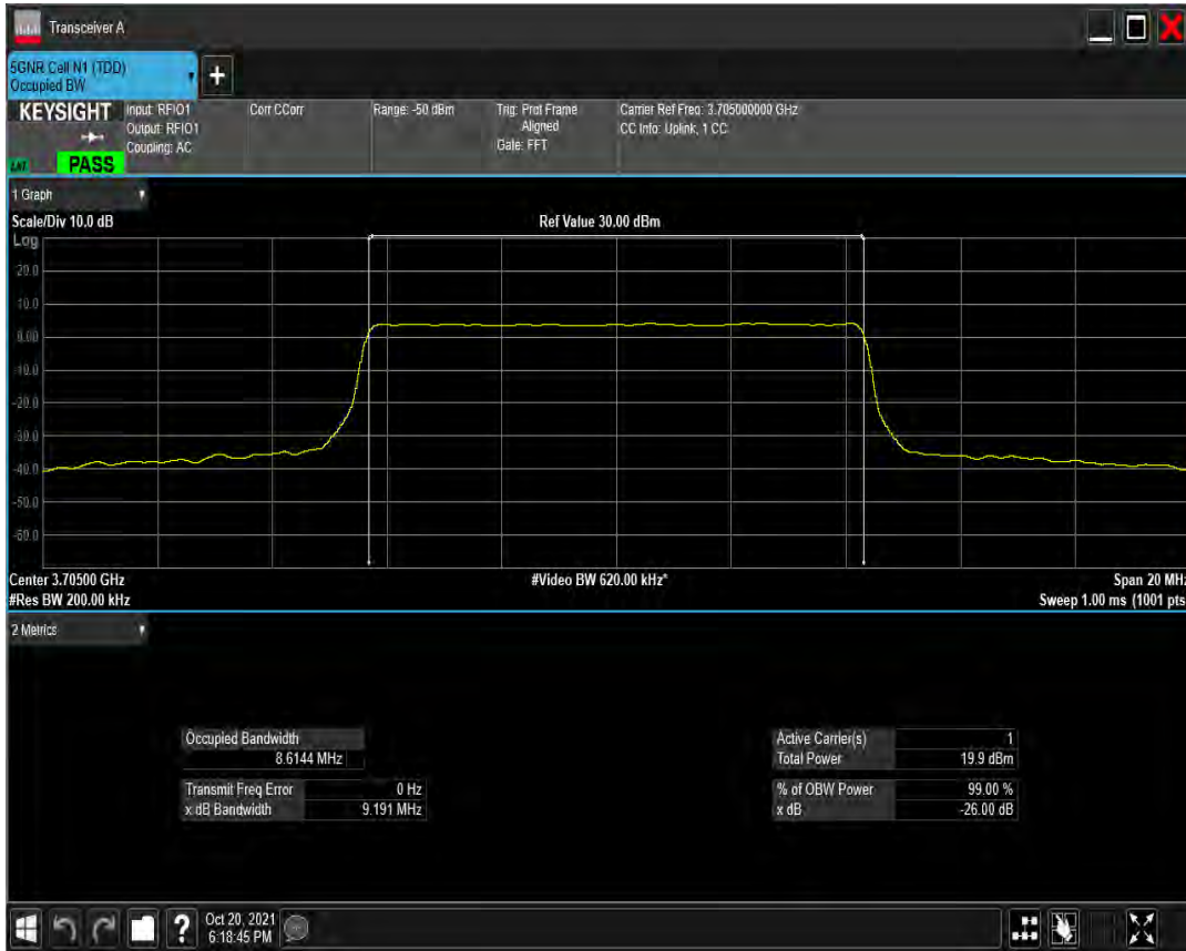
n78(3700-3800) SCS=30kHz CP_QAM64 BW=10MHz Channel=647000 RB=24@0
