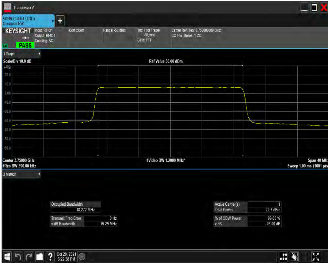
n78(3700-3800) SCS=30kHz CP_QAM64 BW=20MHz Channel=650000 RB=51 @0
