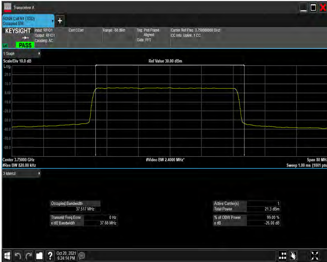
n78(3700-3800) SCS=30kHz CP_QPSK BW=40MHz Channel=650000 RB=106@0
