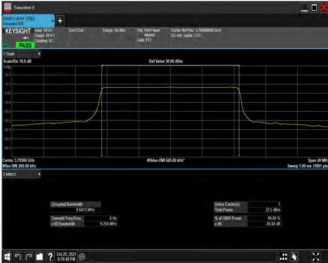
n78(3700-3800) SCS=30kHz CP_QAM16 BW=10MHz Channel=653000 RB=24@0
