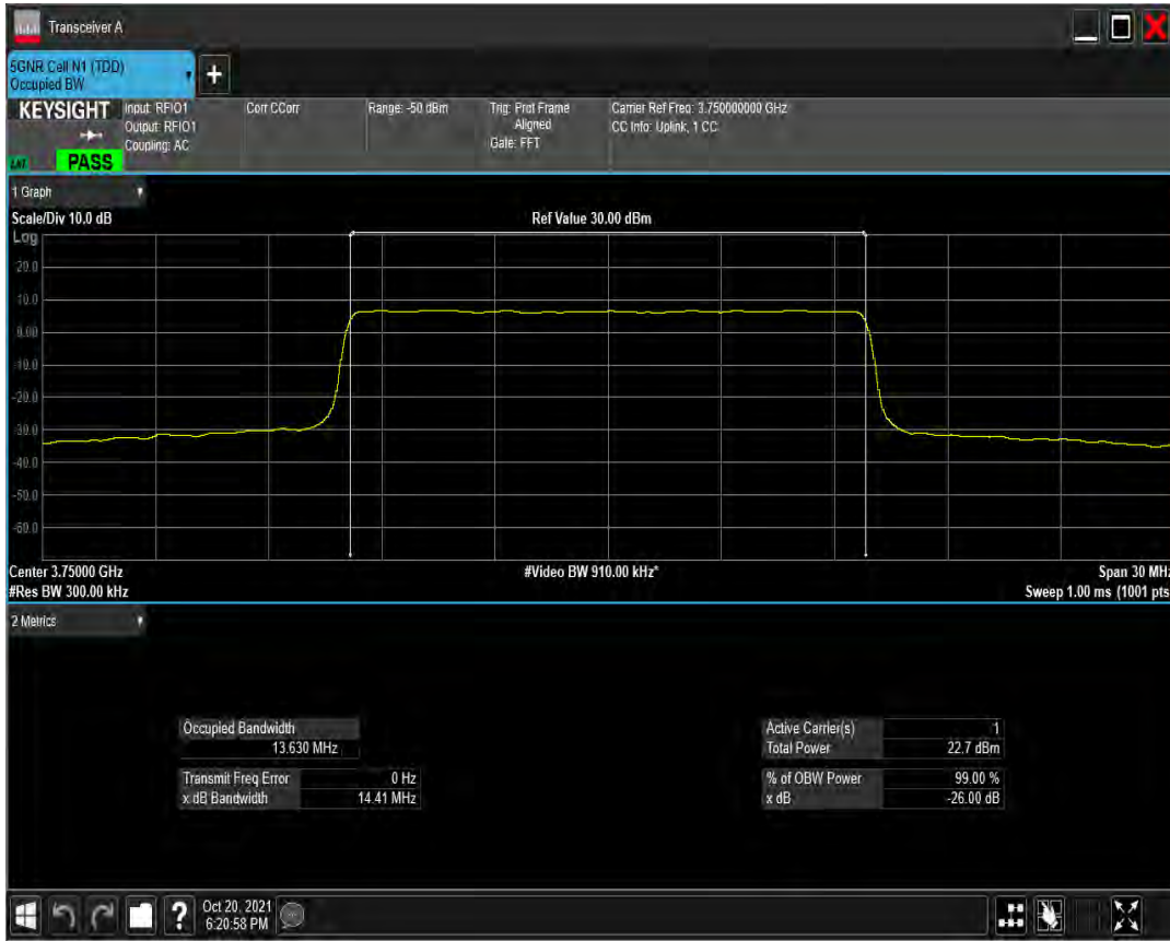
n78(3700-3800) SCS=30kHz CP_QAM64 BW=15MHz Channel=650000 RB=38@0
