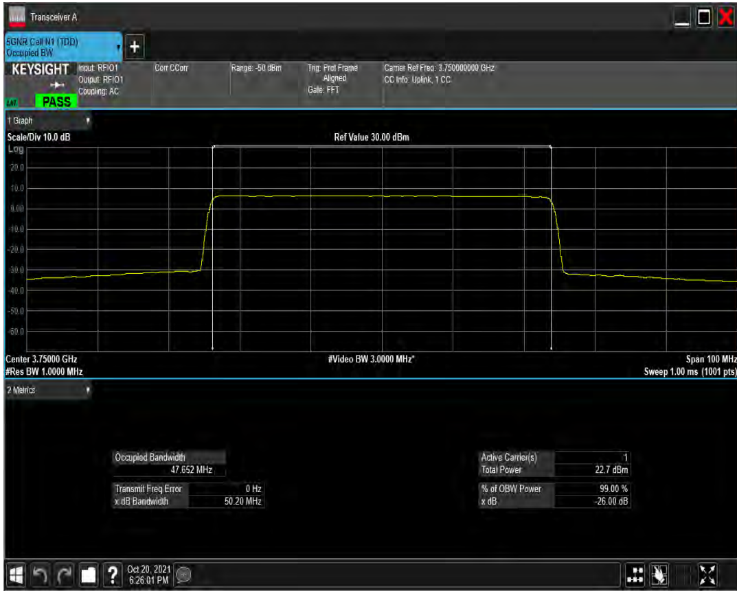
n78(3700-3800) SCS=30kHz CP_QAM64 BW=50MHz Channel=650000 RB=133@0
