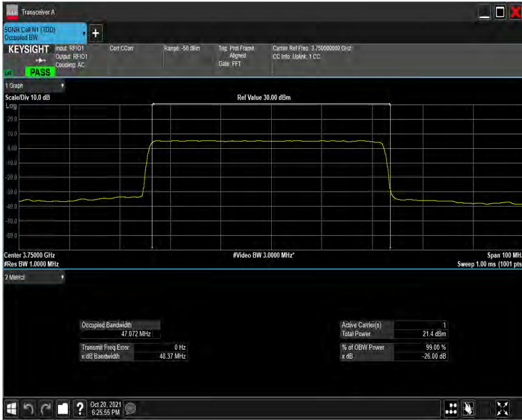
n78(3700-3800) SCS=30kHz CP_QPSK BW=50MHz Channel=650000 RB=133@0
