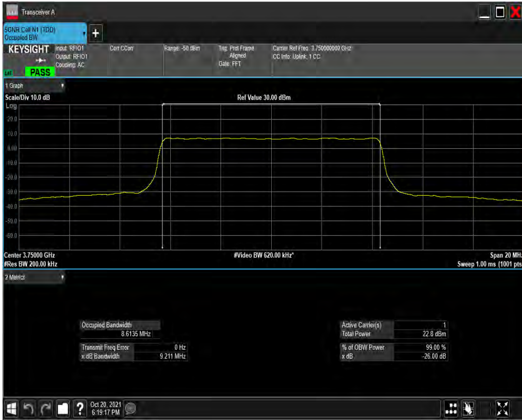
n78(3700-3800) SCS=30kHz CP_QAM64 BW=10MHz Channel=650000 RB=24@0
