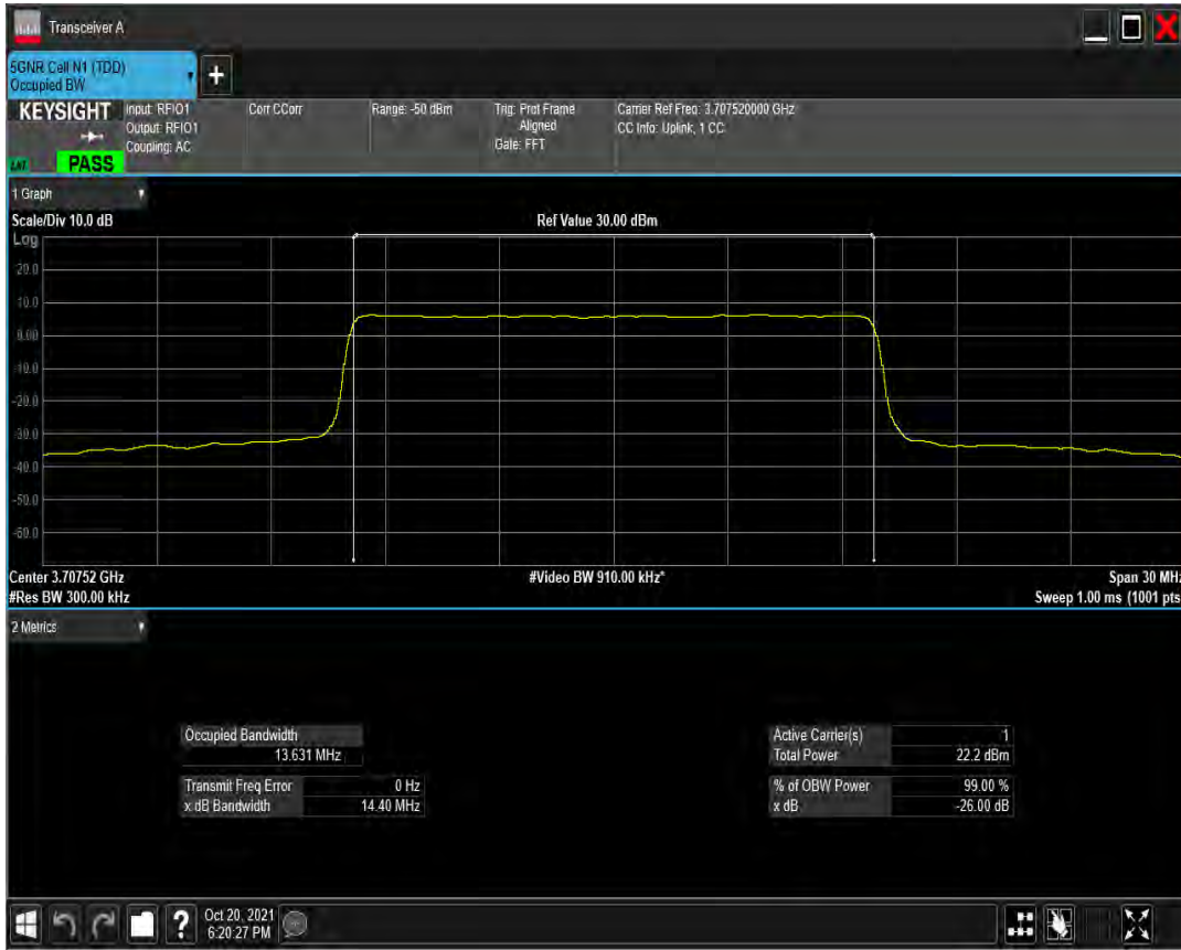
n78(3700-3800) SCS=30kHz CP_QAM256 BW=15MHz Channel=647168 RB=38@0
