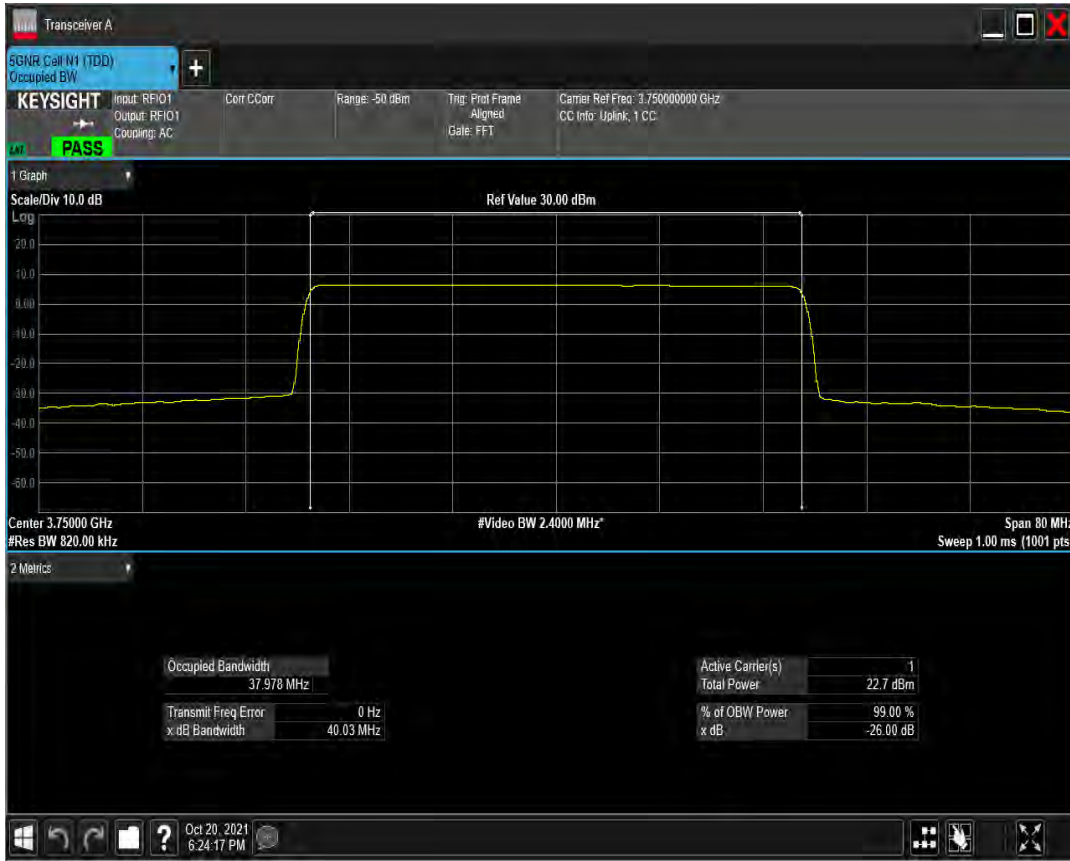
n78(3700-3800) SCS=30kHz CP_QAM16 BW=40MHz Channel=650000 RB=106@0
