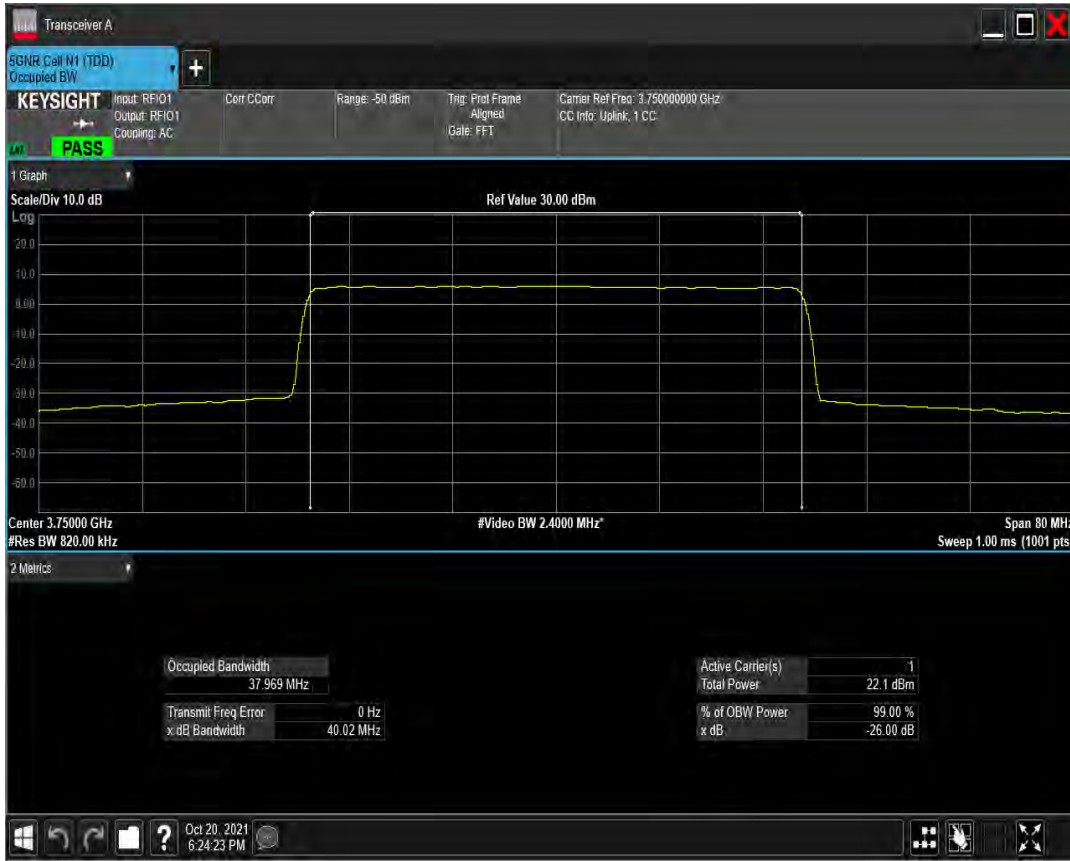
n78(3700-3800) SCS=30kHz CP_QAM256 BW=40MHz Channel=650000 RB=106@0
