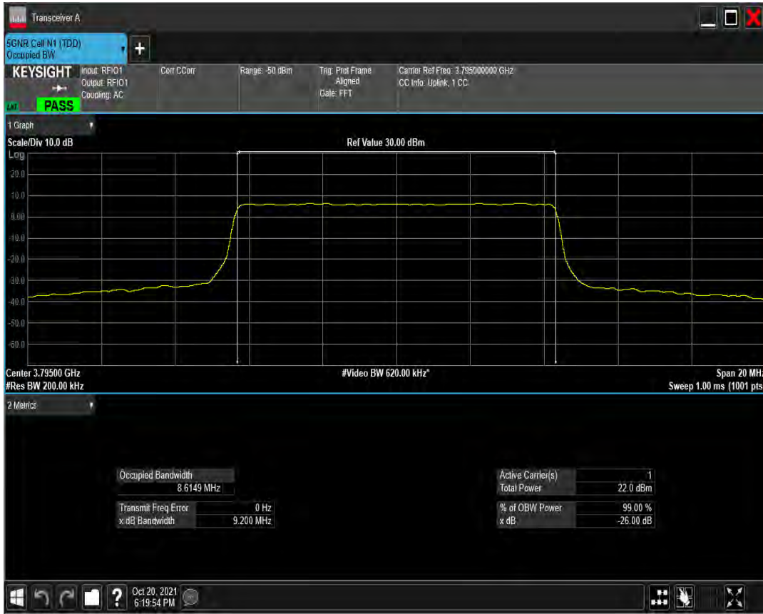
n78(3700-3800) SCS=30kHz CP_QAM256 BW=10MHz Channel=653000 RB=24@0
