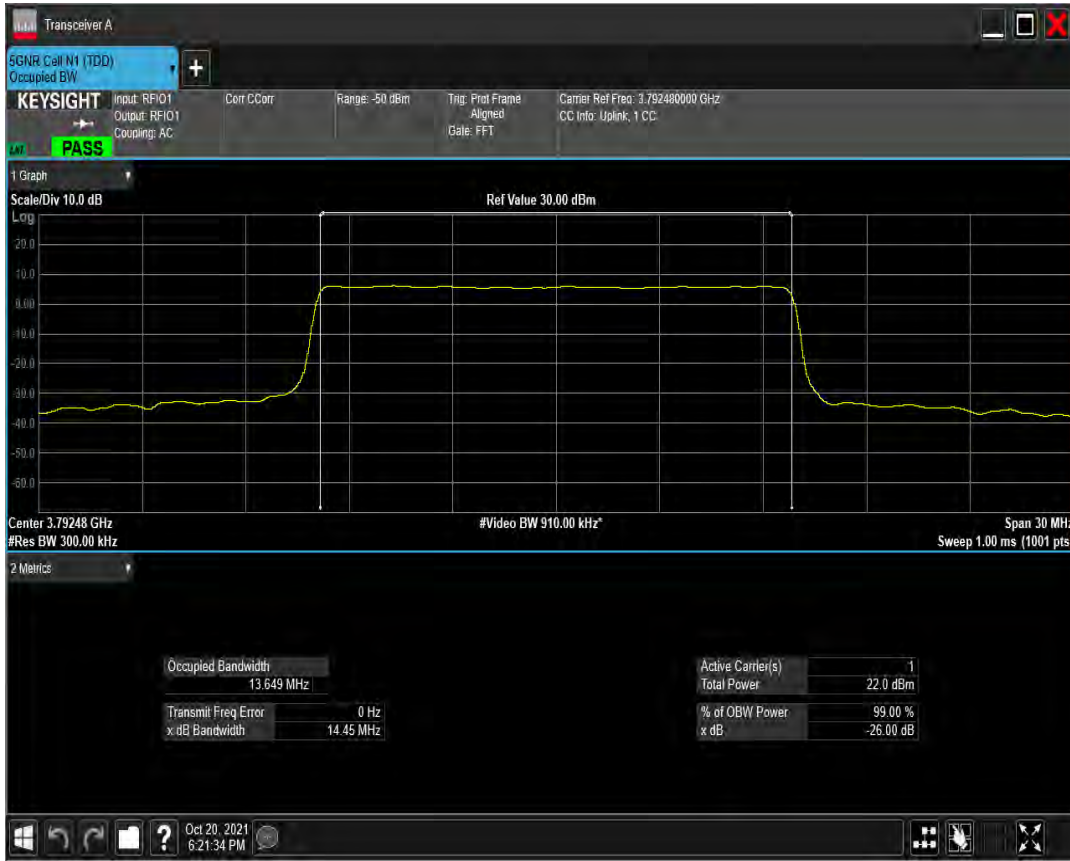
n78(3700-3800) SCS=30kHz CP_QAM256 BW=15MHz Channel=652832 RB=38@0
