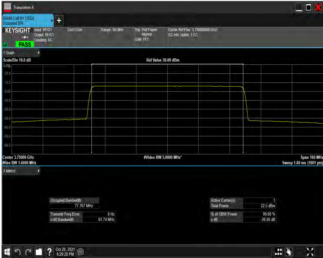
n78(3700-3800) SCS=30kHz CP_QAM16 BW=80MHz Channel=650000 RB=217@0
