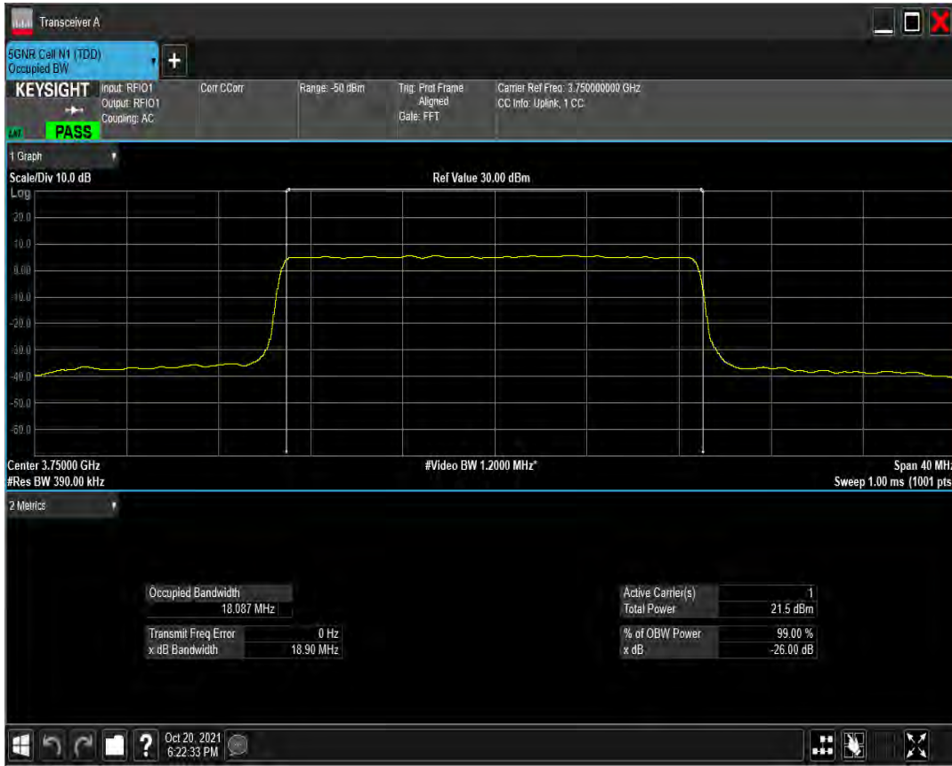
n78(3700-3800) SCS=30kHz CP_QPSK BW=20MHz Channel=650000 RB=51 @0
