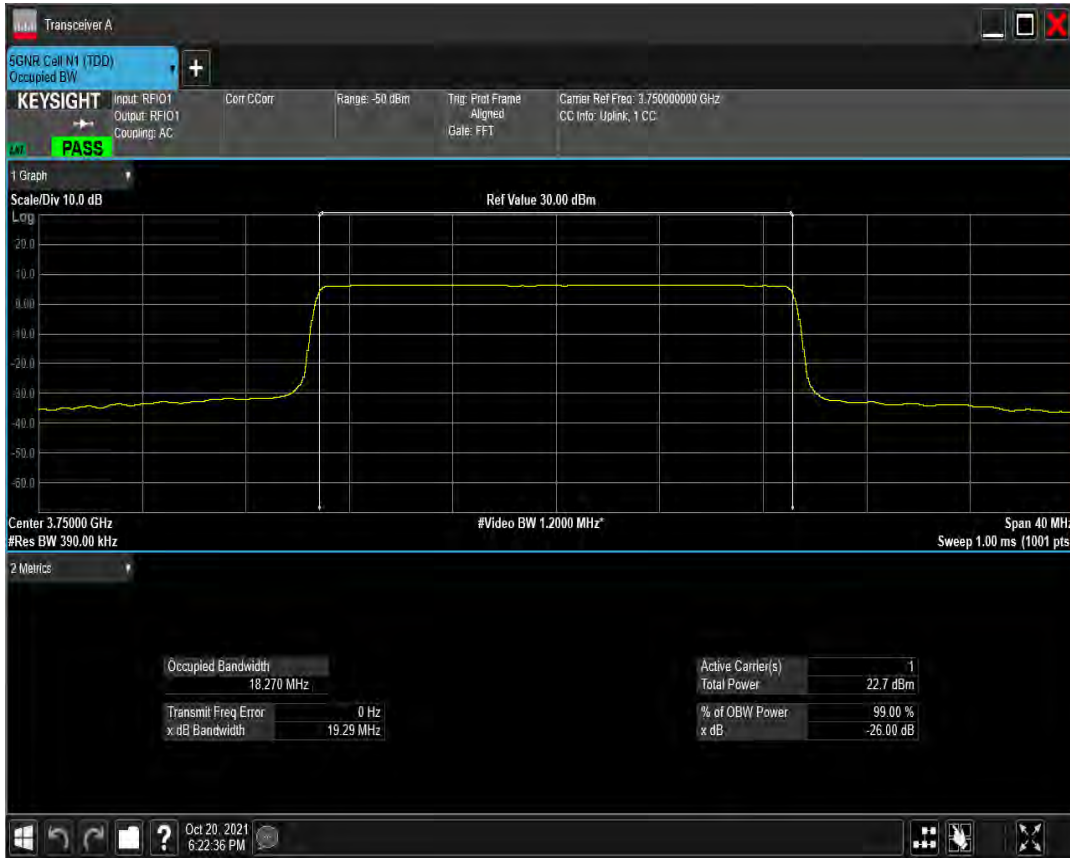
n78(3700-3800) SCS=30kHz CP_QAM16 BW=20MHz Channel=650000 RB=51 @0
