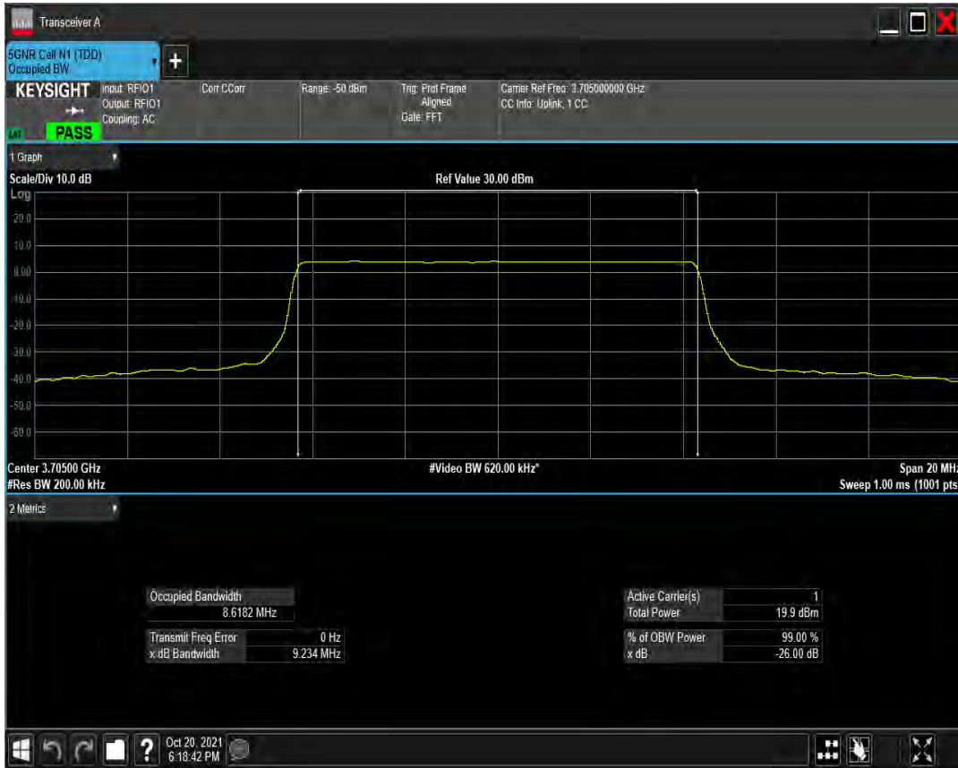
n78(3700-3800) SCS=30kHz CP_QAM16 BW=10MHz Channel=647000 RB=24@0
