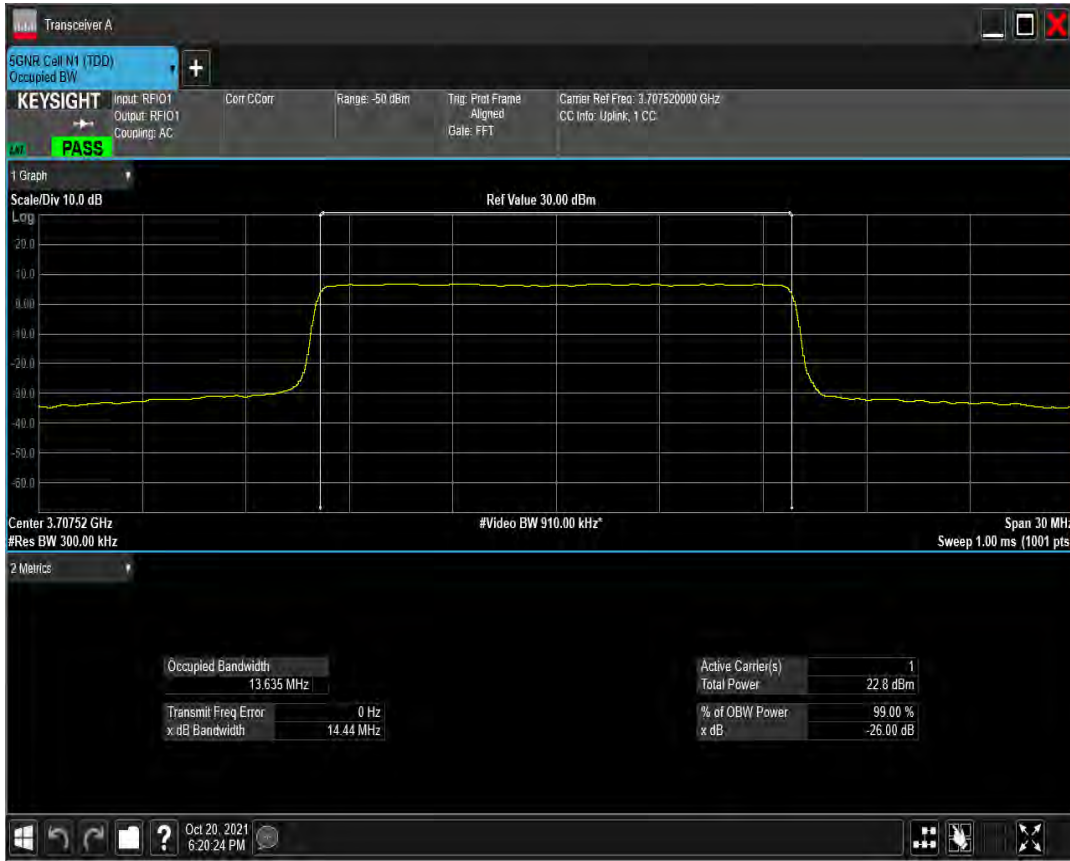
n78(3700-3800) SCS=30kHz CP_QAM64 BW=15MHz Channel=647168 RB=38@0
