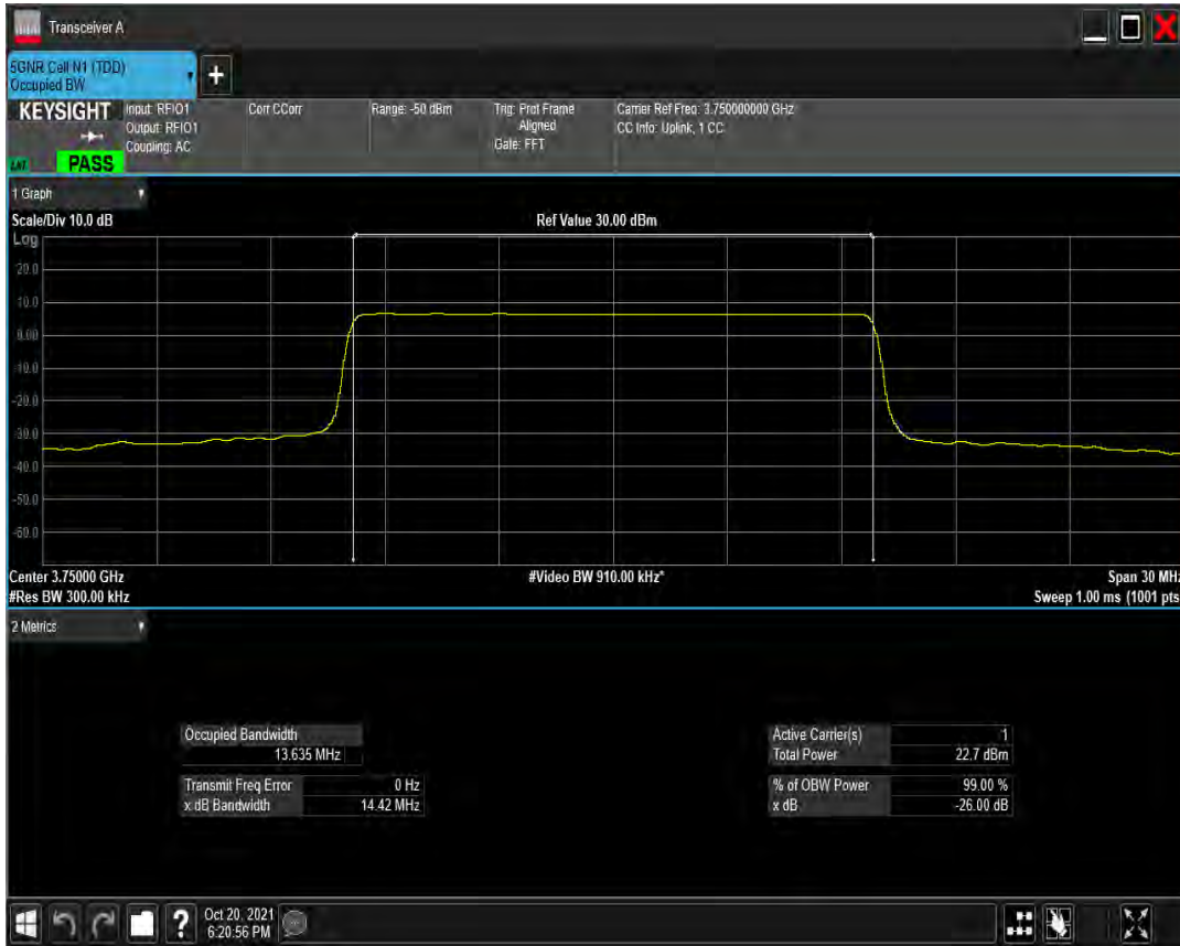
n78(3700-3800) SCS=30kHz CP_QAM16 BW=15MHz Channel=650000 RB=38@0
