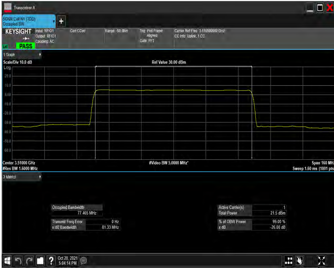
n77(3450-3550) SCS=30kHz CP_QPSK BW=80MHz Channel=634000 RB=217@0
