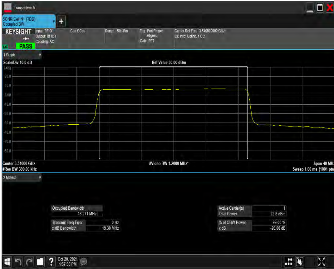
n77(3450-3550) SCS=30kHz CP_QAM16 BW=20MHz Channel=636000 RB=51 @0
