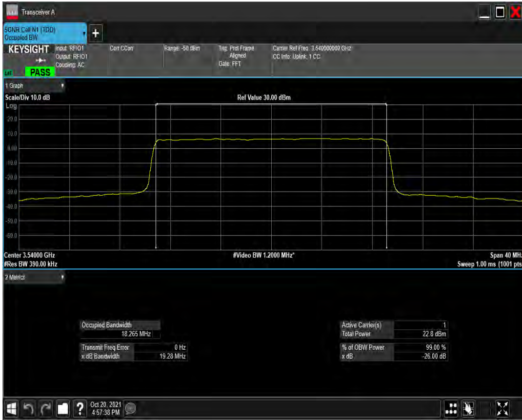
n77(3450-3550) SCS=30kHz CP_QAM64 BW=20MHz Channel=636000 RB=51 @0
