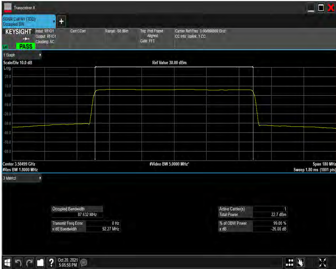
n77(3450-3550) SCS=30kHz CP_QAM16 BW=90MHz Channel=633666 RB=245@0
