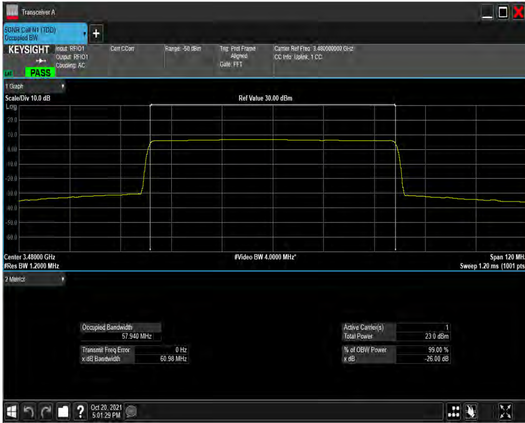
n77(3450-3550) SCS=30kHz CP_QAM16 BW=60MHz Channel=632000 RB=162@0
