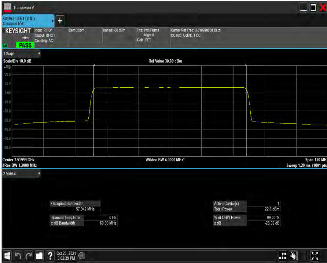
n77(3450-3550) SCS=30kHz CP_QAM64 BW=60MHz Channel=634666 RB=162@0
