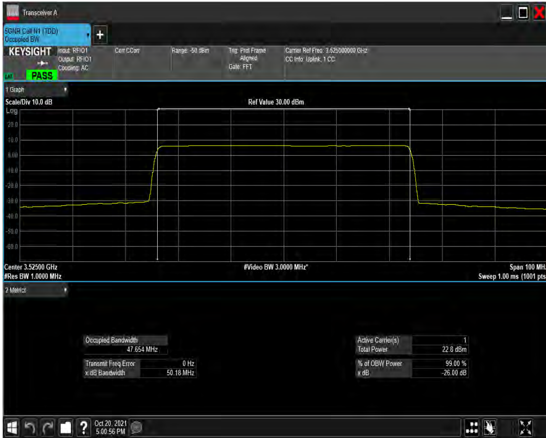
n77(3450-3550) SCS=30kHz CP_QAM16 BW=50MHz Channel=635000 RB=133@0
