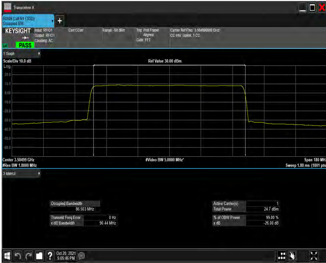
n77(3450-3550) SCS=30kHz DFT_QAM16 BW=90MHz Channel=633666 RB=240@0
