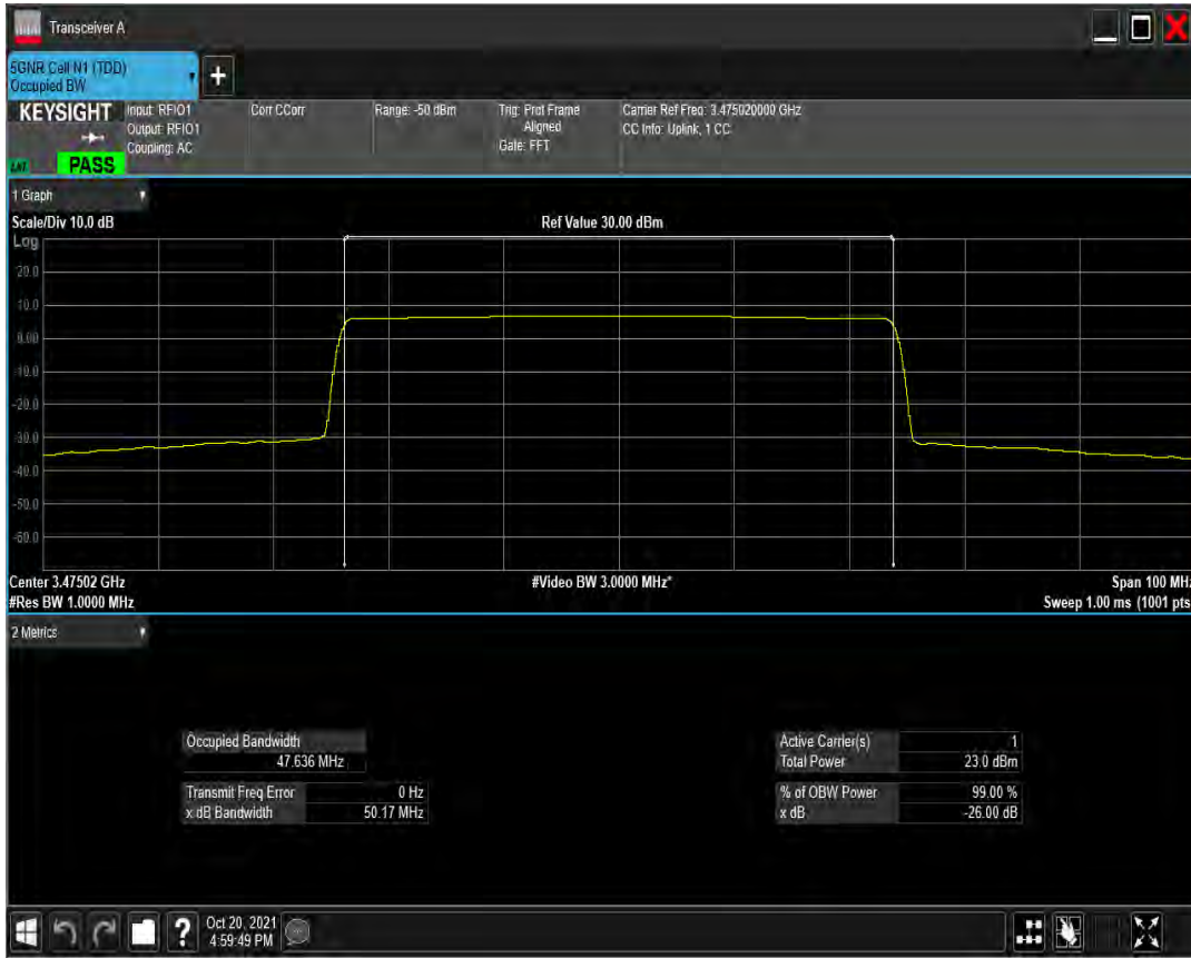
n77(3450-3550) SCS=30kHz CP_QAM16 BW=50MHz Channel=631668 RB=133@0
