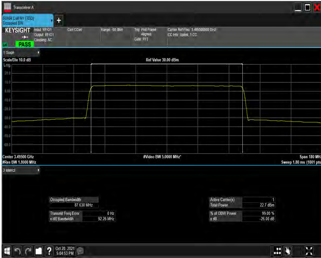
n77(3450-3550) SCS=30kHz CP_QAM64 BW=90MHz Channel=633000 RB=245@0
