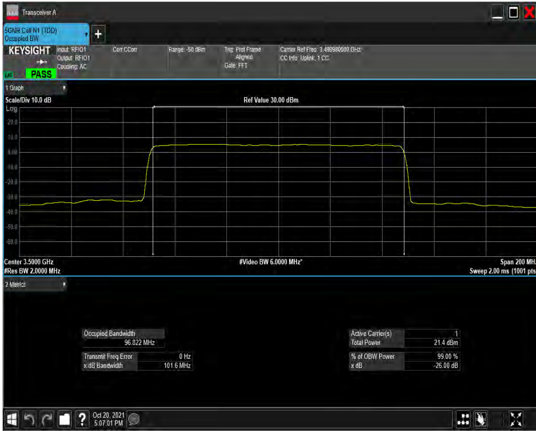
n77(3450-3550) SCS=30kHz CP_QPSK BW=100MHz Channel=633332 RB=273@0
