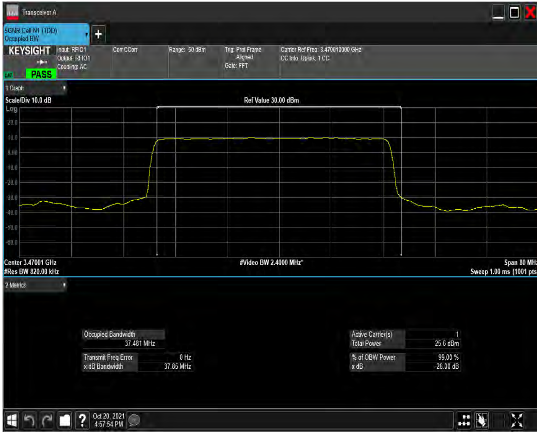
n77(3450-3550) SCS=30kHz DFT_QPSK BW=40MHz Channel=631334 RB=100@0
