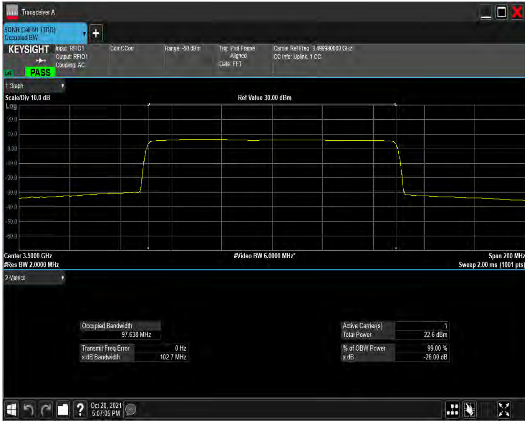
n77(3450-3550) SCS=30kHz CP_QAM16 BW=100MHz Channel=633332 RB=273@0
