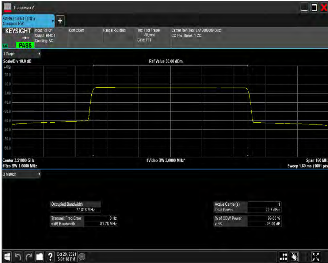
n77(3450-3550) SCS=30kHz CP_QAM16 BW=80MHz Channel=634000 RB=217@0
