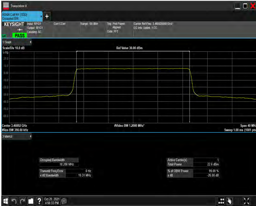
n77(3450-3550) SCS=30kHz CP_QAM256 BW=20MHz Channel=630668 RB=51 @0
