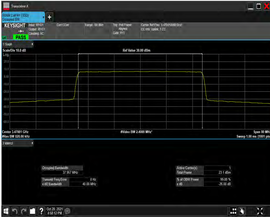
n77(3450-3550) SCS=30kHz CP_QAM64 BW=40MHz Channel=631334 RB=106@0
