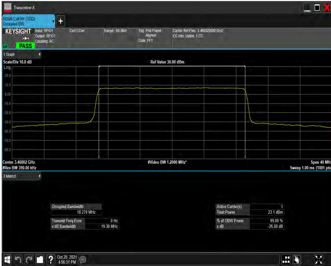
n77(3450-3550) SCS=30kHz CP_QAM64 BW=20MHz Channel=630668 RB=51 @0
