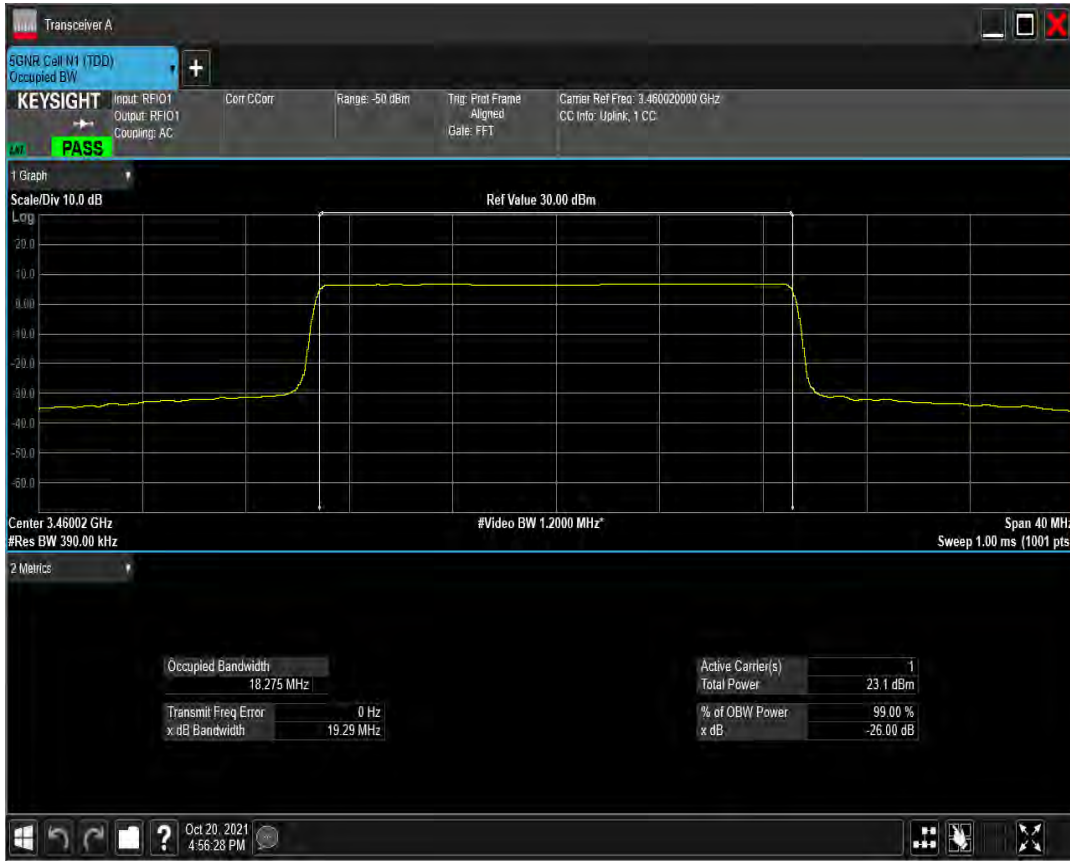
n77(3450-3550) SCS=30kHz CP_QAM16 BW=20MHz Channel=630668 RB=51 @0
