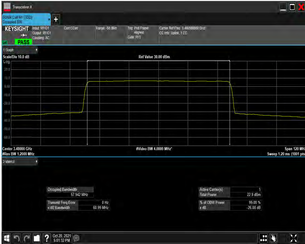
n77(3450-3550) SCS=30kHz CP_QAM64 BW=60MHz Channel=632000 RB=162@0
