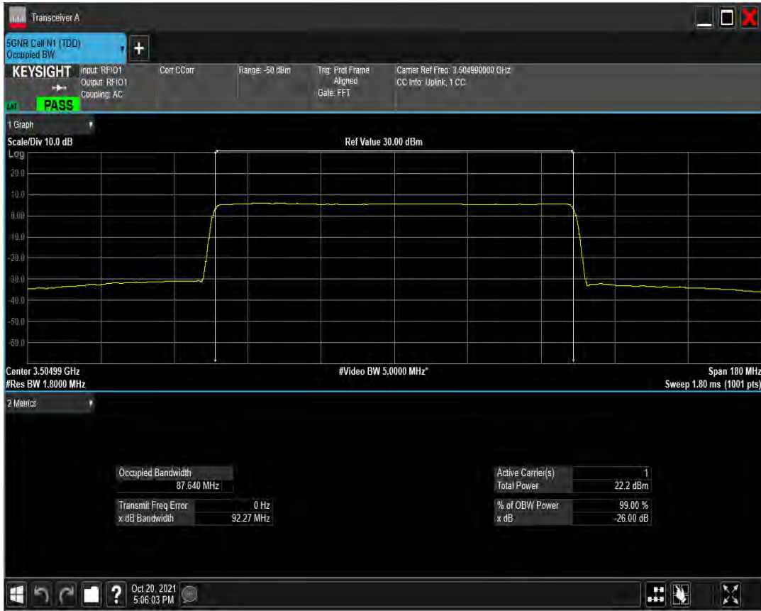
n77(3450-3550) SCS=30kHz CP_QAM256 BW=90MHz Channel=633666 RB=245@0
