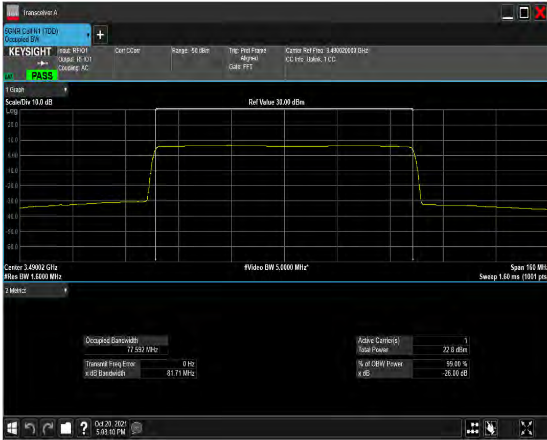
n77(3450-3550) SCS=30kHz CP_QAM16 BW=80MHz Channel=632668 RB=217@0
