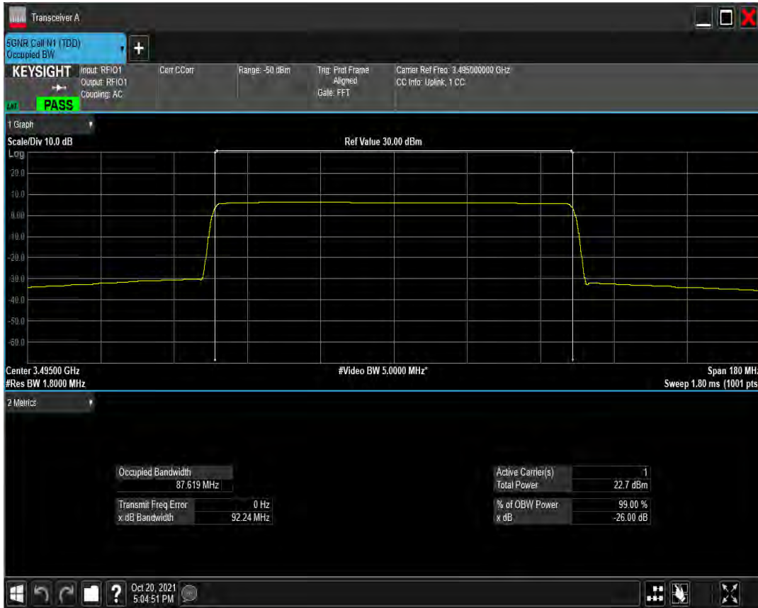
n77(3450-3550) SCS=30kHz CP_QAM16 BW=90MHz Channel=633000 RB=245@0
