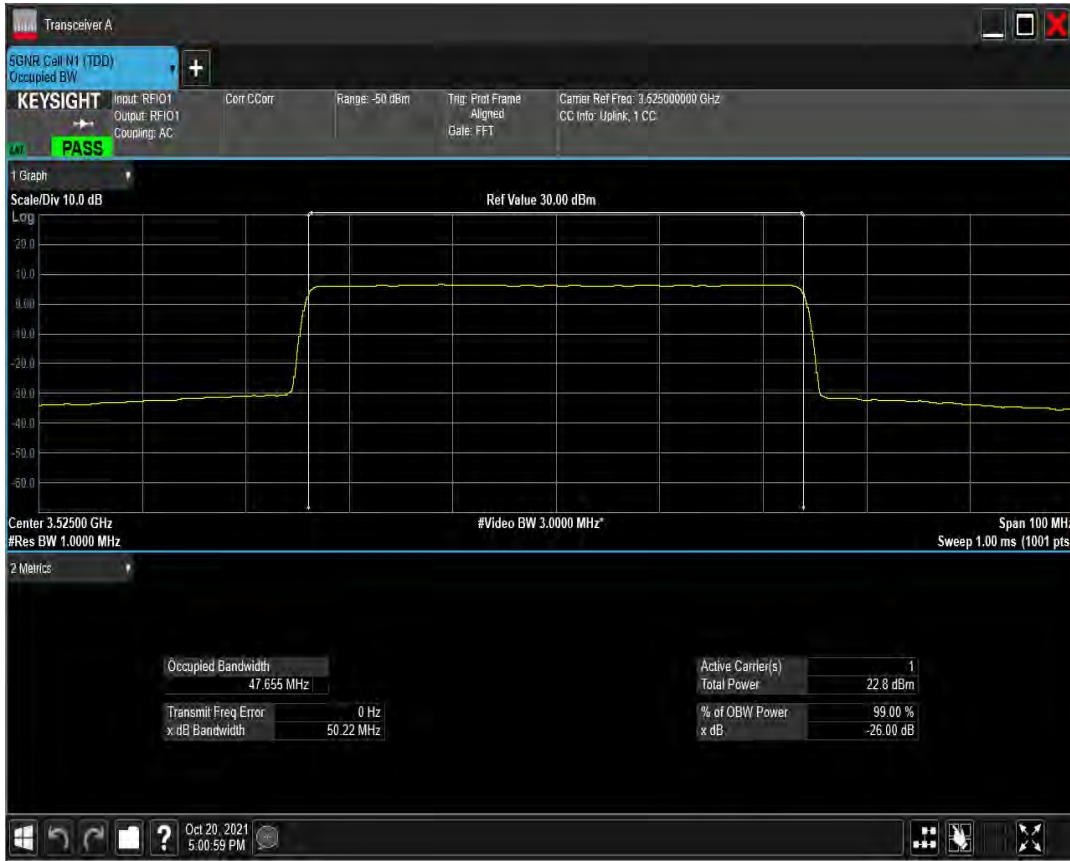
n77(3450-3550) SCS=30kHz CP_QAM64 BW=50MHz Channel=635000 RB=133@0
