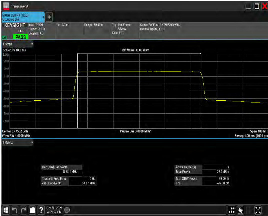
n77(3450-3550) SCS=30kHz CP_QAM64 BW=50MHz Channel=631668 RB=133@0
