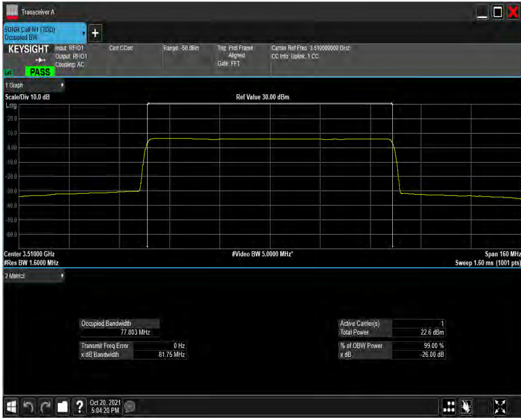
n77(3450-3550) SCS=30kHz CP_QAM64 BW=80MHz Channel=634000 RB=217@0
