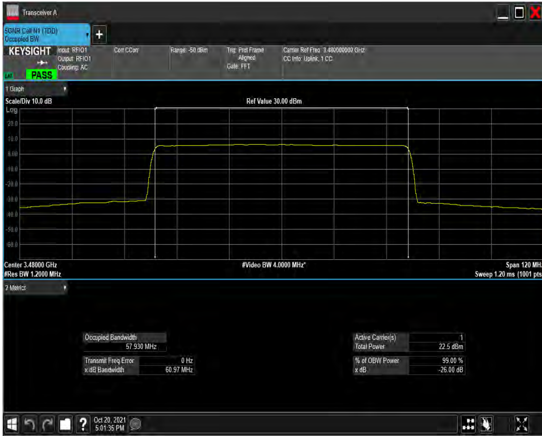
n77(3450-3550) SCS=30kHz CP_QAM256 BW=60MHz Channel=632000 RB=162@0
