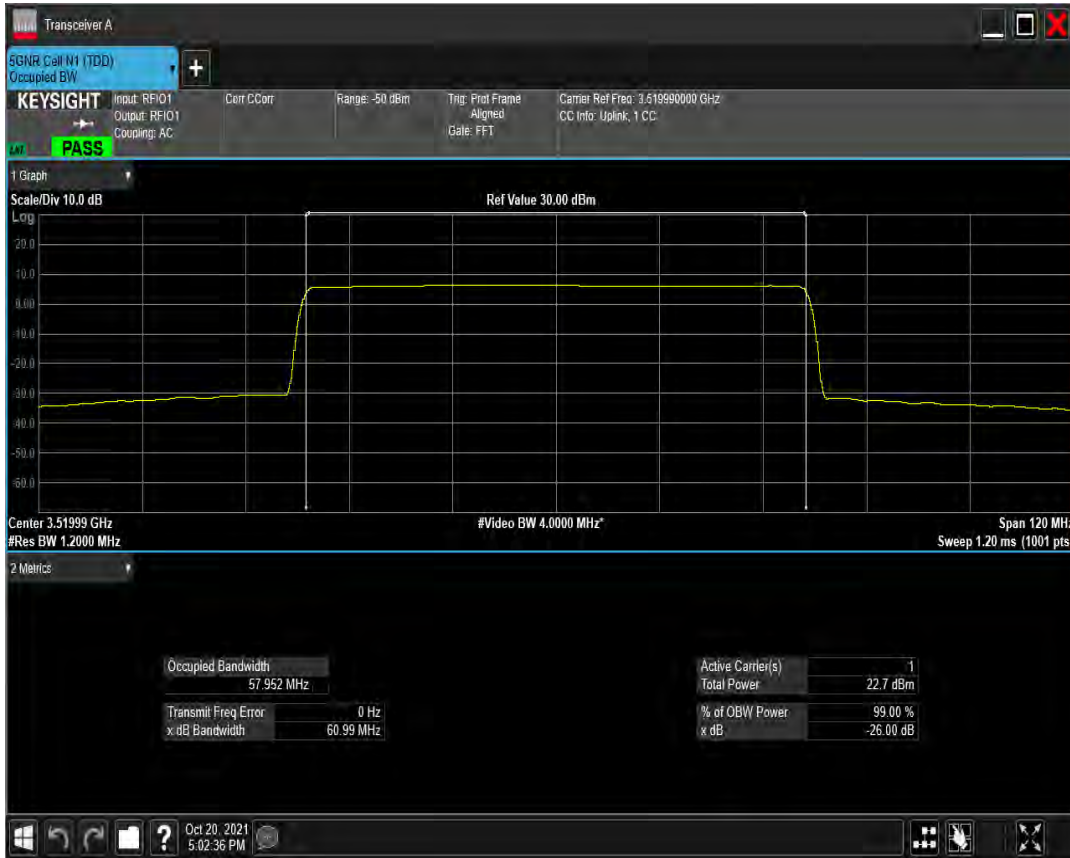
n77(3450-3550) SCS=30kHz CP_QAM16 BW=60MHz Channel=634666 RB=162@0
