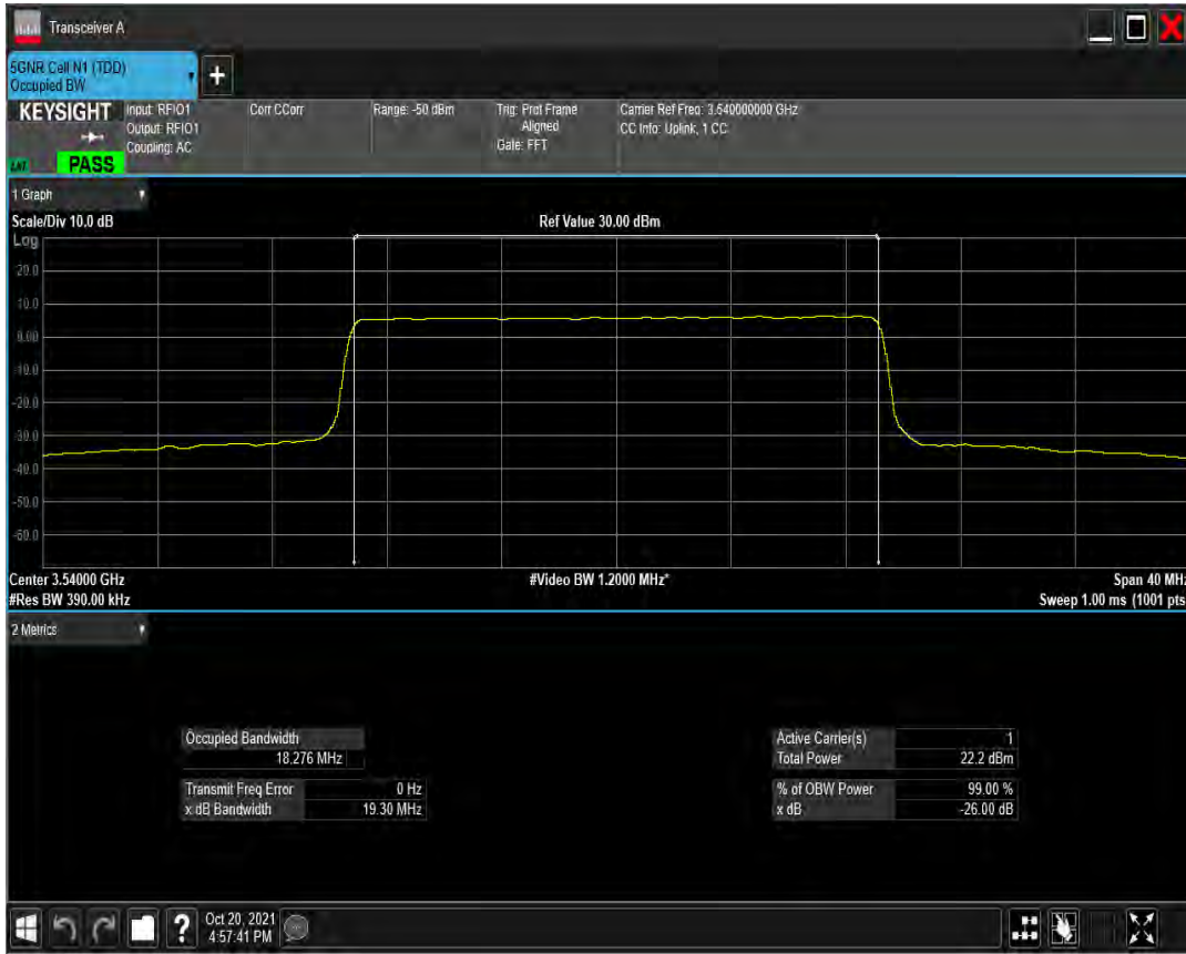
n77(3450-3550) SCS=30kHz CP_QAM256 BW=20MHz Channel=636000 RB=51 @0
