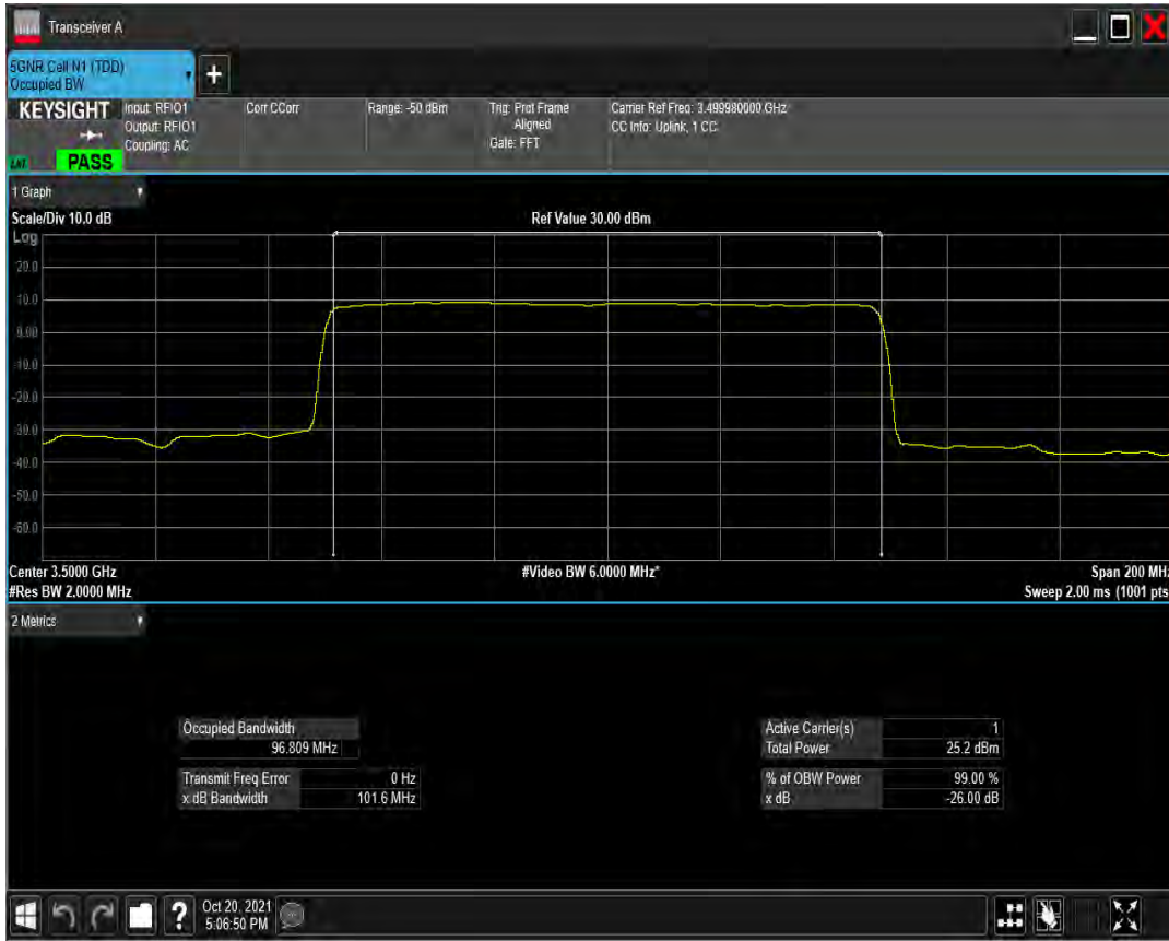
n77(3450-3550) SCS=30kHz DFT_QPSK BW=100MHz Channel=633332 RB=270@0
