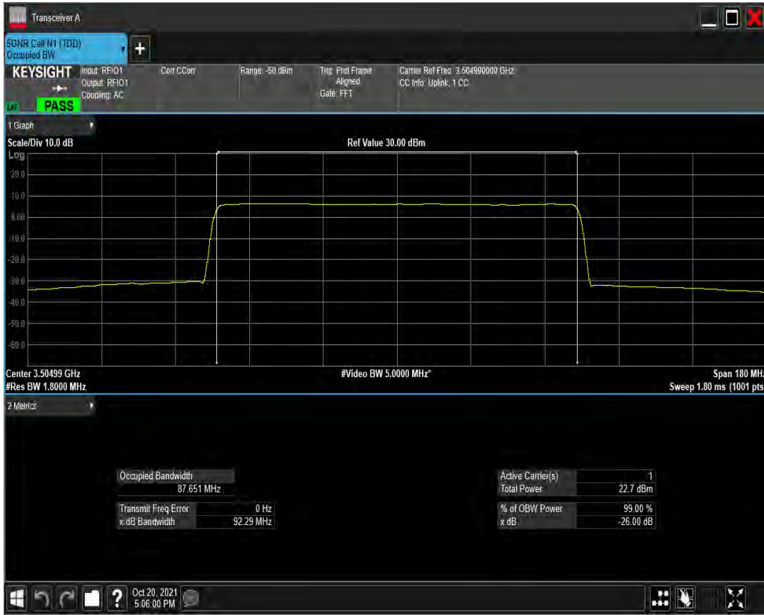
n77(3450-3550) SCS=30kHz CP_QAM64 BW=90MHz Channel=633666 RB=245@0
