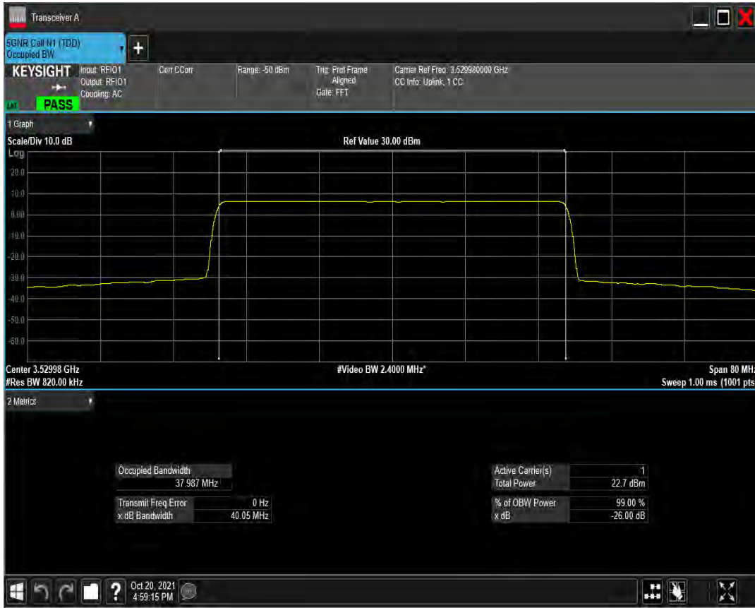
n77(3450-3550) SCS=30kHz CP_QAM16 BW=40MHz Channel=635332 RB=106@0
