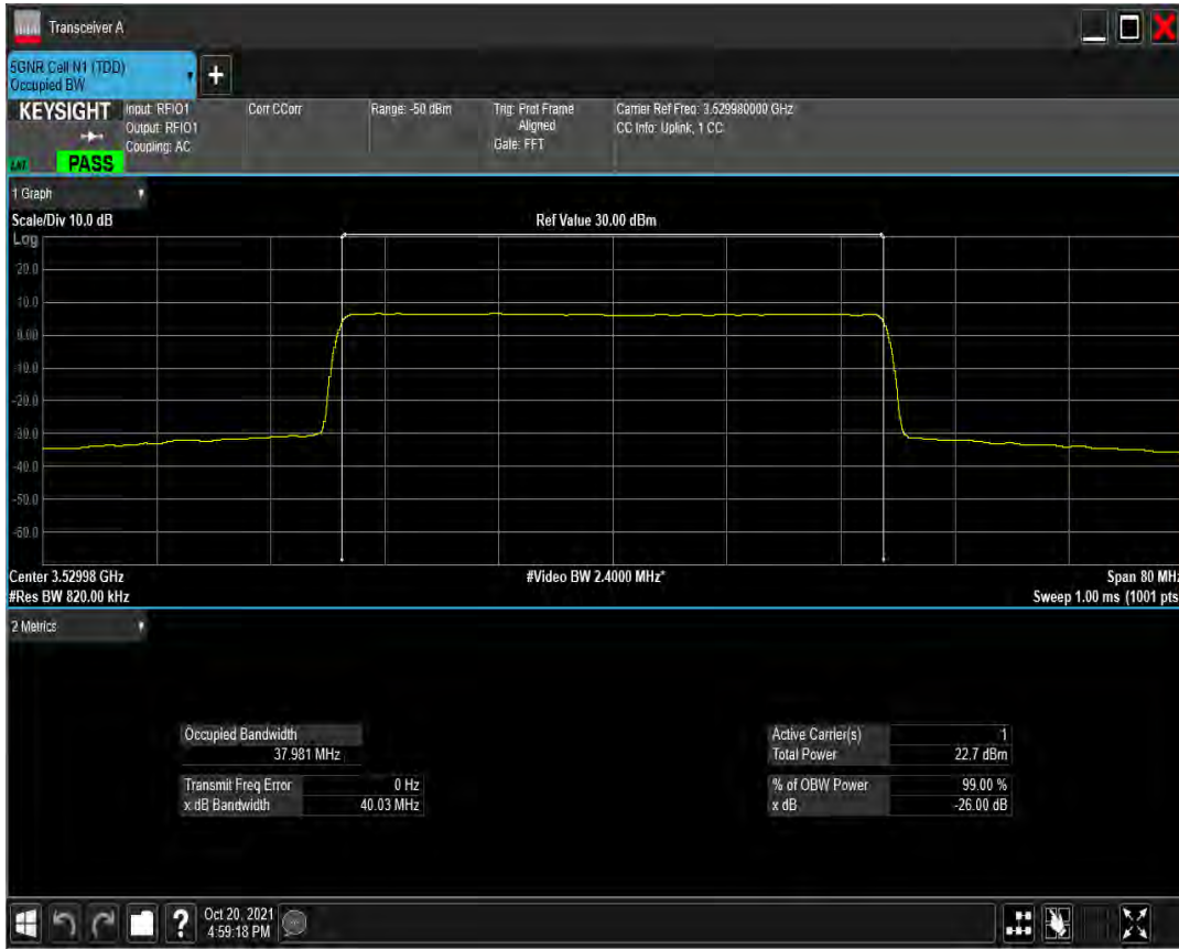
n77(3450-3550) SCS=30kHz CP_QAM64 BW=40MHz Channel=635332 RB=106@0
