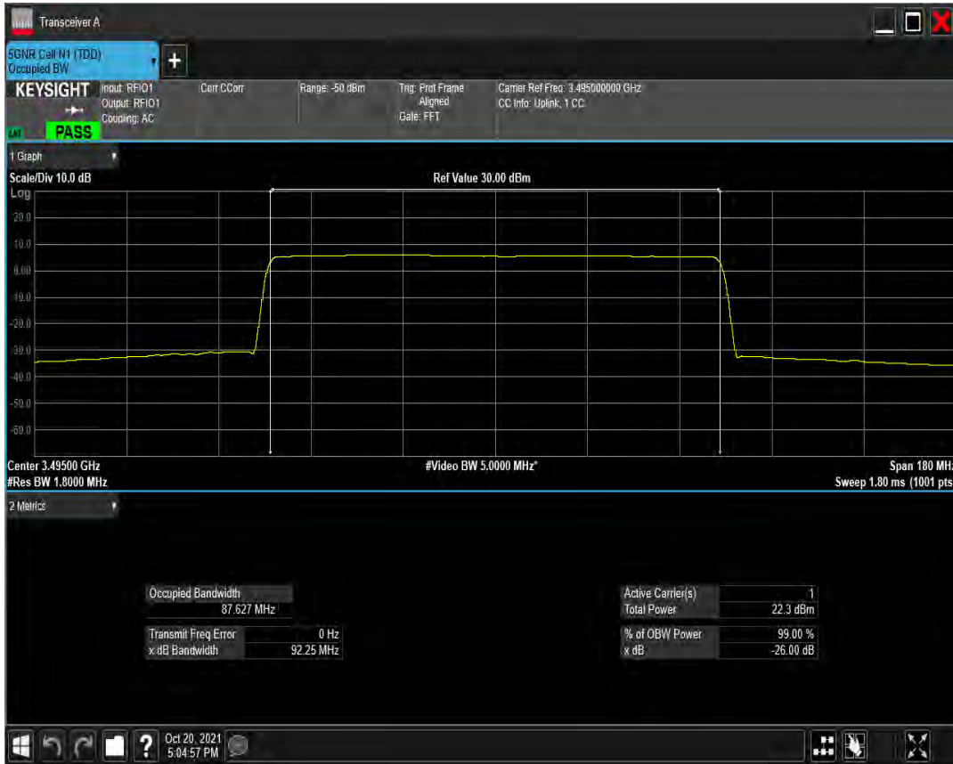
n77(3450-3550) SCS=30kHz CP_QAM256 BW=90MHz Channel=633000 RB=245@0
