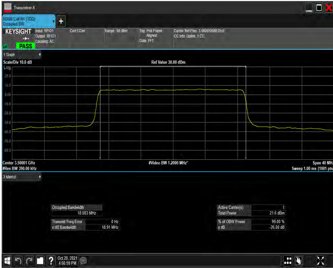
n77(3450-3550) SCS=30kHz CP_QPSK BW=20MHz Channel=633334 RB=51 @0
