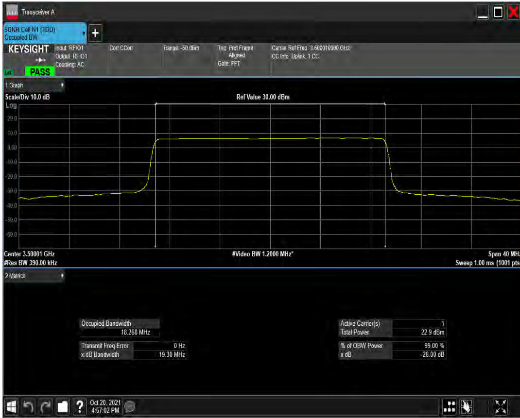
n77(3450-3550) SCS=30kHz CP_QAM16 BW=20MHz Channel=633334 RB=51@0
