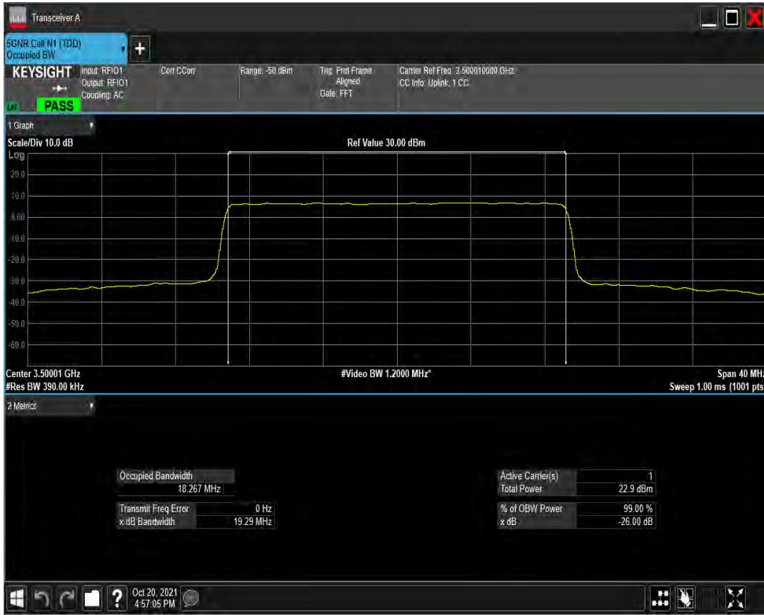
n77(3450-3550) SCS=30kHz CP_QAM64 BW=20MHz Channel=633334 RB=51 @0
