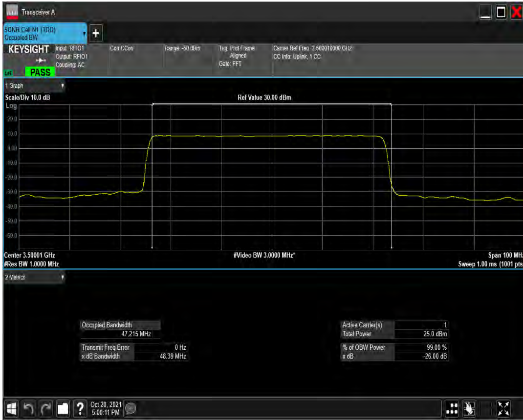
n77(3450-3550) SCS=30kHz DFT_QAM16 BW=50MHz Channel=633334 RB=128@0
