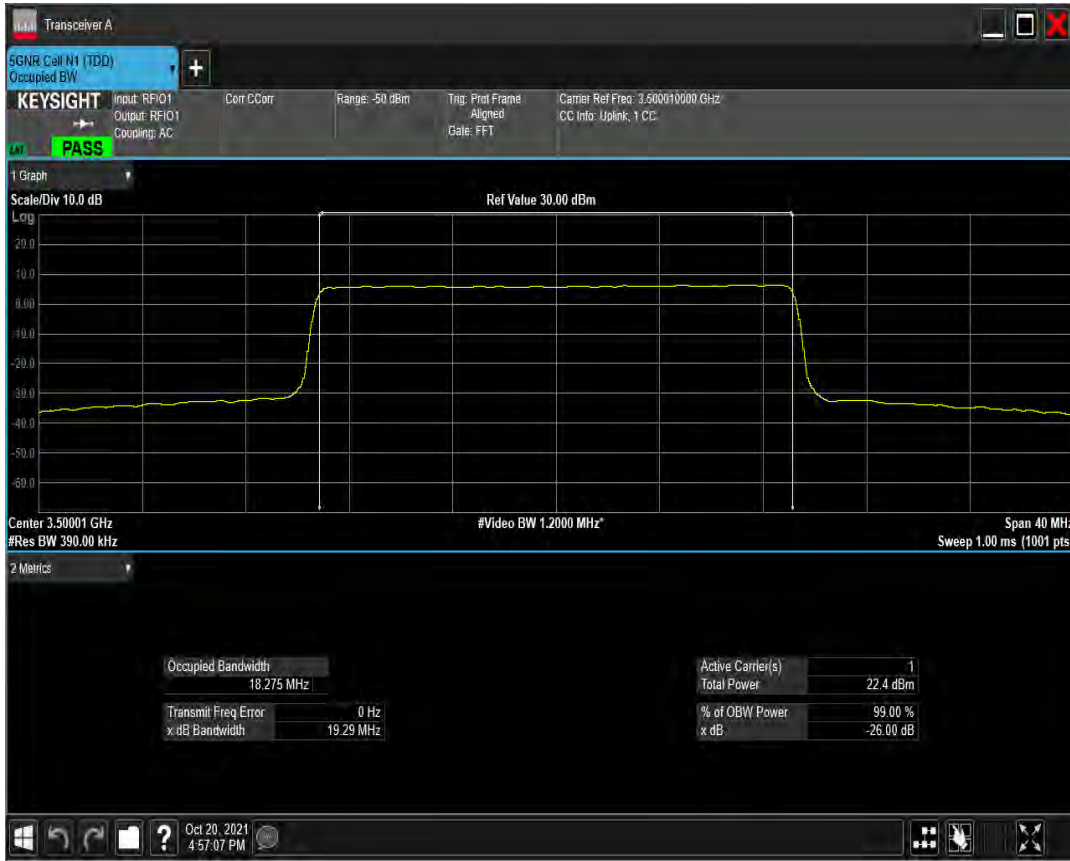
n77(3450-3550) SCS=30kHz CP_QAM256 BW=20MHz Channel=633334 RB=51@0
