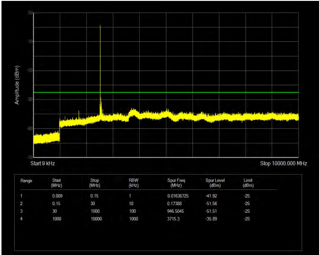
n41(2535-2655) SCS=30kHz DFT_QPSK BW=50MHz Channel=512004 RB=1@132
