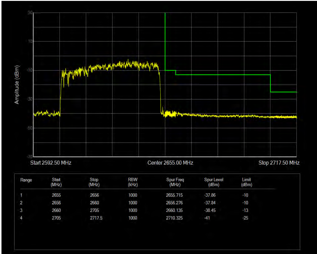
n41(2535-2655) SCS=30kHz DFT_QPSK BW=50MHz Channel=525996 RB=1 @ 132
