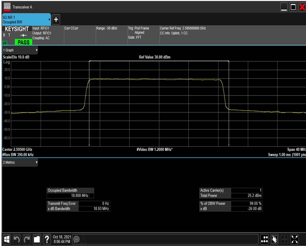
n41(2535-2655) SCS=15kHz DFT_QAM16 BW=20MHz Channel=519000 RB=100@0
