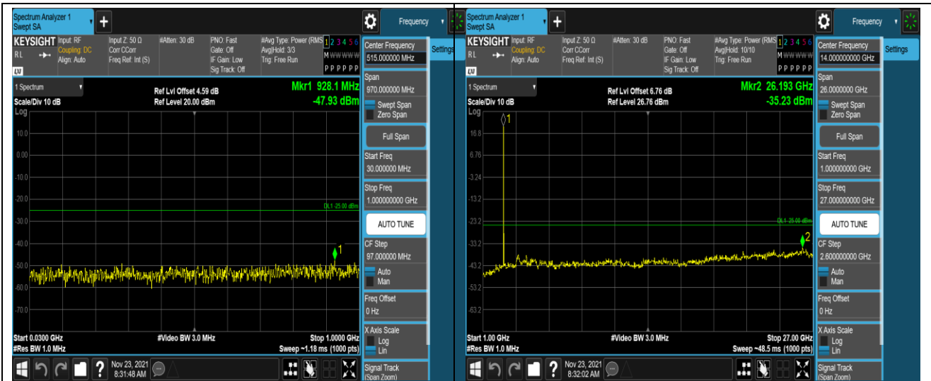
Band38-5MHz-QPSK-38225-1RB#0-Range1:30~1000MHz
