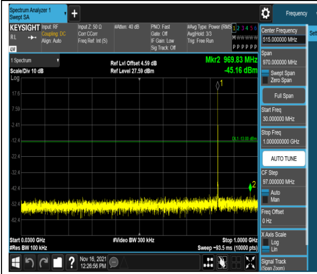
Band5-1.4MHz-16QAM-20525-1RB#0-Range1:30~1000MHz
