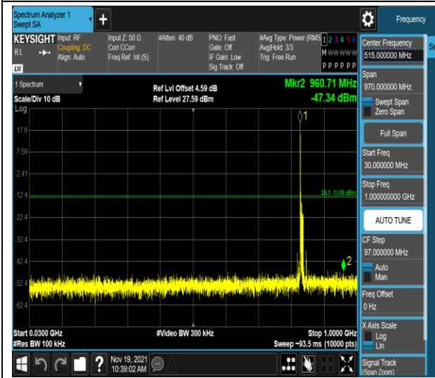
Band5-10MHz-16QAM-20450-1RB#0-Range1:30~1000MHz
