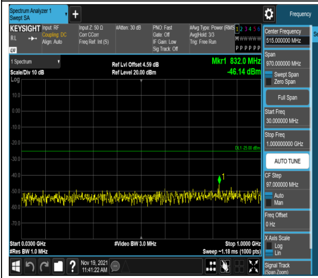
Band7-20MHz-QPSK-21100-1RB#0-Range1:30~1000MHz
