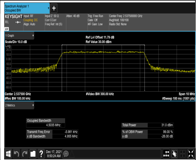
Band41-5MHz-16QAM-40065-25RB#0
