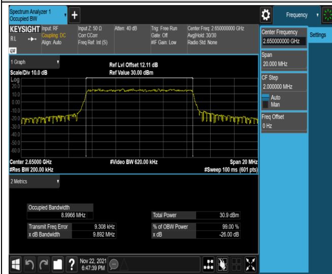
Band41-10MHz-QPSK-41190-50RB#0
