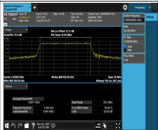
Band41-10MHz-16QAM-41190-50RB#0
