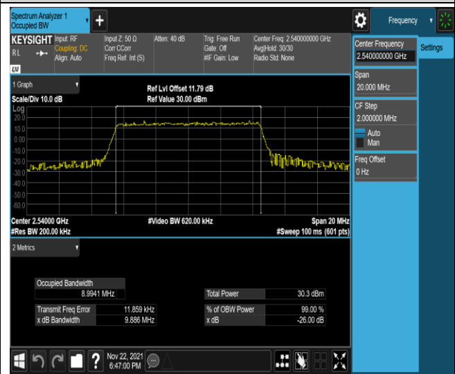
Band41-10MHz-16QAM-40090-50RB#0
