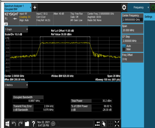
Band41-10MHz-16QAM-40640-50RB#0
