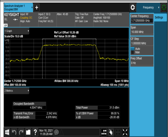
Band4-5MHz-16QAM-19975-25RB#0
