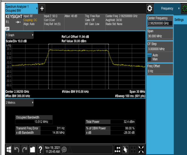
Band7-15MHz-QPSK-21375-75RB#0
