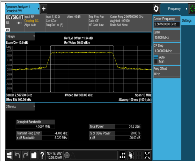
Band7-5MHz-QPSK-21425-25RB#0
