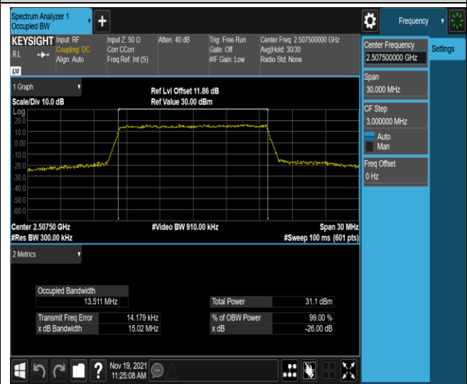
Band7-15MHz-16QAM-20825-75RB#0
