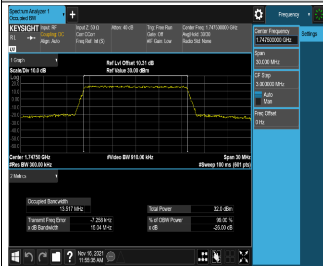
Band4-15MHz-QPSK-20325-75RB#0
