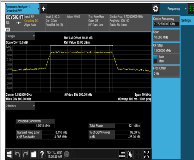
Band4-5MHz-QPSK-20375-25RB#0
