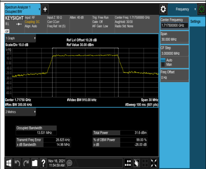
Band4-15MHz-16QAM-20025-75RB#0
