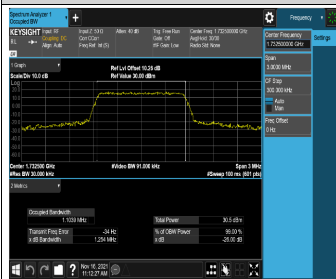
Band4-1.4MHz-16QAM-20175-6RB#0
