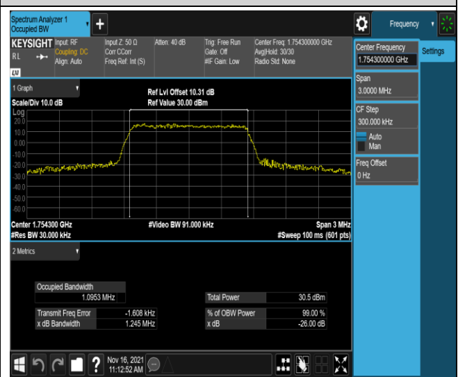
Band4-1.4MHz-16QAM-20393-6RB#0
