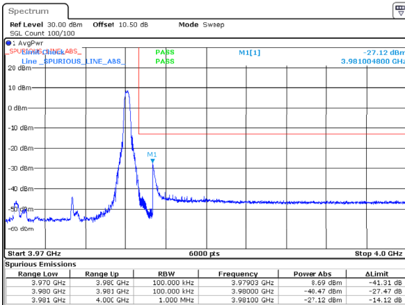
n77_3_10MHz_30kHz_3975MHz_DFT-s-OFDM QPSK_RB1@23 -27.124MHz
