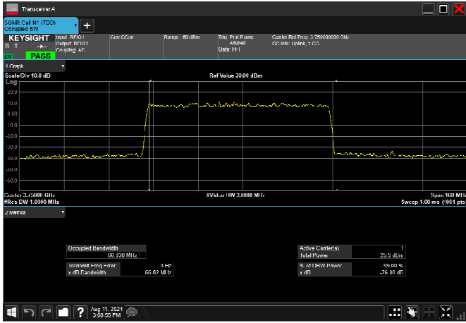
n78_3_70MHz_30kHz_3750MHz_DFT-s-OFDM 16 QAM_RB180@0 66.612MHz
