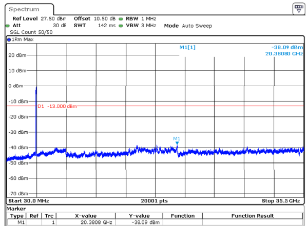
n77_1_80MHz_30kHz_3500MHz_DFT-s-OFDM QPSK_RB216@0 -38.09dBm
