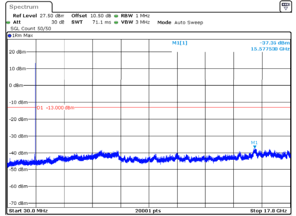
n66_40MHz_15kHz_1745MHz_DFT-s-OFDM QPSK_RB1@215 -37.35dBm
