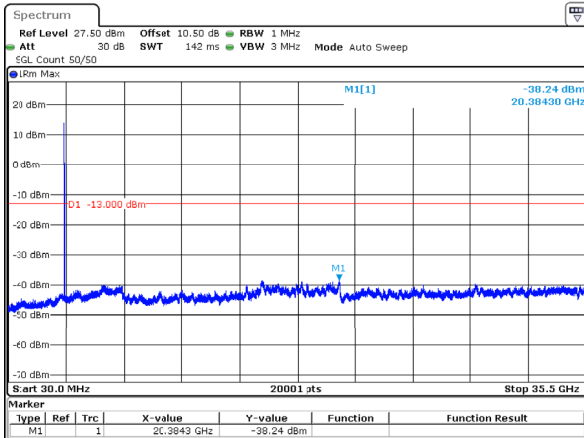
n77_1_15MHz_30kHz_3457.5MHz_DFT-s-OFDM QPSK_RB1@37 -38.24dBm
