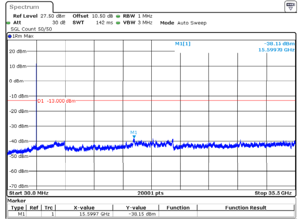
n77_1_100MHz_30kHz_3500MHz_DFT-s-OFDM QPSK_RB1@272 -38.15dBm
