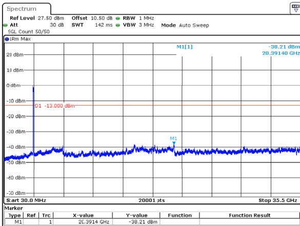
n77_1_80MHz_30kHz_3490MHz_DFT-s-OFDM QPSK_RB216@0 -38.21dBm
