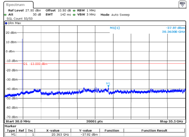
n77_1_15MHz_30kHz_3457.5MHz_DFT-s-OFDM QPSK_RB1@0 -37.92dBm
