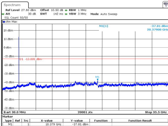
n77_1_10MHz_30kHz_3500MHz_DFT-s-OFDM QPSK_RB1@23 -37.81dBm
