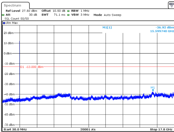
n66_40MHz_15kHz_1760MHz_DFT-s-OFDM QPSK_RB1@215 -36.92dBm
