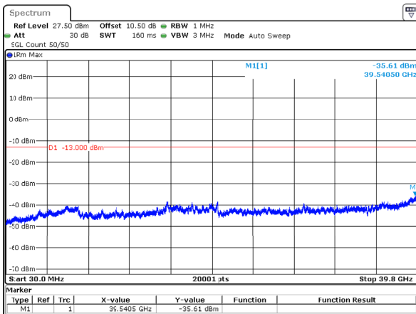
n77_3_15MHz_30kHz_3840MHz_DFT-s-OFDM QPSK_RB1@37 -35.61dBm
