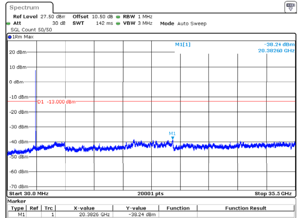
n77_1_15MHz_30kHz_3457.5MHz_DFT-s-OFDM QPSK_RB36@0 -38.24dBm
