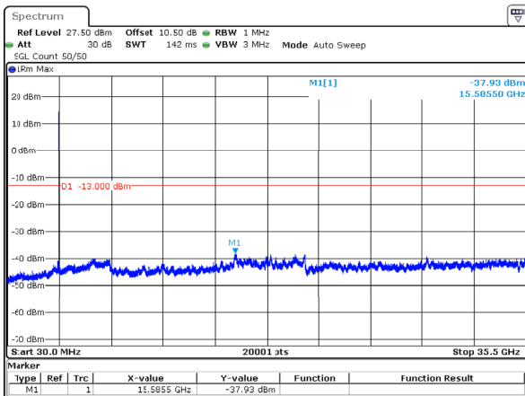
n77_1_80MHz_30kHz_3500MHz_DFT-s-OFDM QPSK_RB1@216 -37.93dBm
