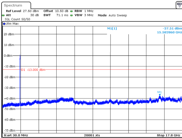
n66_40MHz_15kHz_1745MHz_DFT-s-OFDM QPSK_RB216@0 -37.51dBm
