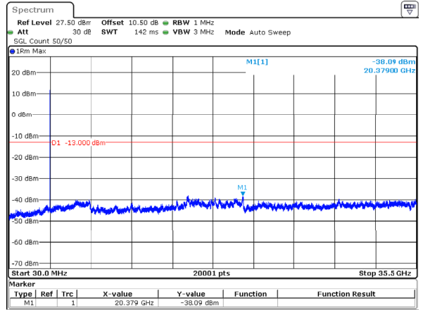
n77_1_20MHz_30kHz_3540MHz_DFT-s-OFDM QPSK_RB1@50 -38.09dBm
