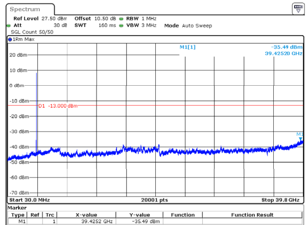
n77_3_15MHz_30kHz_3840MHz_DFT-s-OFDM QPSK_RB36@0 -35.49dBm
