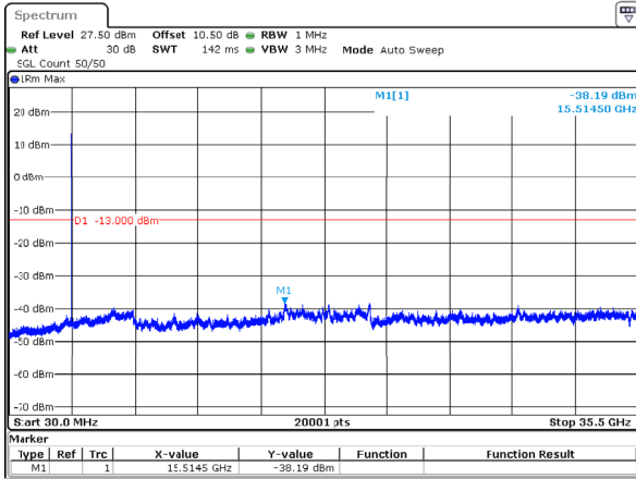
n77_1_10MHz_30kHz_3545MHz_DFT-s-OFDM QPSK_RB1@0 -38.19dBm
