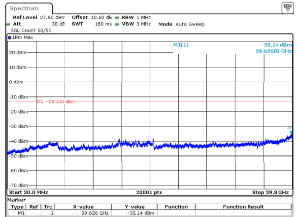
n77_3_15MHz_30kHz_3840MHz_DFT-s-OFDM QPSK_RB1@0 -35.14dBm
