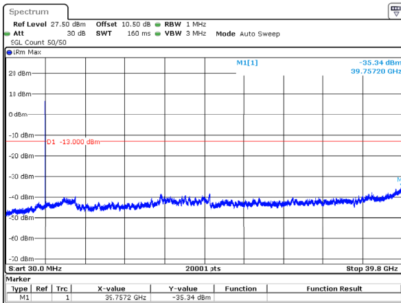
n77_3_15MHz_30kHz_3972.5MHz_DFT-s-OFDM QPSK_RB36@0 -35.34dBm
