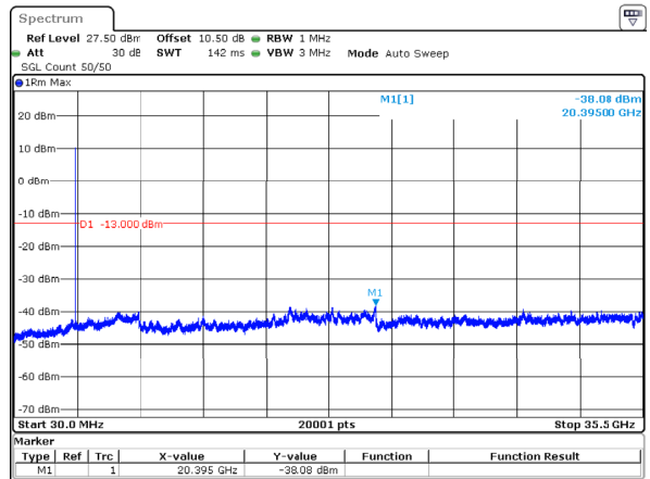
n77_1_80MHz_30kHz_3500MHz_DFT-s-OFDM QPSK_RB1@0 -38.08dBm
