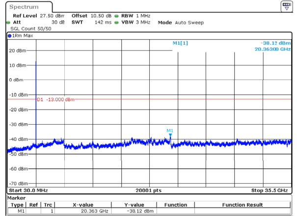
n77_1_10MHz_30kHz_3545MHz_DFT-s-OFDM QPSK_RB1@23 -38.12dBm
