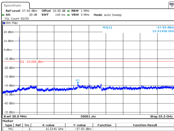
n77_1_30MHz_30kHz_3465MHz_DFT-s-OFDM QPSK_RB1@77 -37.93dBm
