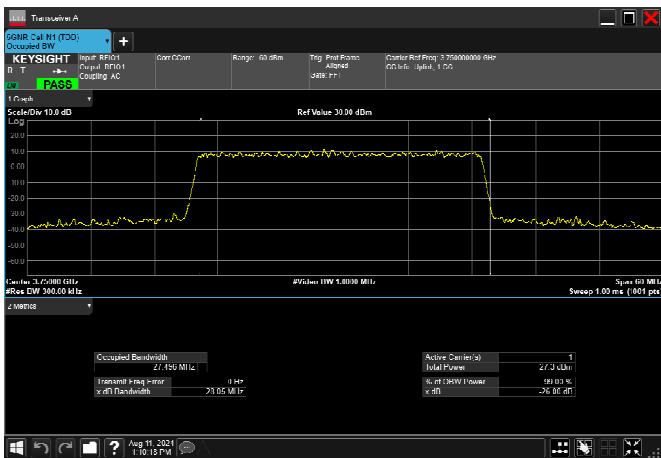
n78_3_30MHz_30kHz_3750MHz_DFT-s-OFDM 256 QAM_RB75@0 27.496MHz
