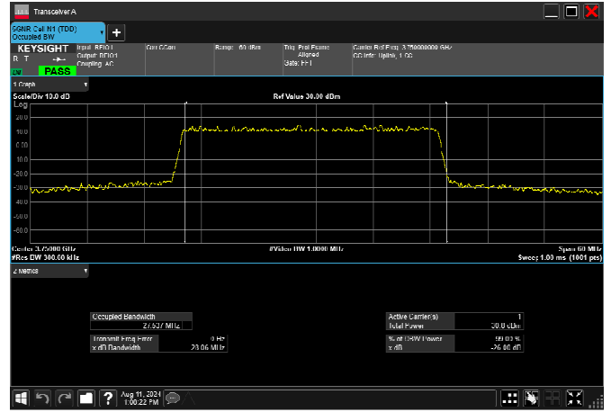
n78_3_30MHz_30kHz_3750MHz_DFT-s-OFDM 64 QAM_RB75@0 27.633MHz
