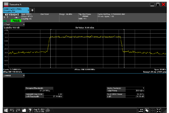
n78_3_40MHz_30kHz_3750MHz_DFT-s-OFDM 16 QAM_RB100@0 37.354MHz
