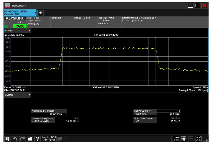
n78_3_40MHz_30kHz_3750MHz_CP-OFDM 256 QAM_RB106@0 37.680MHz
