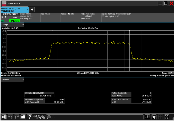
n78_3_30MHz_30kHz_3750MHz_CP-OFDM 256 QAM_RB78@0 27.757MHz
