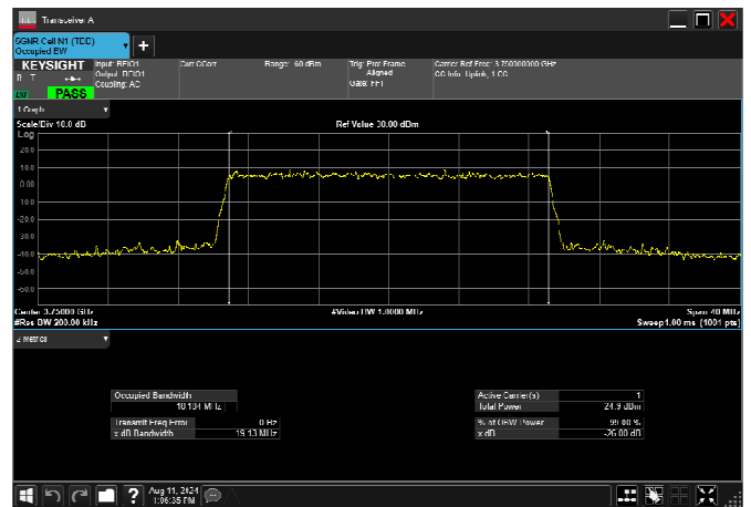
n78_3_20MHz_30kHz_3750MHz_CP-OFDM 256 QAM_RB51@0 18.184MHz
