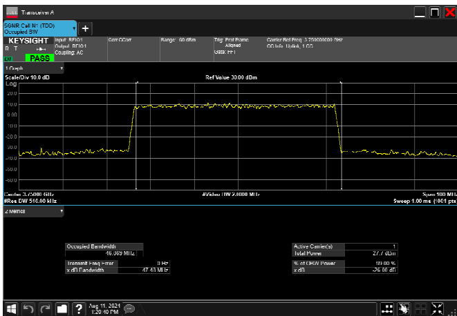
n78_3_50MHz_30kHz_3750MHz_DFT-s-OFDM 256 QAM_RB128@0 46.869MHz
