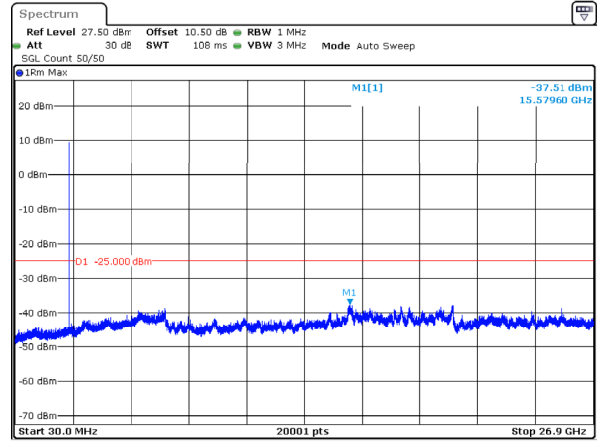
n41_15MHz_30kHz_2503.5MHz_DFT-s-OFDM QPSK_RB1@37 -37.51dBm
