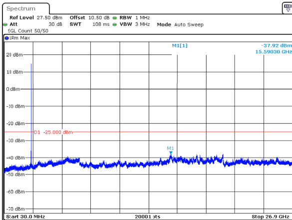
n41_50MHz_30kHz_2521.02MHz_DFT-s-OFDM QPSK_RB1@132 -37.92dBm
