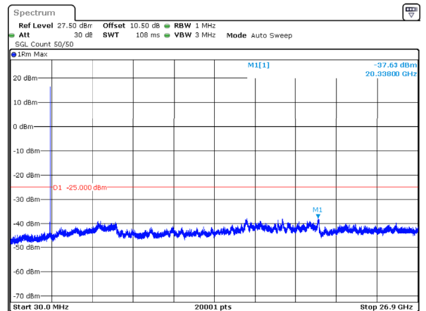
n41_50MHz_30kHz_2592.99MHz_DFT-s-OFDM QPSK_RB1@132 -37.63dBm
