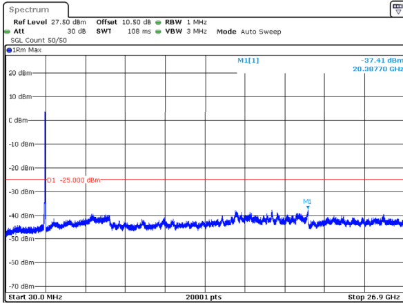
n41_50MHz_30kHz_2664.99MHz_DFT-s-OFDM QPSK_RB128@0 -37.41dBm
