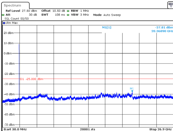
n41_30MHz_30kHz_2592.99MHz_DFT-s-OFDM QPSK_RB1@77 -37.81dBm
