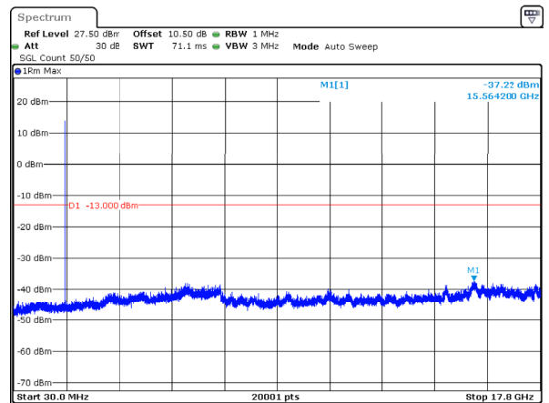
n66_10MHz_15kHz_1745MHz_DFT-s-OFDM QPSK_RB1@0 -37.22dBm
