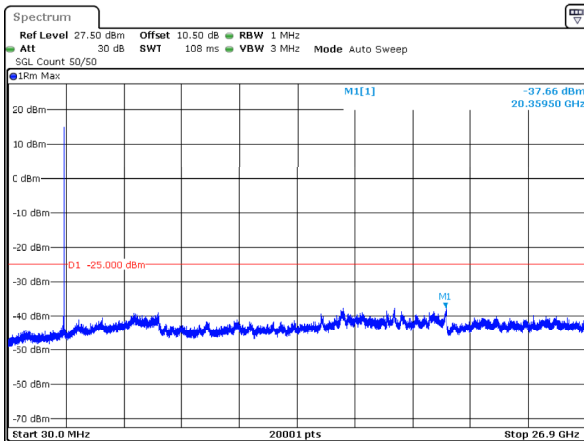
n41_40MHz_30kHz_2592.99MHz_DFT-s-OFDM QPSK_RB1@105 -37.66dBm
