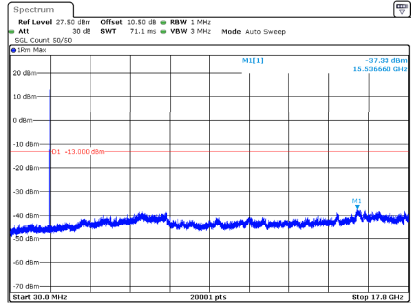
n66_15MHz_15kHz_1745MHz_DFT-s-OFDM QPSK_RB1@78 -37.33dBm
