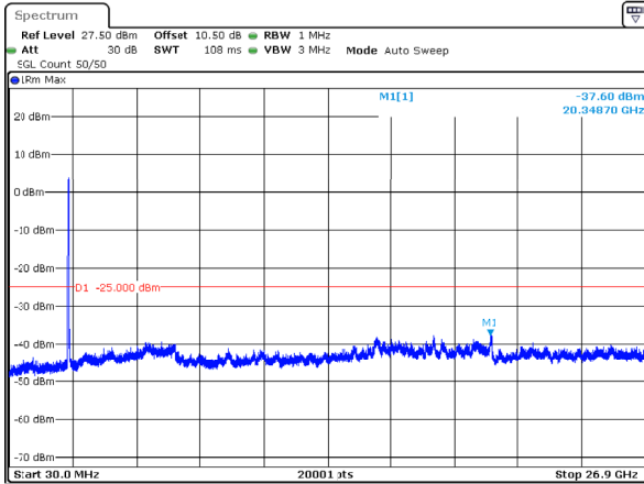
n41_50MHz_30kHz_2521.02MHz_DFT-s-OFDM QPSK_RB128@0 -37.60dBm
