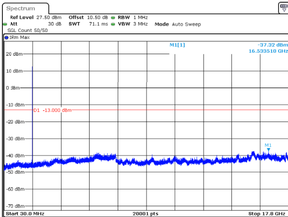
n66_20MHz_15kHz_1770MHz_DFT-s-OFDM QPSK_RB1@105 -37.32dBm
