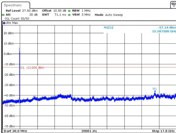
n66_15MHz_15kHz_1745MHz_DFT-s-OFDM QPSK_RB75@0 -37.14dBm
