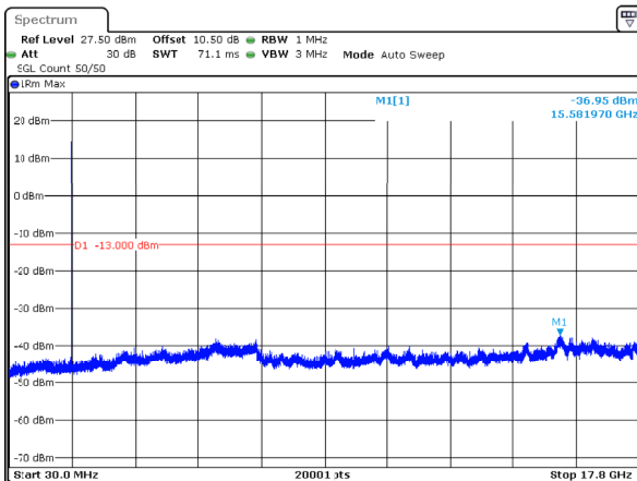
n66_15MHz_15kHz_1772.5MHz_DFT-s-OFDM QPSK_RB1@78 -36.95dBm
