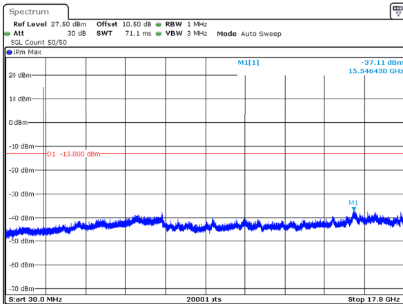
n66_5MHz_15kHz_1712.5MHz_DFT-s-OFDM QPSK_RB1@24 -37.11dBm
