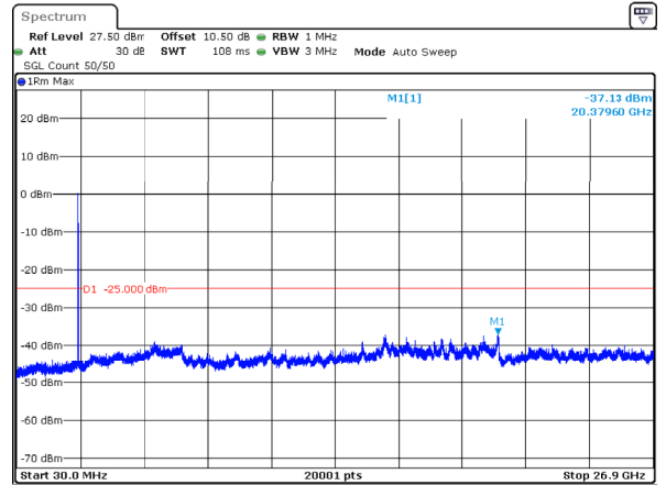
n41_15MHz_30kHz_2592.99MHz_DFT-s-OFDM QPSK_RB36@0 -37.13dBm
