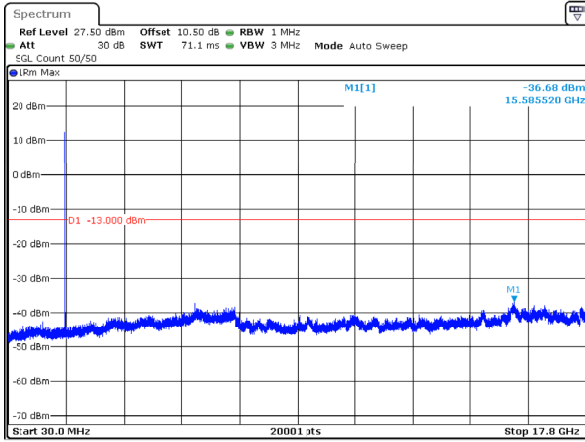
n66_10MHz_15kHz_1775MHz_DFT-s-OFDM QPSK_RB1@0 -36.68dBm
