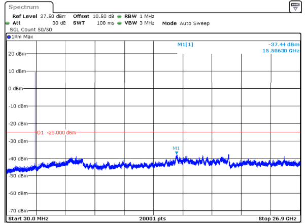
n41_20MHz_30kHz_2592.99MHz_DFT-s-OFDM QPSK_RB1@50 -37.44dBm
