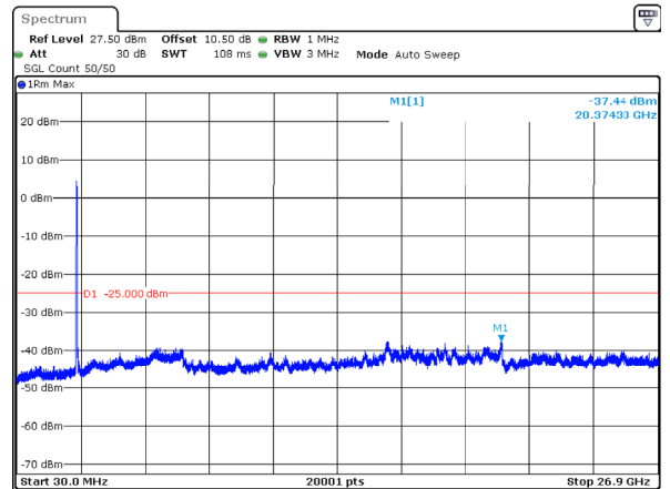
n41_40MHz_30kHz_2516.01MHz_DFT-s-OFDM QPSK_RB100@0 -37.44dBm
