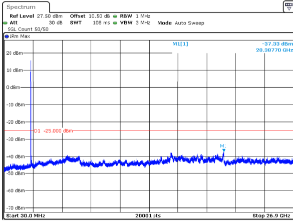
n41_100MHz_30kHz_2546.01MHz_DFT-s-OFDM QPSK_RB1@0 -37.33dBm
