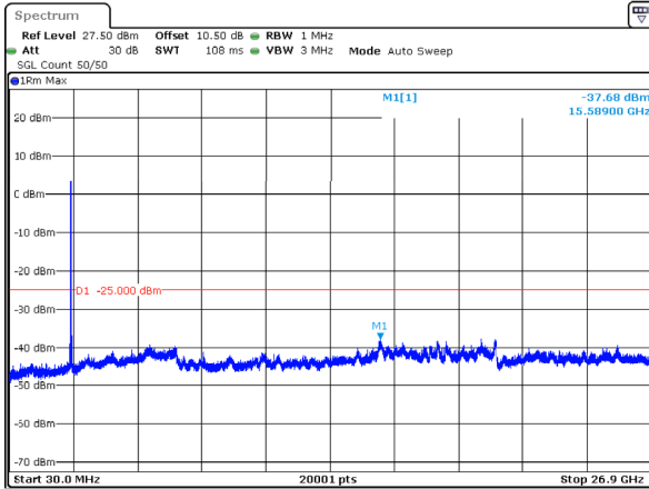
n41_40MHz_30kHz_2592.99MHz_DFT-s-OFDM QPSK_RB100@0 -37.68dBm
