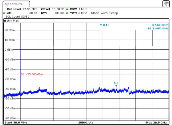
n41_90MHz_30kHz_2592.99MHz_DFT-s-OFDM QPSK_RB1@244 -37.62dBm
