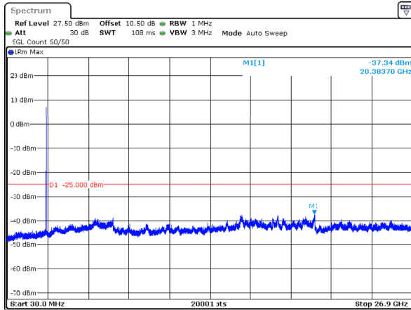
n41_15MHz_30kHz_2592.99MHz_DFT-s-OFDM QPSK_RB1@37 -37.34dBm
