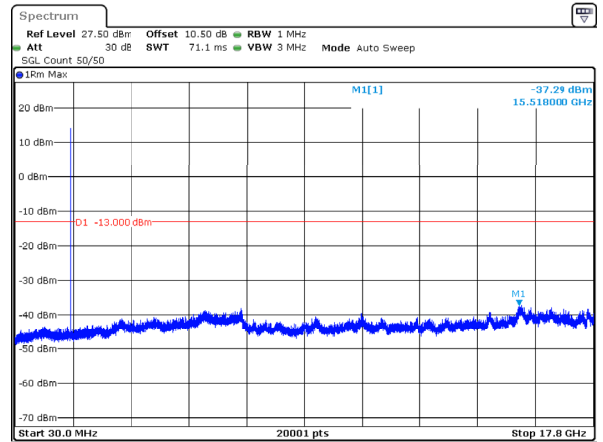
n66_10MHz_15kHz_1715MHz_DFT-s-OFDM QPSK_RB1@51 -37.29dBm
