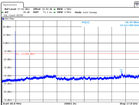
n66_10MHz_15kHz_1745MHz_DFT-s-OFDM QPSK_RB1@51 -36.33dBm
