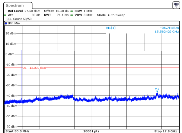
n66_15MHz_15kHz_1772.5MHz_DFT-s-OFDM QPSK_RB75@0 -36.78dBm
