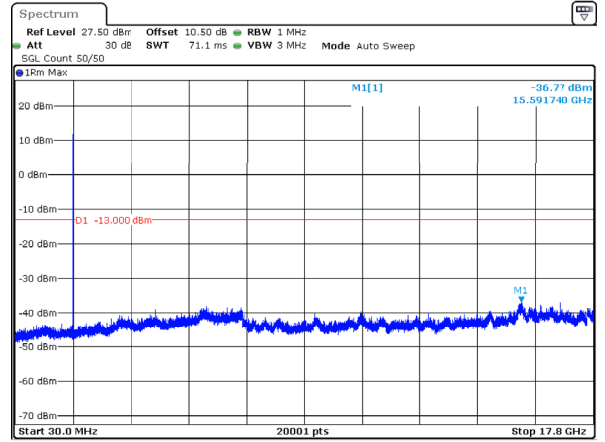
n66_10MHz_15kHz_1775MHz_DFT-s-OFDM QPSK_RB1@51 -36.77dBm
