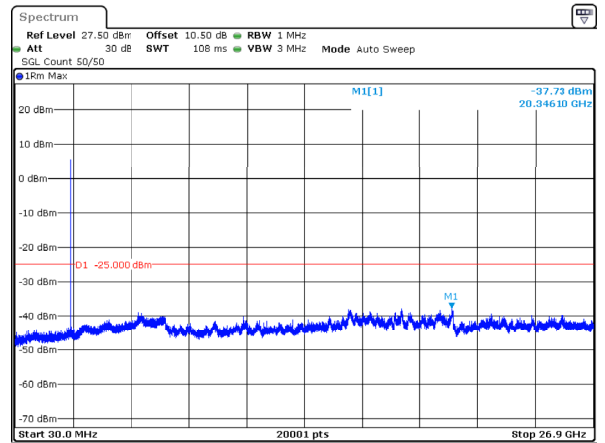
n41_15MHz_30kHz_2592.99MHz_DFT-s-OFDM QPSK_RB1@0 -37.73dBm
