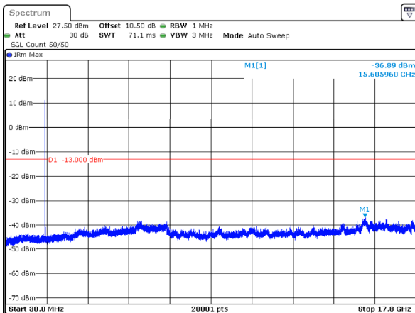
n66_25MHz_15kHz_1722.5MHz_DFT-s-OFDM QPSK_RB1@0 -36.89dBm
