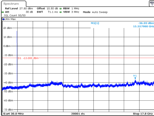
n66_15MHz_15kHz_1745MHz_DFT-s-OFDM QPSK_RB1@0 -36.03dBm
