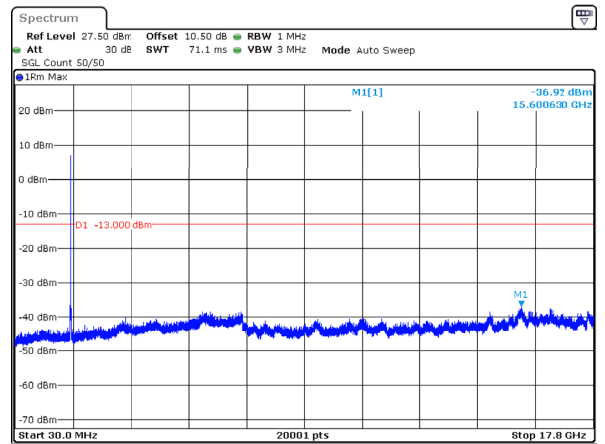
n66_15MHz_15kHz_1717.5MHz_DFT-s-OFDM QPSK_RB75@0 -36.92dBm
