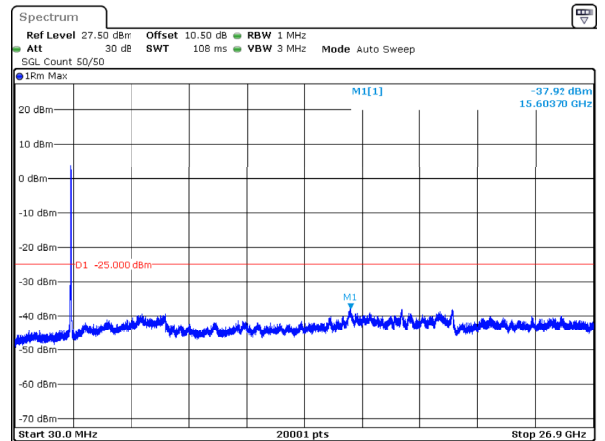
n41_50MHz_30kHz_2592.99MHz_DFT-s-OFDM QPSK_RB128@0 -37.92dBm
