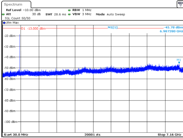
n12_15MHz_15kHz_706.5MHz_DFT-s-OFDM QPSK_RB1@0 -45.78dBm
