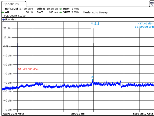
n38_30MHz_30kHz_2605MHz_DFT-s-OFDM QPSK_RB1@77 -37.40dBm
