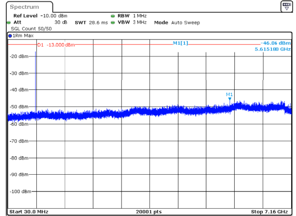
n12_5MHz_15kHz_713.5MHz_DFT-s-OFDM QPSK_RB1@24 -46.06dBm
