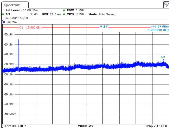
n12_15MHz_15kHz_706.5MHz_DFT-s-OFDM QPSK_RB75@0 -46.37dBm
