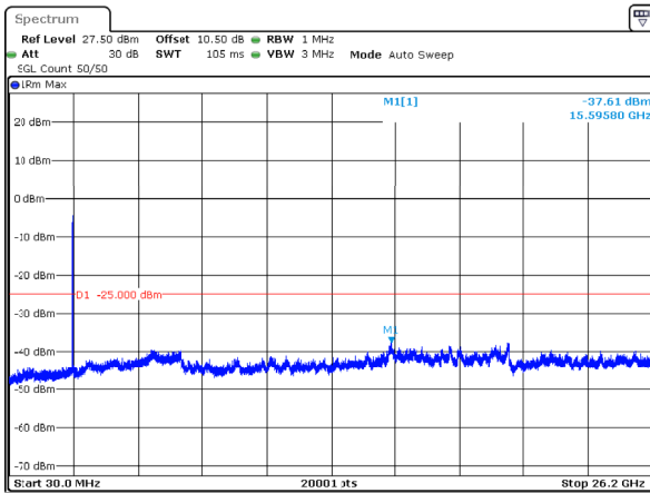
n38_30MHz_30kHz_2595MHz_DFT-s-OFDM QPSK_RB75@0 -37.61dBm
