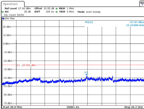
n38_40MHz_30kHz_2600MHz_DFT-s-OFDM QPSK_RB1@105 -37.07dBm
