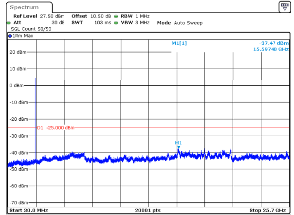
n7_5MHz_15kHz_2502.5MHz_DFT-s-OFDM QPSK_RB1@24 -37.47dBm
