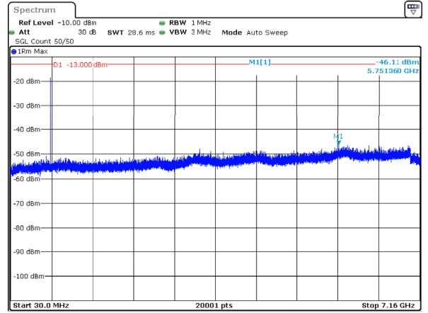
n12_15MHz_15kHz_706.5MHz_DFT-s-OFDM QPSK_RB1@78 -46.11dBm
