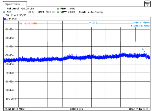
n12_5MHz_15kHz_707.5MHz_DFT-s-OFDM QPSK_RB1@0 -46.47dBm
