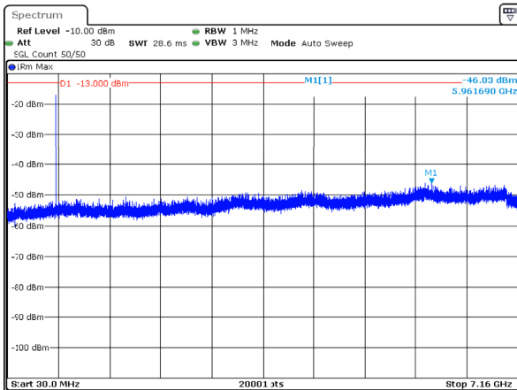
n12_5MHz_15kHz_707.5MHz_DFT-s-OFDM QPSK_RB1@24 -46.03dBm
