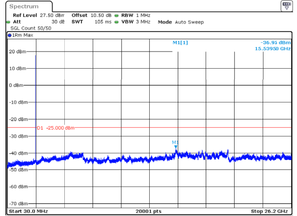
n38_5MHz_15kHz_2572.5MHz_DFT-s-OFDM QPSK_RB1@24 -36.95dBm
