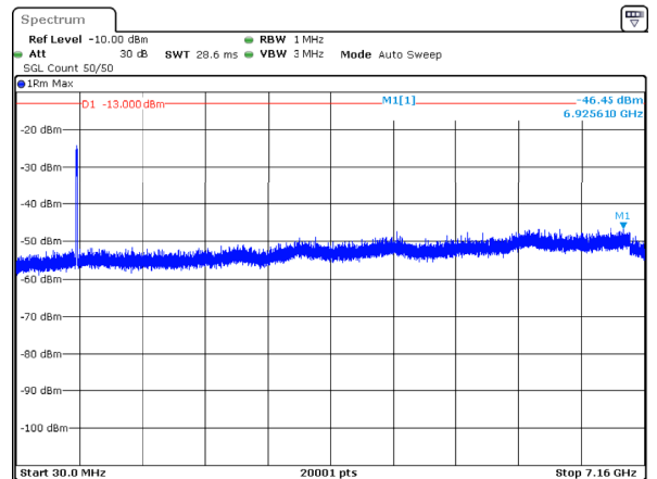
n12_15MHz_15kHz_707.5MHz_DFT-s-OFDM QPSK_RB75@0 -46.45dBm
