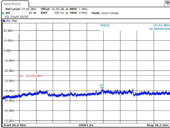
n38_5MHz_15kHz_2572.5MHz_DFT-s-OFDM QPSK_RB1@0 -37.61dBm
