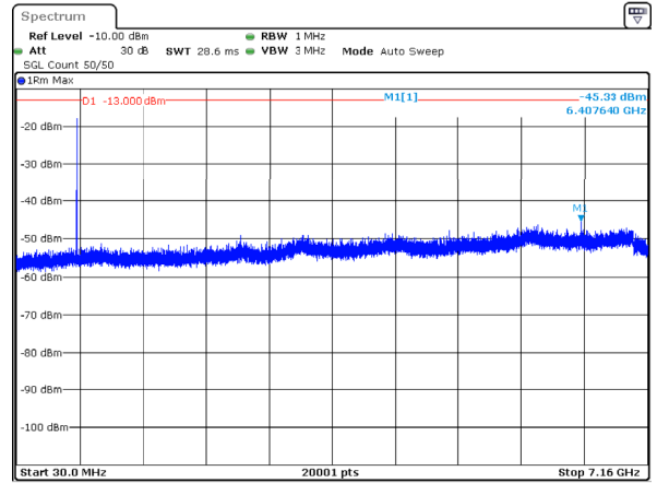
n12_5MHz_15kHz_701.5MHz_DFT-s-OFDM QPSK_RB1@24 -45.33dBm
