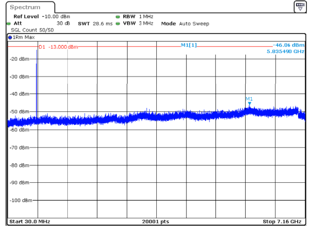
n12_10MHz_15kHz_707.5MHz_DFT-s-OFDM QPSK_RB1@51 -46.06dBm
