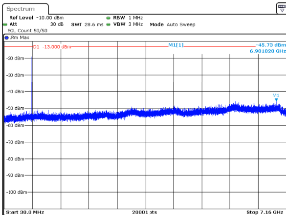
n12_15MHz_15kHz_707.5MHz_DFT-s-OFDM QPSK_RB1@78 -45.73dBm
