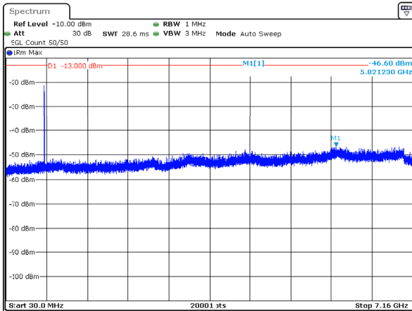
n12_5MHz_15kHz_701.5MHz_DFT-s-OFDM QPSK_RB25@0 -46.60dBm
