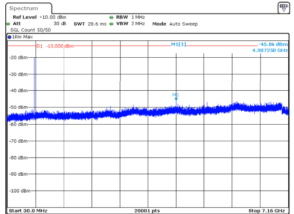
n12_10MHz_15kHz_711MHz_DFT-s-OFDM QPSK_RB1@0 -45.86dBm
