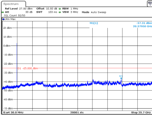
n7_5MHz_15kHz_2502.5MHz_DFT-s-OFDM QPSK_RB1@0 -37.31dBm
