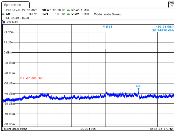
n7_5MHz_15kHz_2502.5MHz_DFT-s-OFDM QPSK_RB25@0 -36.51dBm
