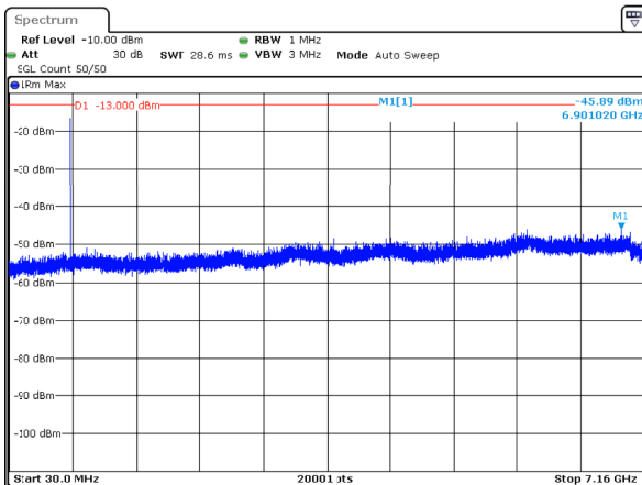
n12_10MHz_15kHz_711MHz_DFT-s-OFDM QPSK_RB1@51 -45.89dBm
