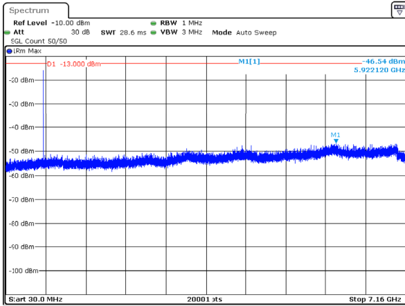
n12_5MHz_15kHz_701.5MHz_DFT-s-OFDM QPSK_RB1@0 -46.54dBm
