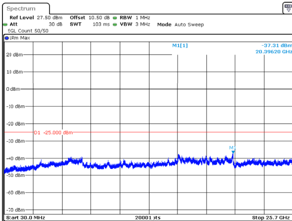
n7_5MHz_15kHz_2535MHz_DFT-s-OFDM QPSK_RB1@24 -37.31dBm
