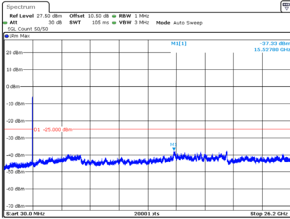
n38_40MHz_30kHz_2600MHz_DFT-s-OFDM QPSK_RB100@0 -37.33dBm
