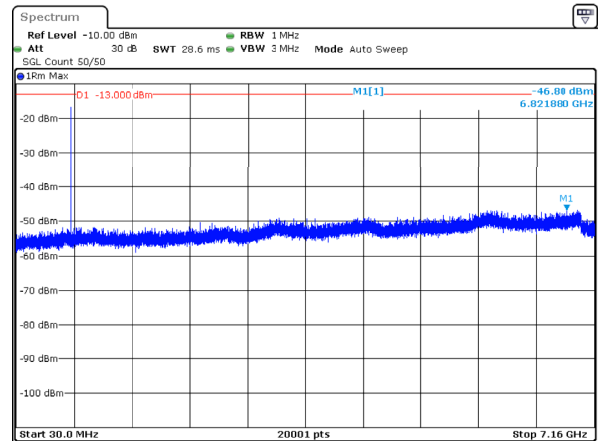
n12_10MHz_15kHz_704MHz_DFT-s-OFDM QPSK_RB1@0 -46.80dBm
