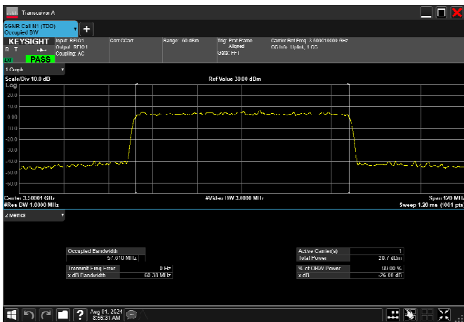
n78_1_60MHz_30kHz_3500MHz_DFT-s-OFDM 256 QAM_RB162@0 57.610MHz
