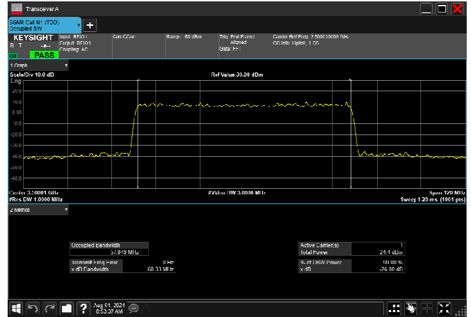
n78_1_60MHz_30kHz_3500MHz_DFT-s-OFDM 64 QAM_RB162@0 57.915MHz
