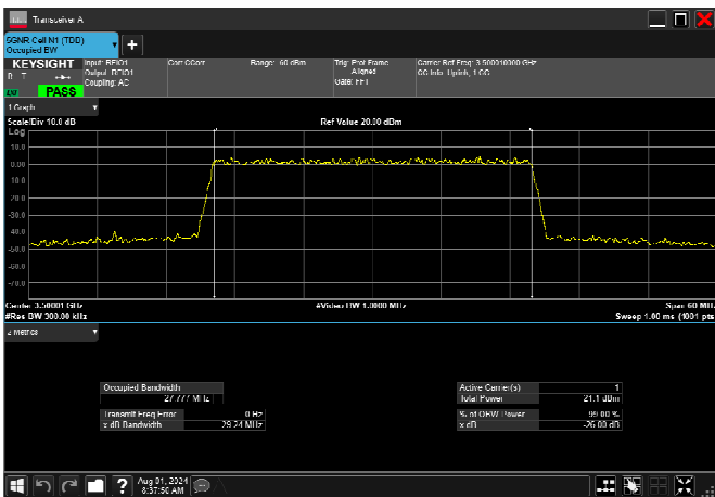
n78_1_30MHz_30kHz_3500MHz_CP-OFDM 64 QAM_RB78@0 27.777MHz
