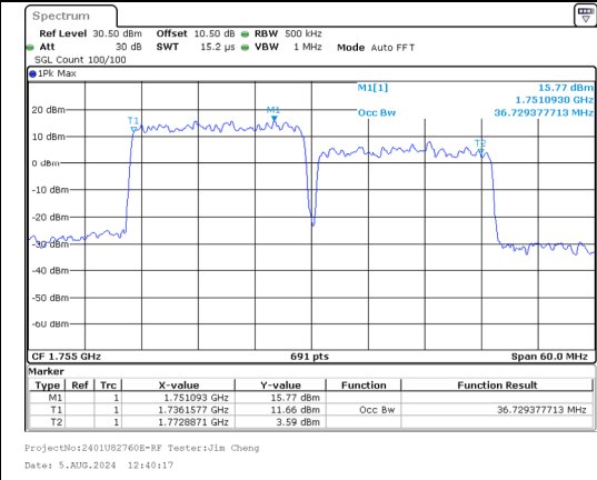
99%OBW Band 66 20MHz/1745.1/Mid QPSK 100@0 Band 66 20MHz/1764.9/Mid QPSK 100@0
