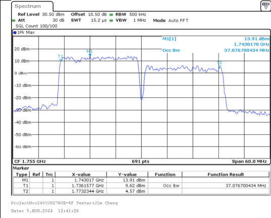
99%OBW Band 66 20MHz/1745.1/Mid 16QAM 100@0 Band 66 20MHz/1764.9/Mid 16QAM 100@0
