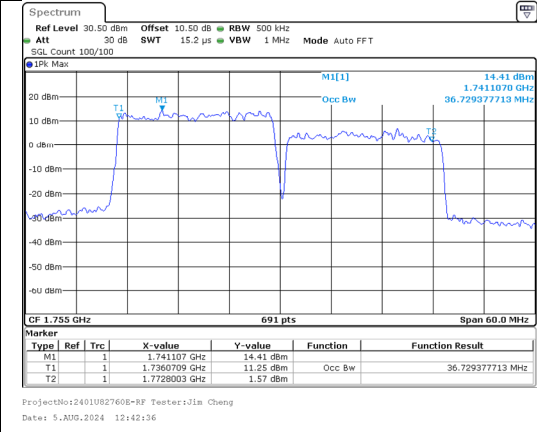
99%OBW Band 66 20MHz/1745.1/Mid 64QAM 100@0 Band 66 20MHz/1764.9/Mid 64QAM 100@0
