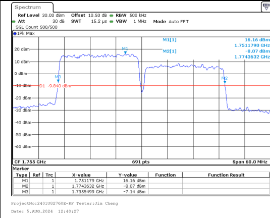
26%OBW Band 66 20MHz/1745.1/Mid QPSK 100@0 Band 66 20MHz/1764.9/Mid QPSK 100@0
