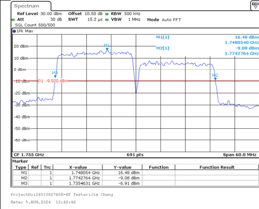
26%OBW Band 66 20MHz/1745.1/Mid 64QAM 100@0 Band 66 20MHz/1764.9/Mid 64QAM 100@0
