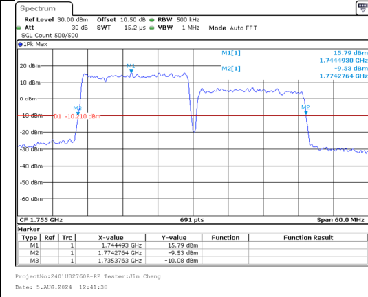
26%OBW Band 66 20MHz/1745.1/Mid 16QAM 100@0 Band 66 20MHz/1764.9/Mid 16QAM 100@0
