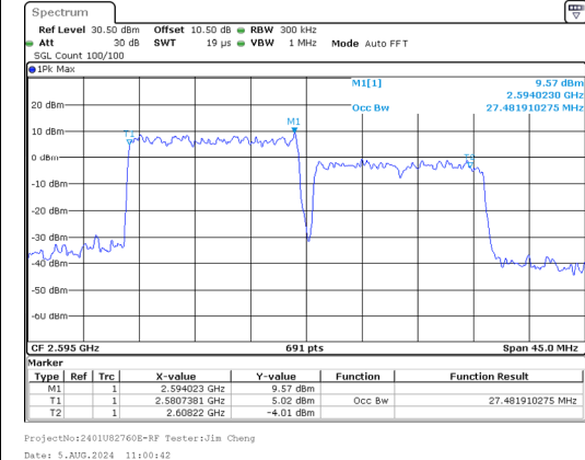
99%OBW Band 38 15MHz/2587.5/Mid 64QAM 75@0 Band 38 15MHz/2602.5/Mid 64QAM 75@0
