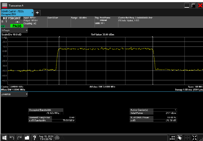
n77_3_80MHz_30kHz_3840MHz_DFT-s-OFDM QPSK_RB216@0 76.925MHz
