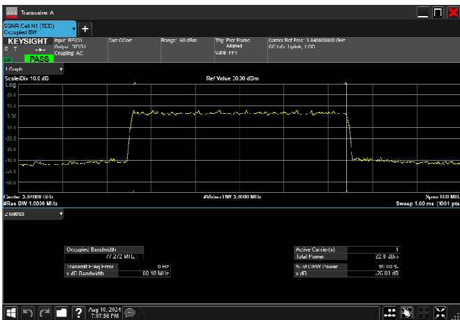
n77_3_80MHz_30kHz_3840MHz_CP-OFDM 64 QAM_RB217@0 77.272MHz
