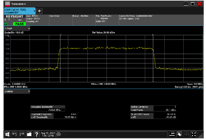
n77_3_80MHz_30kHz_3840MHz_CP-OFDM 16 QAM_RB217@0 77.139MHz
