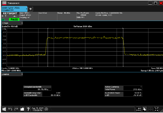
n77_3_90MHz_30kHz_3840MHz_DFT-s-OFDM 16 QAM_RB243@0 86.468MHz
