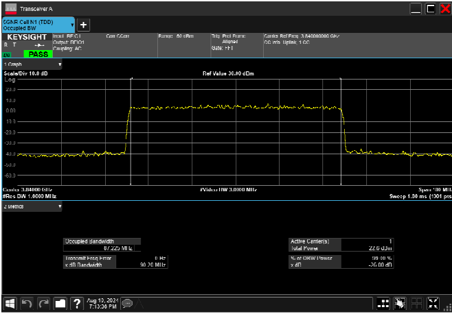
n77_3_90MHz_30kHz_3840MHz_CP-OFDM 256 QAM_RB245@0 87.193MHz
