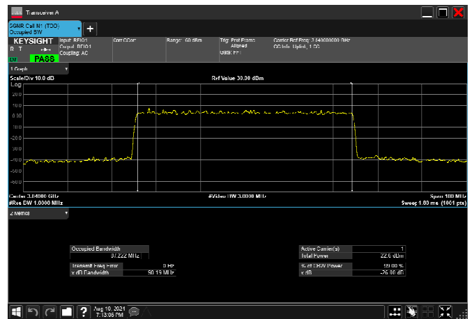
n77_3_90MHz_30kHz_3840MHz_CP-OFDM QPSK_RB245@0 87.222MHz
