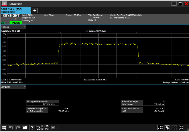
n77_3_70MHz_30kHz_3840MHz_CP-OFDM 256 QAM_RB189@0 67.297MHz
