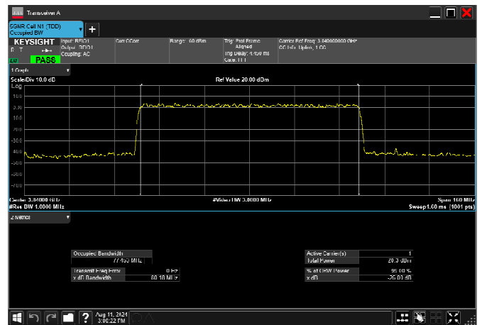
n77_3_80MHz_30kHz_3840MHz_CP-OFDM 256 QAM_RB217@0 77.453MHz
