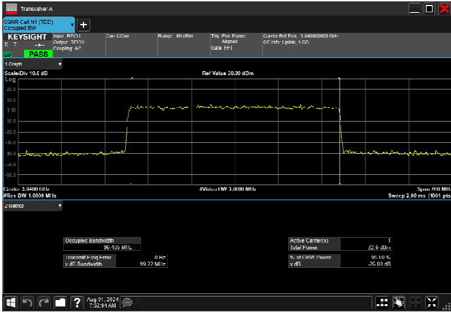
n77_3_100MHz_30kHz_3840MHz_CP-OFDM QPSK_RB273@0 97.279MHz
