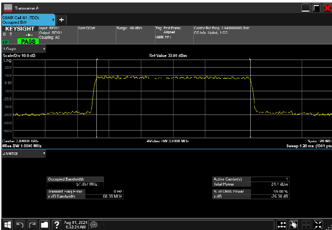
n77_3_60MHz_30kHz_3840MHz_DFT-s-OFDM QPSK_RB162@0 57.857MHz
