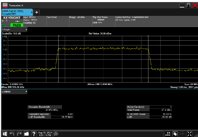
n77_3_40MHz_30kHz_3840MHz_CP-OFDM 64 QAM_RB106@0 37.812MHz
