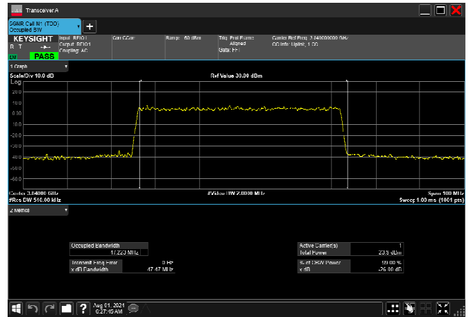
n77_3_50MHz_30kHz_3840MHz_DFT-s-OFDM 64 QAM_RB128@0 47.029MHz
