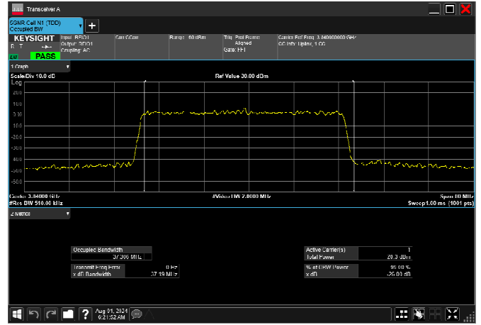
n77_3_40MHz_30kHz_3840MHz_CP-OFDM 16 QAM_RB106@0 37.775MHz
