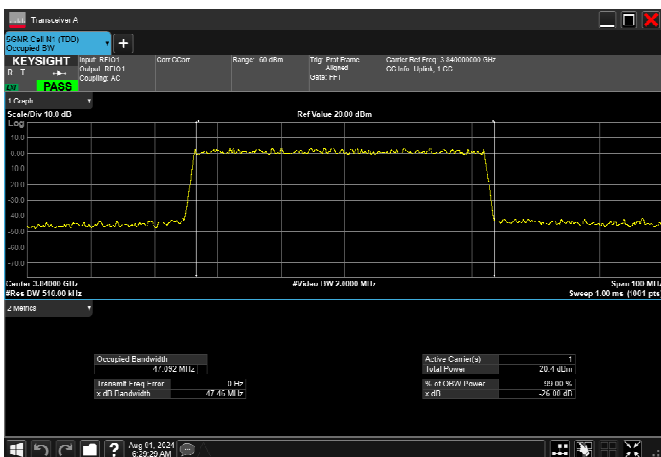
n77_3_50MHz_30kHz_3840MHz_DFT-s-OFDM 256 QAM_RB128@0 47.092MHz
