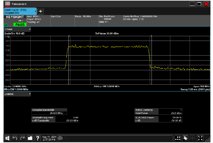
n77_3_70MHz_30kHz_3840MHz_DFT-s-OFDM 64 QAM_RB180@0 66.586MHz
