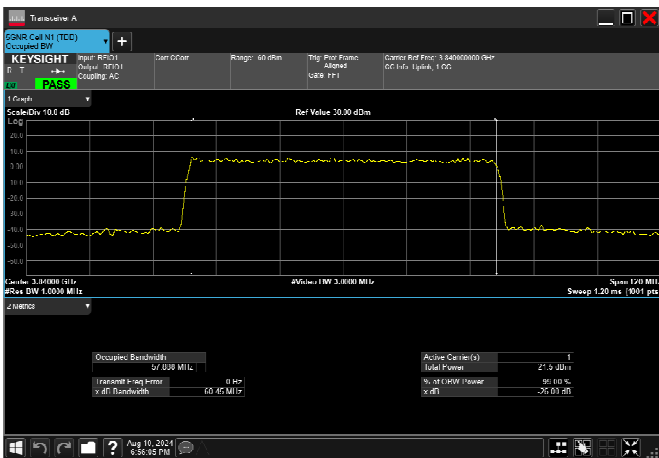
n77_3_60MHz_30kHz_3840MHz_CP-OFDM 64 QAM_RB162@0 57.888MHz
