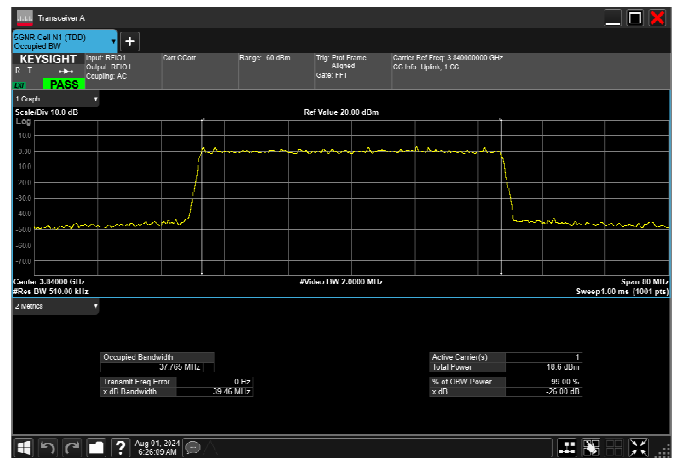
n77_3_40MHz_30kHz_3840MHz_CP-OFDM 256 QAM_RB106@0 37.765MHz
