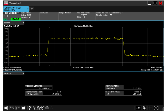
n77_3_60MHz_30kHz_3840MHz_DFT-s-OFDM \pi/2 BPSK_RB162@0 57.884MHz
