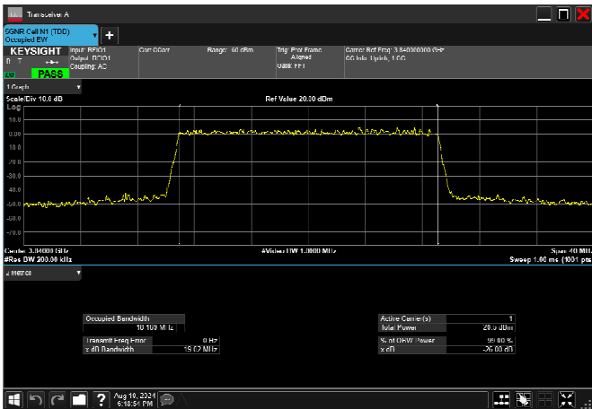
n77_3_20MHz_30kHz_3840MHz_CP-OFDM 64 QAM_RB51@0 18.169MHz
