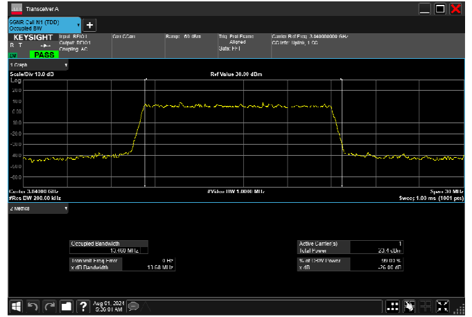
n77_3_15MHz_30kHz_3840MHz_DFT-s-OFDM 64 QAM_RB36@0 13.502MHz
