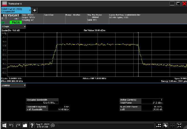
n77_3_15MHz_30kHz_3840MHz_CP-OFDM 256 QAM_RB38@0 13.525MHz
