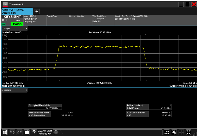
n77_3_30MHz_30kHz_3840MHz_DFT-s-OFDM 16 QAM_RB75@0 27.735MHz
