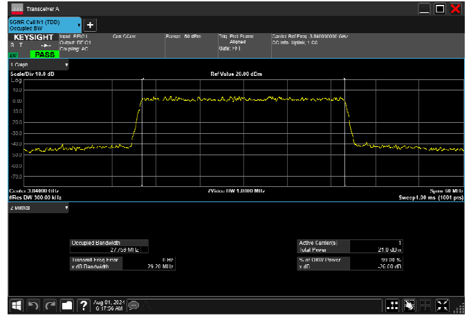
n77_3_40MHz_30kHz_3840MHz_DFT-s-OFDM \pi/2 BPSK_RB100@0 37.505MHz
