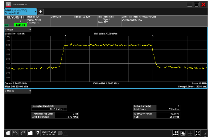
n77_3_20MHz_30kHz_3840MHz_CP-OFDM 16 QAM_RB51@0 18.183MHz
