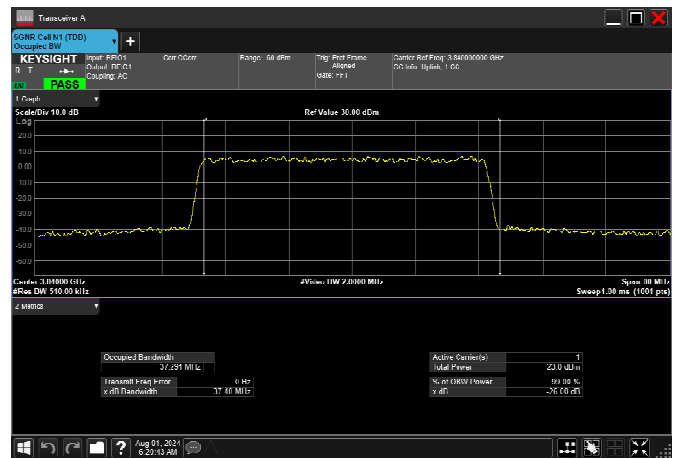
n77_3_40MHz_30kHz_3840MHz_DFT-s-OFDM 16 QAM_RB100@0 37.291MHz
