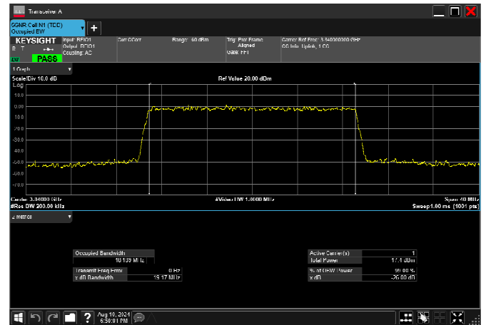
n77_3_20MHz_30kHz_3840MHz_CP-OFDM 256 QAM_RB51@0 18.189MHz
