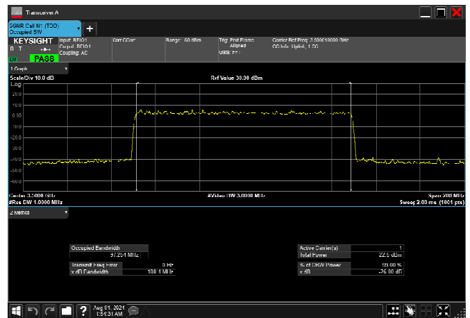
n77_1_100MHz_30kHz_3500MHz_CP-OFDM QPSK_RB273@0 97.254MHz
