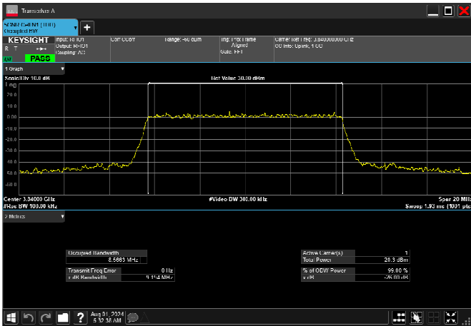
n77_3_10MHz_30kHz_3840MHz_CP-OFDM 64 QAM_RB24@0 8.568MHz
