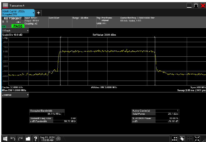
n77_1_100MHz_30kHz_3500MHz_DFT-s-OFDM 256 QAM_RB270@0 96.145MHz
