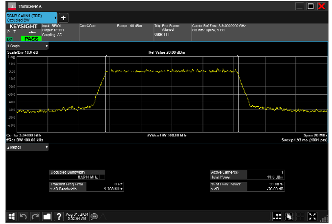
n77_3_10MHz_30kHz_3840MHz_CP-OFDM 16 QAM_RB24@0 8.540MHz
