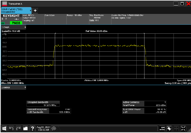
n77_1_100MHz_30kHz_3500MHz_CP-OFDM 16 QAM_RB273@0 97.276MHz
