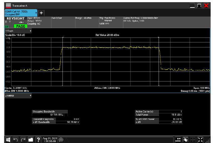
n77_1_90MHz_30kHz_3500MHz_CP-OFDM 256 QAM_RB245@0 87.196MHz
