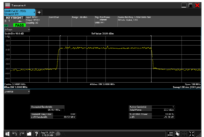
n77_1_90MHz_30kHz_3500MHz_DFT-s-OFDM 16 QAM_RB243@0 86.467MHz
