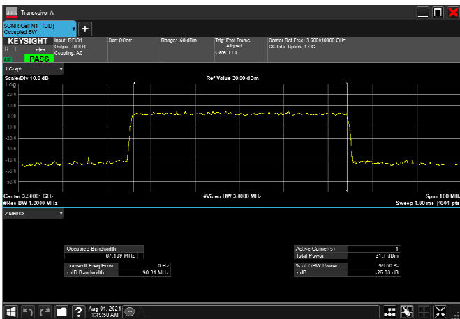
n77_1_90MHz_30kHz_3500MHz_CP-OFDM 64 QAM_RB245@0 87.189MHz
