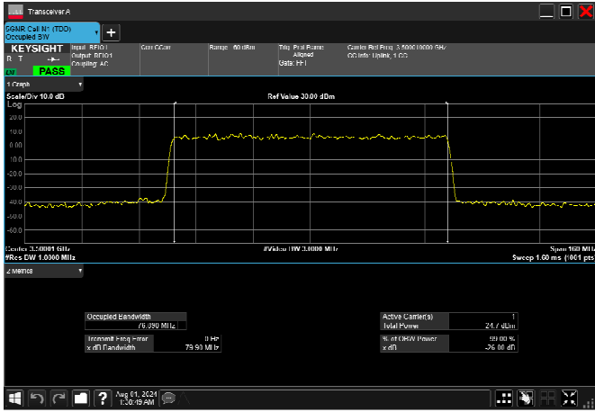
n77_1_80MHz_30kHz_3500MHz_DFT-s-OFDM 16 QAM_RB216@0 76.910MHz
