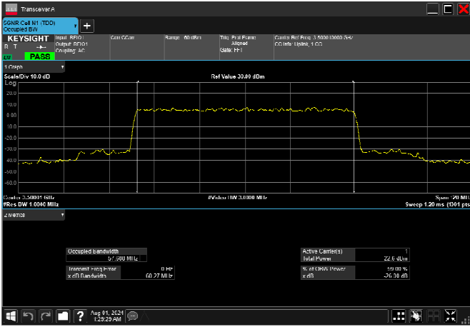
n77_1_60MHz_30kHz_3500MHz_CP-OFDM 256 QAM_RB162@0 57.713MHz
