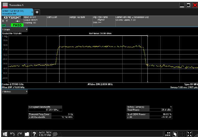
n38_40MHz_30kHz_2595MHz_DFT-s-OFDM 256 QAM_RB100@0 37.290MHz
