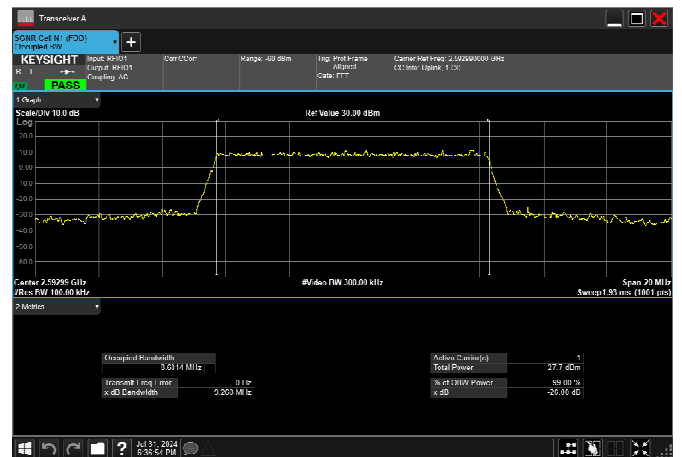
n41_10MHz_30kHz_2592.99MHz_DFT-s-OFDM 16 QAM_RB24@0 8.601MHz
