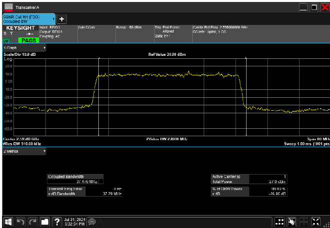
n38_40MHz_30kHz_2595MHz_DFT-s-OFDM 16 QAM_RB100@0 37.291MHz
