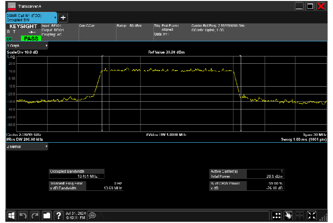
n41_15MHz_30kHz_2592.99MHz_DFT-s-OFDM 64 QAM_RB36@0 13.456MHz
