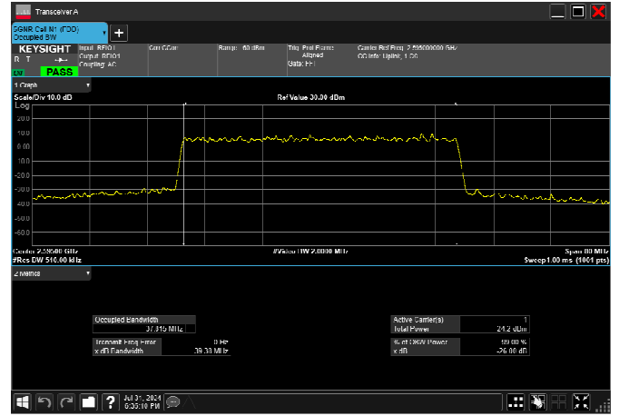
n38_40MHz_30kHz_2595MHz_CP-OFDM 64 QAM_RB106@0 37.815MHz
