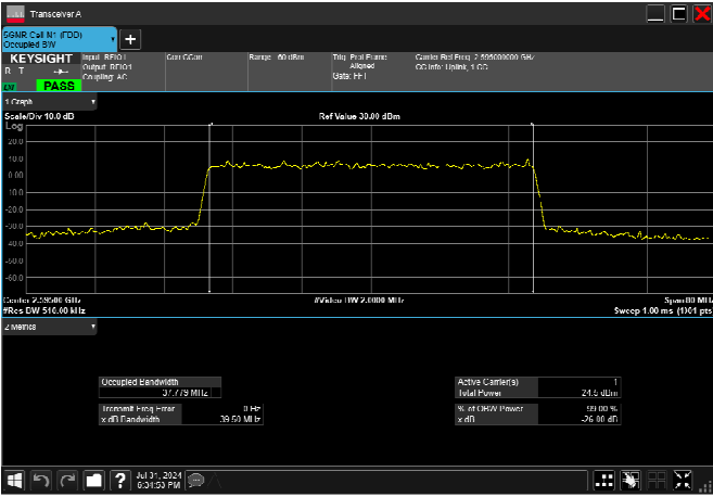
n38_40MHz_30kHz_2595MHz_CP-OFDM 16 QAM_RB106@0 37.779MHz
