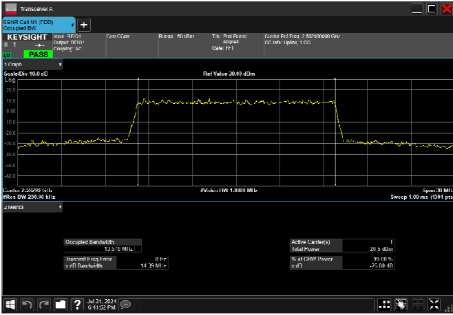
n41_15MHz_30kHz_2592.99MHz_CP-OFDM 256 QAM_RB38@0 13.560MHz
