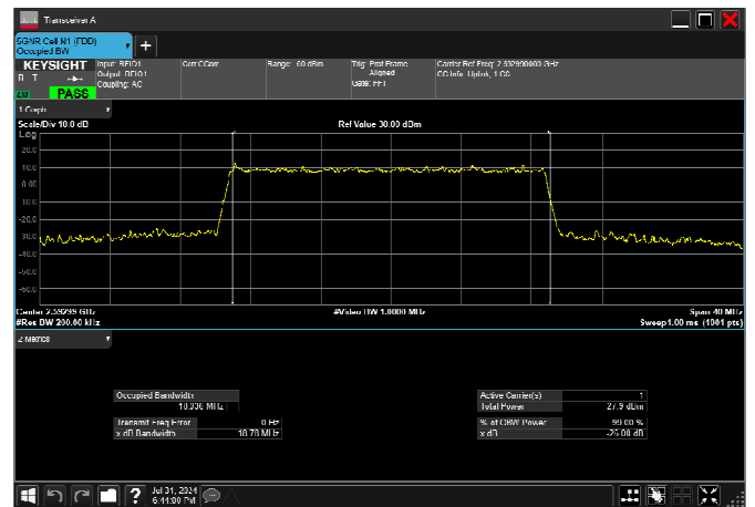
n41_20MHz_30kHz_2592.99MHz_DFT-s-OFDM 16 QAM_RB50@0 18.036MHz
