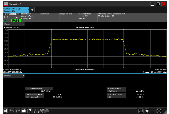
n38_15MHz_30kHz_2595MHz_CP-OFDM QPSK_RB38@0 13.571MHz
