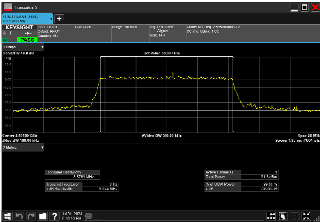
n38_10MHz_30kHz_2595MHz_CP-OFDM 64 QAM_RB24@0 8.567MHz
