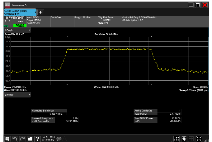
n38_10MHz_30kHz_2595MHz_DFT-s-OFDM 16 QAM_RB24@0 8.565MHz
