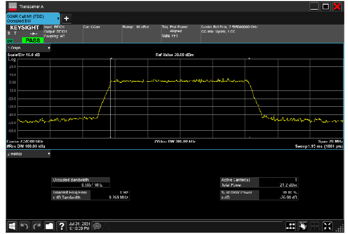
n38_10MHz_30kHz_2595MHz_CP-OFDM 16 QAM_RB24@0 8.573MHz
