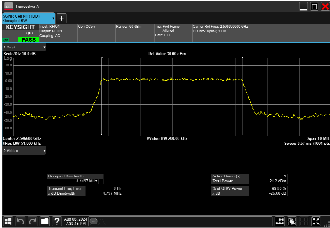
n38_5MHz_15kHz_2595MHz_DFT-s-OFDM 16 QAM_RB25@0 4.467MHz
