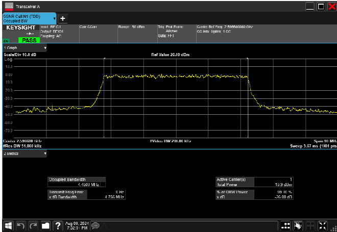
n38_5MHz_15kHz_2595MHz_CP-OFDM 256 QAM_RB25@0 4.469MHz
