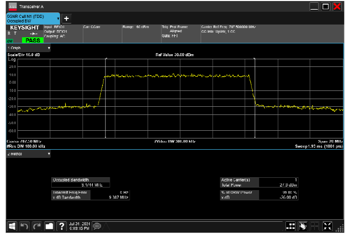
n12_10MHz_15kHz_707.5MHz_CP-OFDM 16 QAM_RB52@0 9.299MHz
