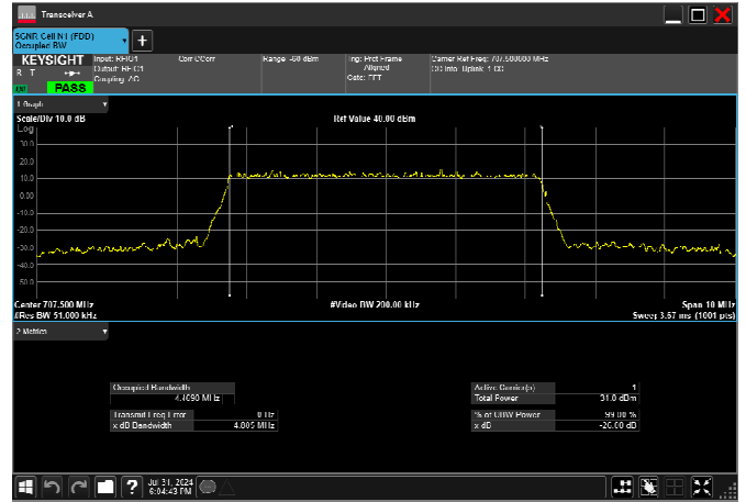
n12_5MHz_15kHz_707.5MHz_DFT-s-OFDM 64 QAM_RB25@0 4.487MHz
