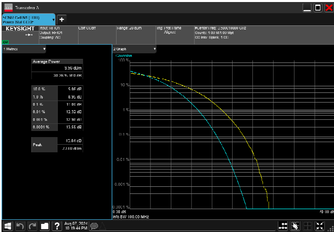
n78_1_100MHz_30kHz_3500MHz_CP-OFDM 64 QAM_RB273@0 11.07dB
