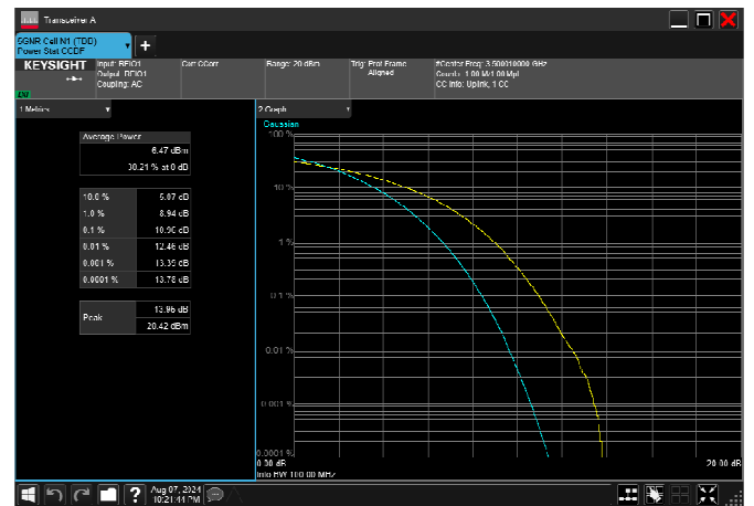
n78_1_100MHz_30kHz_3500MHz_CP-OFDM 256 QAM_RB273@0 10.96dB
