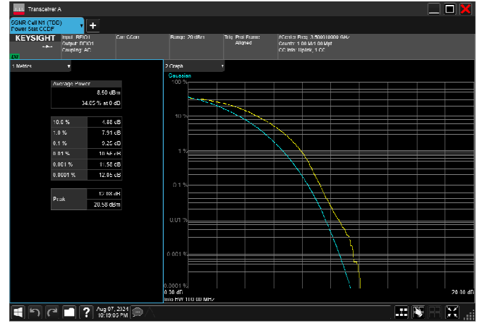
n78_1_100MHz_30kHz_3500MHz_CP-OFDM 16 QAM_RB273@0 11.09dB
