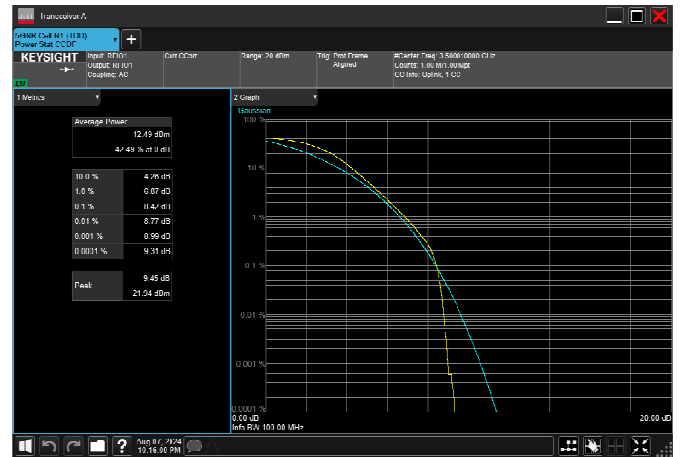
n78_1_100MHz_30kHz_3500MHz_DFT-s-OFDM 16 QAM_RB270@0 9.10dB
