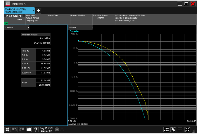
n77_1_100MHz_30kHz_3500MHz_CP-OFDM 16 QAM_RB273@0 11.12dB
