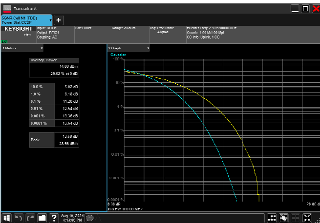
n41_100MHz_30kHz_2592.99MHz_CP-OFDM 64 QAM_RB273@0 11.28dB
