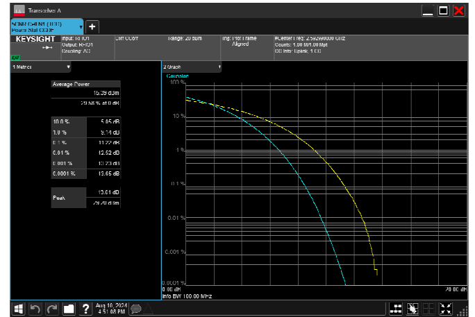
n41_100MHz_30kHz_2592.99MHz_CP-OFDM 256 QAM_RB273@0 11.25dB
