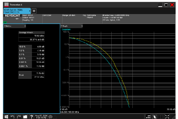
n77_1_100MHz_30kHz_3500MHz_DFT-s-OFDM 16 QAM_RB270@0 9.10dB
