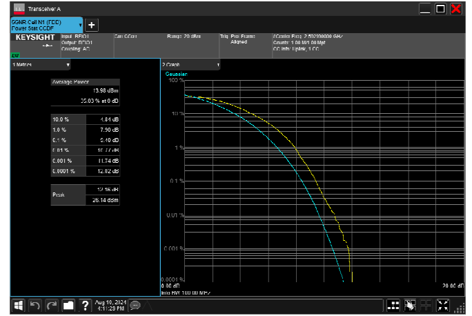
n41_100MHz_30kHz_2592.99MHz_CP-OFDM 16 QAM_RB273@0 11.22dB
