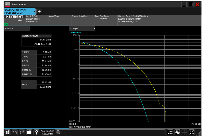
n38_40MHz_30kHz_2595MHz_CP-OFDM 64 QAM_RB106@0 11.34dB
