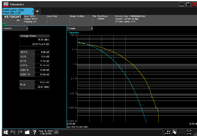
n38_40MHz_30kHz_2595MHz_CP-OFDM 16 QAM_RB106@0 11.12dB
