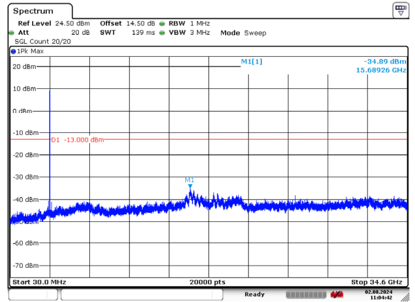
1_20MHz_Low_QPSK_100@0 -34.89dBm
