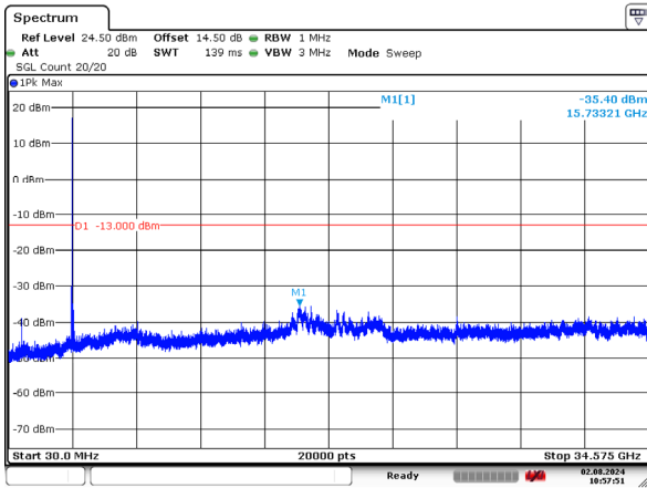
1_15MHz_Low_QPSK_1@0 -35.40dBm
