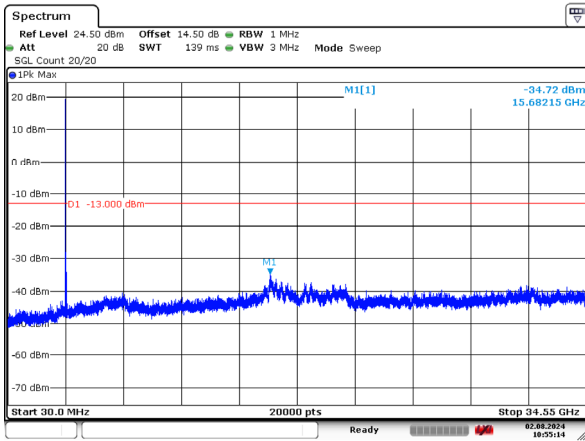
1_10MHz_Low_QPSK_1@0 -34.72dBm
