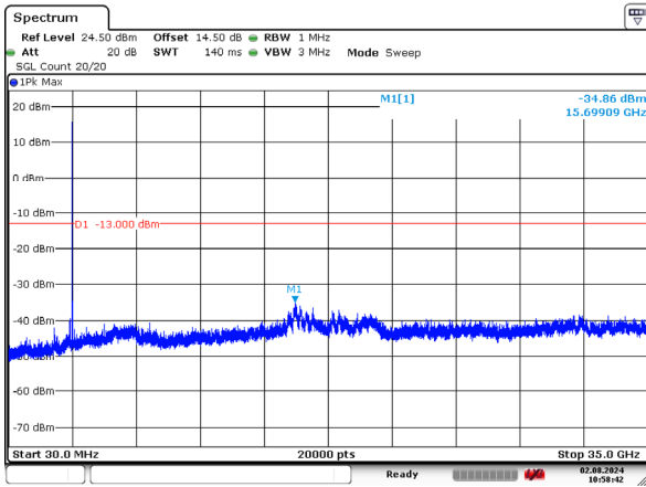
1_15MHz_Middle_QPSK_1@0 -34.86dBm
