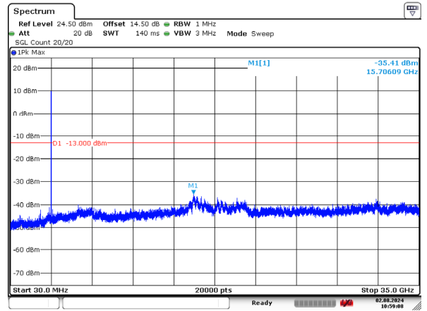
1_15MHz_Middle_QPSK_75@0 -35.41dBm
