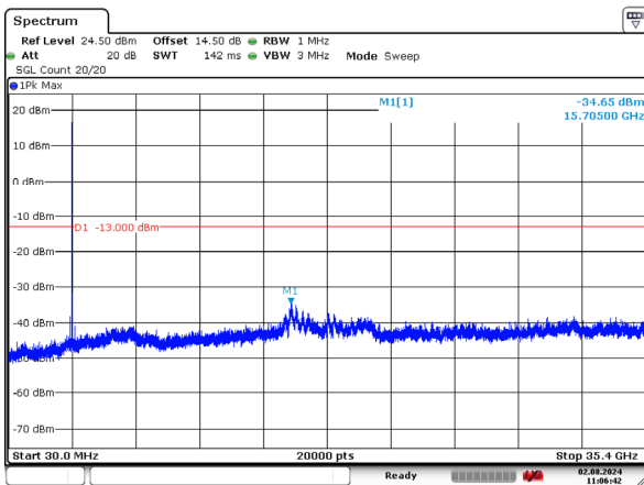
1_20MHz_High_QPSK_1@0 -34.65dBm
