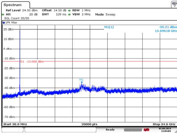
1_20MHz_Low_QPSK_1@0 -35.21dBm
