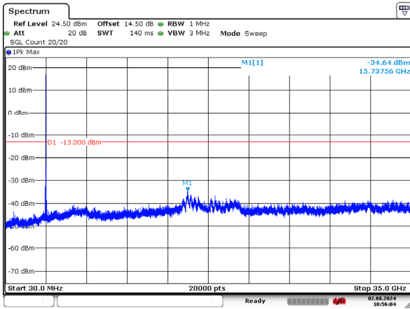
1_10MHz_Middle_QPSK_1@0 -34.64dBm
