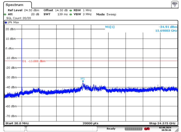
1_15MHz_Low_QPSK_75@0 -34.91dBm
