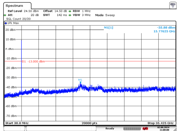
1_15MHz_High_QPSK_75@0 -35.88dBm
