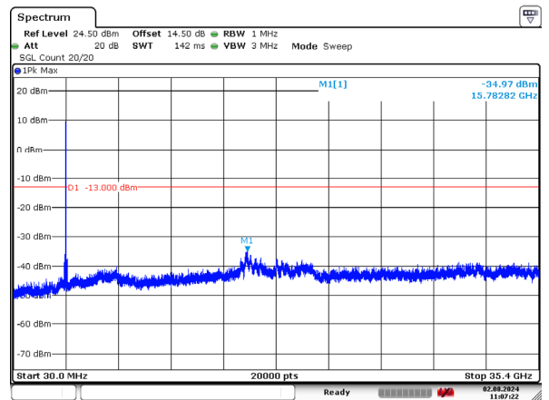
1_20MHz_High_QPSK_100@0 -34.97dBm
