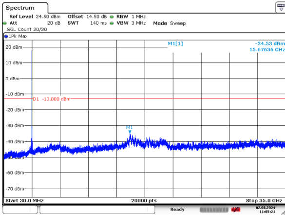
1_20MHz_Middle_QPSK_1@0 -34.53dBm
