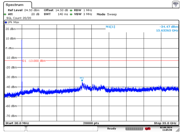
1_20MHz_Middle_QPSK_100@0 -34.47dBm
