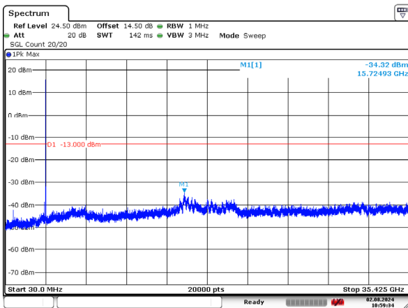
1_15MHz_High_QPSK_1@0 -34.32dBm
