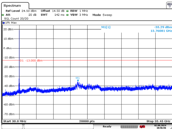
1_10MHz_High_QPSK_1@0 -35.29dBm
